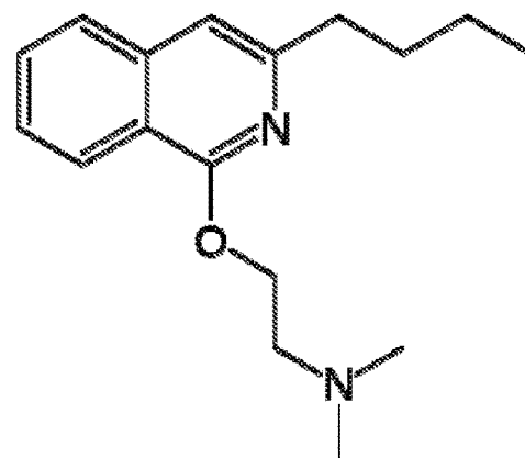
QUINISOCAINE
