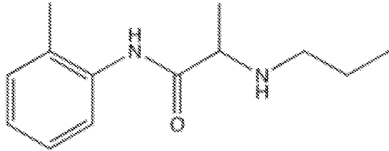
PRILOCAINE
