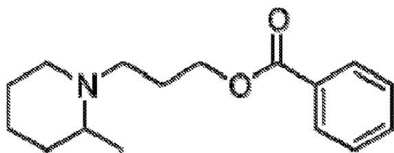
PIPEROCAINE
