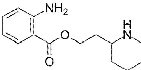
PIRIDOCAINE
