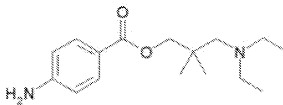
DIMETHOCAINE
