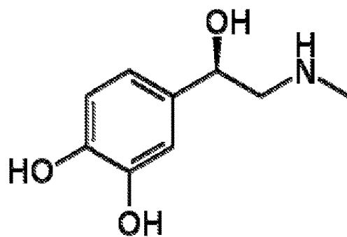
EPINEPHRINE
