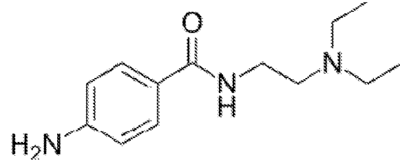
PROCAINAMIDE
