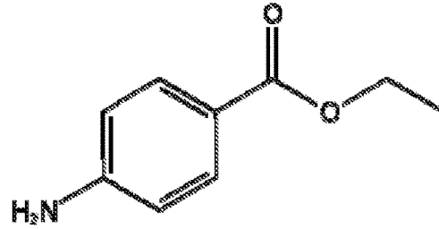
BENZOCAINE
