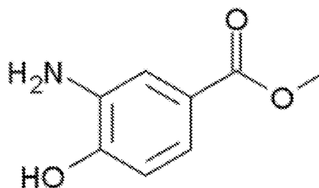
ORTHOCAINE
