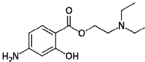
HYDROXYPROCAINE
