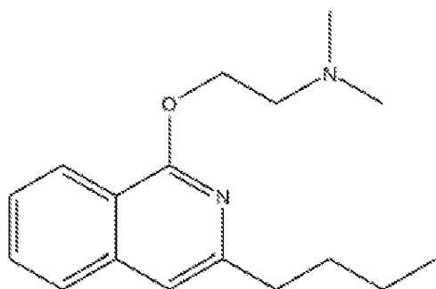
DIMETHISOQUIN
