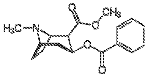
COCAINE
