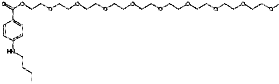
BENZONATATE
