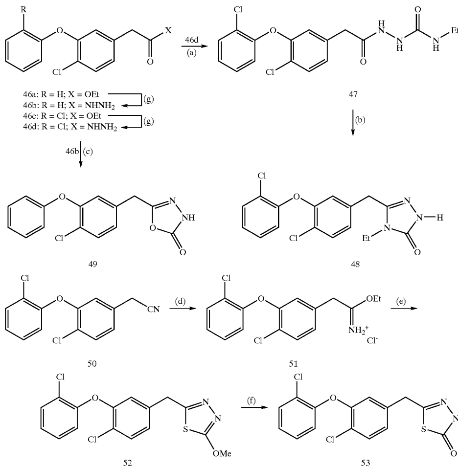
SCHEME 13
