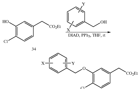
SCHEME 11
