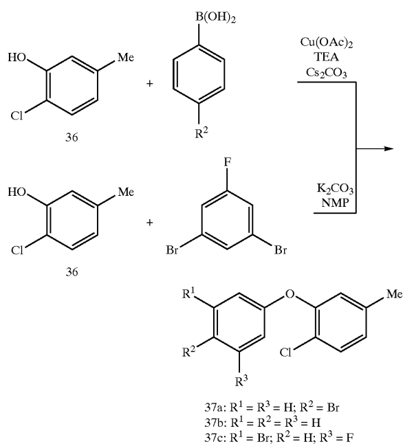
SCHEME 9
