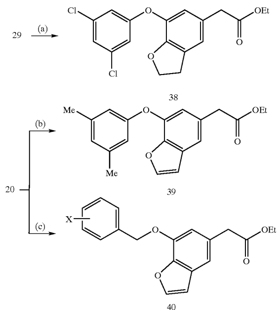
SCHEME 10
