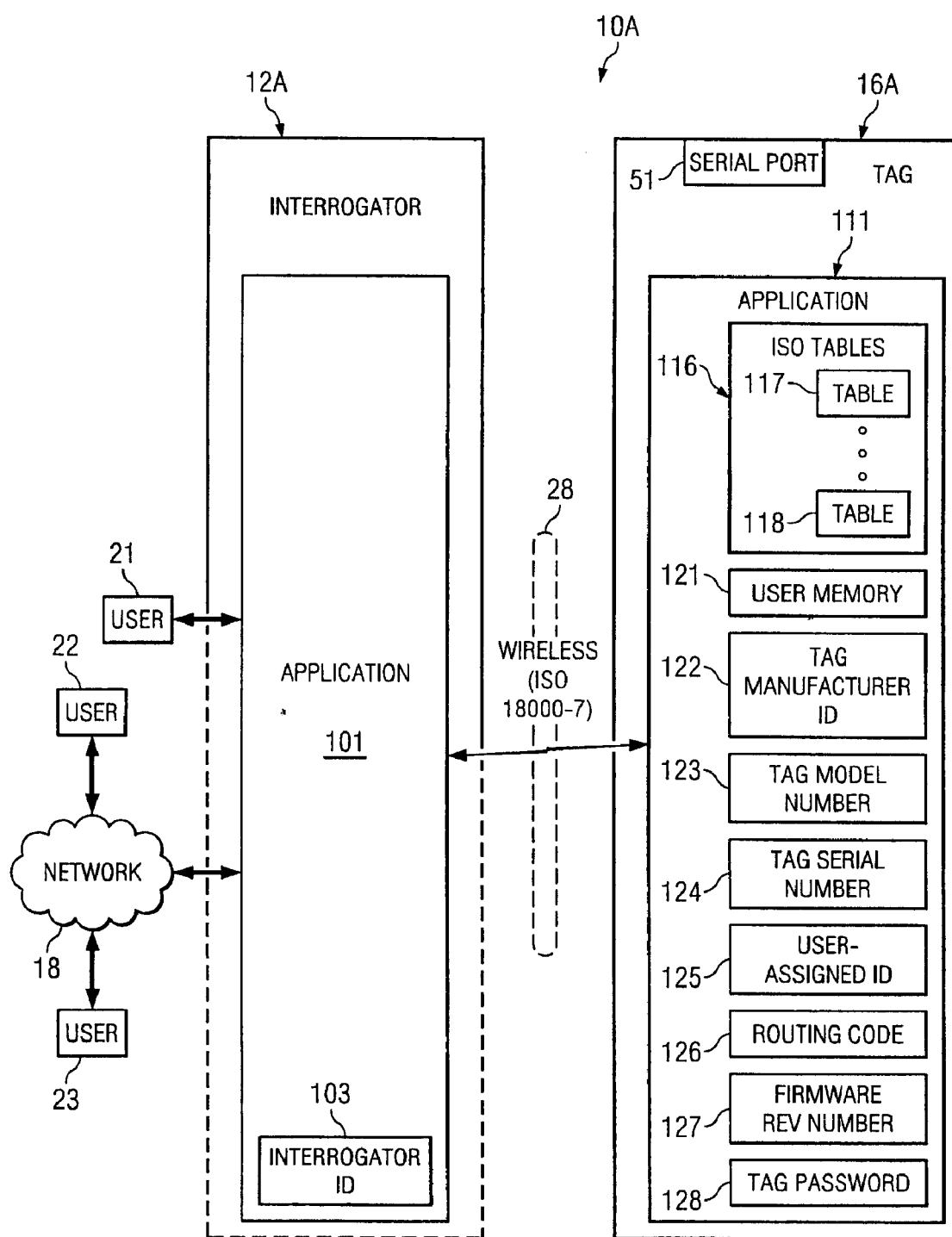
Fig. 2 (PRIOR ART)
