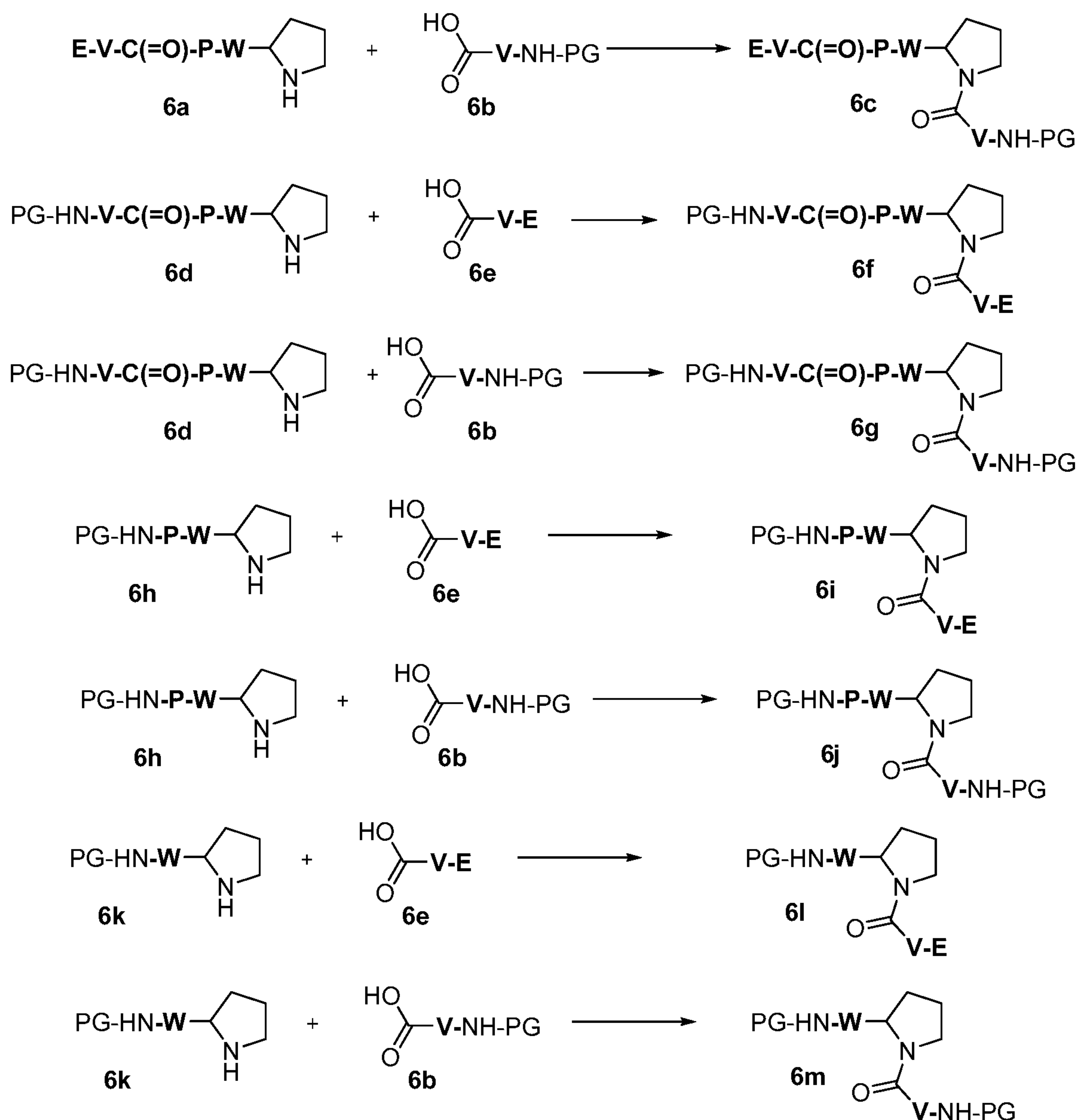
Scheme 6. Representative synthesis of R^1-V-C(=O)-P-R^2
