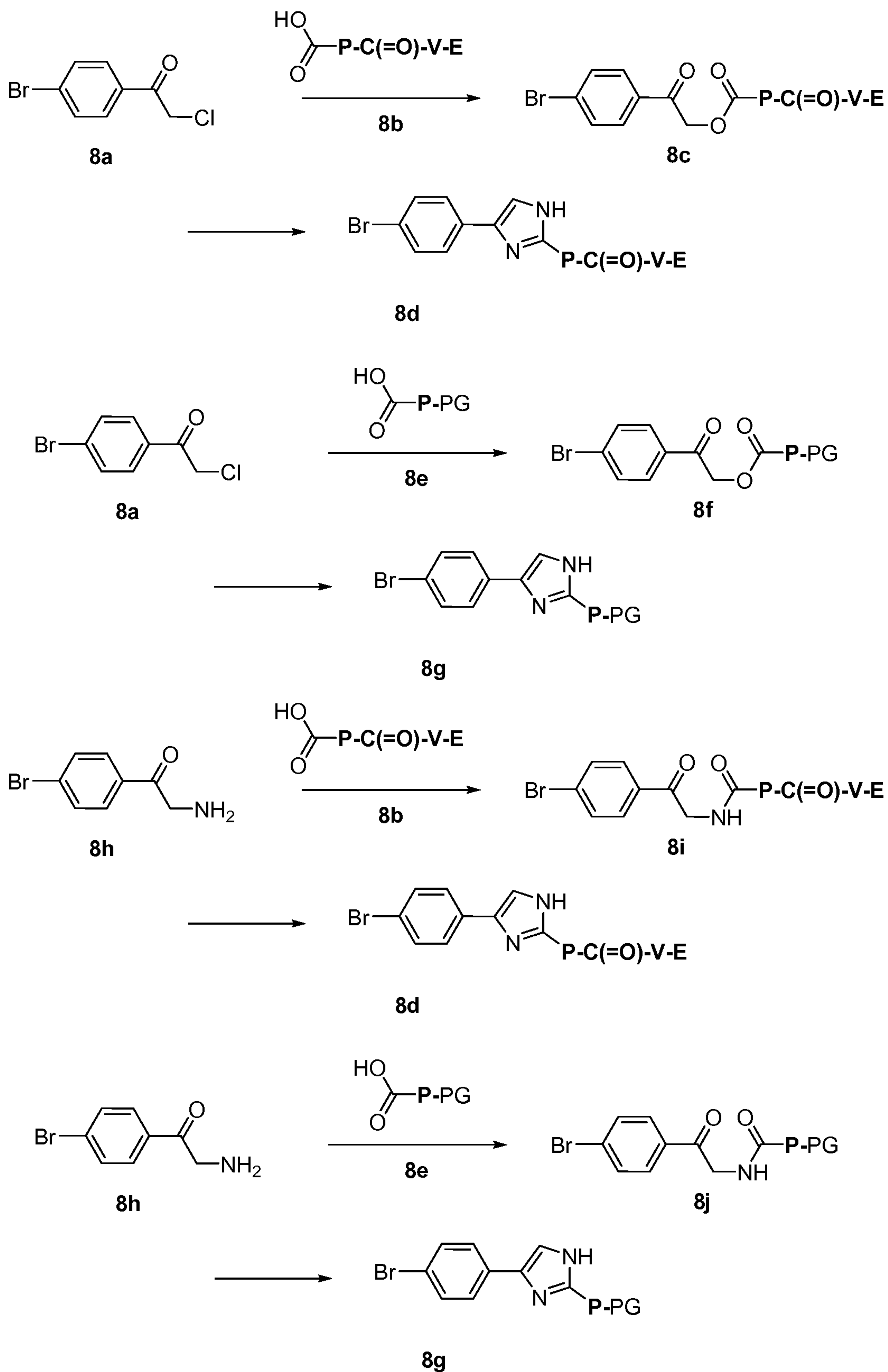
Scheme 8. Representative synthesis of R^1 -P- R^2
