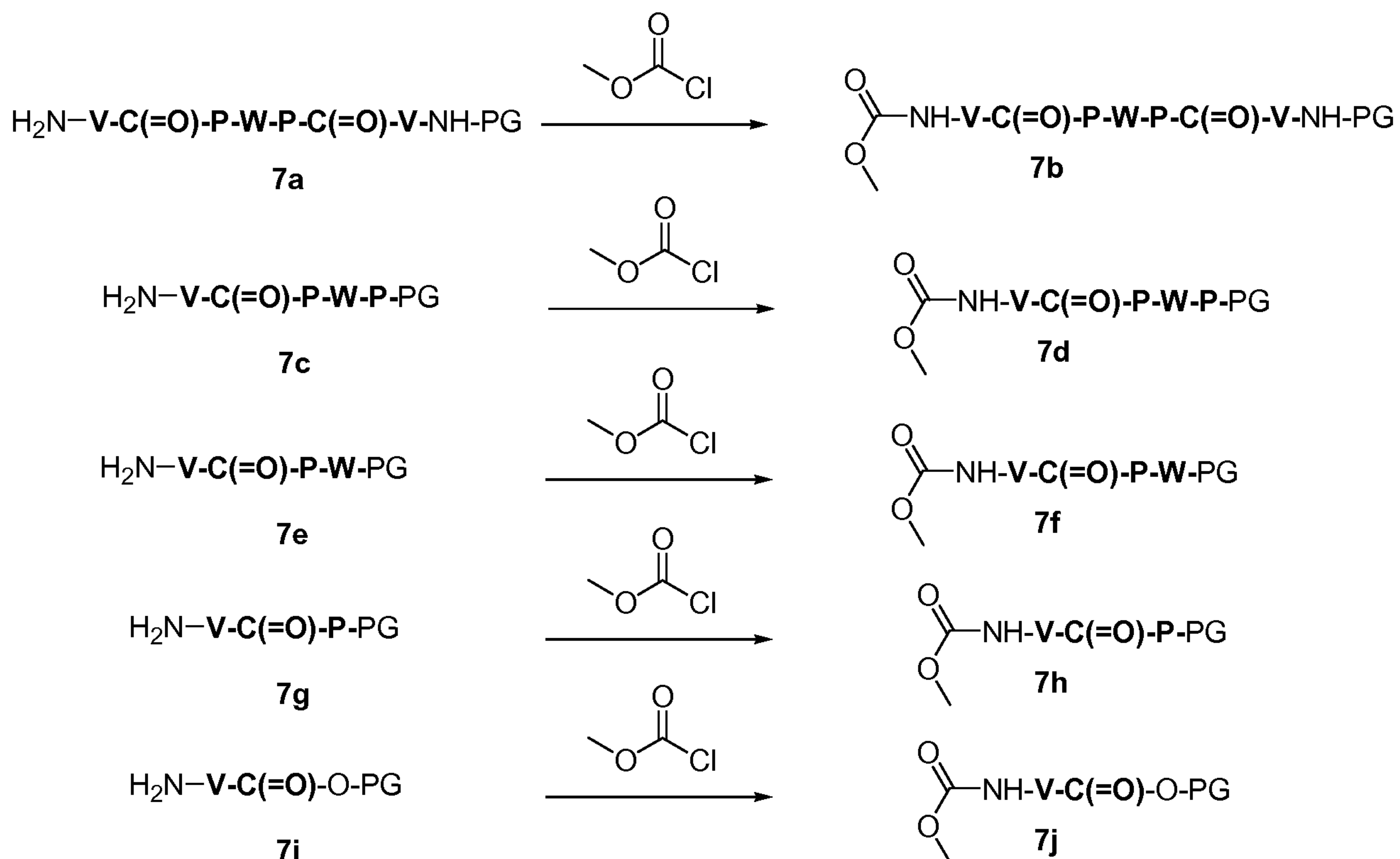
Scheme 7. Representative synthesis of E-V-C(=O)- R^1
