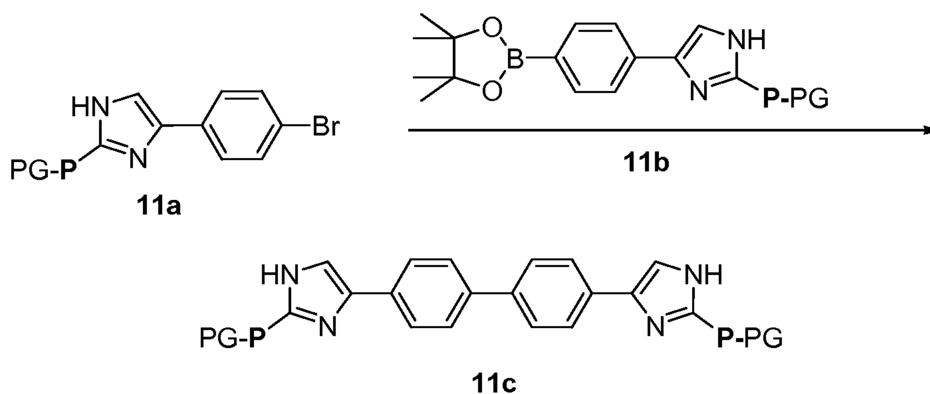
Scheme 11. Representative synthesis of R 1 -P-W-P-R 2
