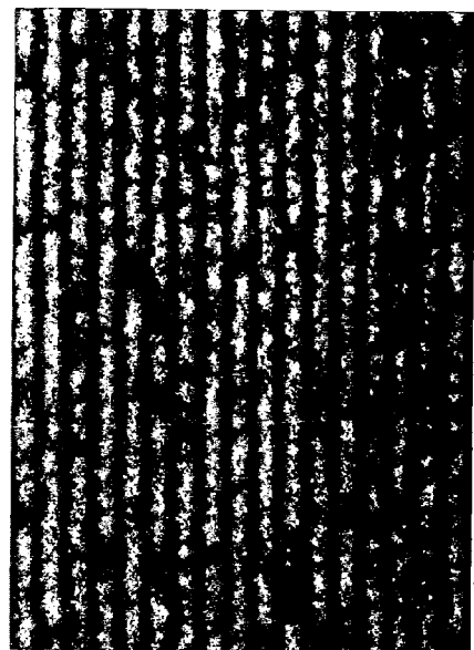
Figs 9a-c: SEM Images of 50 nm Patterned Polystyrene Brushes G = .7 \text{ chains/nm}^2
