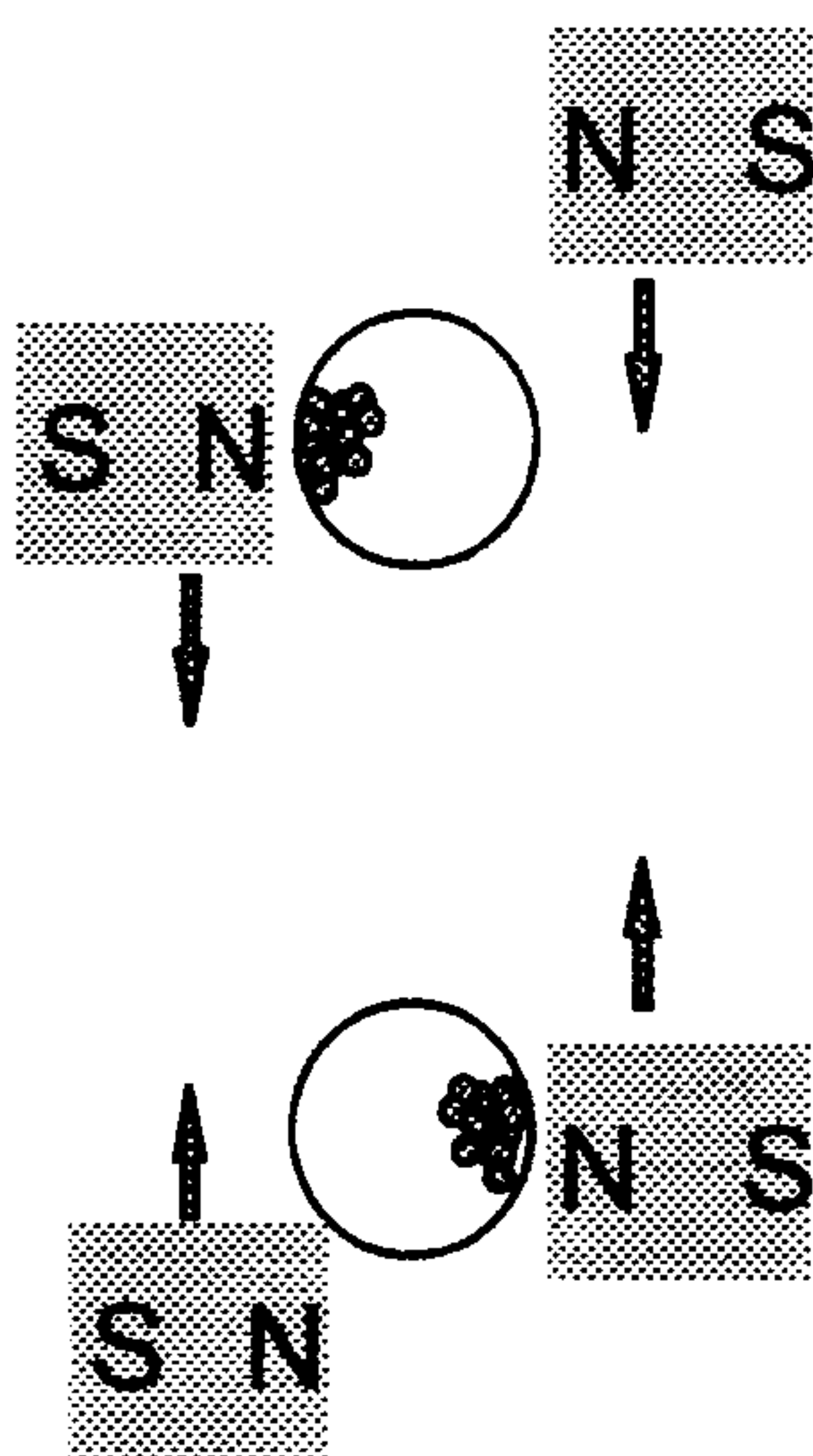
Top view
