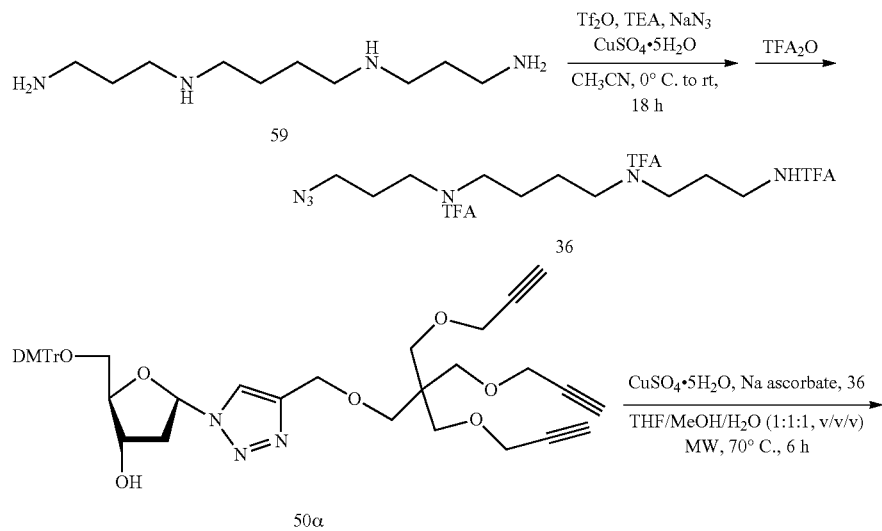
Scheme 3: Synthesis of polyamine azide (36), its CuAA with 50 \alpha and synthesis of amidite 61a and CPG 63 \alpha .
