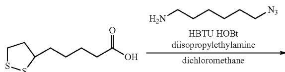
Scheme 11. Synthesis of azide 43
