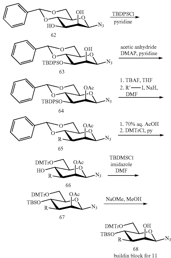
Scheme 14.: Synthesis of azide 11 following the literature procedure 37-38 .
