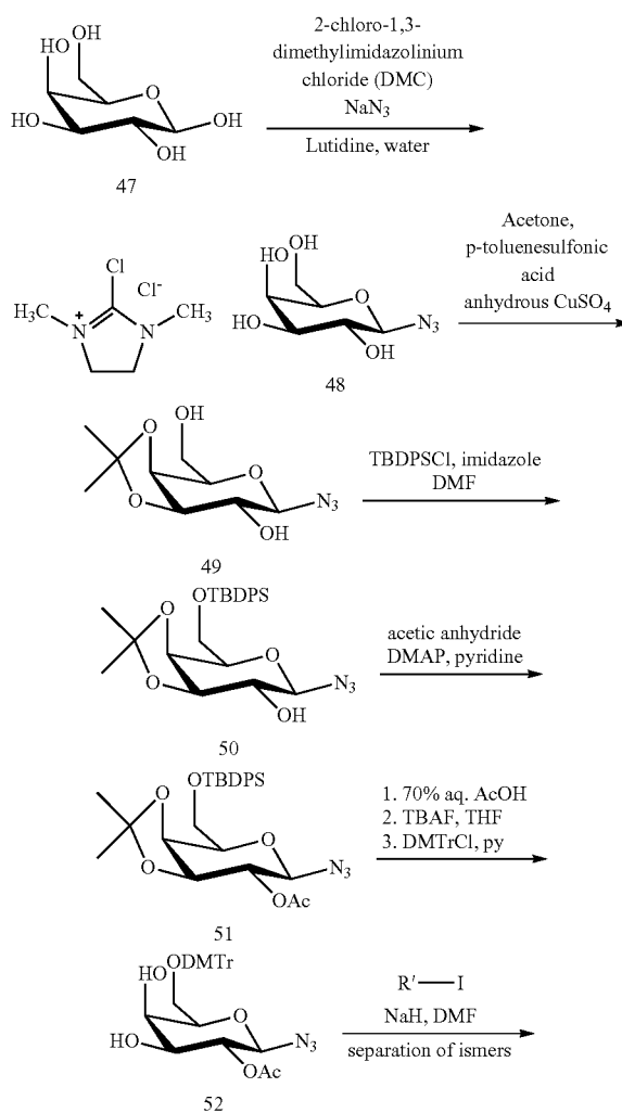
Scheme 13: Synthesis of azide 3-5. Compound 48 was obtained following the literature procedure 35 . Azides 6-9 synthesized following the same synthetic route.
