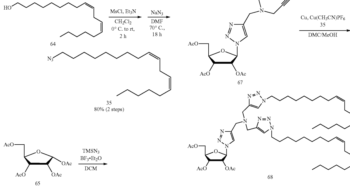
Scheme 4: Synthesis of linoleyl azide (35), anomeric azide scaffold (66 24 ), di-valent alkyne scaffold (67) and lipophilic conjugate (68).
