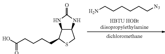
Scheme 12. Synthesis of azide 46
