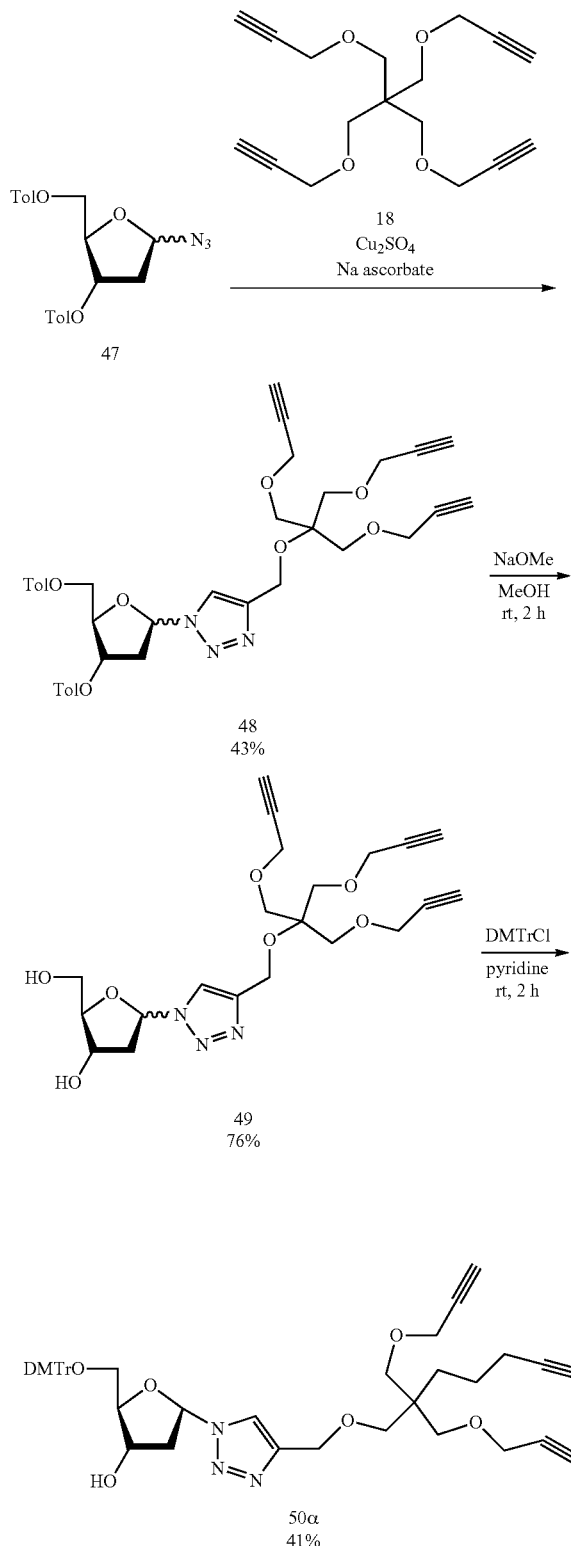
Scheme 1: Synthesis of amidites and CPGs for trivalent conjugation site.
