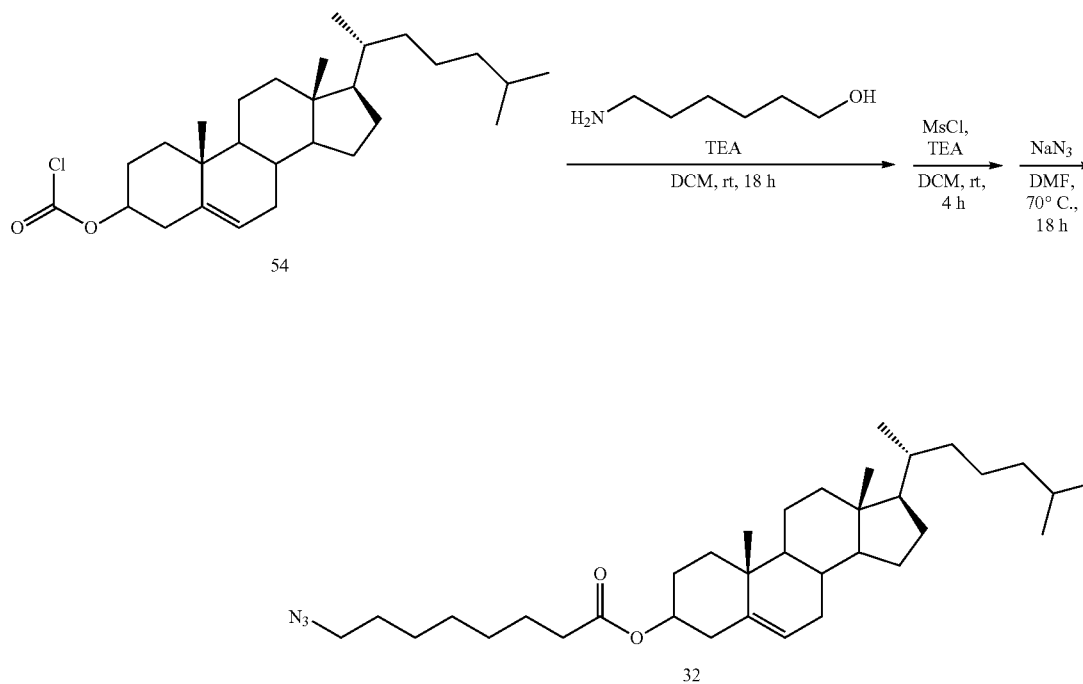
Scheme 2: Synthesis of cholesterol azide (32), its CuAAC with a 50a and synthesis of amidite 56a and CPG 58a.
