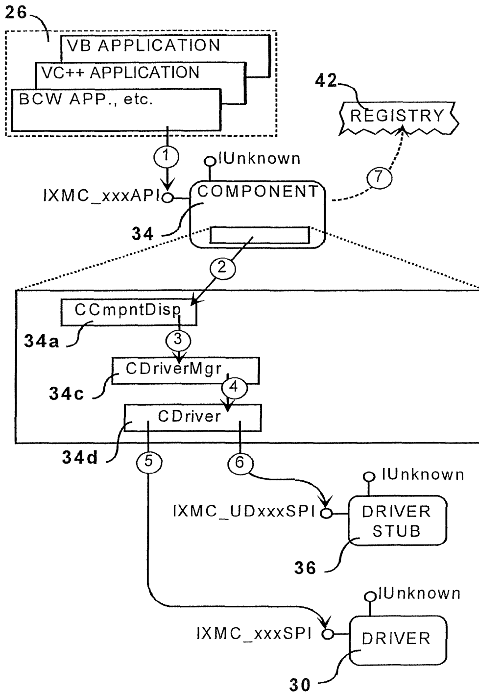
FIG. 8 Scenario-Map - Clean-up.
