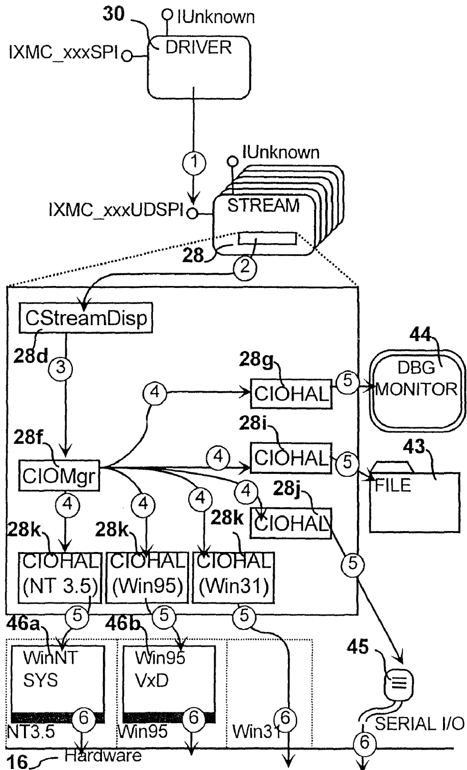
FIG. 30 Scenario-Map - Writing Data
