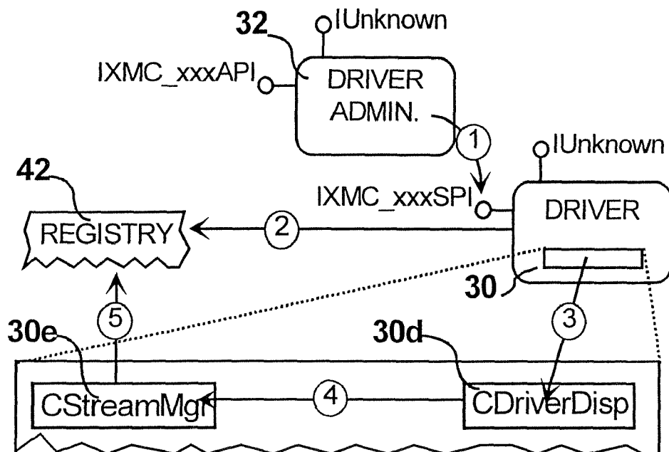
FIG. 14 Scenario-Map - Init. by Driver Admin.
