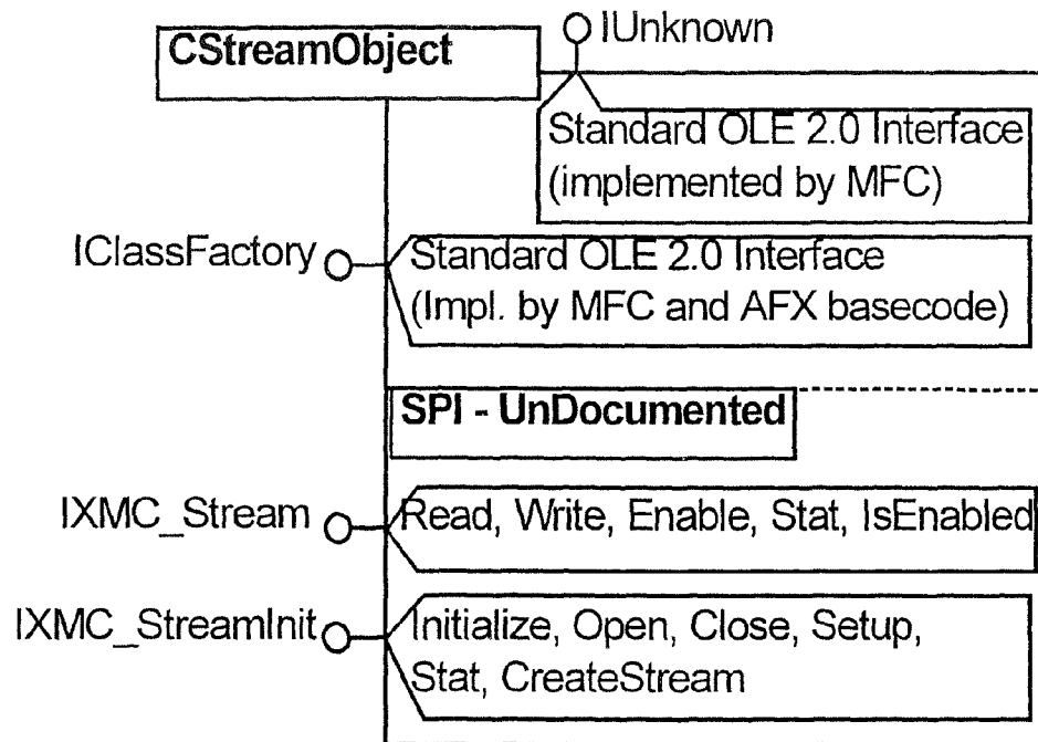
FIG. 33 Interface-Map
