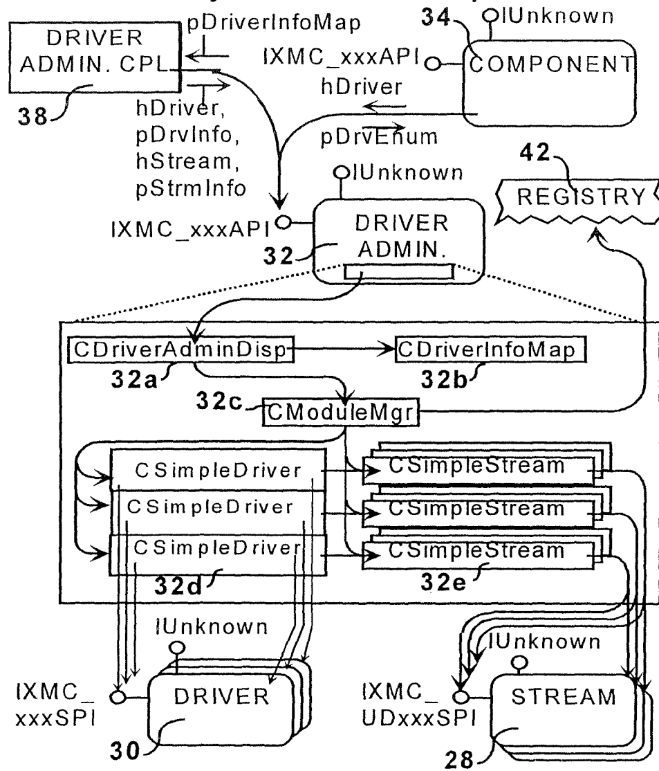
FIG. 41 Object Interaction-Map
