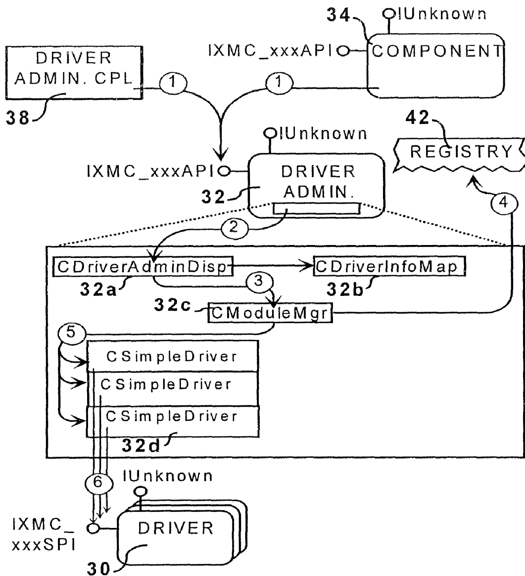
FIG. 42 Scenario-Map - Initialization
