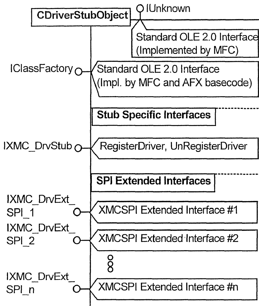
FIG. 39 Interface-Map
