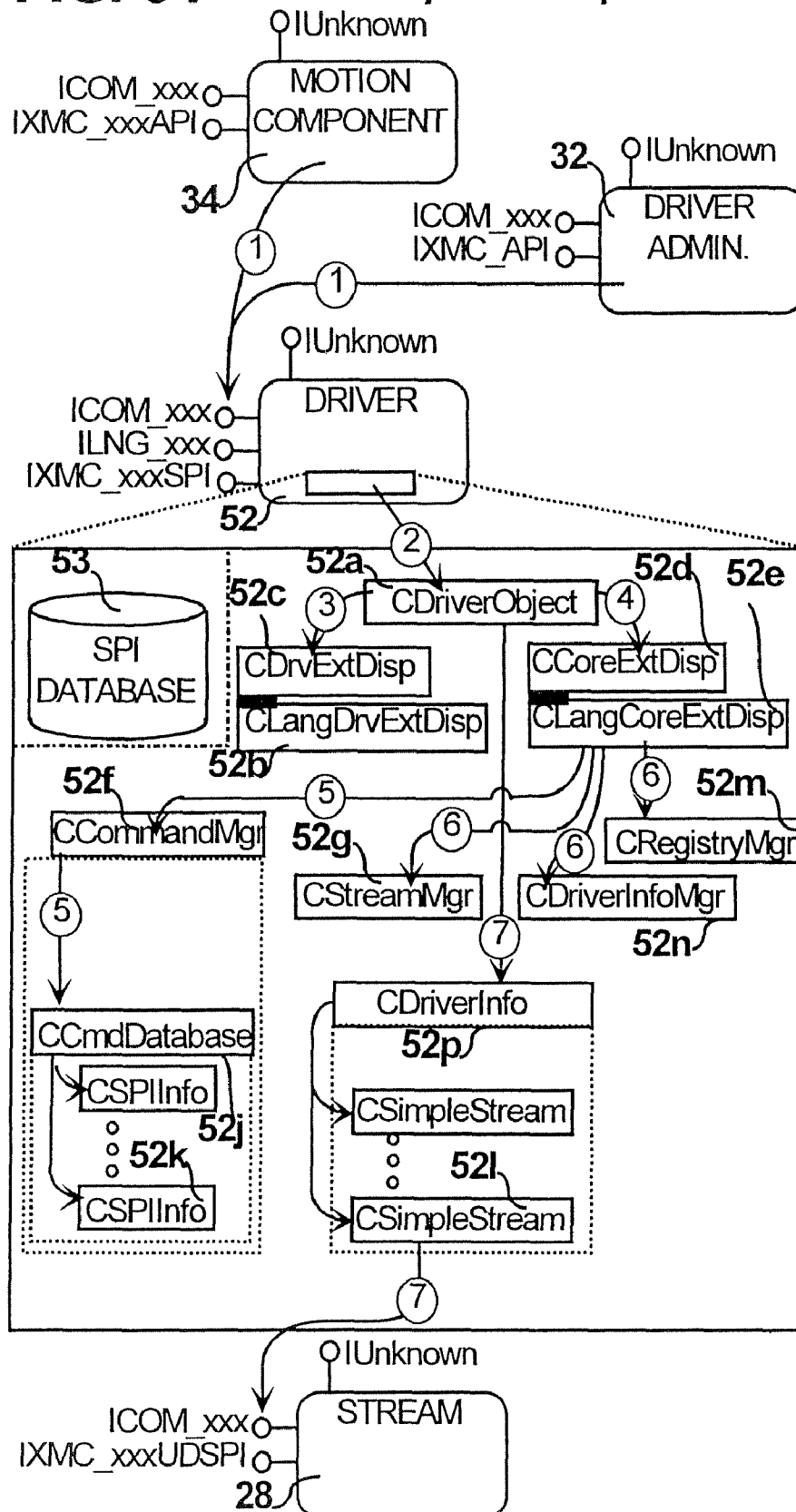
FIG. 64 Scenario-Map - Clean-up
