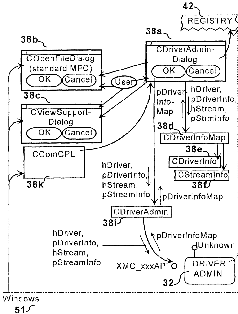
FIG. 52 Object Interaction-Map
