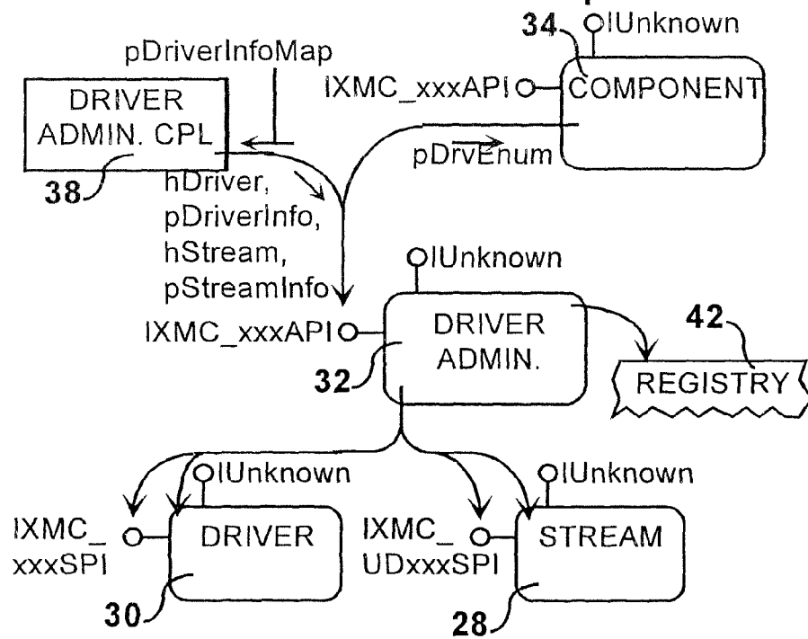
FIG. 40 Module Interaction-Map
