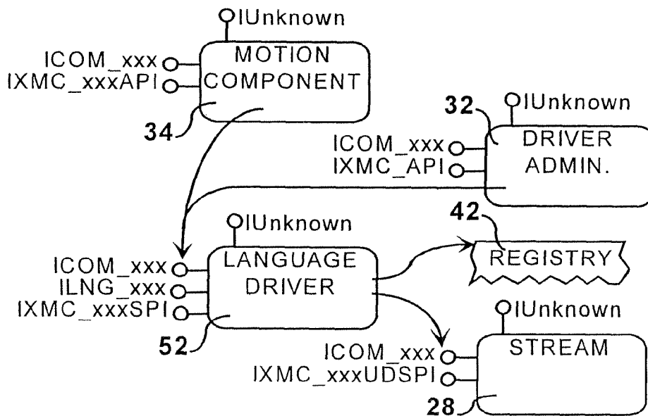
FIG. 58 Module Interaction-Map
