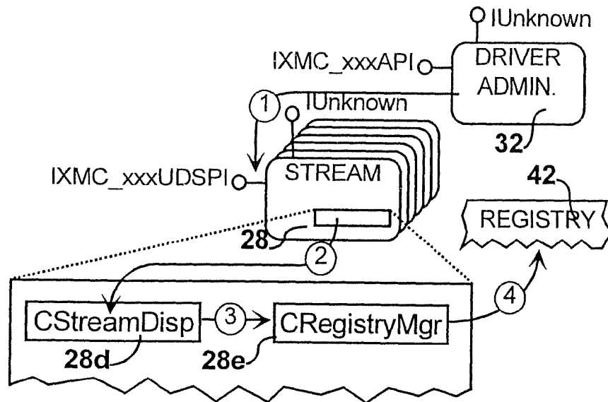
FIG. 27 Scenario-Map - Clean-up
