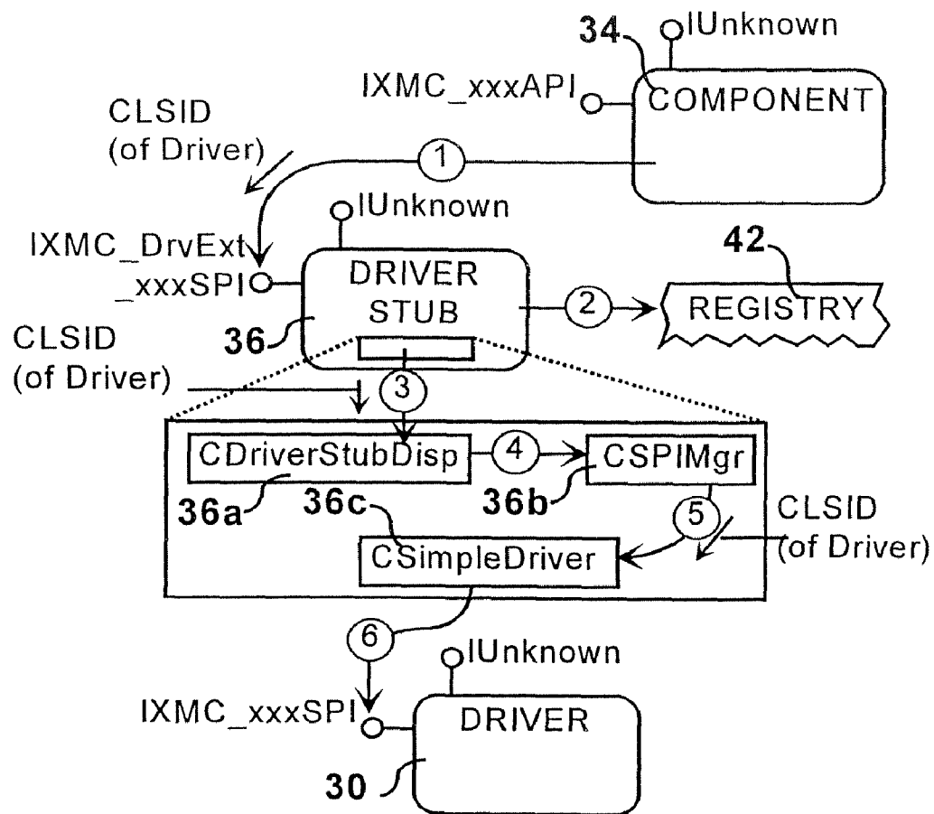
FIG. 36 Scenario-Map - Initialization
