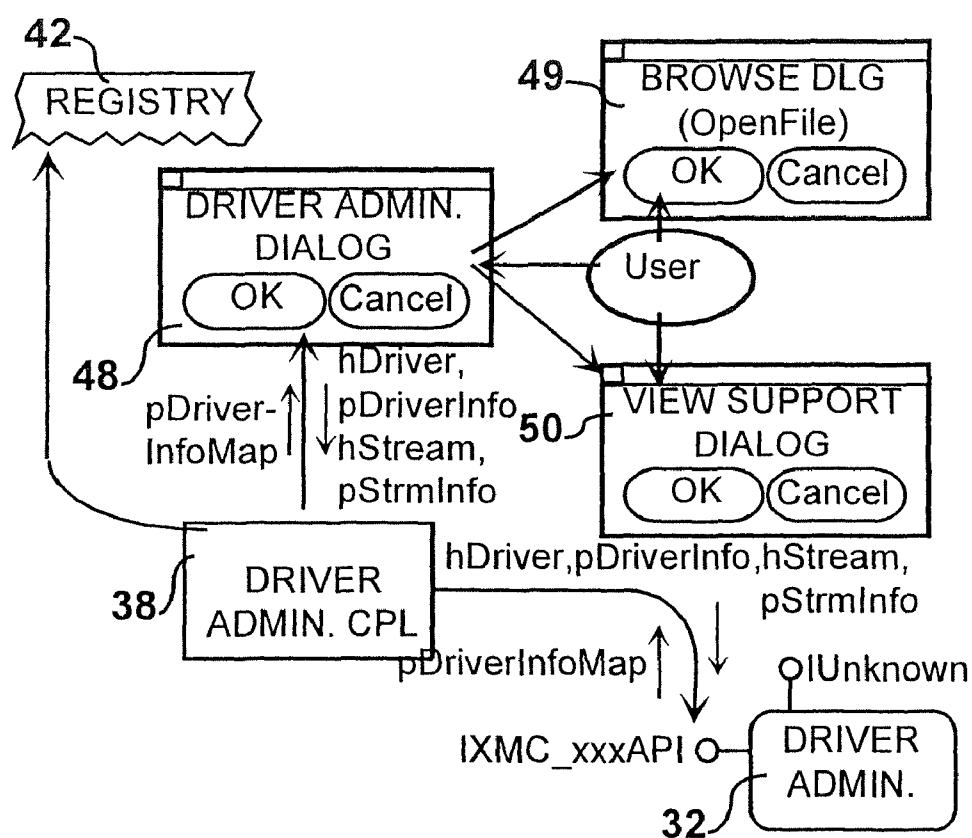
FIG. 51 Module Interaction-Map
