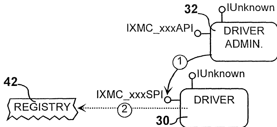
FIG. 13 Scenario-Map - Registration
