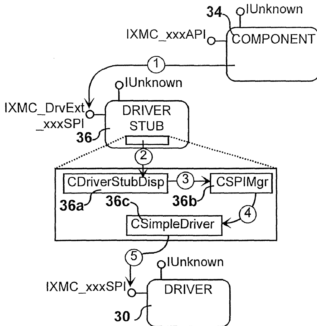
FIG. 38 Scenario-Map - Clean-up
