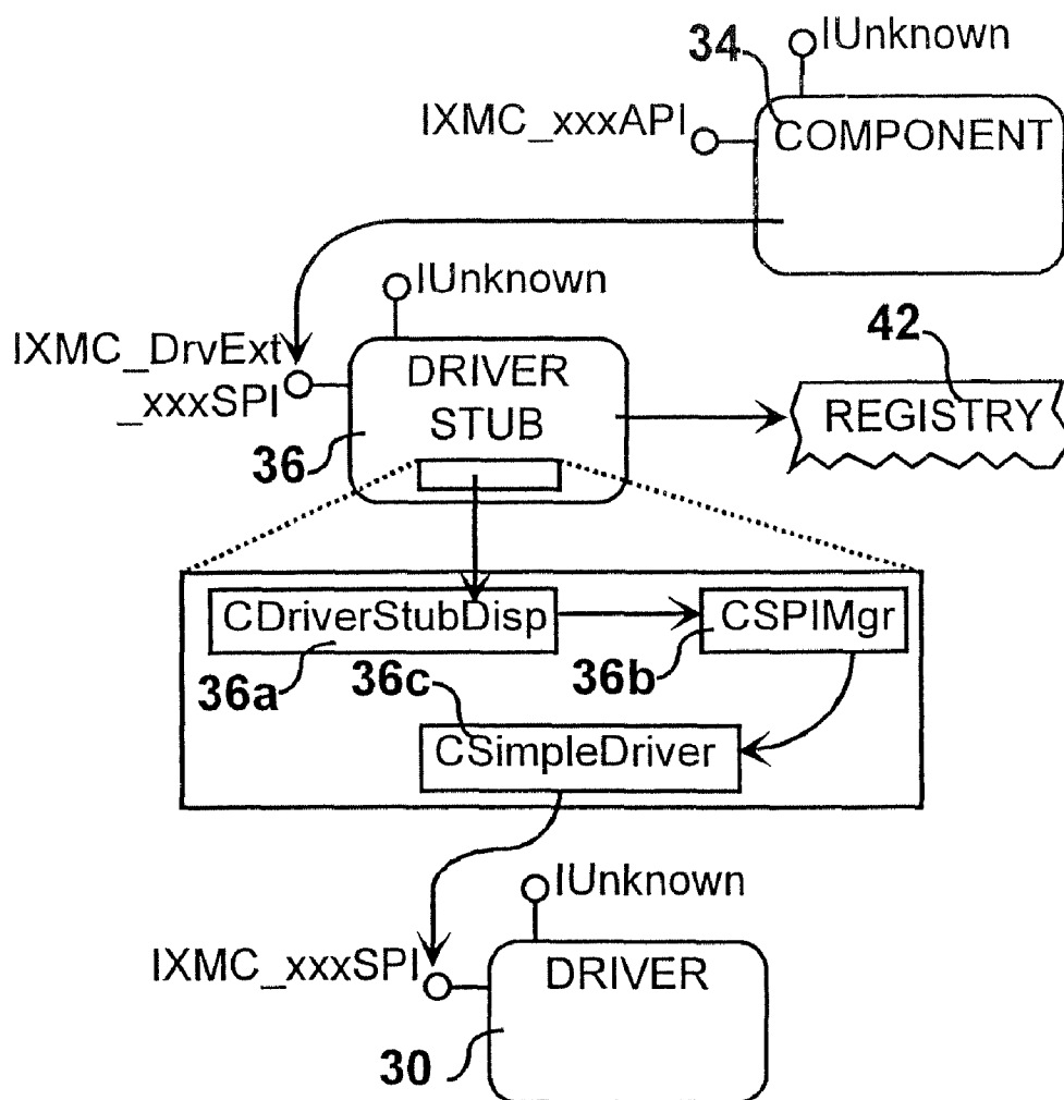
FIG. 35 Object Interaction-Map
