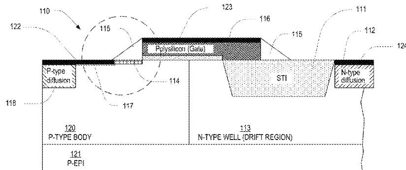
Hybrid Contact LDMOS Transistor
