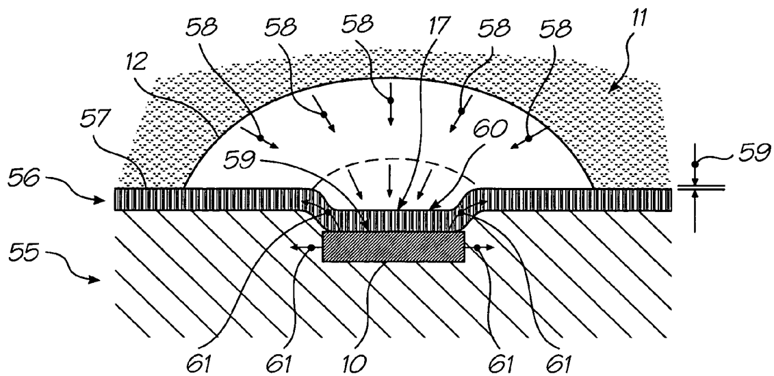
FIG. 47 (PRIOR ART)
