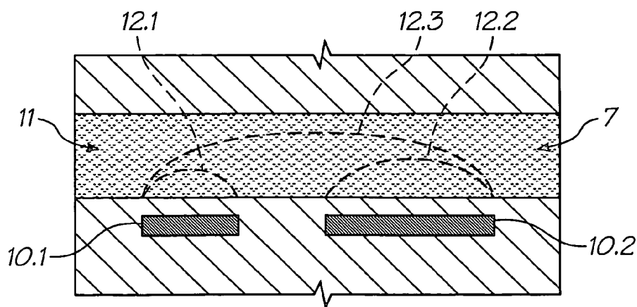
FIG. 52 (PRIOR ART)
