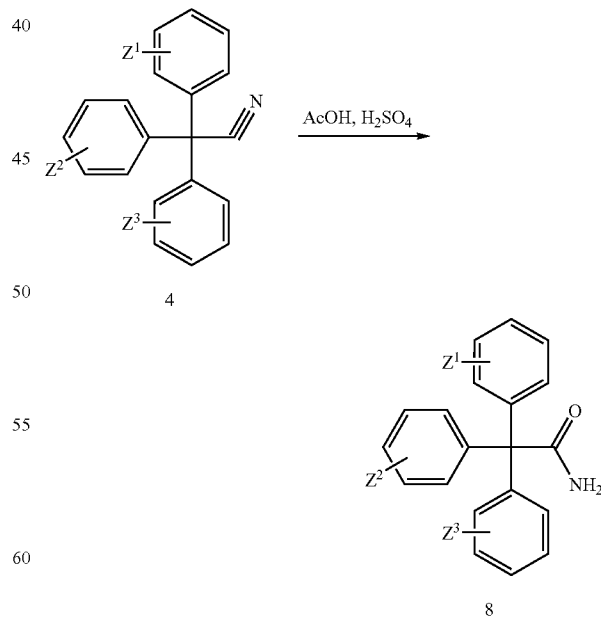
Scheme 6
