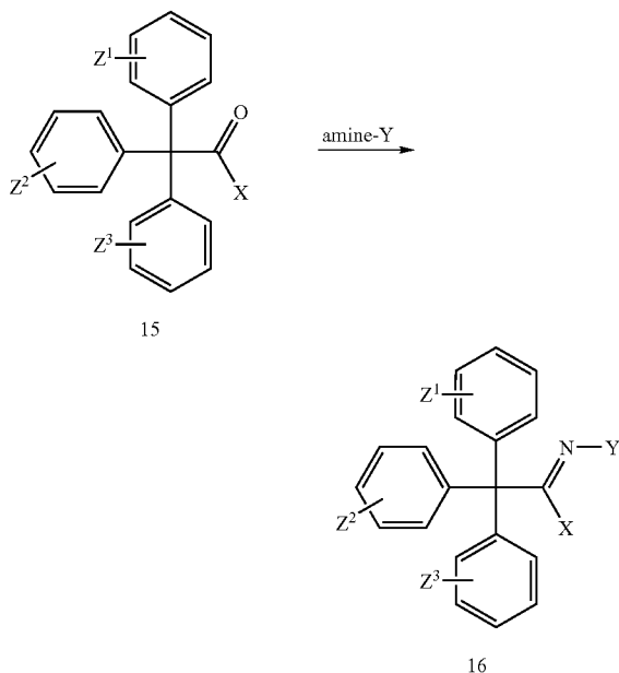
Scheme 11
