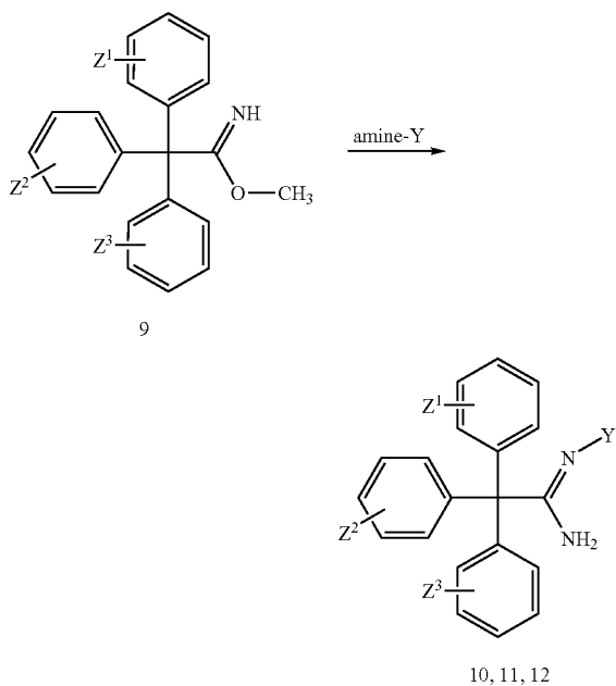
Scheme 8
