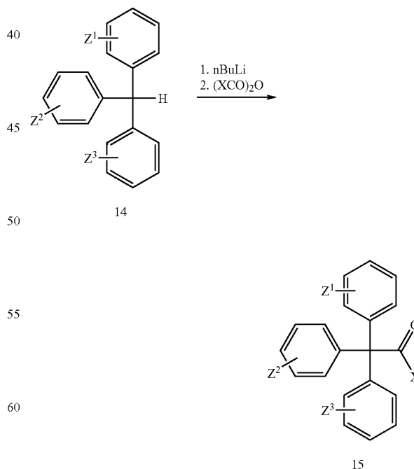
Scheme 10
