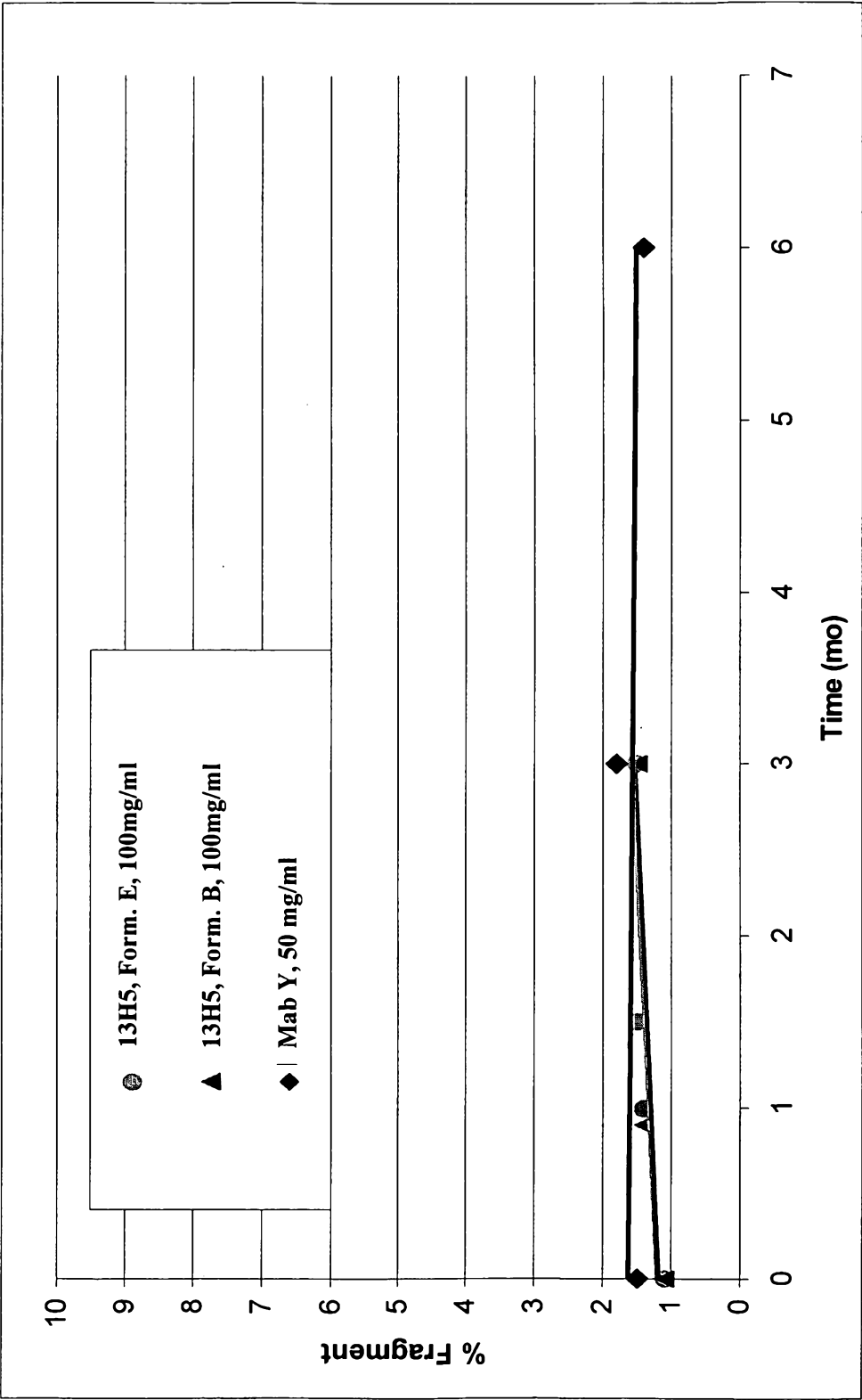
Stability of 13H5 formulation at 5°C
