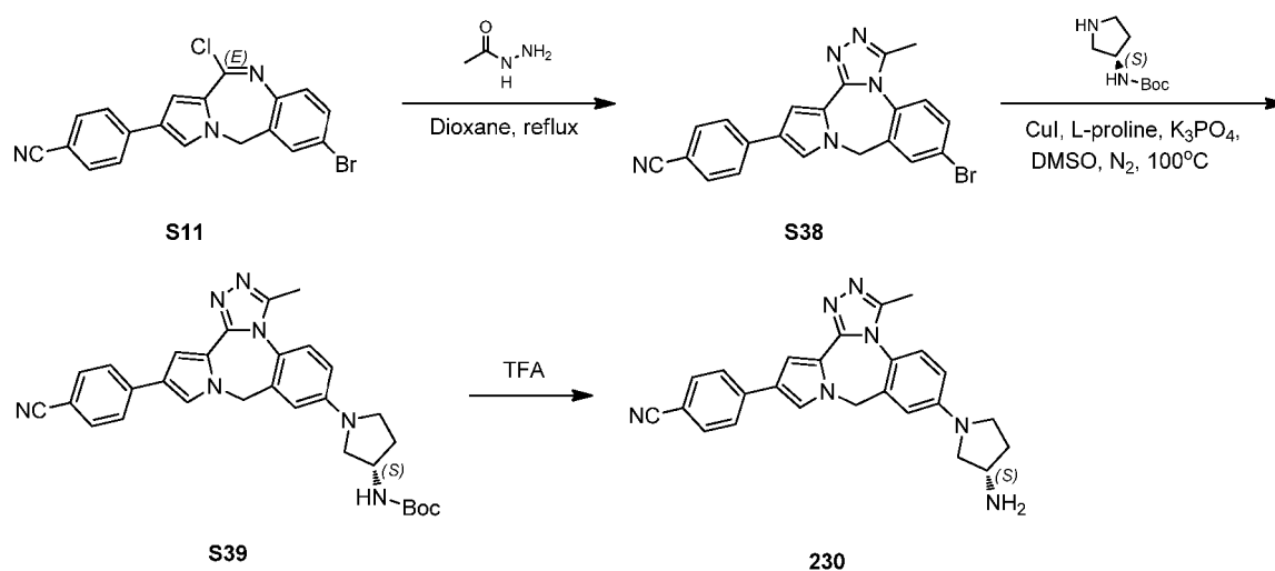
Scheme 14
