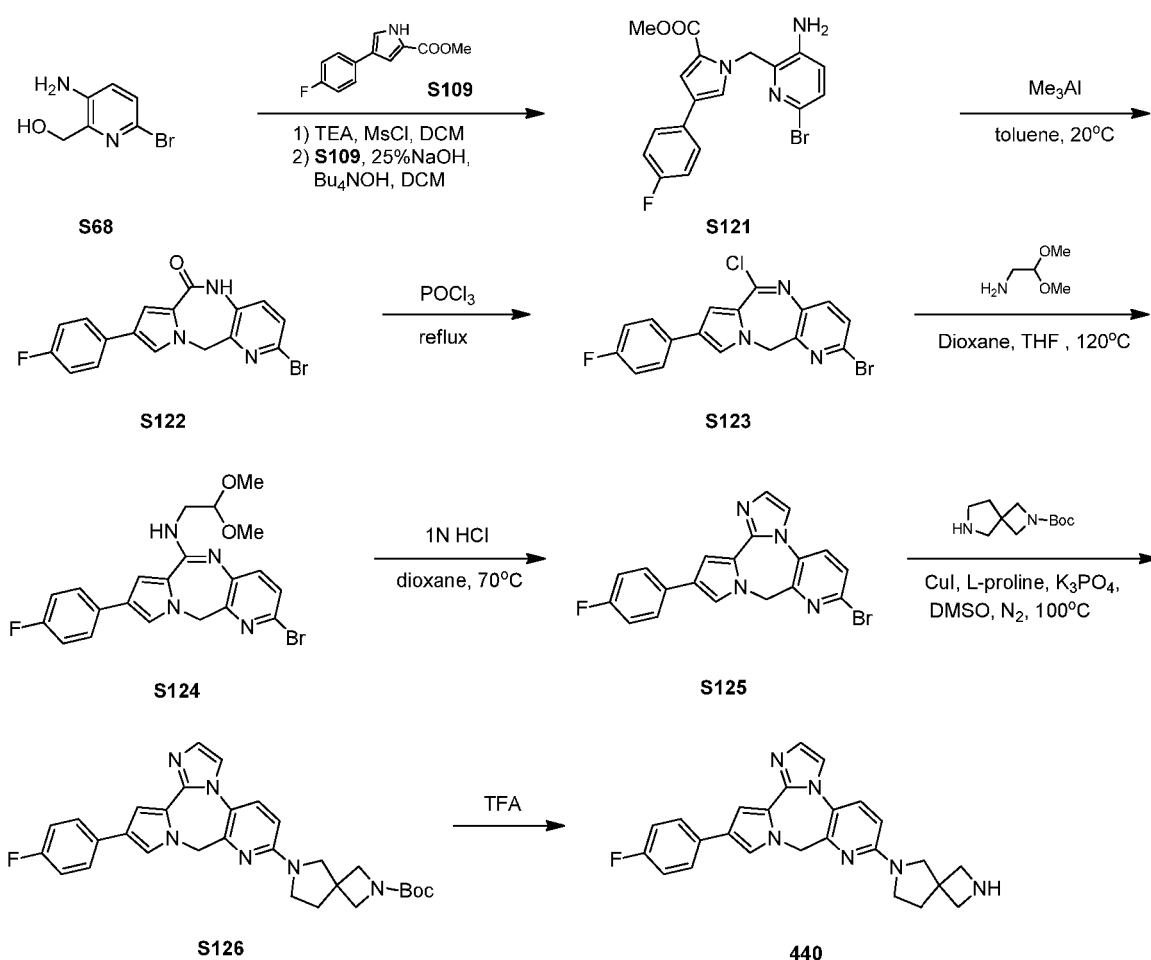
Scheme 35
