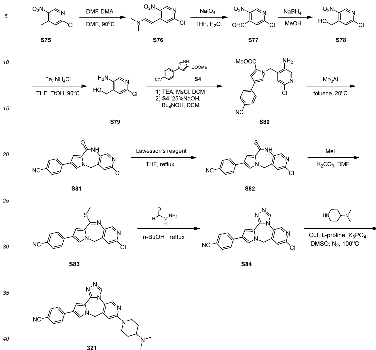
Scheme 27
