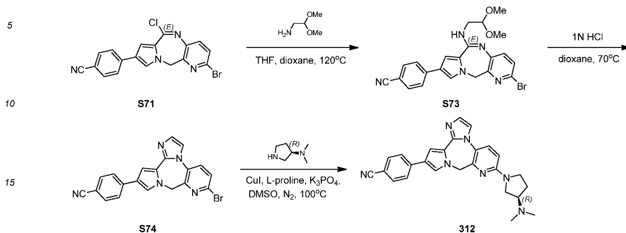
Scheme 26
