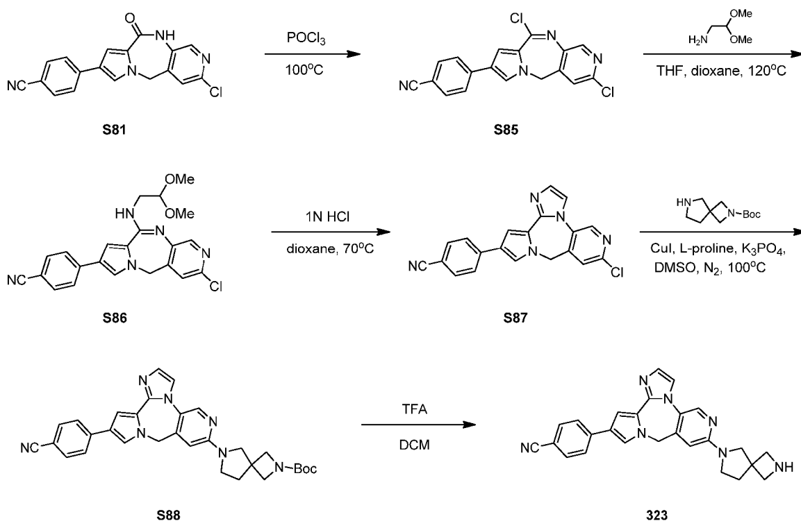
Scheme 28
