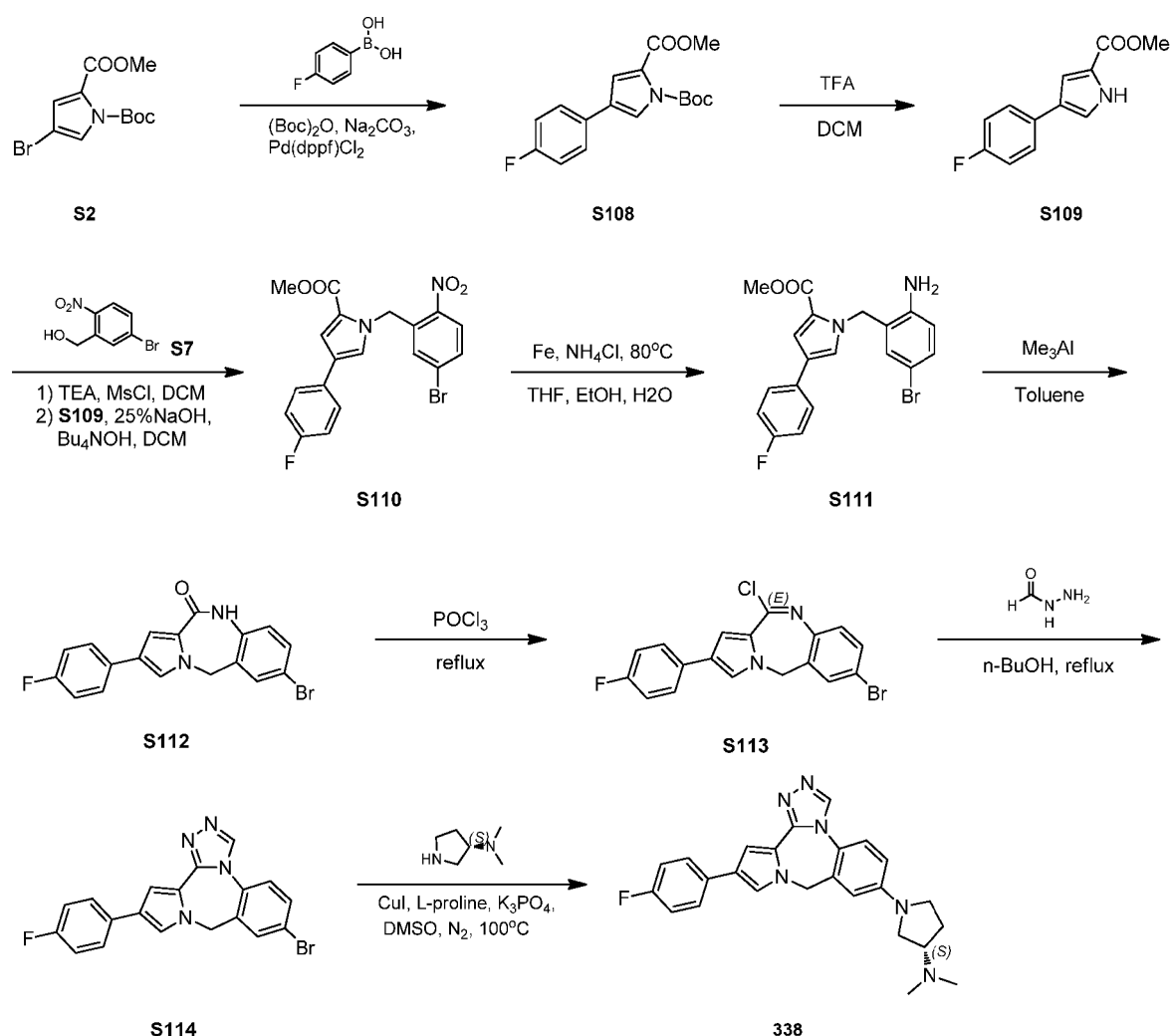
Scheme 31
