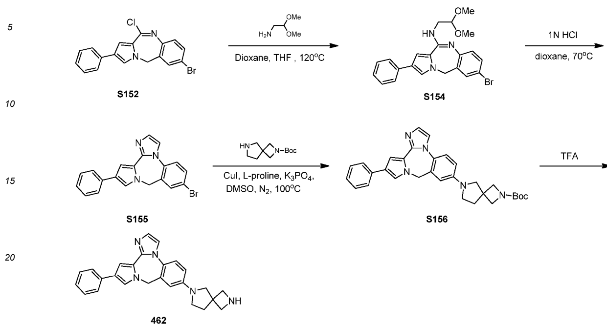
Scheme 41
