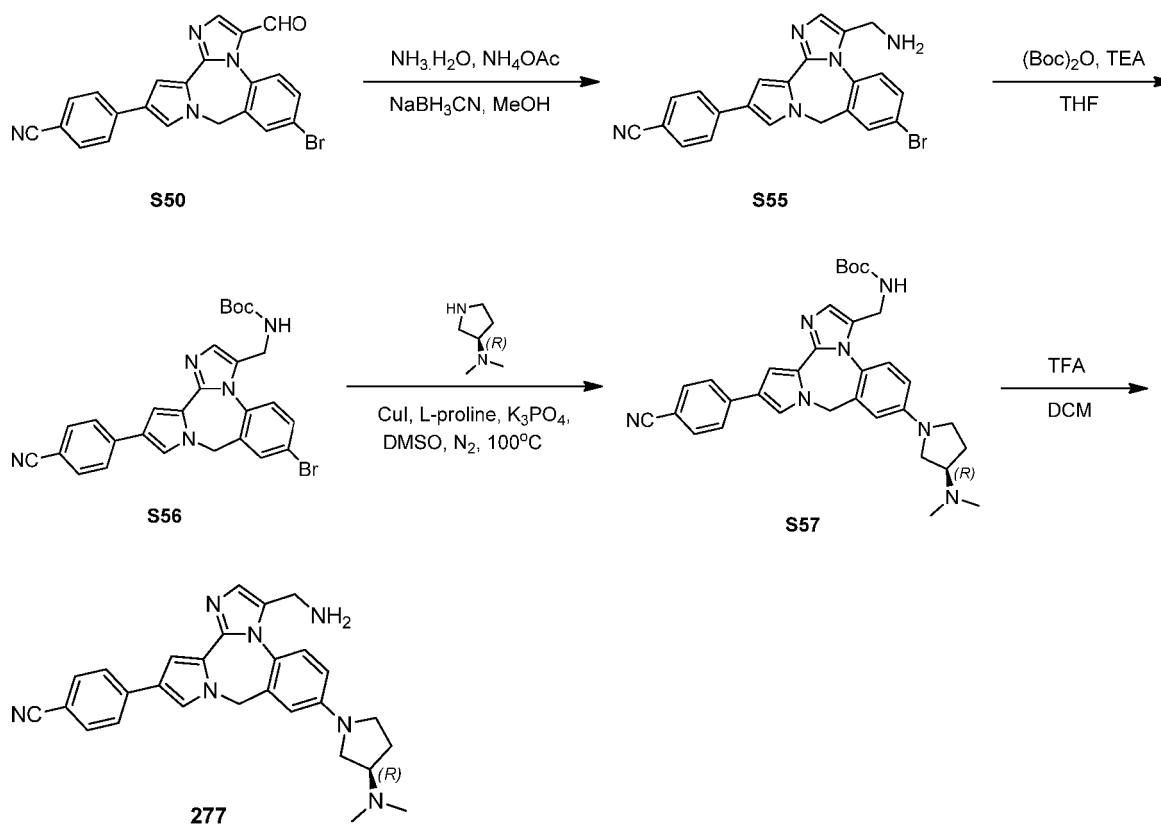
Scheme 21
