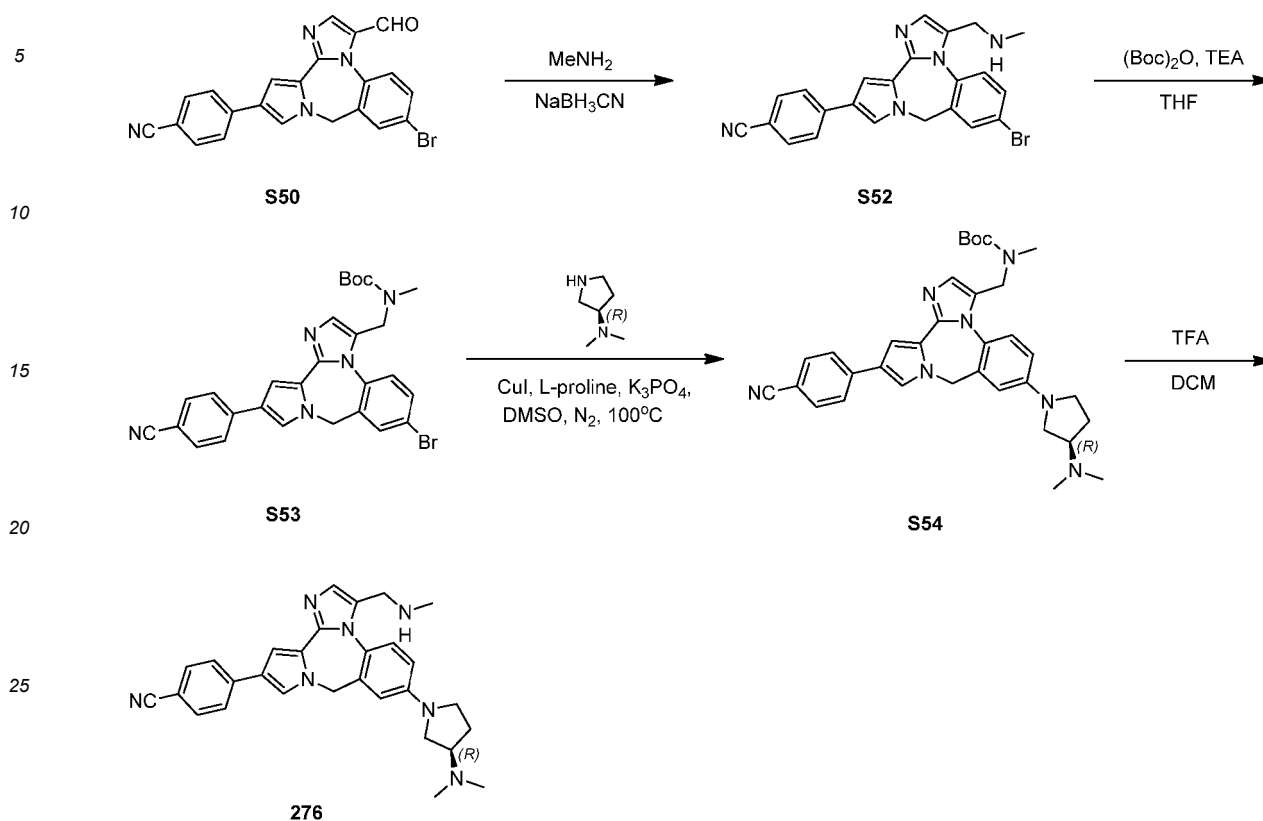
Scheme 20
