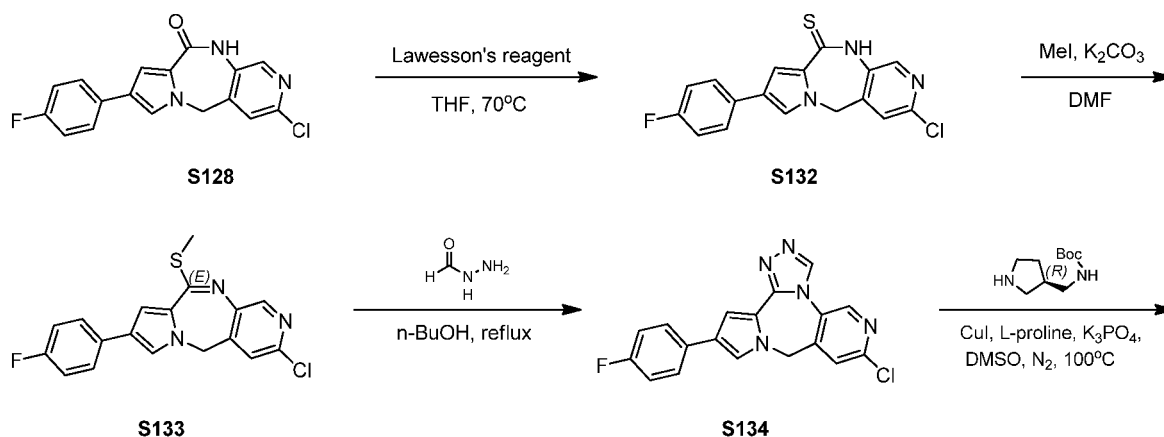
Scheme 37
