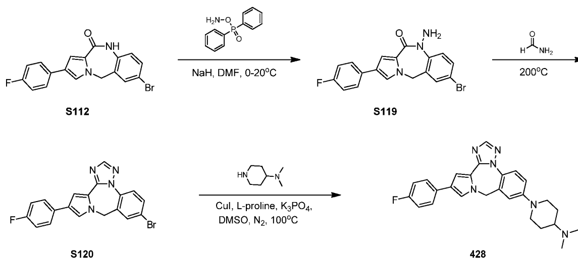
Scheme 34
