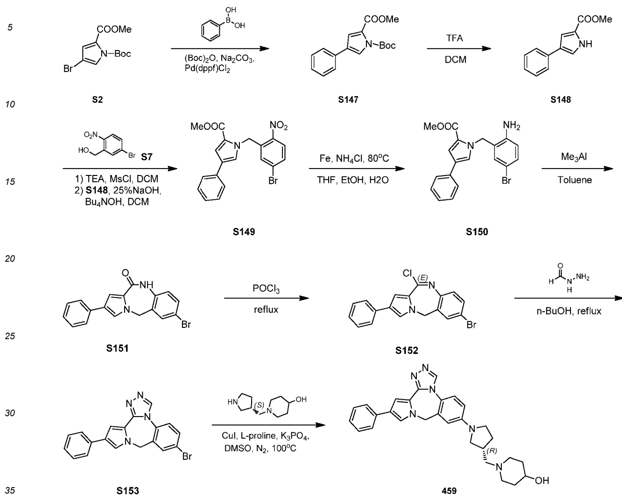
Scheme 40
