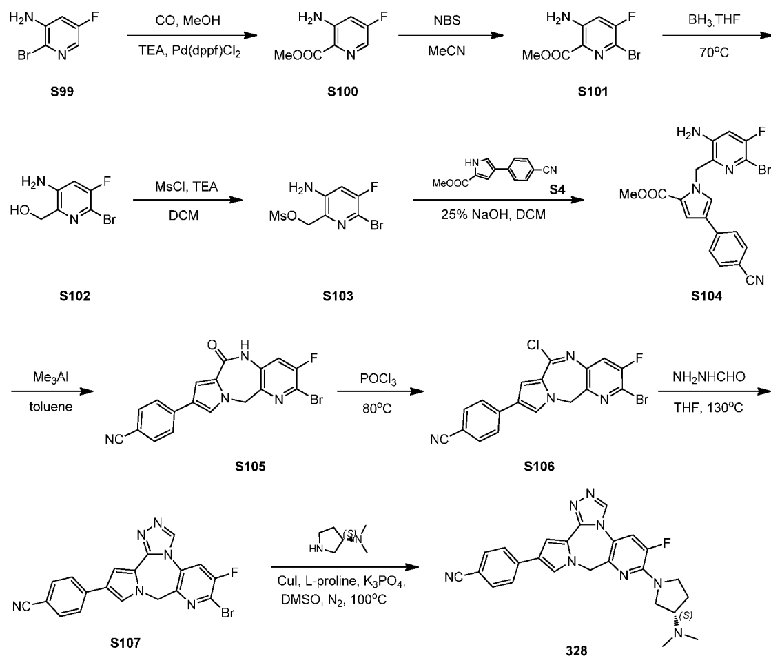
Scheme 30
