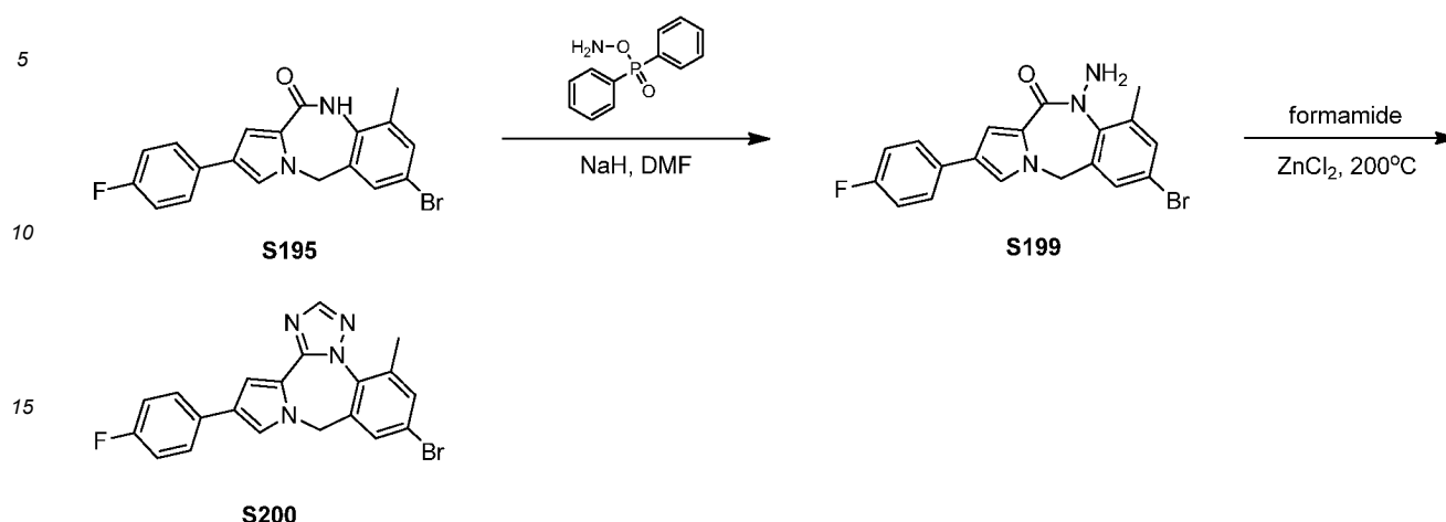
Scheme 52:
