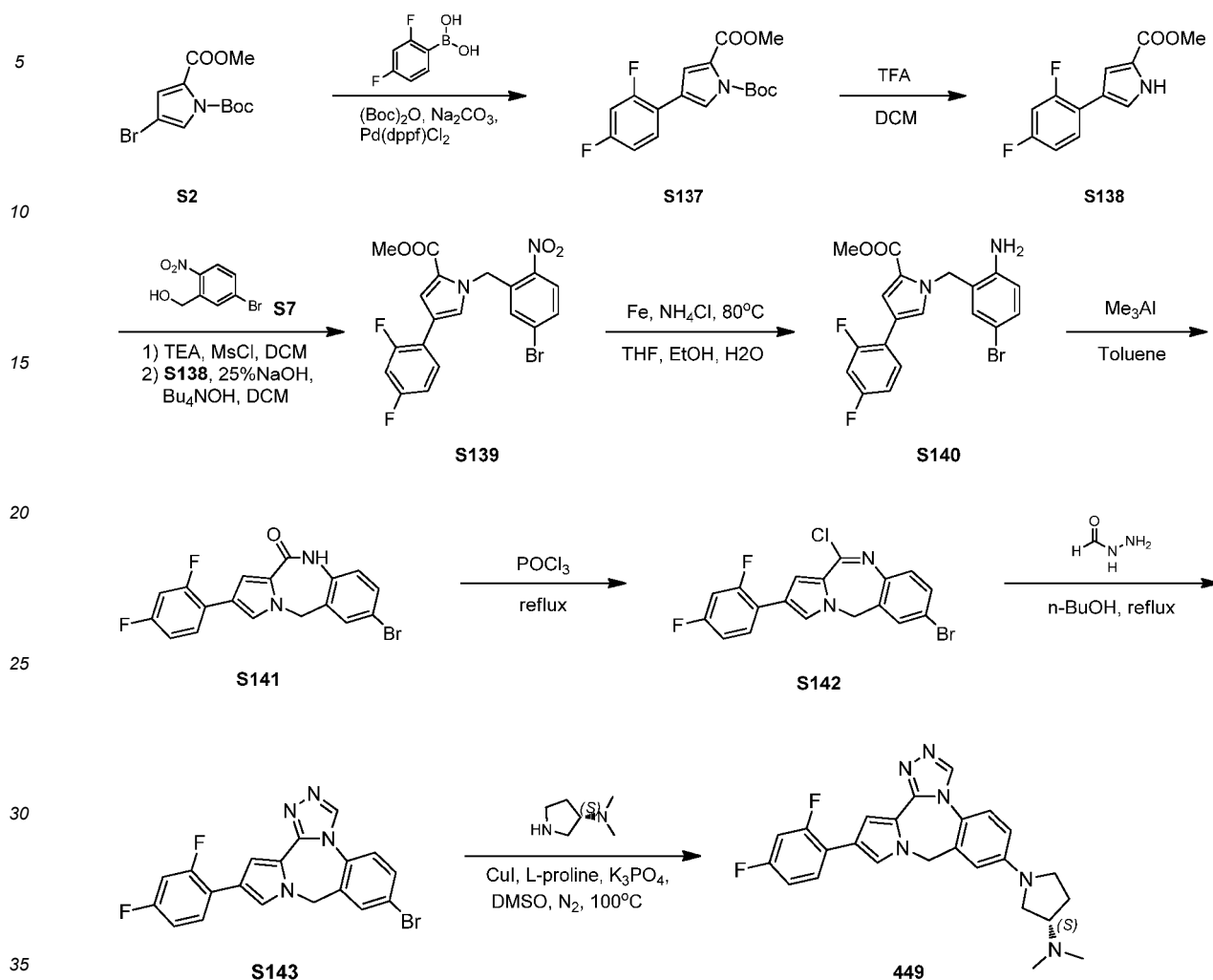
Scheme 38
