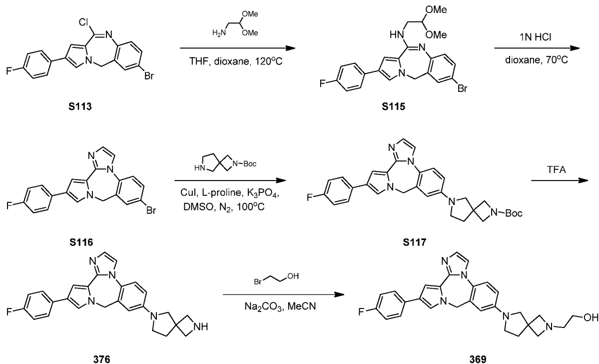
Scheme 32
