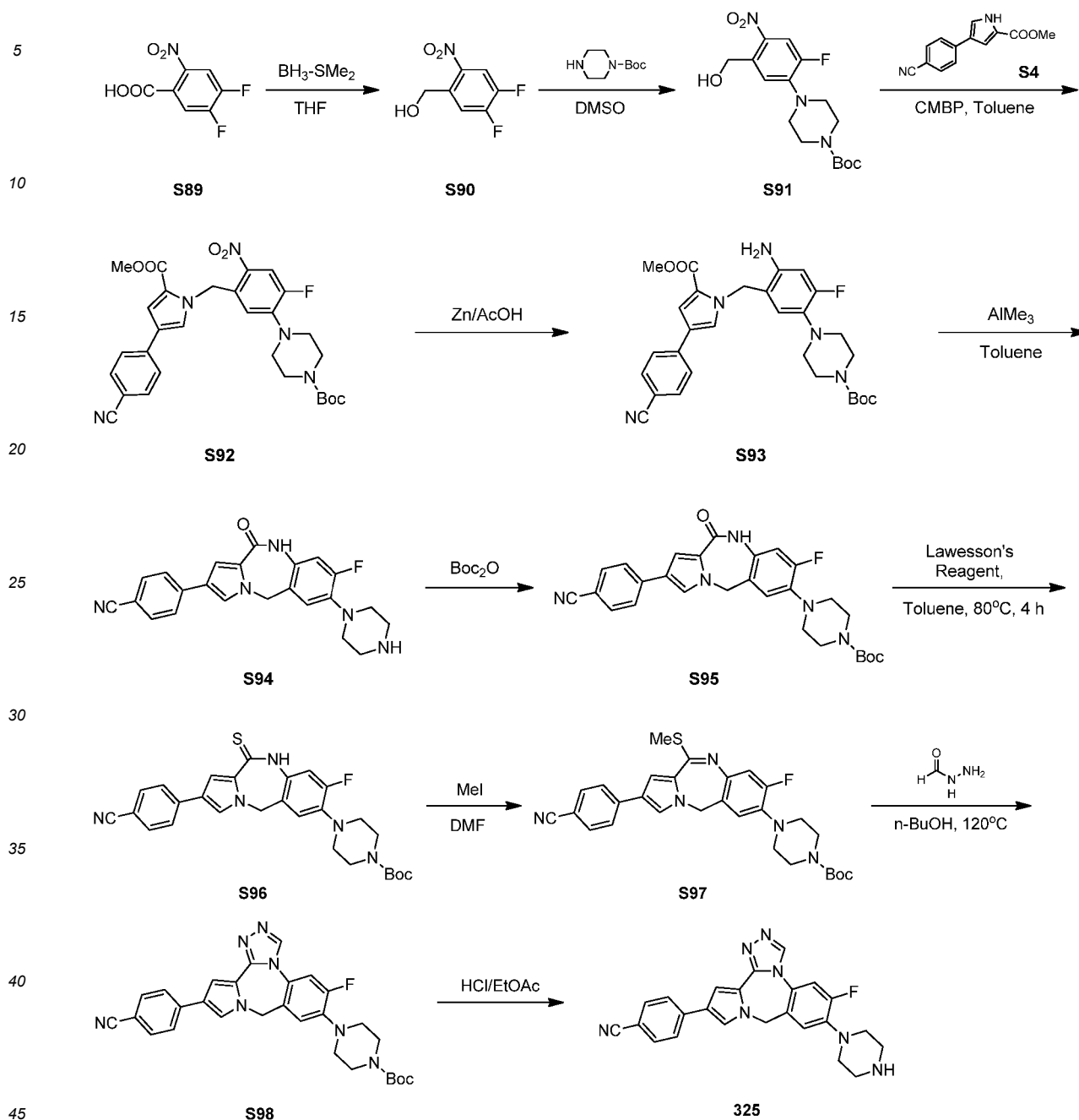
Scheme 29
