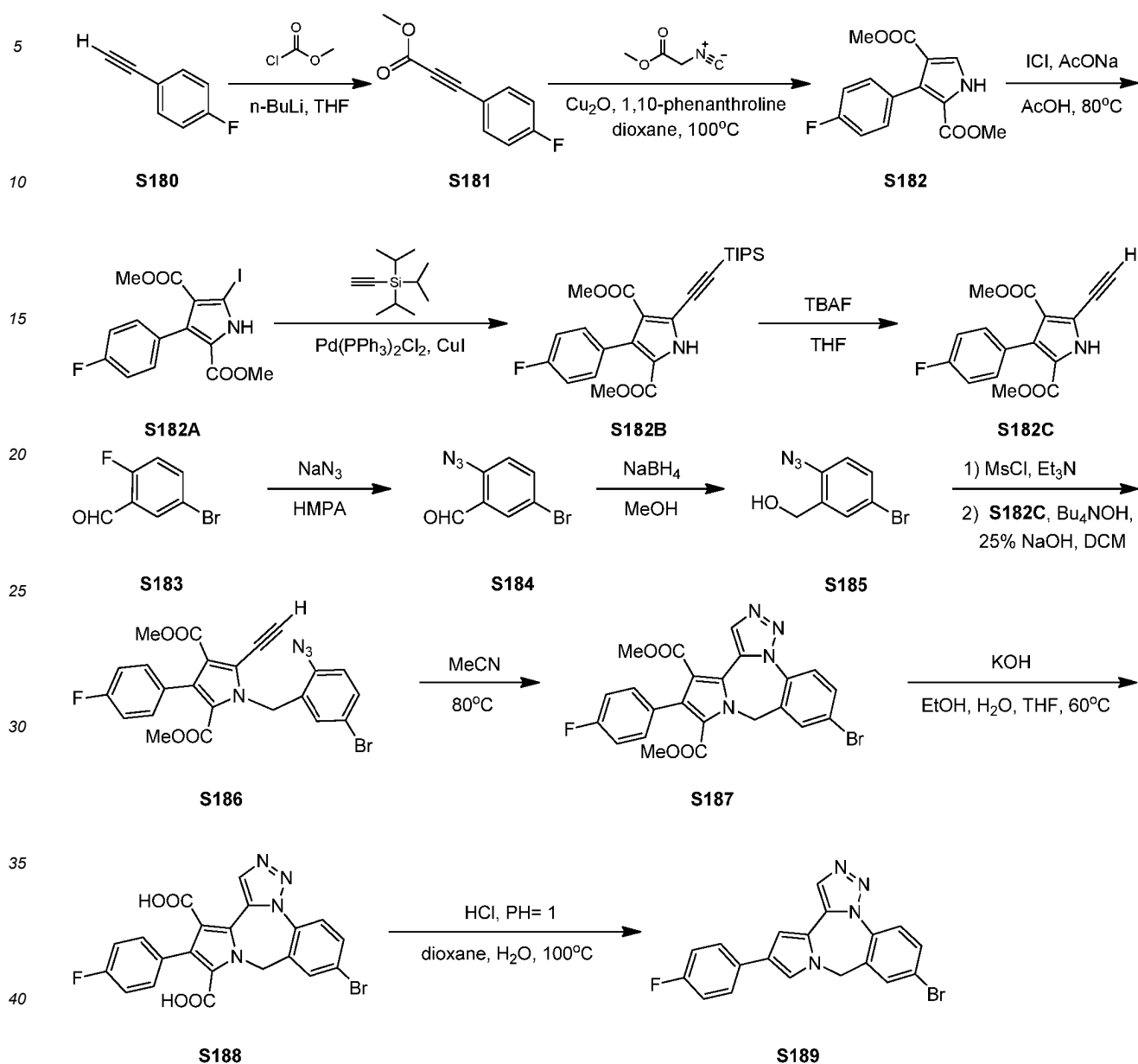
Scheme 50:
