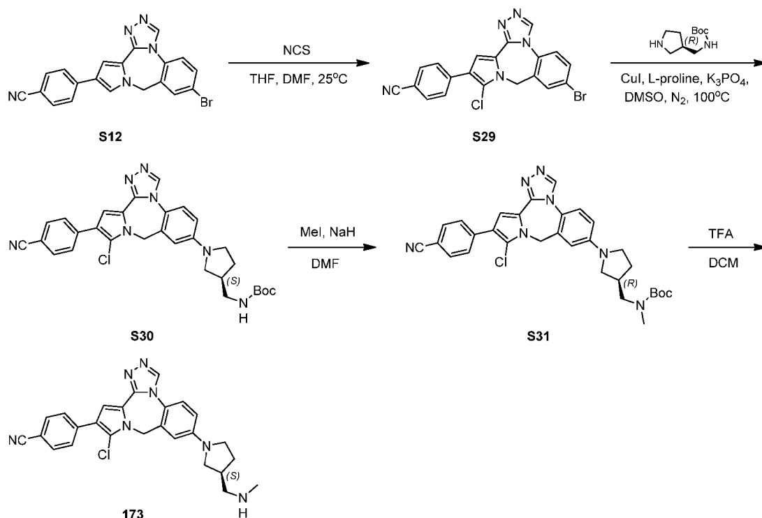
Scheme 10
