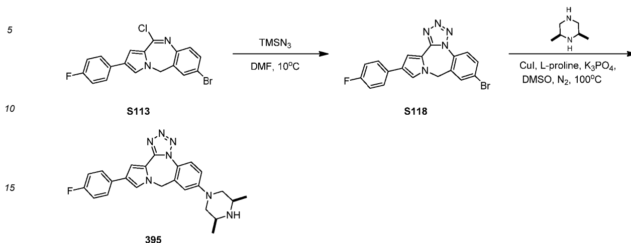
Scheme 33
