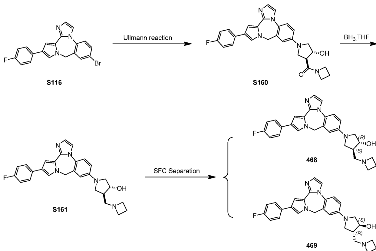
Scheme 46:
