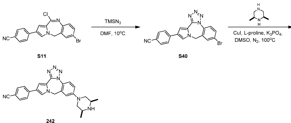
Scheme 15
