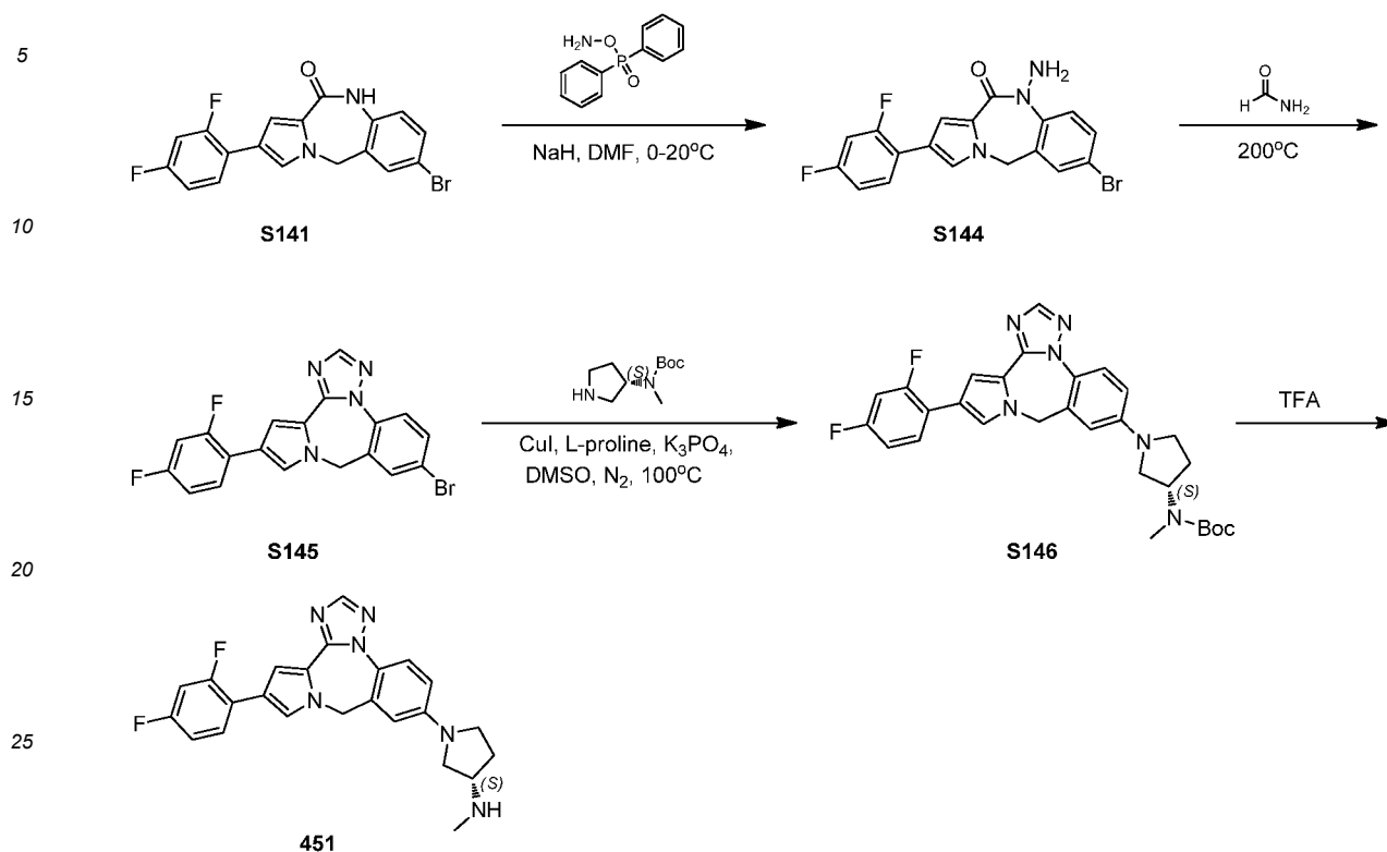
Scheme 39
