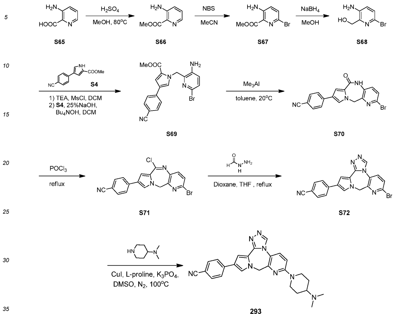
Scheme 25
