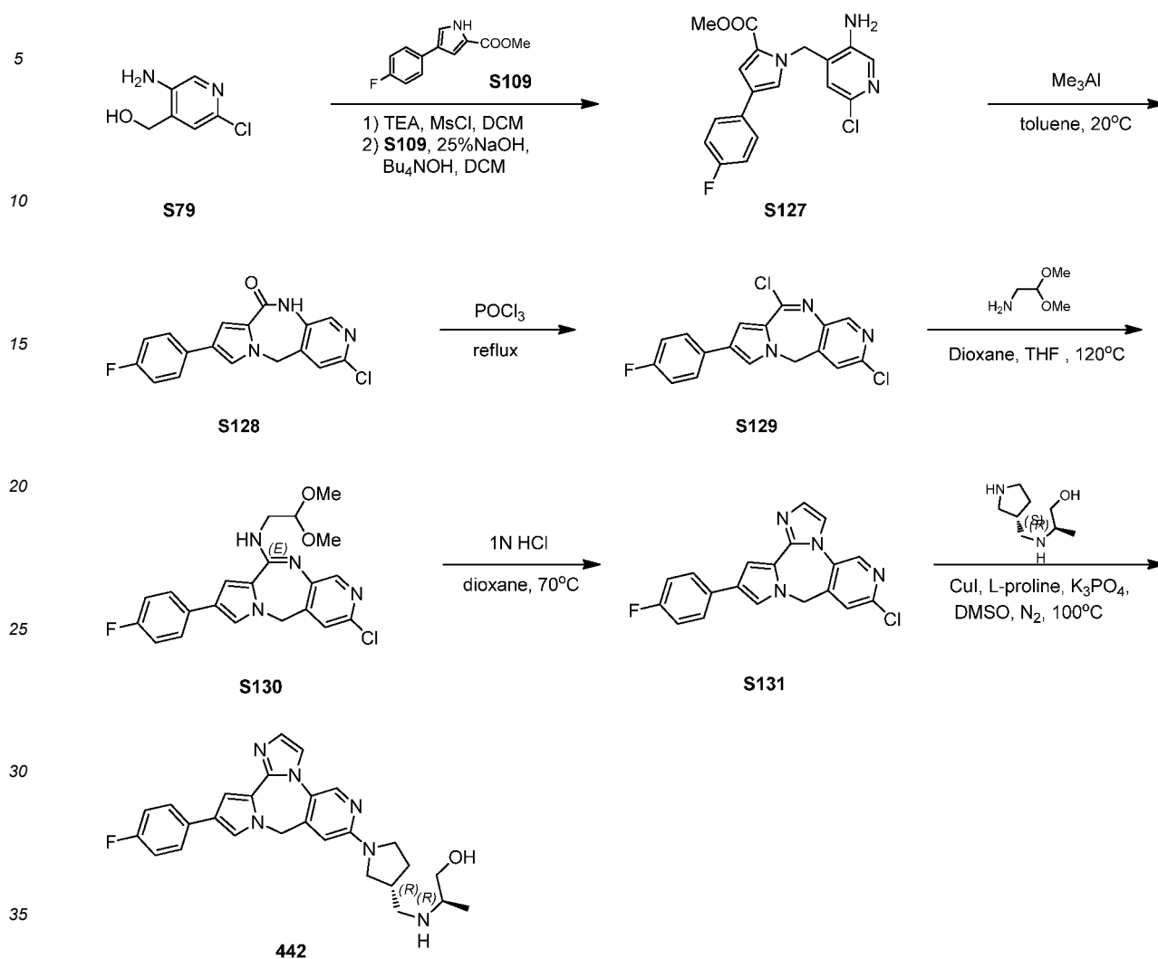
Scheme 36
