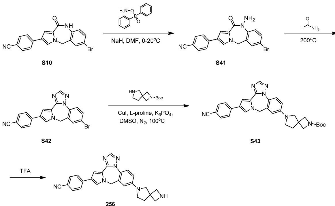
Scheme 16
