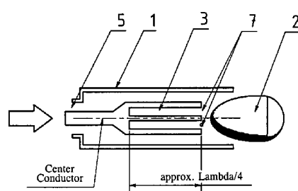
Resonant ignition structure in the inner conductor
