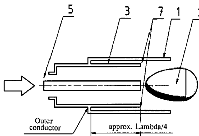
Resonant ignition structure in the outer conductor
