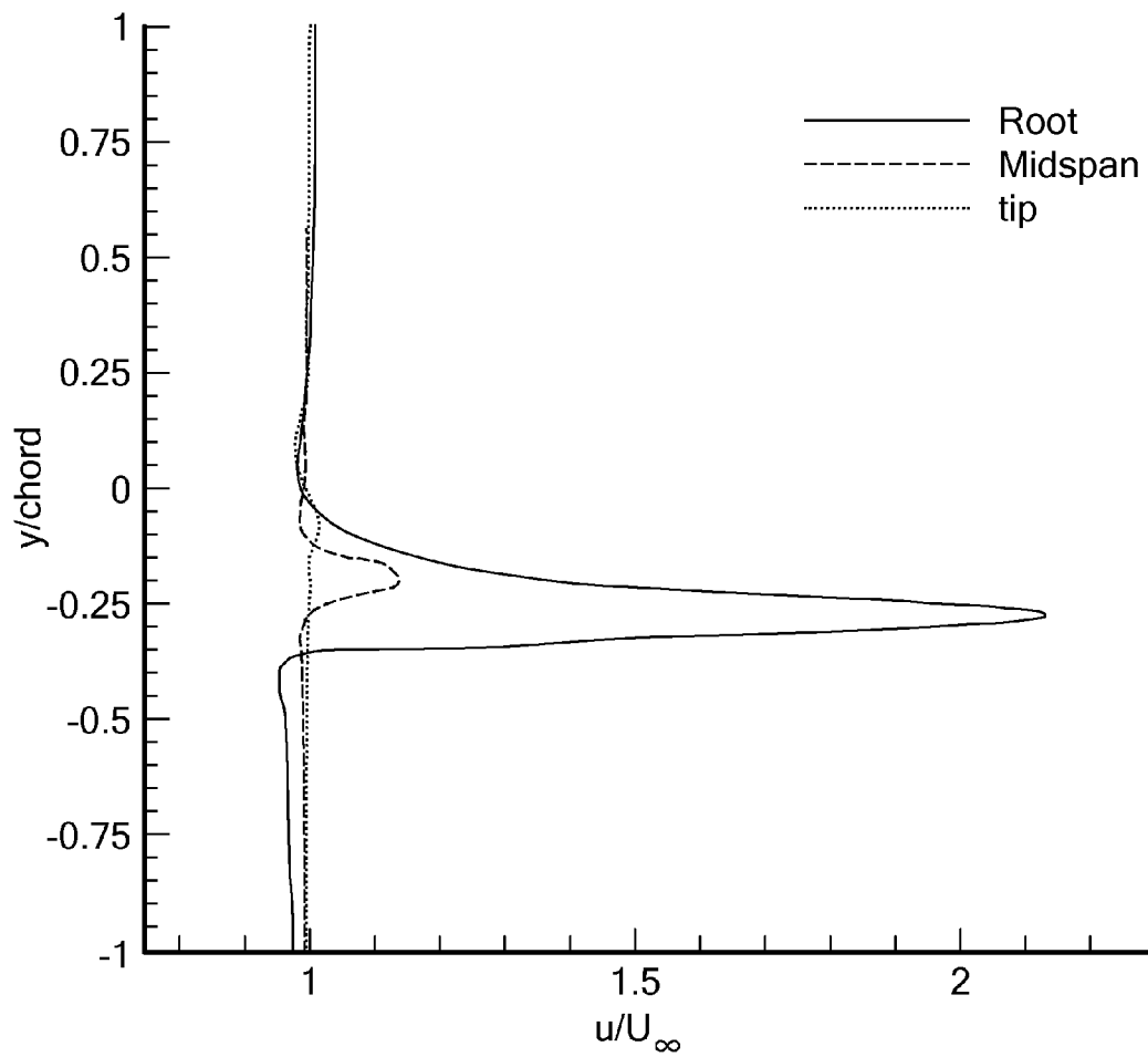
3-D Wake profile plot for A\alpha A = 0^\circ
