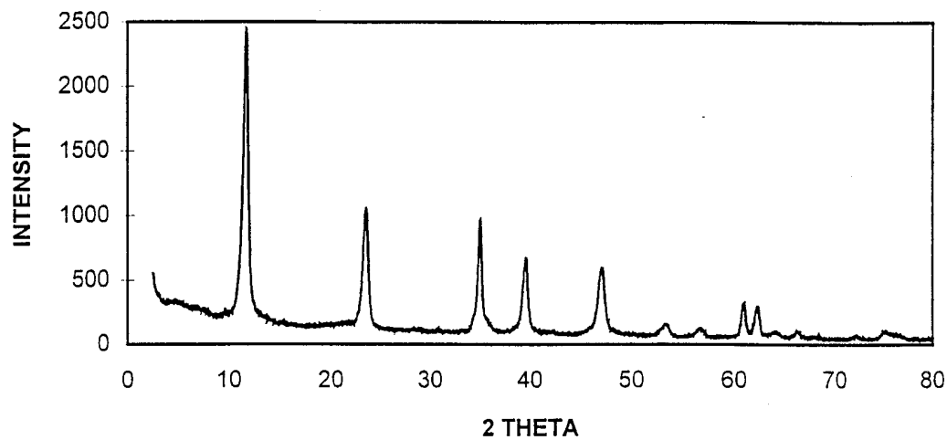
FIGURE 1: X-RAY DIFFRACTION PATTERN FOR COMMERCIAL ANIONIC CLAY
