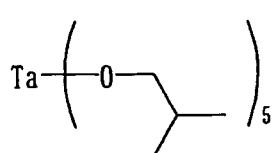
Compound No.58
