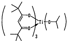
Compound No.19
