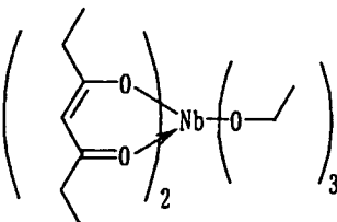
Compound No.67
