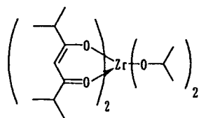
Compound No.28
