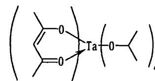
Compound No.72
