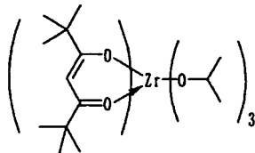
Compound No.24
