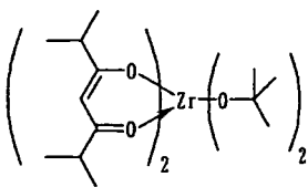
Compound No.29
