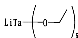
Compound No.97
