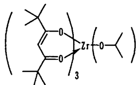
Compound No.22
