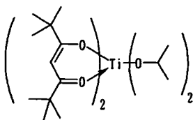
Compound No.17
