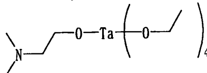
Compound No.62
