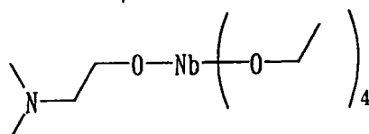
Compound No.61
