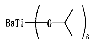
Compound No.101
