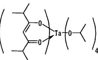
Compound No.73
