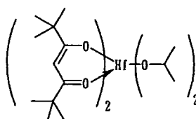
Compound No.32
