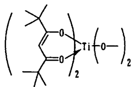
Compound No.16
