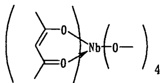
Compound No.66
