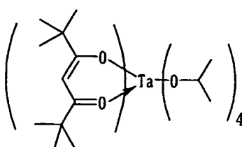
Compound No.70
