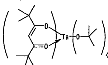
Compound No.71
