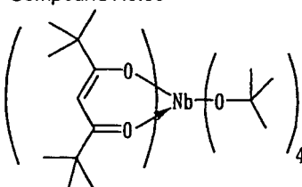
Compound No.65
