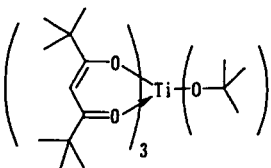
Compound No.20
