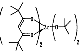
Compound No.26
