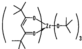
Compound No.27
