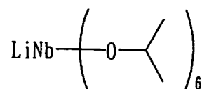
Compound No.95
