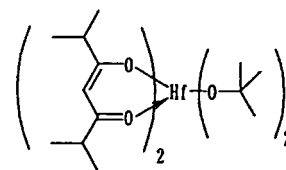
Compound No.33
