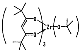
Compound No.25
