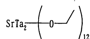
Compound No.108
