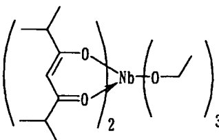
Compound No.68
