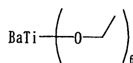
Compound No.100
