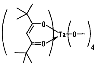
Compound No.69
