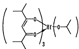
Compound No.31
