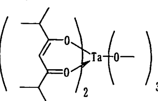
Compound No.74
