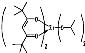
Compound No.23
