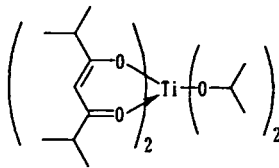
Compound No.21
