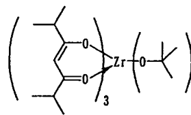
Compound No.30
