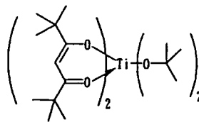
Compound No.18
