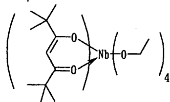
Compound No.63
