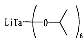
Compound No.98
