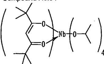
Compound No.64
