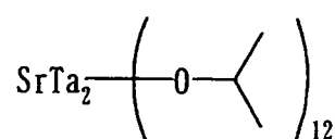
Compound No.109
