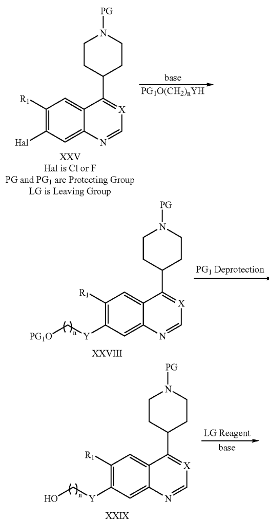
Scheme 10
