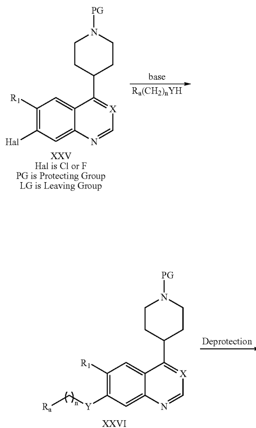
Scheme 9
