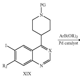
Scheme 7
