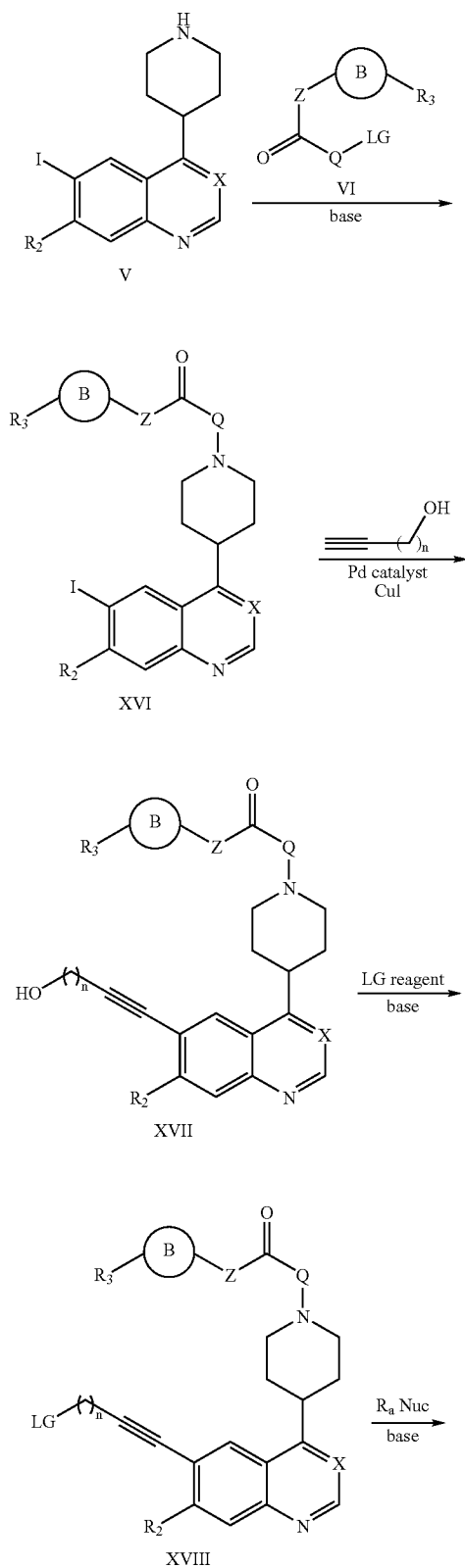
Scheme 6
