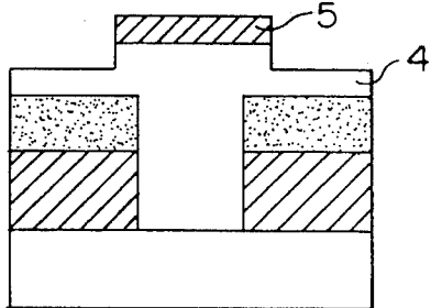
FIG. 1c PRIOR ART
