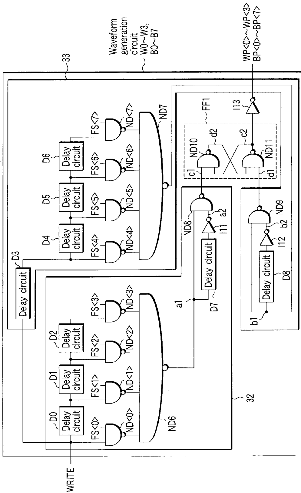
FIG. 54 • One of FS<0> to FS<3> changes to "H", and one of FS<4> to FS<7> changes to "H"
