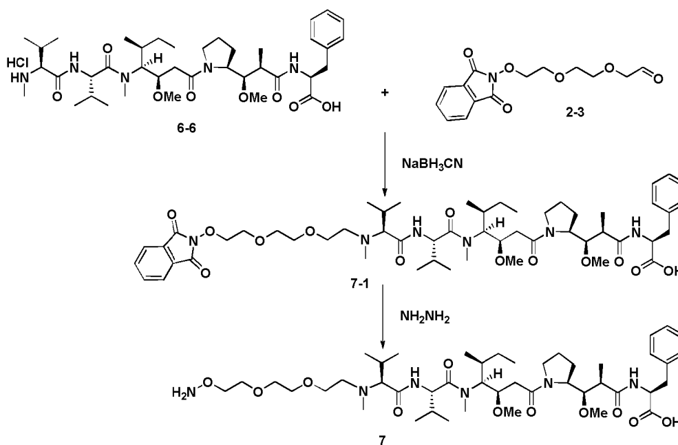
Scheme 7
