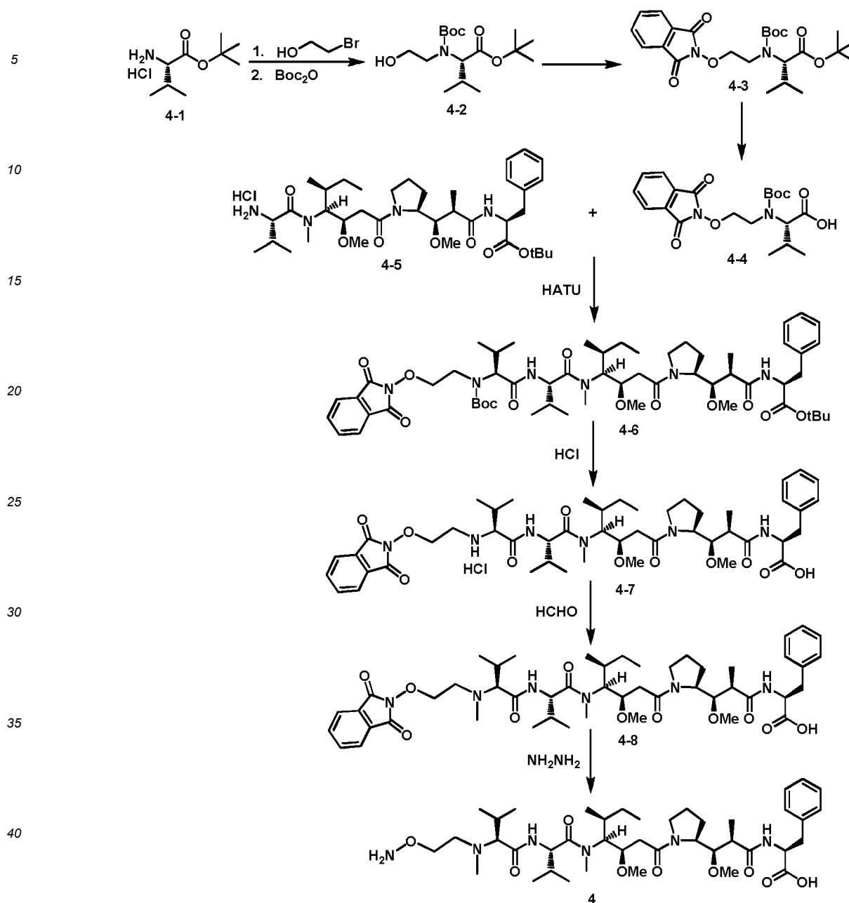
Scheme 4
