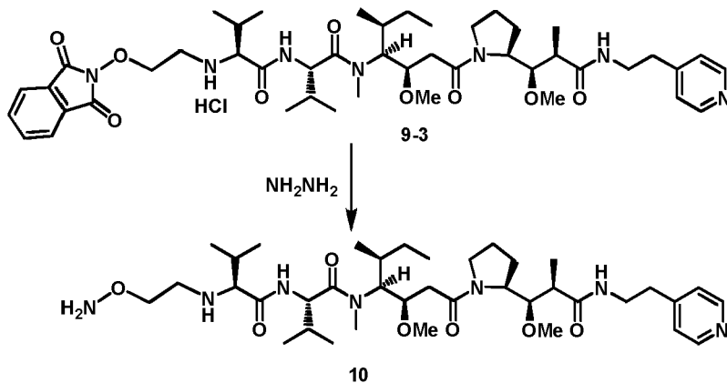
Scheme 10
