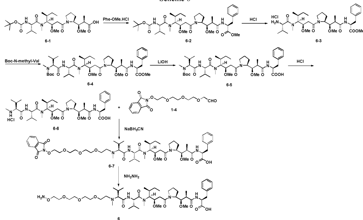
Scheme 6
