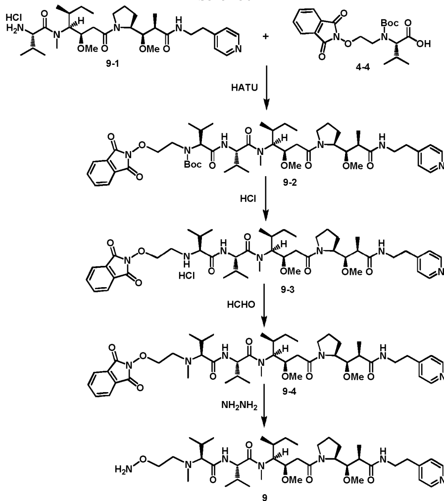
Scheme 9
