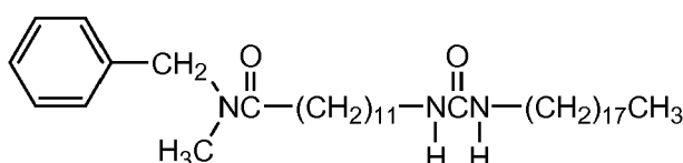
Structural Formula (2)
