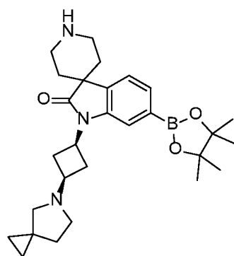
1-((1s,3s)-3-(5-azaspiro[2.4]heptan-5-yl)cyclobutyl)-6-(4,4,5,5-tetramethyl-1,3,2-dioxaborolan-2-yl)spiro[indoline-3,4'-piperidin]-2-one
