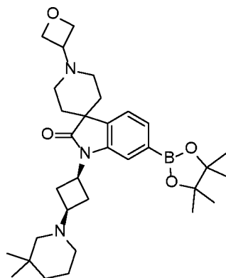
1-((1s,3s)-3-(3,3-dimethylpiperidin-1-yl)cyclobutyl)-1'-(oxetan-3-yl)-6-(4,4,5,5-tetramethyl-1,3,2-dioxaborolan-2-yl)spiro[indoline-3,4'-piperidin]-2-one
