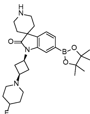
1-(((1s,3s)-3-(4-fluoropiperidin-1-yl)cyclobutyl)-6-(4,4,5,5-tetramethyl-1,3,2-dioxaborolan-2-yl)spiro[indoline-3,4'-piperidin]-2-one
