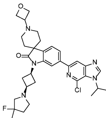
6-(4-chloro-3-isopropyl-3H-imidazo[4,5-c]pyridin-6-yl)-1-((1s,3s)-3-(3-fluoro-3-methylpyrrolidin-1-yl)cyclobutyl)-1'-(oxetan-3-yl)spiro[indoline-3,4'-piperidin]-2-one
