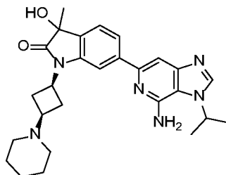
6-(4-amino-3-isopropyl-3H-imidazo[4,5-c]pyridin-6-yl)-3-hydroxy-3-methyl-1-((1s,3s)-3-(piperidin-1-yl)cyclobutyl)indolin-2-one
