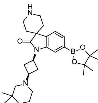
1-((1s,3s)-3-(3,3-dimethylpiperidin-1-yl)cyclobutyl)-6-(4,4,5,5-tetramethyl-1,3,2-dioxaborolan-2-yl)spiro[indoline-3,4'-piperidin]-2-one
