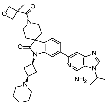
6-(4-amino-3-isopropyl-3H-imidazo[4,5-c]pyridin-6-yl)-1'-((3-methyloxetane-3-carbonyl)-1-((1s,3s)-3-(piperidin-1-yl)cyclobutyl)spiro[indoline-3,4'-piperidin]-2-one
