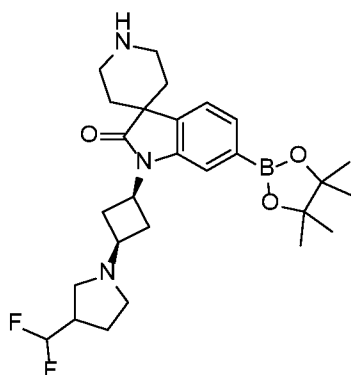
1-((1s,3s)-3-(3-(difluoromethyl)pyrrolidin-1-yl)cyclobutyl)-6-(4,4,5,5-tetramethyl-1,3,2-dioxaborolan-2-yl)spiro[indoline-3,4'-piperidin]-2-one
