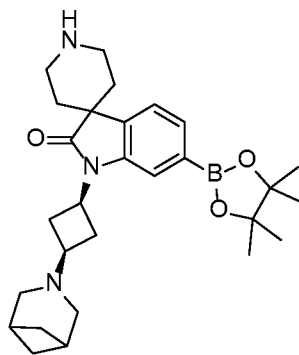
1-((1s,3s)-3-(3-azabicyclo[3.1.1]heptan-3-yl)cyclobutyl)-6-(4,4,5,5-tetramethyl-1,3,2-dioxaborolan-2-yl)spiro[indoline-3,4'-piperidin]-2-one
