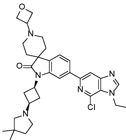
6-(4-chloro-3-ethyl-3H-imidazo[4,5-c]pyridin-6-yl)-1'-((1s,3s)-3-(3,3-dimethylpyrrolidin-1-yl)cyclobutyl)-1'-(oxetan-3-yl)spiro[indoline-3,4'-piperidin]-2-one
