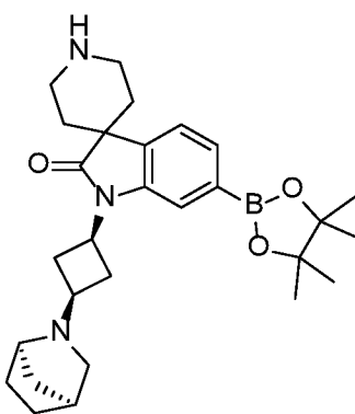
1-((1S,3s)-3-((1R,4S)-2-azabicyclo[2.2.1]heptan-2-yl)cyclobutyl)-6-(4,4,5,5-tetramethyl-1,3,2-dioxaborolan-2-yl)spiro[indoline-3,4'-piperidin]-2-one
