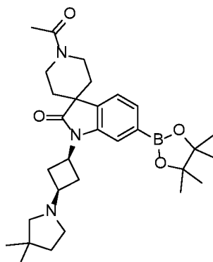
1'-Acetyl-1-((1s,3s)-3-(3,3-dimethylpyrrolidin-1-yl)cyclobutyl)-6-(4,4,5,5-tetramethyl-1,3,2-dioxaborolan-2-yl)spiro[indoline-3,4'-piperidin]-2-one
