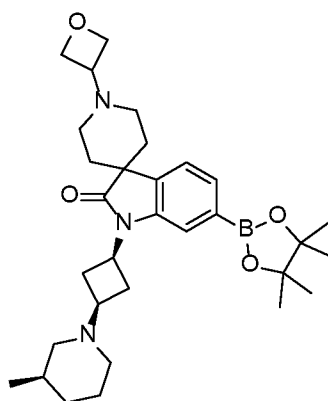
1-((1S,3s)-3-((R)-3-methylpiperidin-1-yl)cyclobutyl)-1'-(oxetan-3-yl)-6-(4,4,5,5-tetramethyl-1,3,2-dioxaborolan-2-yl)spiro[indoline-3,4'-piperidin]-2-one
