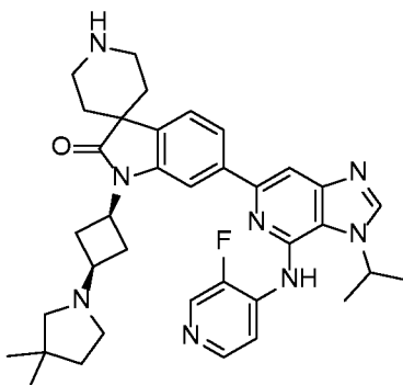
1-((1s,3s)-3-(3,3-dimethylpyrrolidin-1-yl)cyclobutyl)-6-(4-((3-fluoropyridin-4-yl)amino)-3-isopropyl-3H-imidazo[4,5-c]pyridin-6-yl)spiro[indoline-3,4'-piperidin]-2-one
