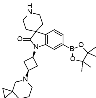
1-((1s,3s)-3-(5-azaspiro[2.5]octan-5-yl)cyclobutyl)-6-(4,4,5,5-tetramethyl-1,3,2-dioxaborolan-2-yl)spiro[indoline-3,4'-piperidin]-2-one
