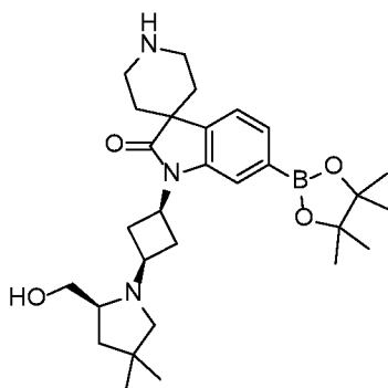
1-((1S,3r)-3-((S)-2-(hydroxymethyl)-4,4-dimethylpyrrolidin-1-yl)cyclobutyl)-6-(4,4,5,5-tetramethyl-1,3,2-dioxaborolan-2-yl)spiro[indoline-3,4'-piperidin]-2-one
