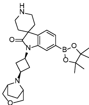
1-((1s,3s)-3-(3-oxa-8-azabicyclo[3.2.1]octan-8-yl)cyclobutyl)-6-(4,4,5,5-tetramethyl-1,3,2-dioxaborolan-2-yl)spiro[indoline-3,4'-piperidin]-2-one
