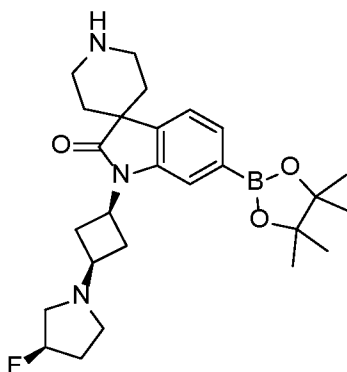
1-((1S,3s)-3-((R)-3-fluoropyrrolidin-1-yl)cyclobutyl)-6-(4,4,5,5-tetramethyl-1,3,2-dioxaborolan-2-yl)spiro[indoline-3,4'-piperidin]-2-one
