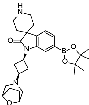
1-((1s,3s)-3-(8-oxa-3-azabicyclo[3.2.1]octan-3-yl)cyclobutyl)-6-(4,4,5,5-tetramethyl-1,3,2-dioxaborolan-2-yl)spiro[indoline-3,4'-piperidin]-2-one
