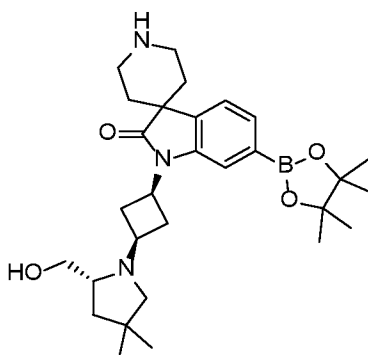
1-((1S,3s)-3-((R)-2-(hydroxymethyl)-4,4-dimethylpyrrolidin-1-yl)cyclobutyl)-6-(4,4,5,5-tetramethyl-1,3,2-dioxaborolan-2-yl)spiro[indoline-3,4'-piperidin]-2-one
