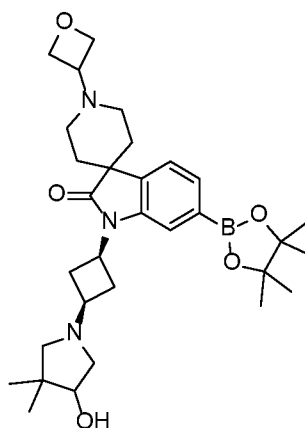
1-((1s,3s)-3-(4-hydroxy-3,3-dimethylpyrrolidin-1-yl)cyclobutyl)-1'-(oxetan-3-yl)-6-(4,4,5,5-tetramethyl-1,3,2-dioxaborolan-2-yl)spiro[indoline-3,4'-piperidin]-2-one
