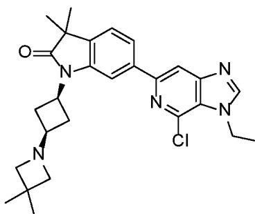
6-(4-chloro-3-ethyl-3H-imidazo[4,5-c]pyridin-6-yl)-1-((1s,3s)-3-(3,3-dimethylazetidin-1-yl)cyclobutyl)-3,3-dimethylindolin-2-one
