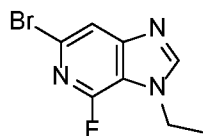
6-bromo-3-ethyl-4-fluoro-3H-imidazo[4,5-c]pyridine
