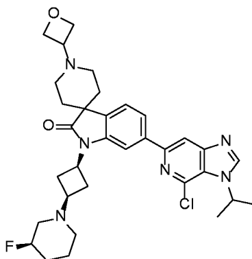
6-(4-chloro-3-isopropyl-3H-imidazo[4,5-c]pyridin-6-yl)-1-((1S,3s)-3-((R)-3-fluoropiperidin-1-yl)cyclobutyl)-1'-(oxetan-3-yl)spiro[indoline-3,4'-piperidin]-2-one
