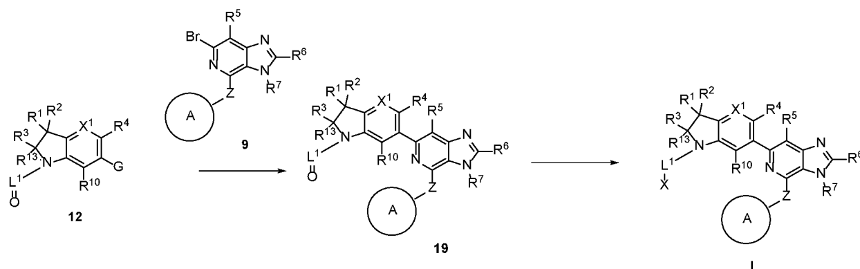
Reaction Scheme V
