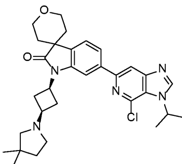
6-(4-chloro-3-isopropyl-3H-imidazo[4,5-c]pyridin-6-yl)-1-((1s,3s)-3-(3,3-dimethylpyrrolidin-1-yl)cyclobutyl)-2',3',5',6'-tetrahydrospiro[indoline-3,4'-pyran]-2-one
