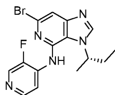
(S)-6-bromo-3-(sec-butyl)-N-(3-fluoropyridin-4-yl)-3H-imidazo[4,5-c]pyridin-4-amine
