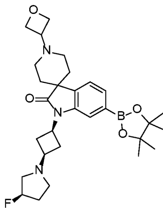
1-((1S,3s)-3-((R)-3-fluoropyrrolidin-1-yl)cyclobutyl)-1'-(oxetan-3-yl)-6-(4,4,5,5-tetramethyl-1,3,2-dioxaborolan-2-yl)spiro[indoline-3,4'-piperidin]-2-one
