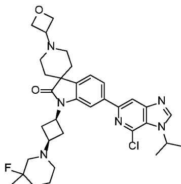
6-(4-chloro-3-isopropyl-3H-imidazo[4,5-c]pyridin-6-yl)-1-((1s,3s)-3-(3-fluoro-3-methylpiperidin-1-yl)cyclobutyl)-1'-(oxetan-3-yl)spiro[indoline-3,4'-piperidin]-2-one
