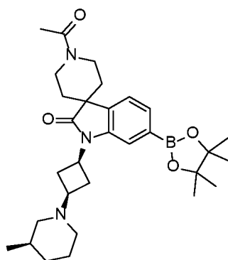
1'-Acetyl-1-((1S,3s)-3-((R)-3-methylpiperidin-1-yl)cyclobutyl)-6-(4,4,5,5-tetramethyl-1,3,2-dioxaborolan-2-yl)spiro[indoline-3,4'-piperidin]-2-one
