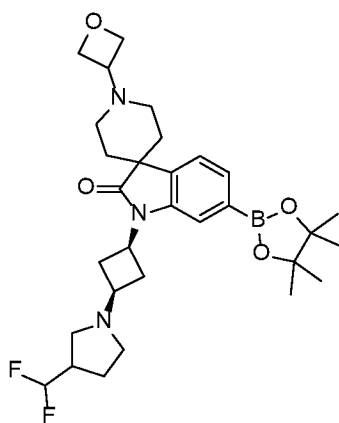
1-((1s,3s)-3-(3-(difluoromethyl)pyrrolidin-1-yl)cyclobutyl)-1'-(oxetan-3-yl)-6-(4,4,5,5-tetramethyl-1,3,2-dioxaborolan-2-yl)spiro[indoline-3,4'-piperidin]-2-one
