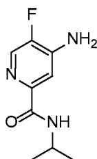
4-amino-5-fluoro-N-isopropylpicolinamide
