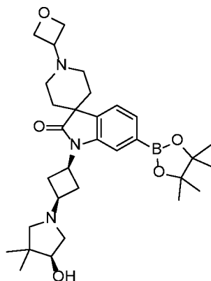
1-((1R,3s)-3-((S)-4-hydroxy-3,3-dimethylpyrrolidin-1-yl)cyclobutyl)-1'-(oxetan-3-yl)-6-(4,4,5,5-tetramethyl-1,3,2-dioxaborolan-2-yl)spiro[indoline-3,4'-piperidin]-2-one
