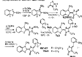
(C) Synthesis of YM-08
