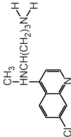
Bisdesehyl-chloroquine
