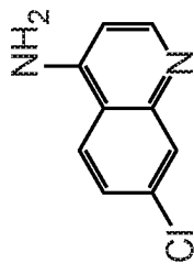
7-Chloro-4-aminoquinoline
