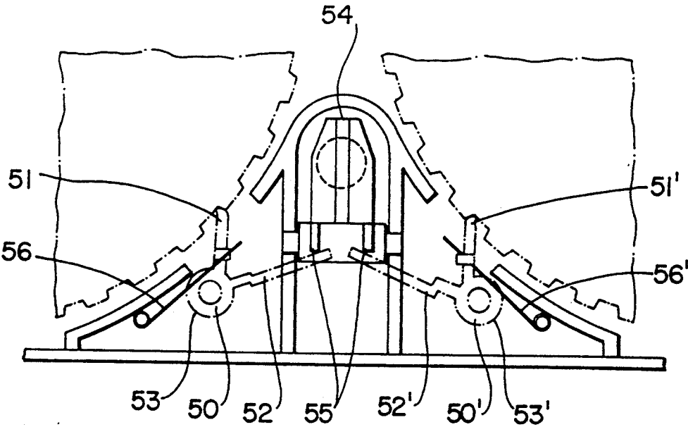
FIG. 5 PRIOR ART
