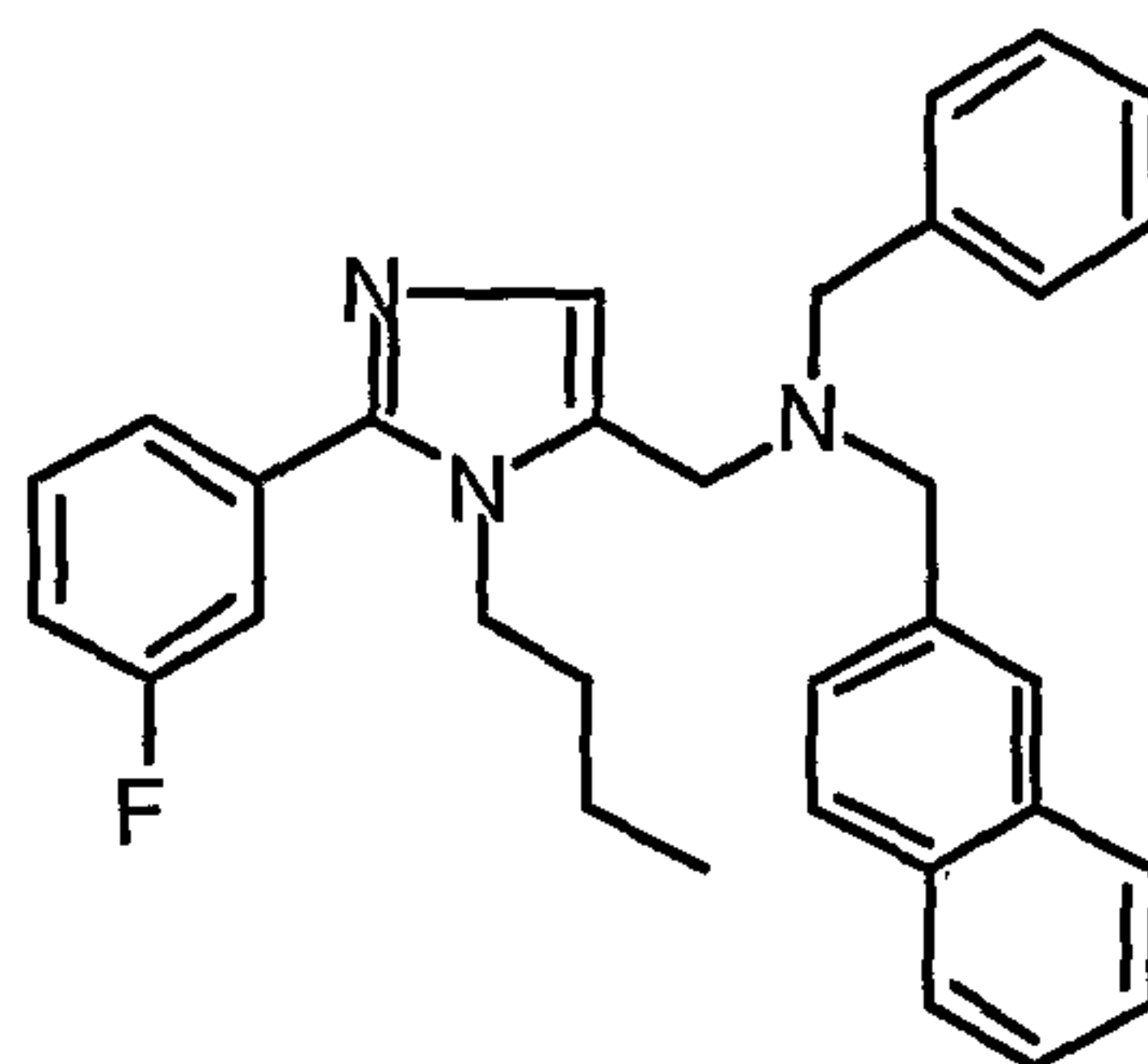
1-(1-Butyl)-2-(3-fluorophenyl)-5-(N-[naphth-2-ylmethyl]-N-phenylmethyl)amino-methylimidazole;
