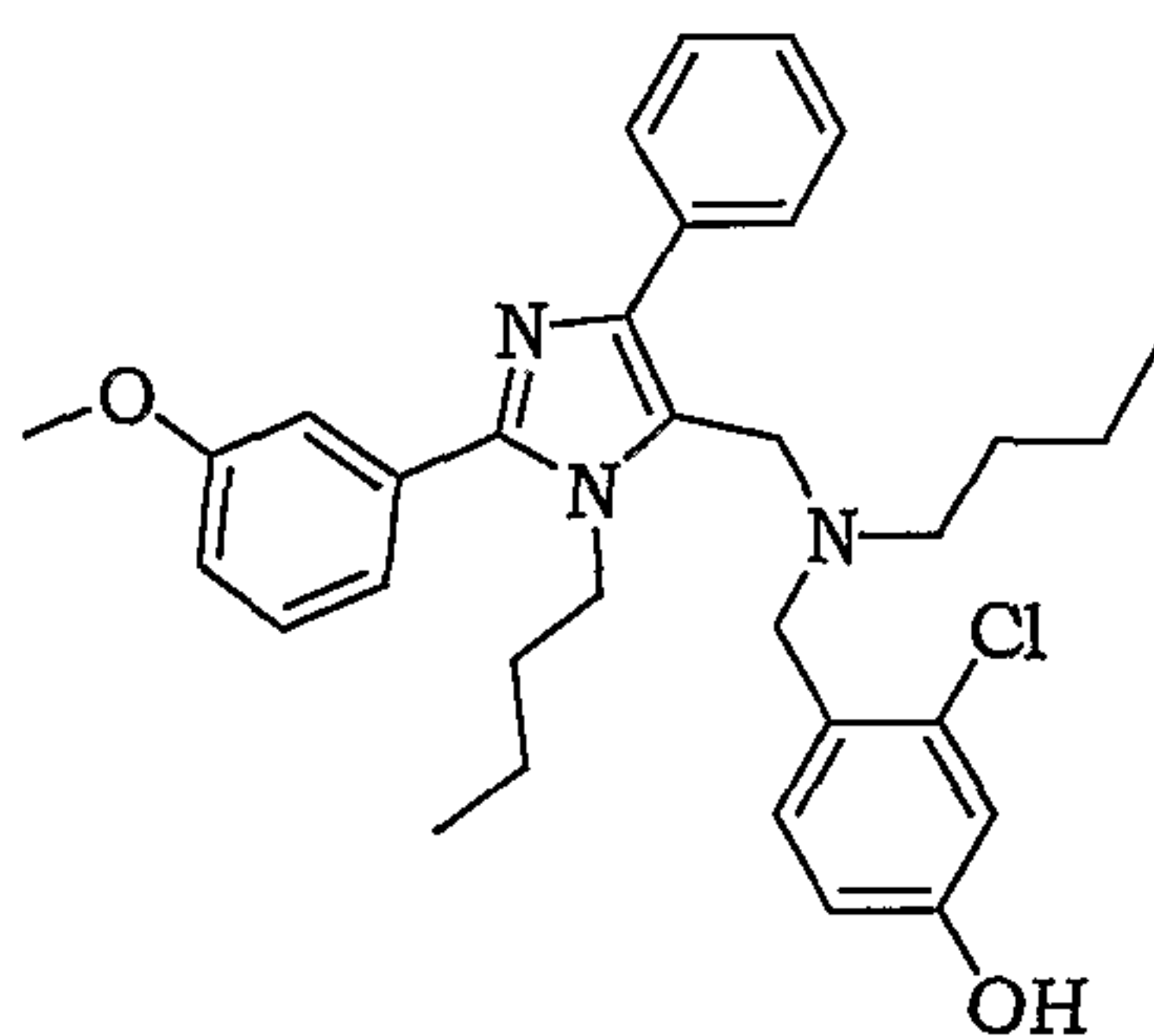
4-((3-butyl-2-(3-methoxy-phenyl)-5-phenyl-3 H -imidazol-4-ylmethyl)-amino)-methyl-3-chlorophenol
