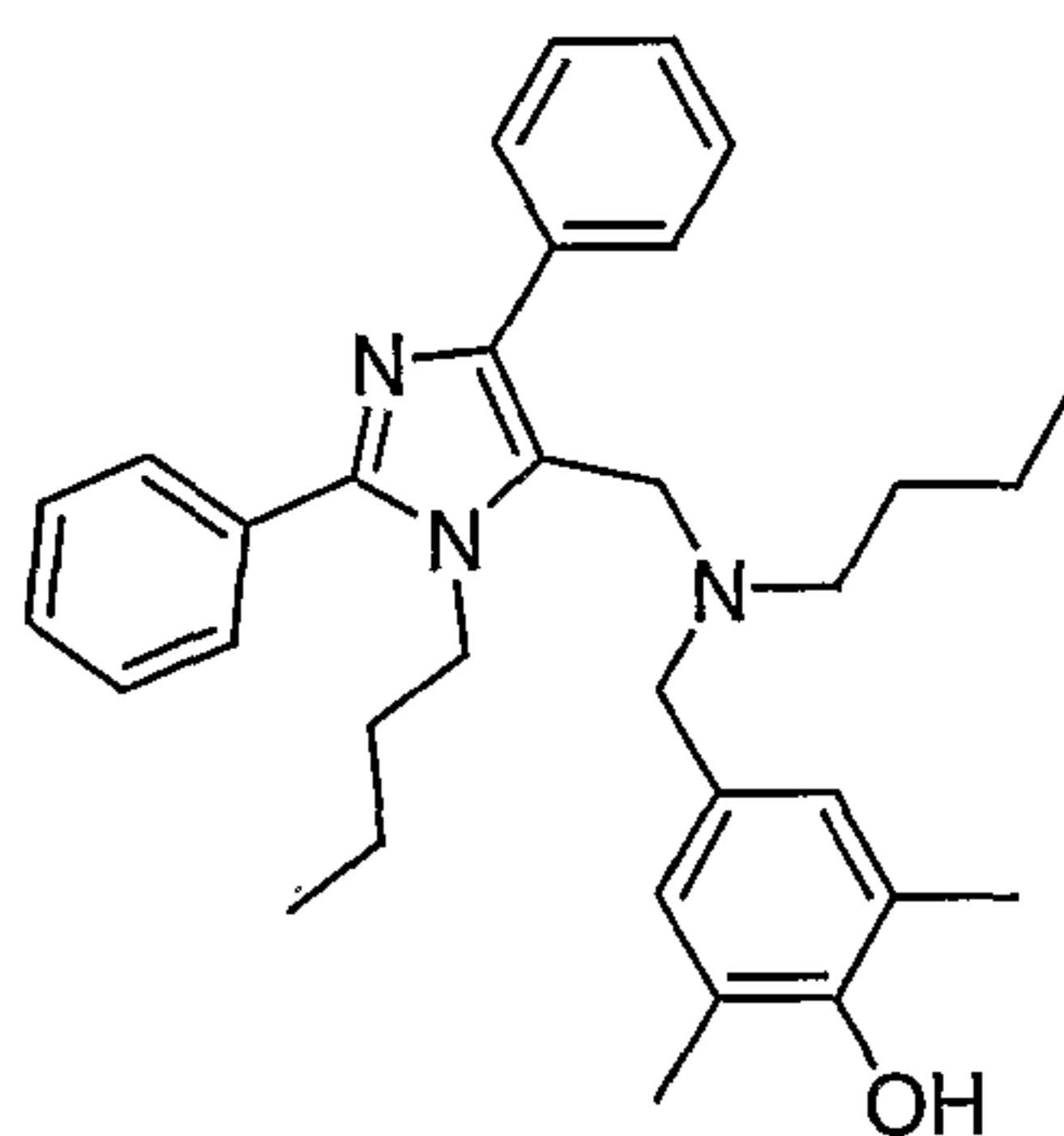
4-((3-butyl-2,5-diphenyl-3 H -imidazol-4-ylmethyl)-amino)-methyl-2,6-dimethyl-phenol
