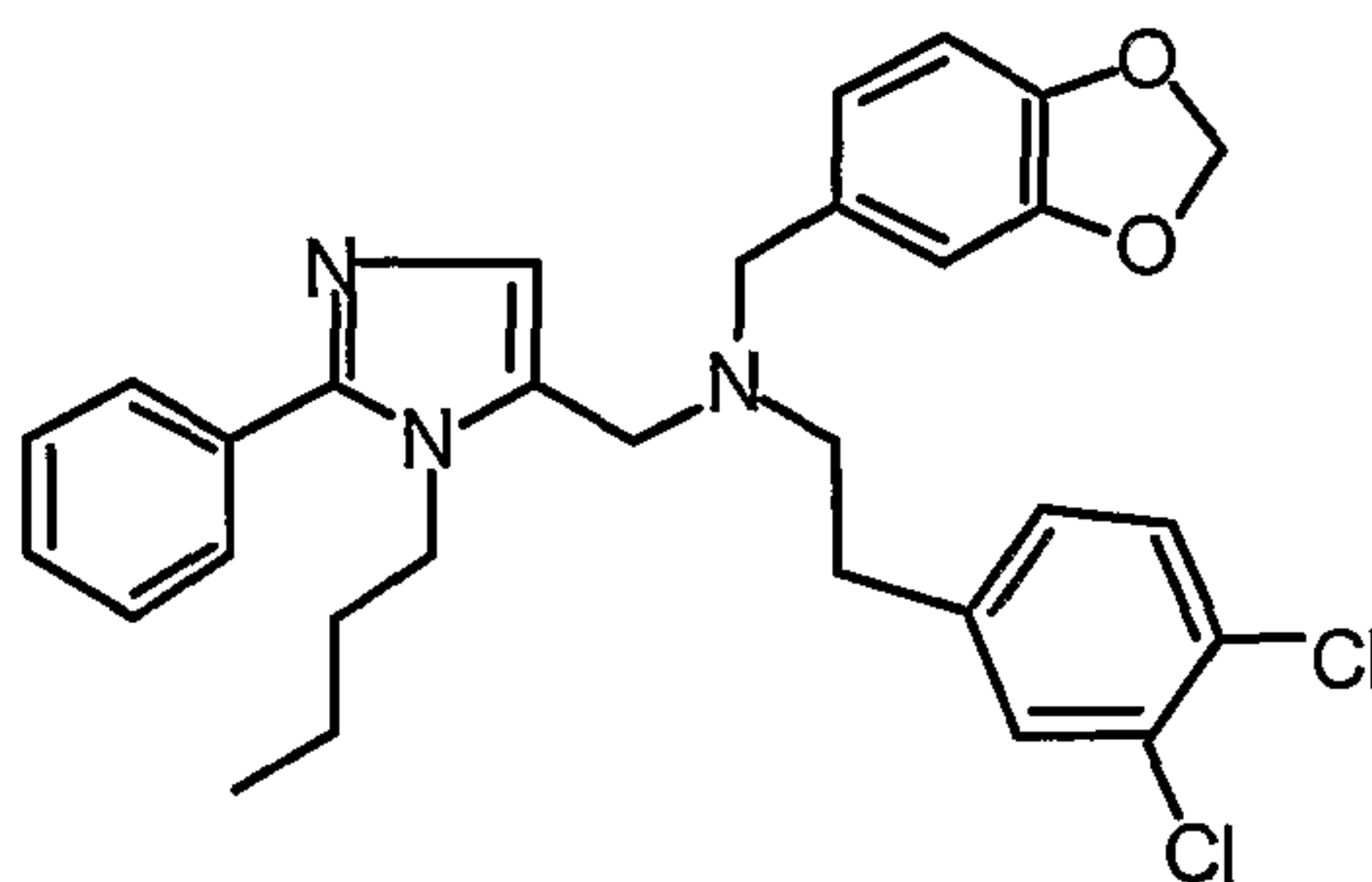
1-(1-Butyl)-2-phenyl-5-(N-[3,4-methylenedioxyphenylmethyl]-N-[3,4-dichlorophenylethyl])aminomethylimidazole;
