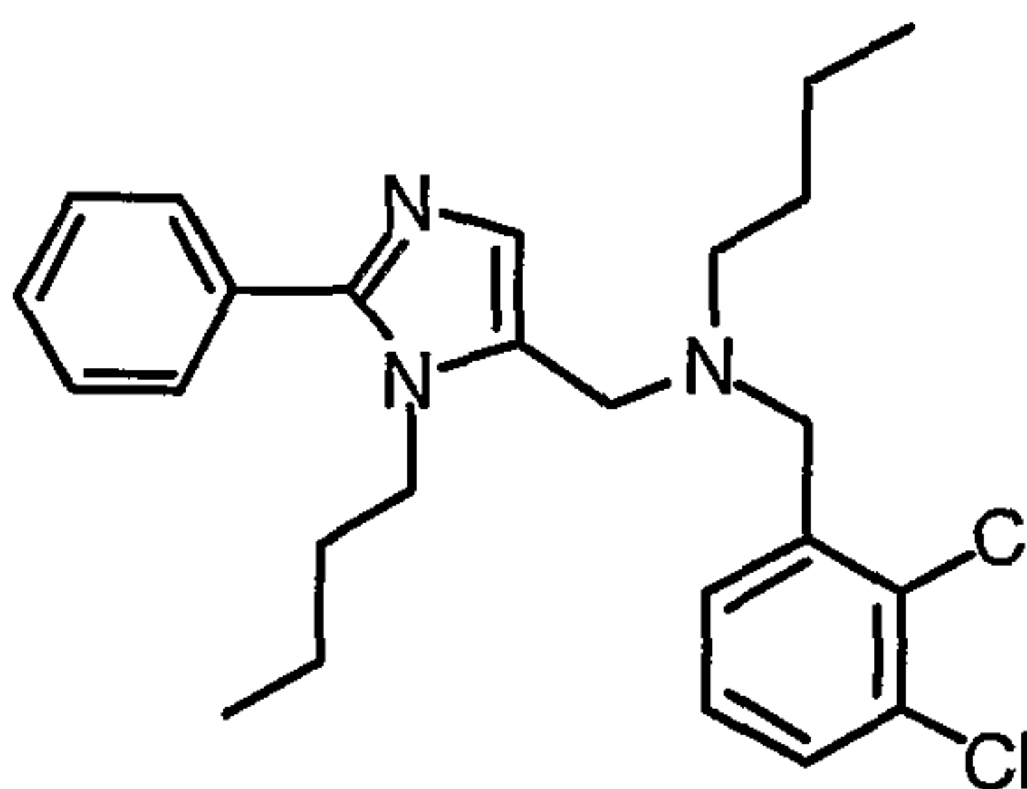
1-(1-Butyl)-2-phenyl-5-(N-[2,3-dichlorophenylmethyl]-N-[1-butyl])aminomethylimidazole;
