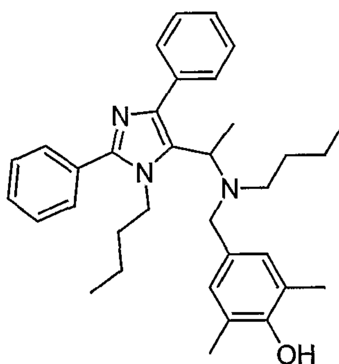
4-((3-butyl-1-(3-butyl-2,5-diphenyl-3 H -imidazol-4-yl)-ethyl)-amino)-methyl-2,6-dimethyl-phenol
