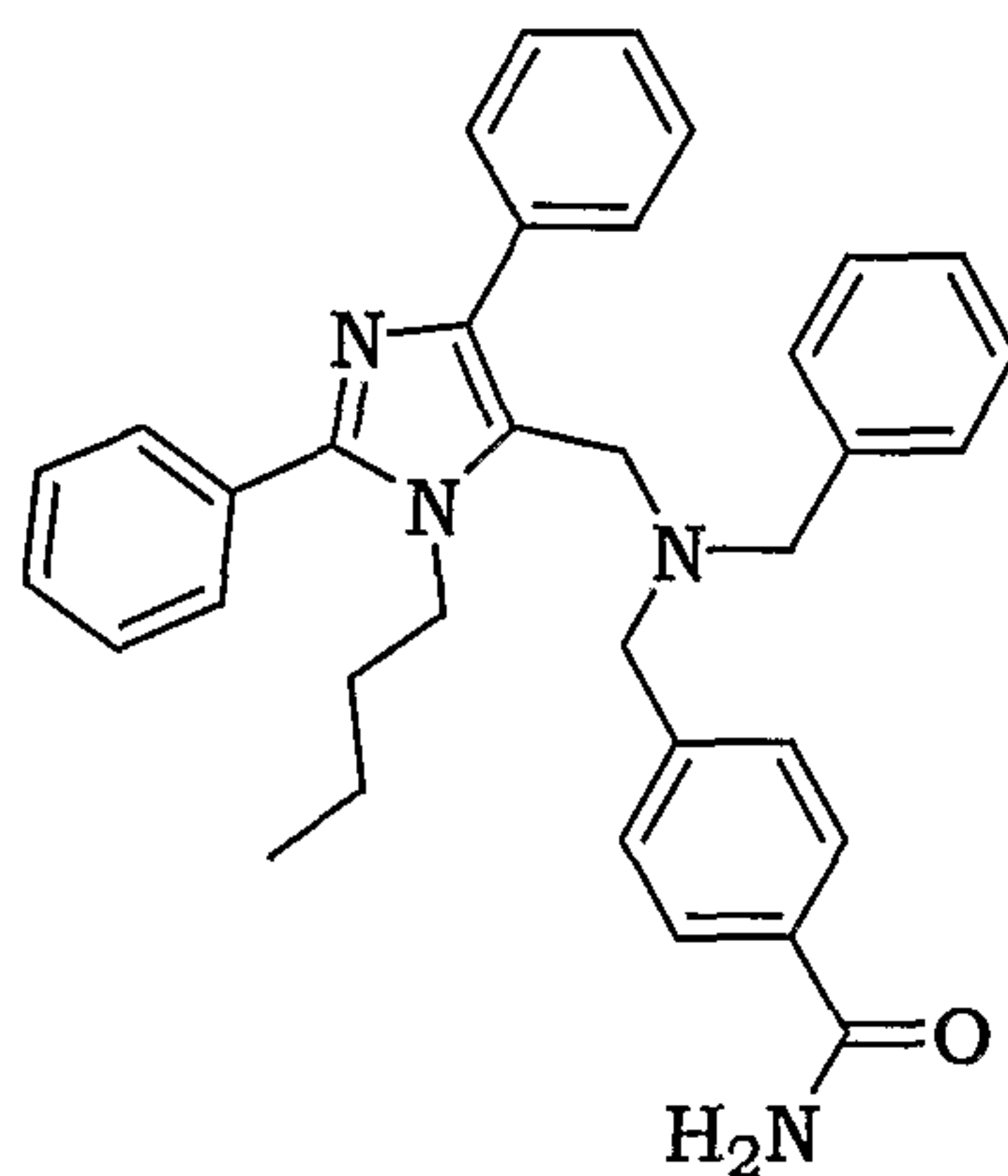
4-[[Benzyl-(3-butyl-2,5-diphenyl-3 H -imidazol-4-ylmethyl)-amino]-methyl]-benzamide
