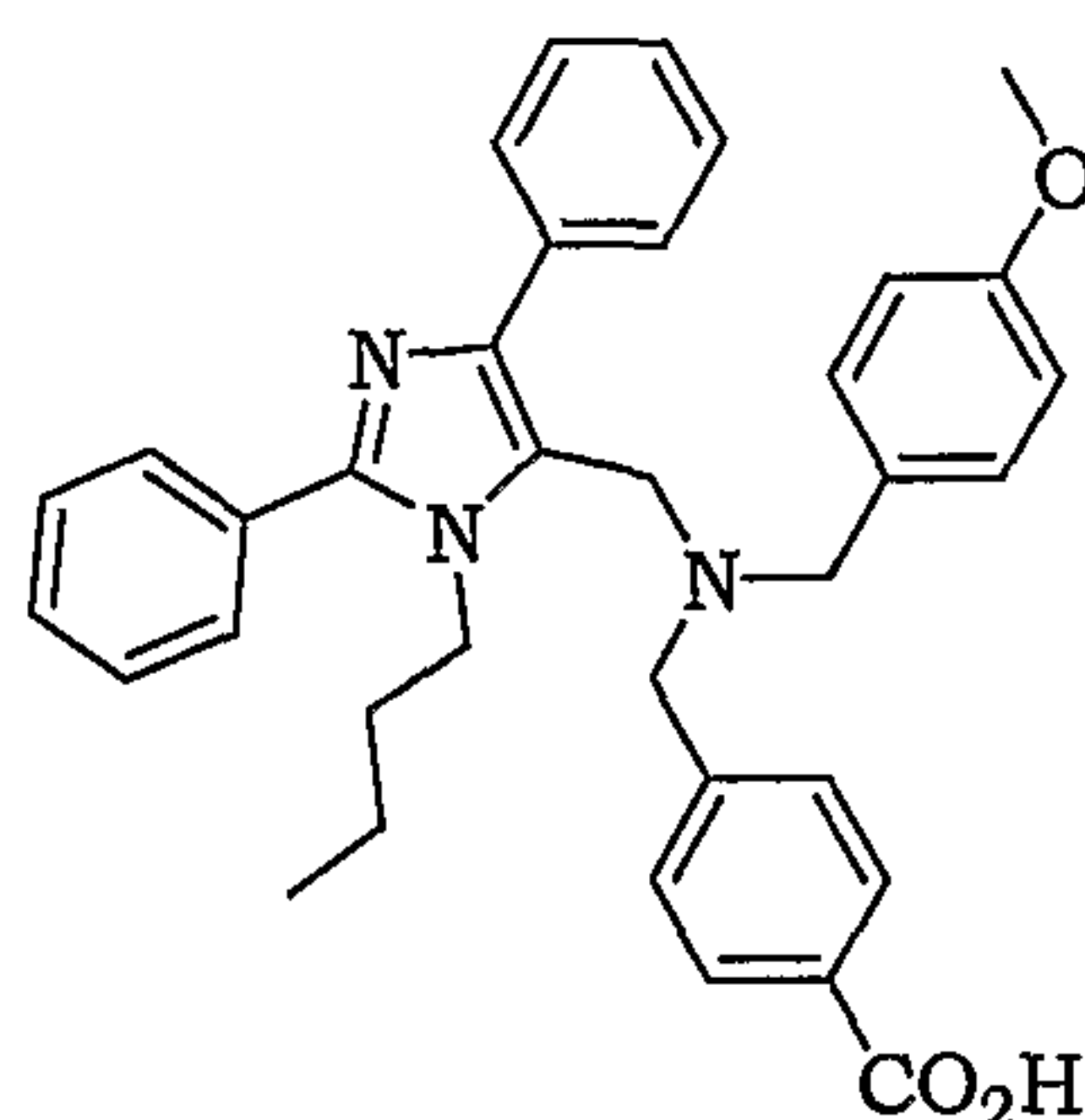
4-((3-butyl-2,5-diphenyl-3 H -imidazol-4-ylmethyl)-(4-methoxy-benzyl)-amino)-methyl-benzoic acid
