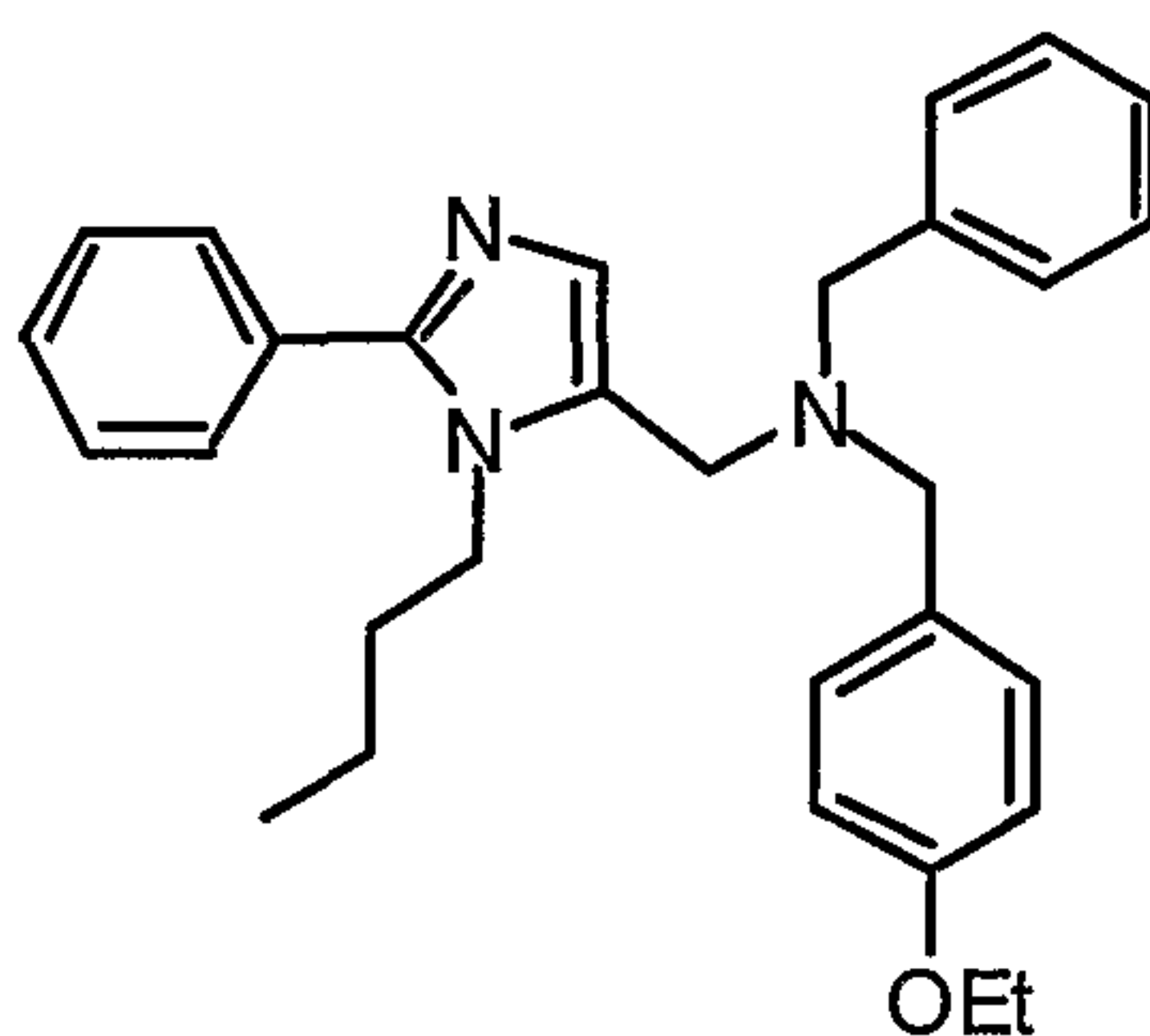
1-(1-Butyl)-2-phenyl-5-(N-[4-ethoxyphenylmethyl]-N-phenylmethyl)aminomethylimidazole;
