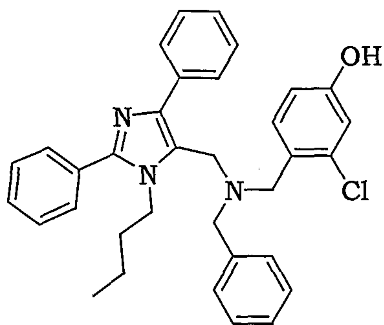
4-[[Benzyl-(3-butyl-2,5-diphenyl-3 H -imidazol-4-ylmethyl)-amino]-methyl]-3-chlorophenol
