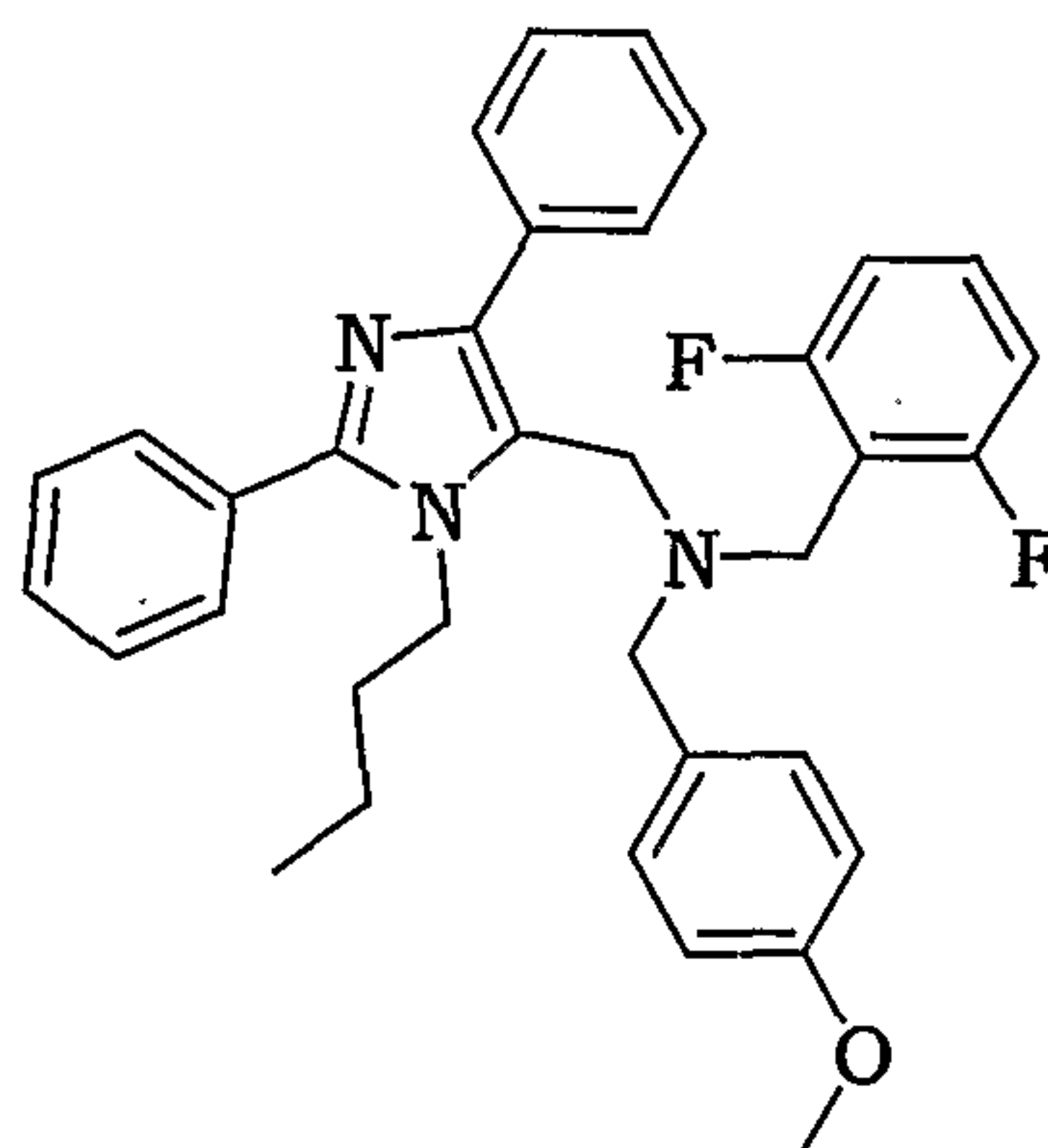
(3-Butyl-2,5-diphenyl-3 H -imidazol-4-ylmethyl)-(2,6-difluoro-benzyl)-(4-methoxy-benzyl)-amine
