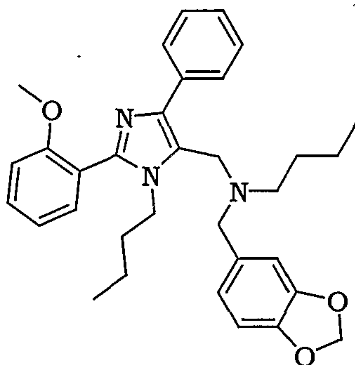
Benzo[1,3]dioxol-5-ylmethyl-butyl-[3-butyl-2-(2-methoxy-phenyl)-5-phenyl-3 H -imidazol-4-yl methyl]-amine
