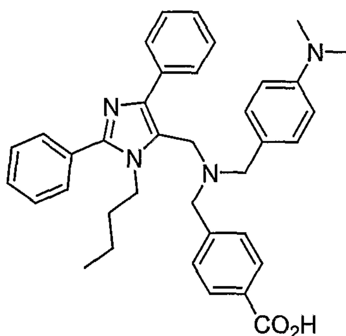
4-((3-butyl-2,5-diphenyl-3 H -imidazol-4-ylmethyl)-(4-dimethylamino-benzyl)-amino)-methyl-benzoic acid
