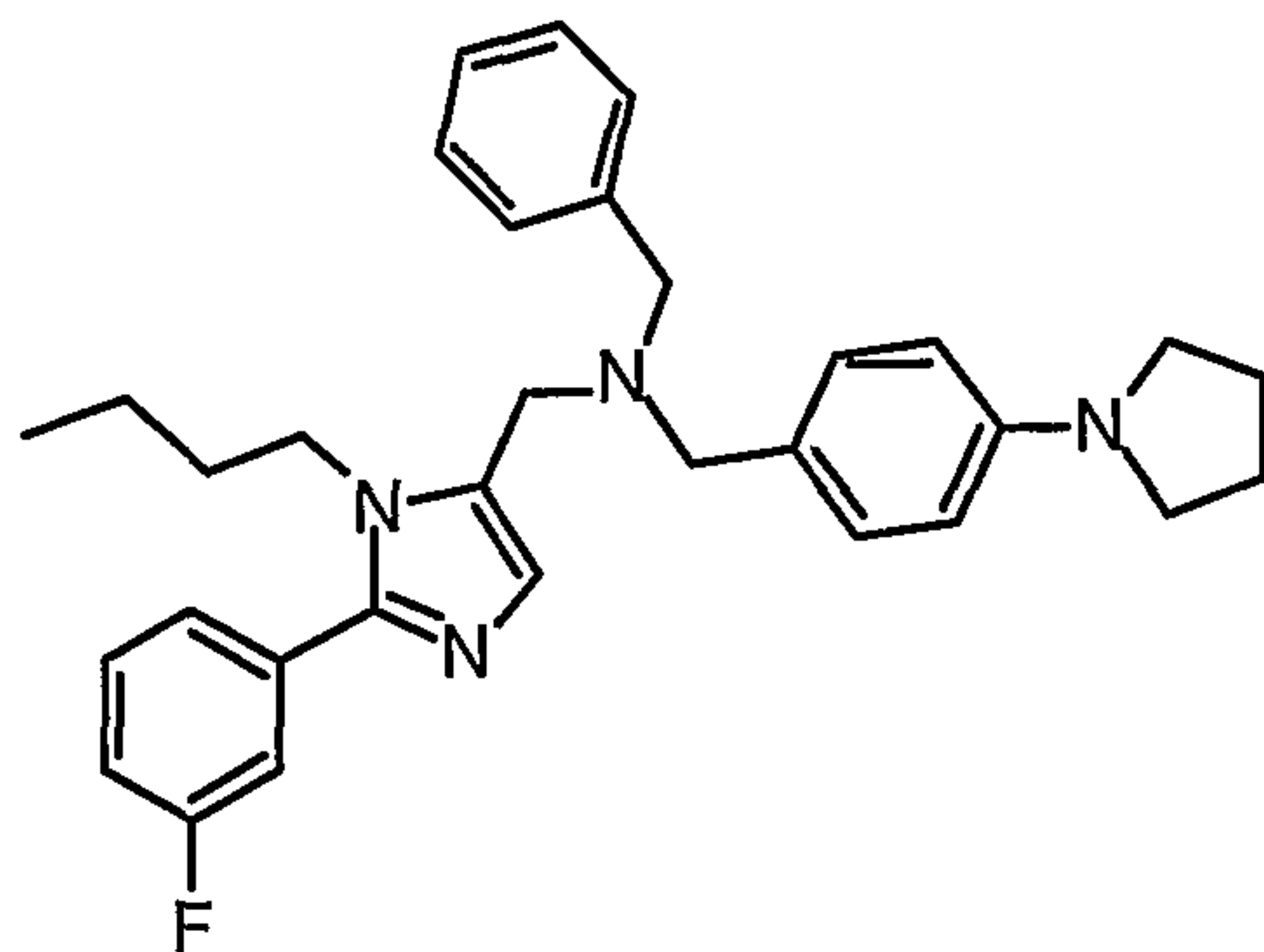
1-(1-Butyl)-2-(3-fluorophenyl)-5-(N-[4-(1-pyrrolidinyl)phenylmethyl]-N-phenylmethyl)amino-methylimidazole;
