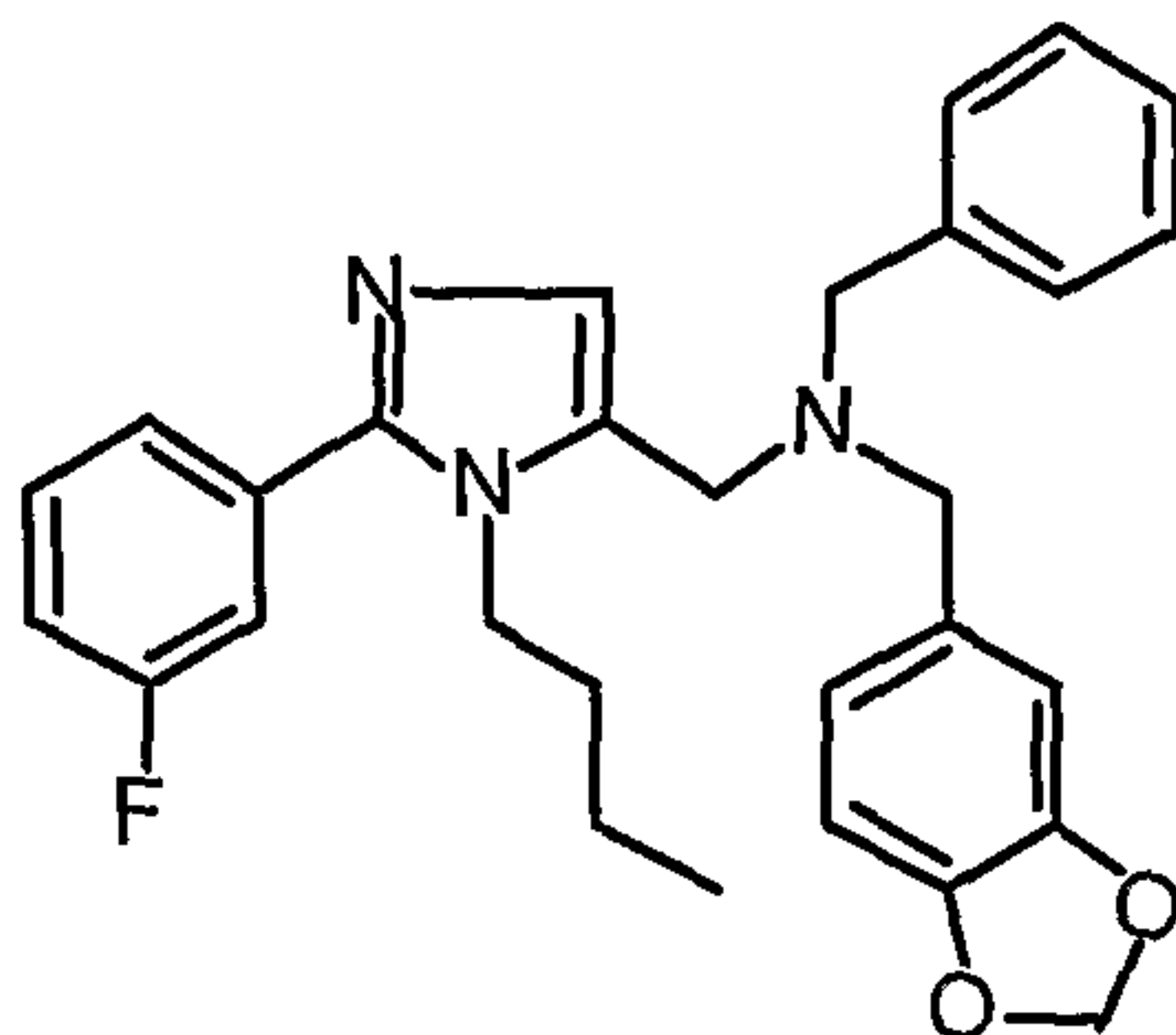
1-(1-Butyl)-2-(3-fluorophenyl)-5-(N-[3,4-methylenedioxyphenylmethyl]-N-phenylmethyl)aminomethylimidazole;
