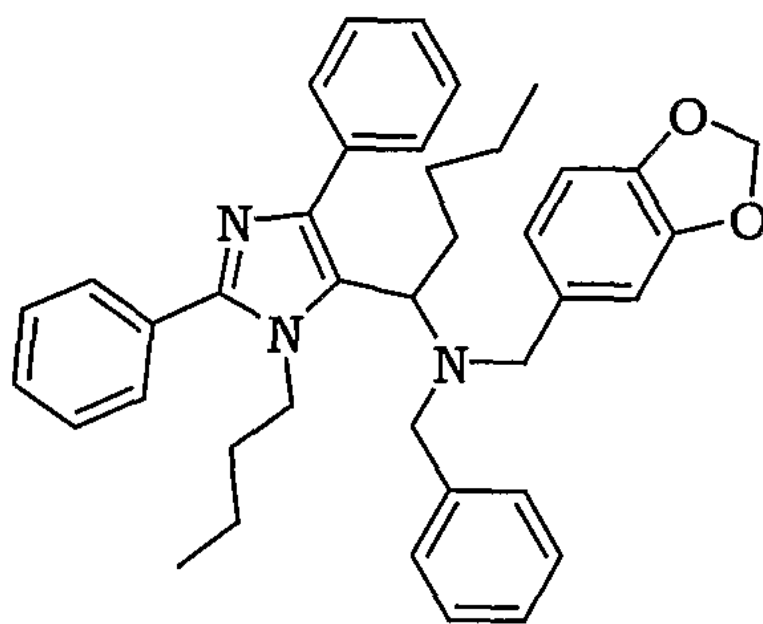
Benzo[1,3]dioxol-5-ylmethyl-benzyl-[1-(3-butyl-2,5-diphenyl-3 H -imidazol-4-yl)-pentyl]-amine
