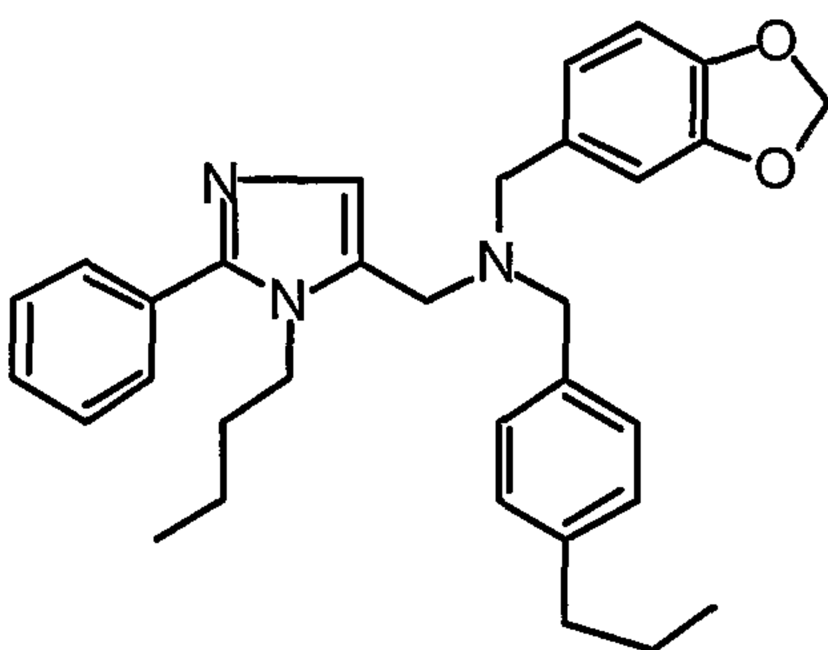
1-(1-Butyl)-2-phenyl-5-(N-[3,4-methylenedioxyphenylmethyl]-N-[4-{1- propyl}phenylmethyl]) aminomethylimidazole;
