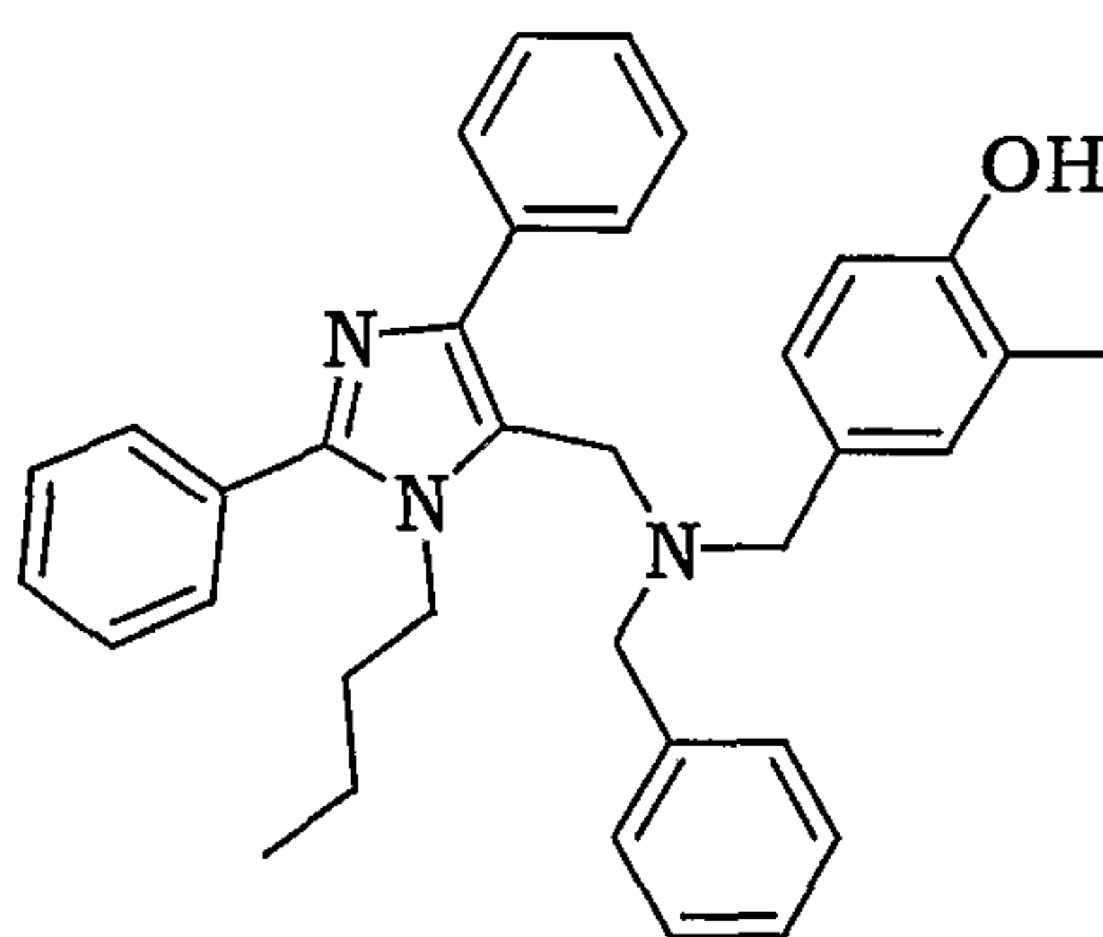
4-[[Benzyl-(3-butyl-2,5-diphenyl-3 H -imidazol-4-ylmethyl)-amino]-methyl]-2-methylphenol
