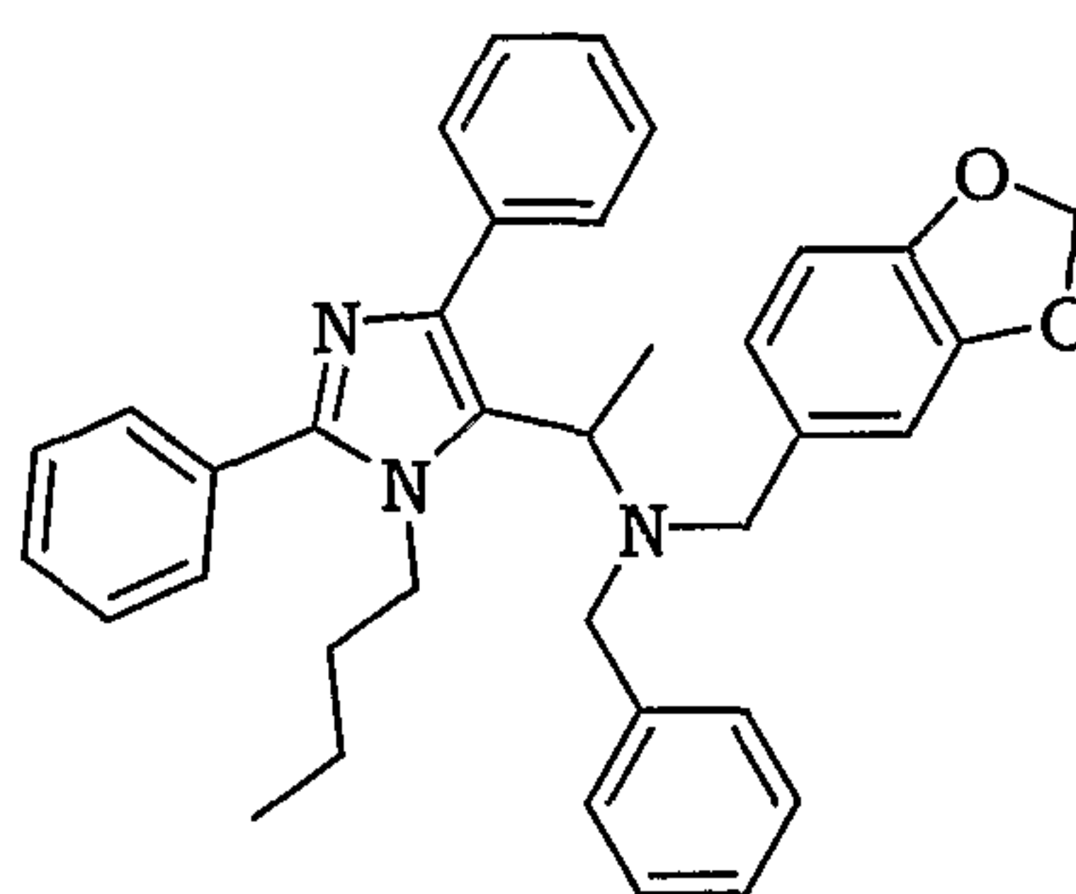
Benzo[1,3]dioxol-5-ylmethyl-benzyl-[1-(3-butyl-2,5-diphenyl-3 H -imidazol-4-yl)-ethyl]-amine
