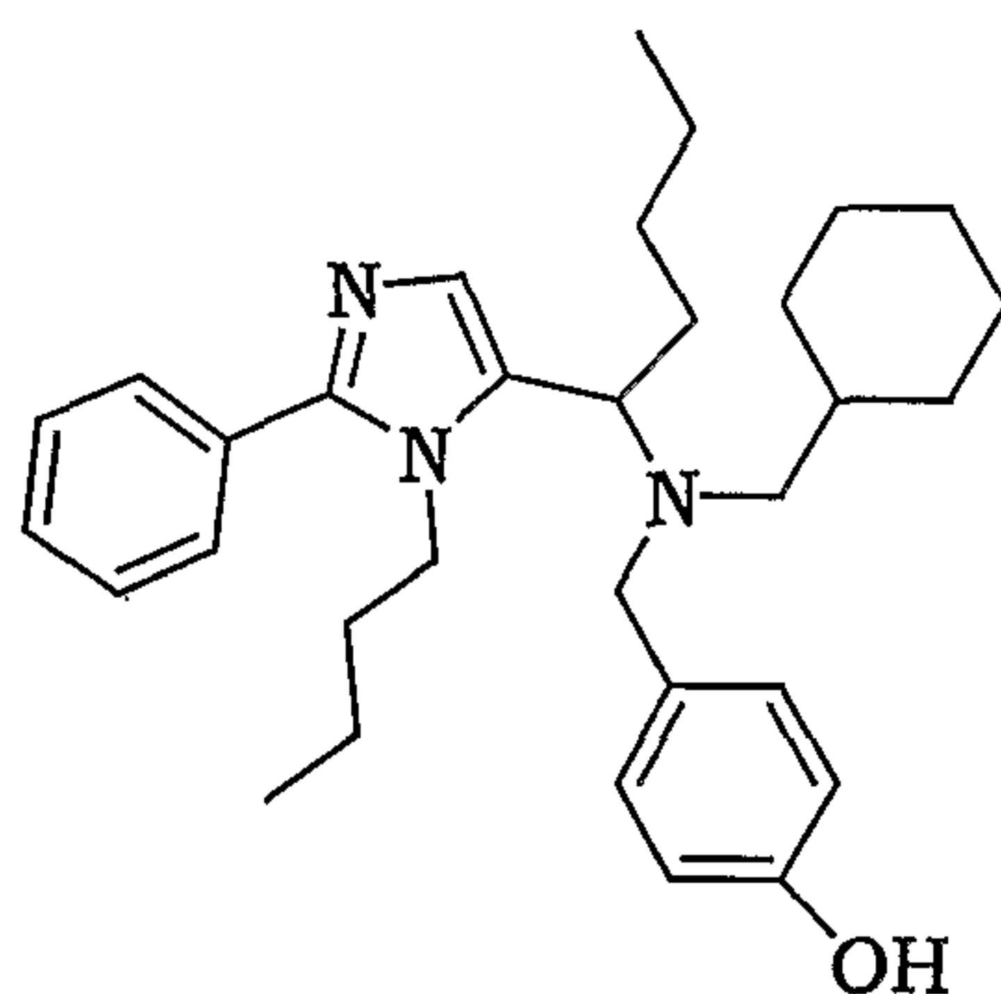
4-[[1-(3-Butyl-2-phenyl-3 H -imidazol-4-yl)-pentyl]-cyclohexylmethyl-amino]-methylphenol
