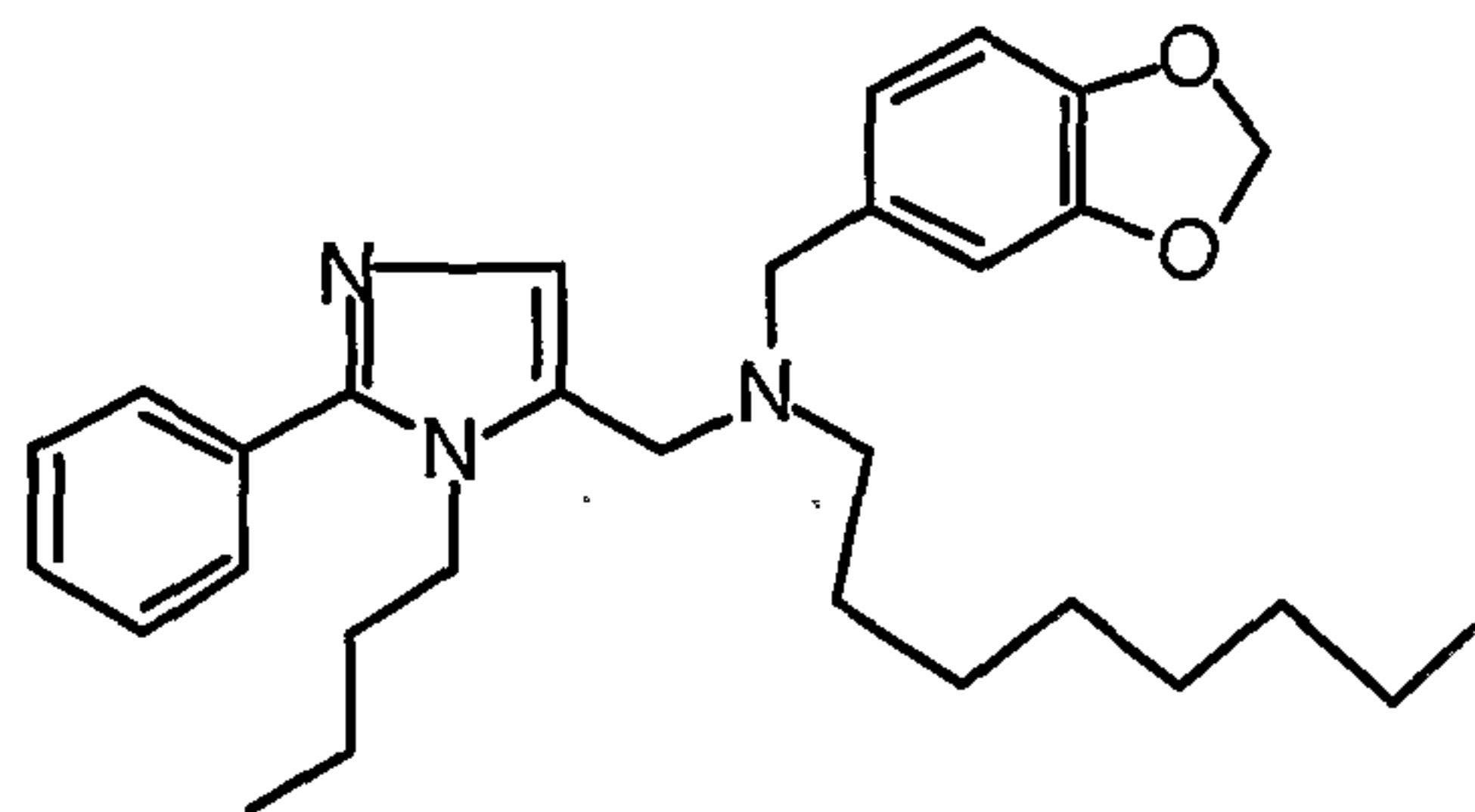
1-(1-Butyl)-2-phenyl-5-(N-[3,4-methylenedioxyphenylmethyl]-N-[1-n-octyl]aminomethyl)-imidazole;
