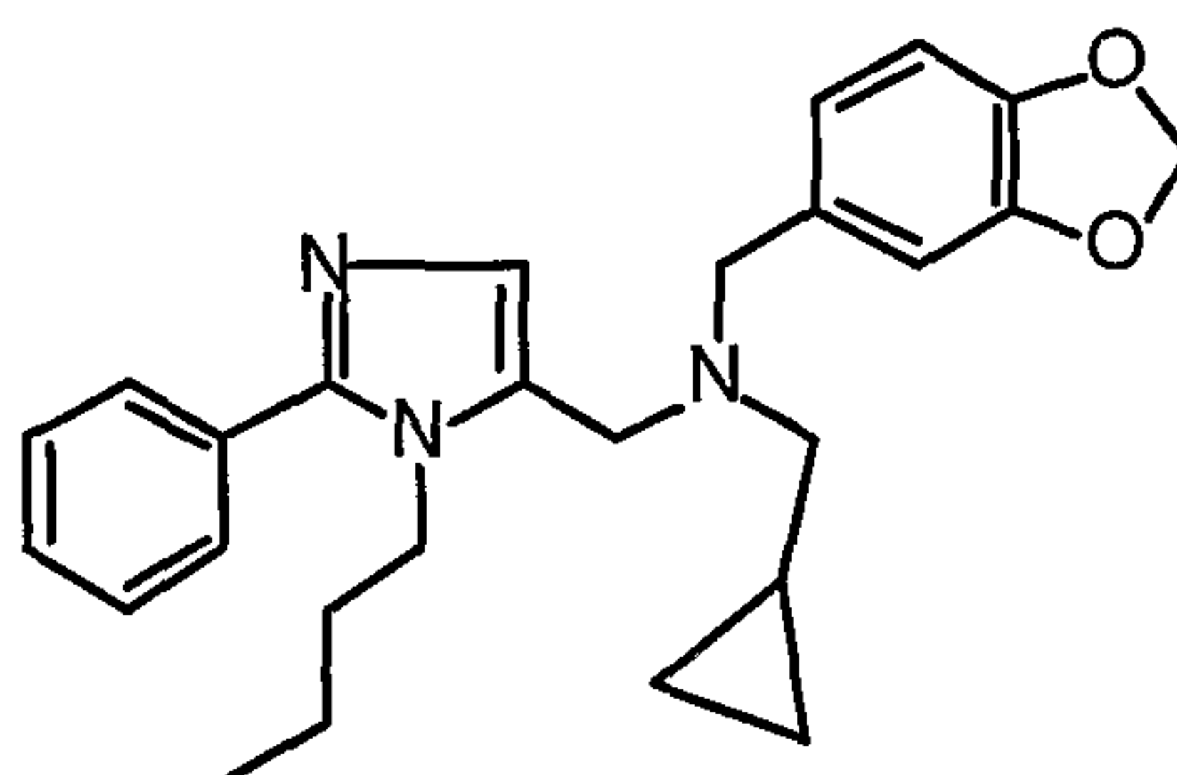
1-(1-Butyl)-2-phenyl-5-(N-[3,4-methylenedioxyphenylmethyl]-N-cyclopropylmethyl)amino-methylimidazole;
