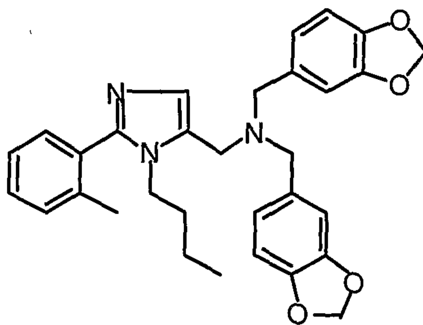
1-(1-Butyl)-2-(2-methylphenyl)-5-(N,N-di[3,4-methylenedioxyphenylmethyl])amino-methylimidazole;
