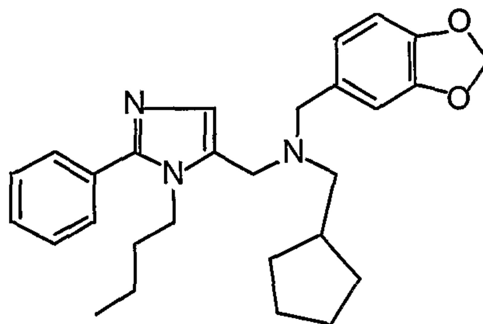
1-(1-Butyl)-2-phenyl-5-(N-[3,4-methylenedioxyphenylmethyl]-N-cyclopentylmethyl)amino-methylimidazole;
