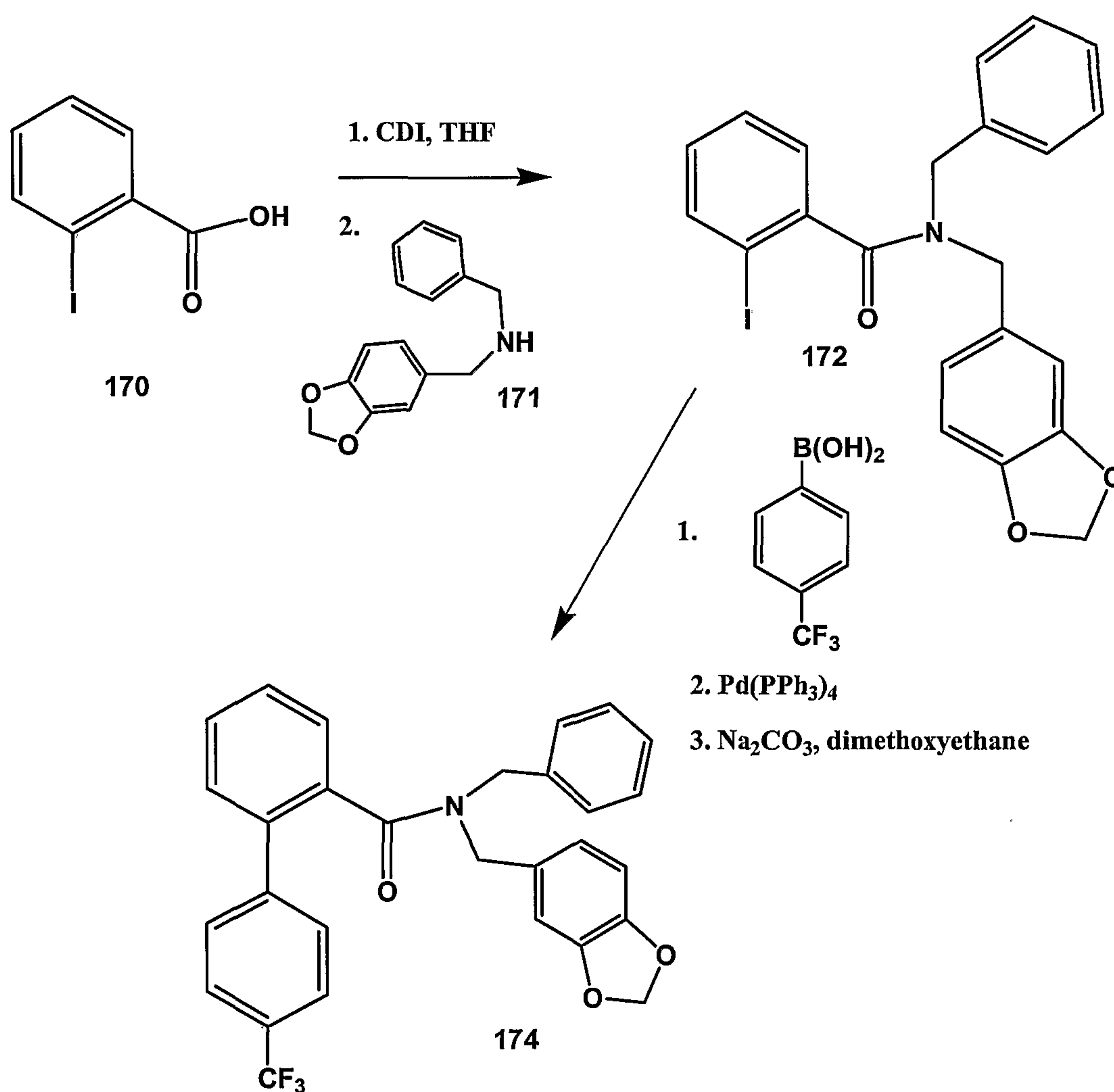
4'-Trifluoromethyl-biphenyl-2-carboxylic acid benzo[1,3]dioxol-5-ylmethyl-benzyl-amide
