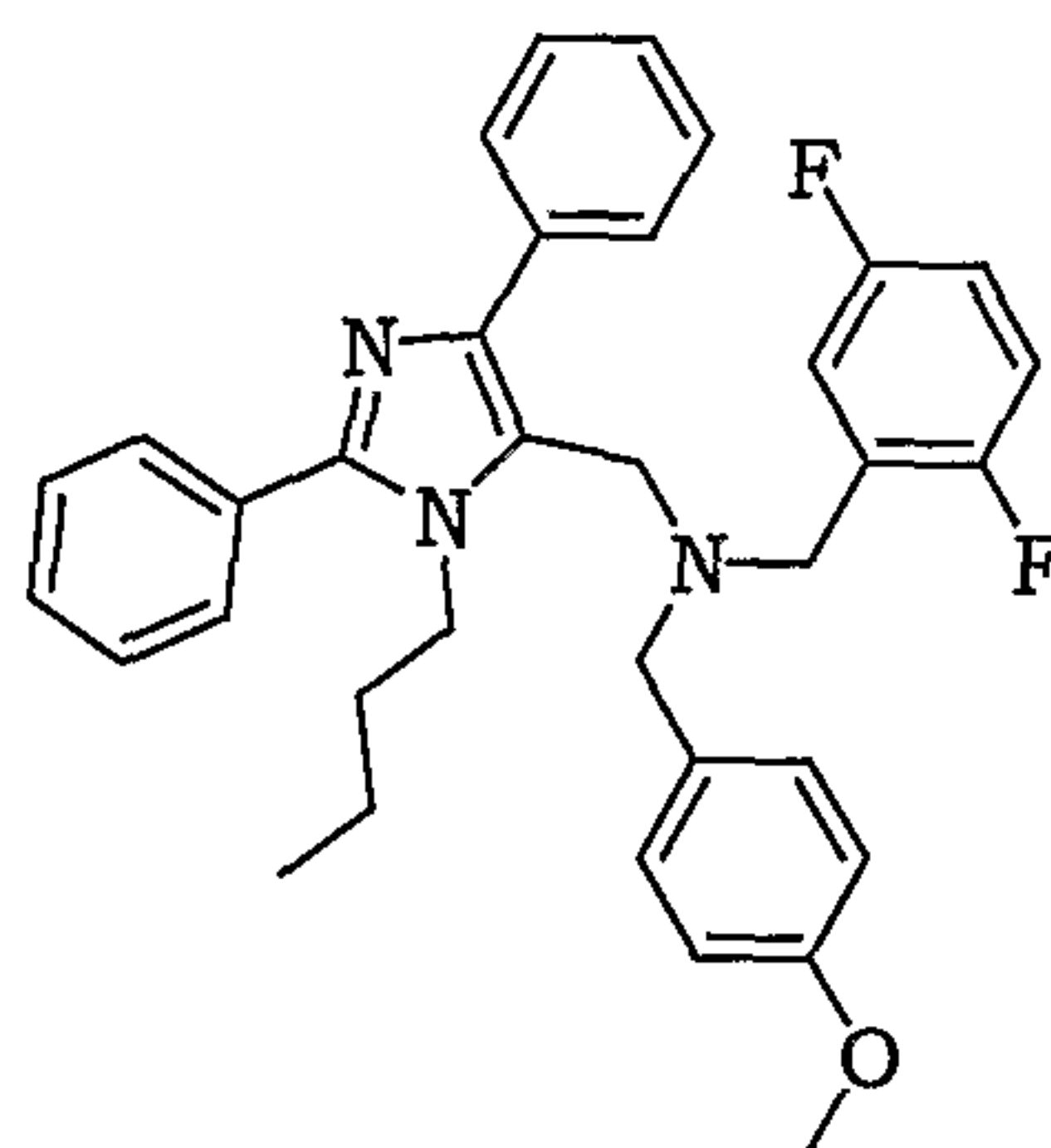
(3-Butyl-2,5-diphenyl-3 H -imidazol-4-ylmethyl)-(2,5-difluoro-benzyl)-(4-methoxy-benzyl)-amine
