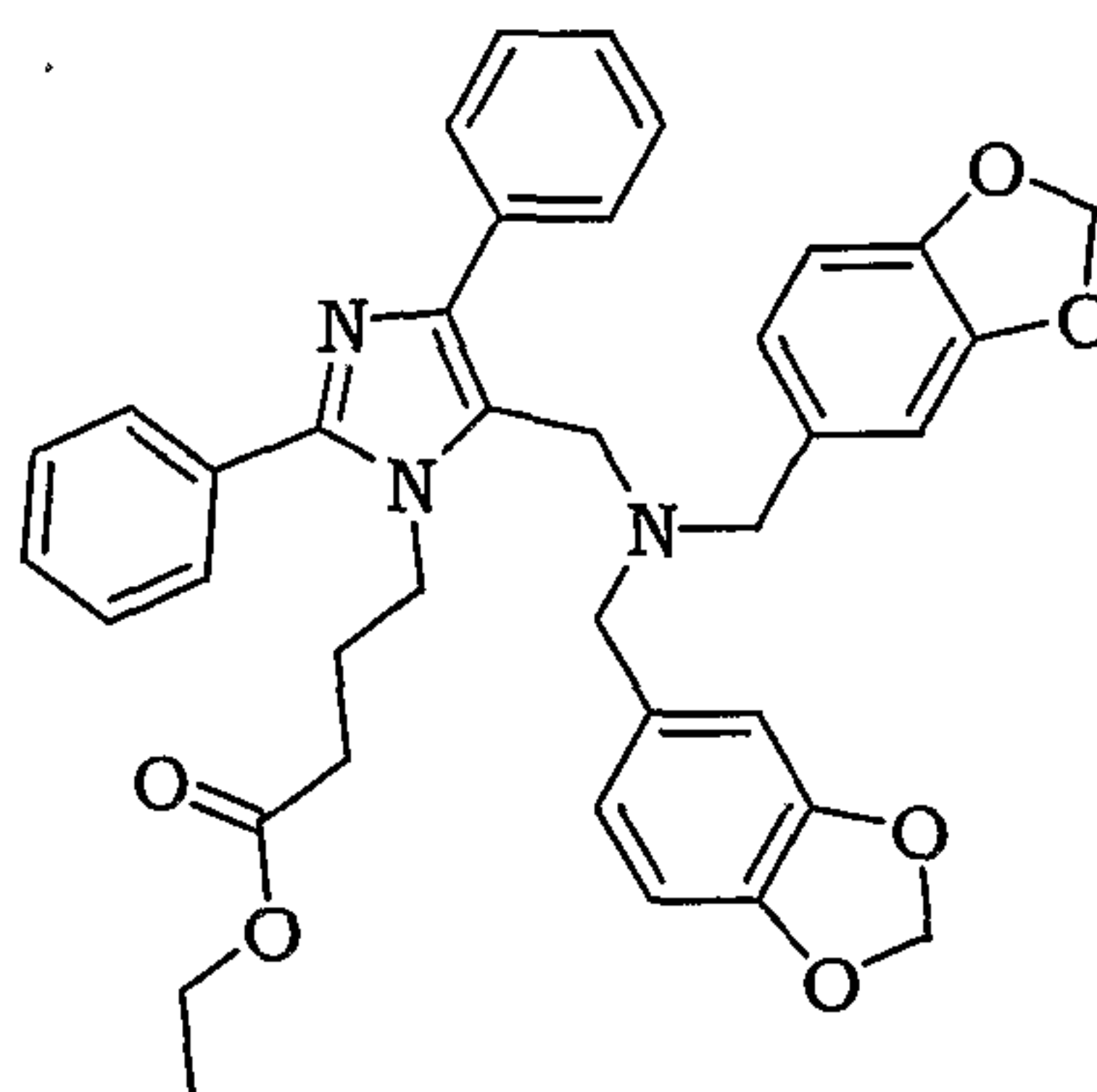
4-{5-[(Bis-benzo[1,3]dioxol-5-ylmethyl-amino)-methyl]-2,4-diphenyl-imidazol-1-yl}-butyric acid ethyl ester
