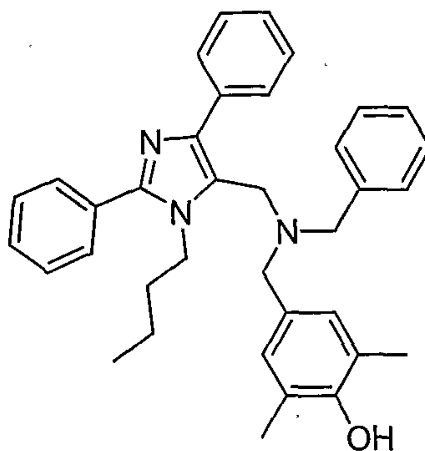
4-[[Benzyl-(3-butyl-2,5-diphenyl-3H-imidazol-4-ylmethyl)-amino]-methyl]-2,6-dimethyl-phenol
