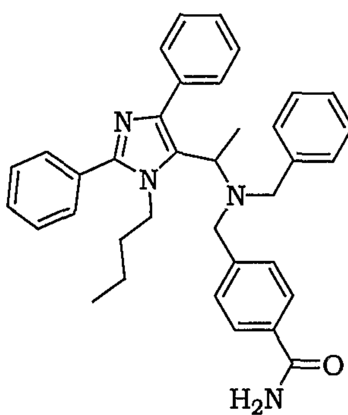
4-({Benzyl-[1-(3-butyl-2,5-diphenyl-3 H -imidazol-4-yl)-ethyl]-amino}-methyl)-benzamide
