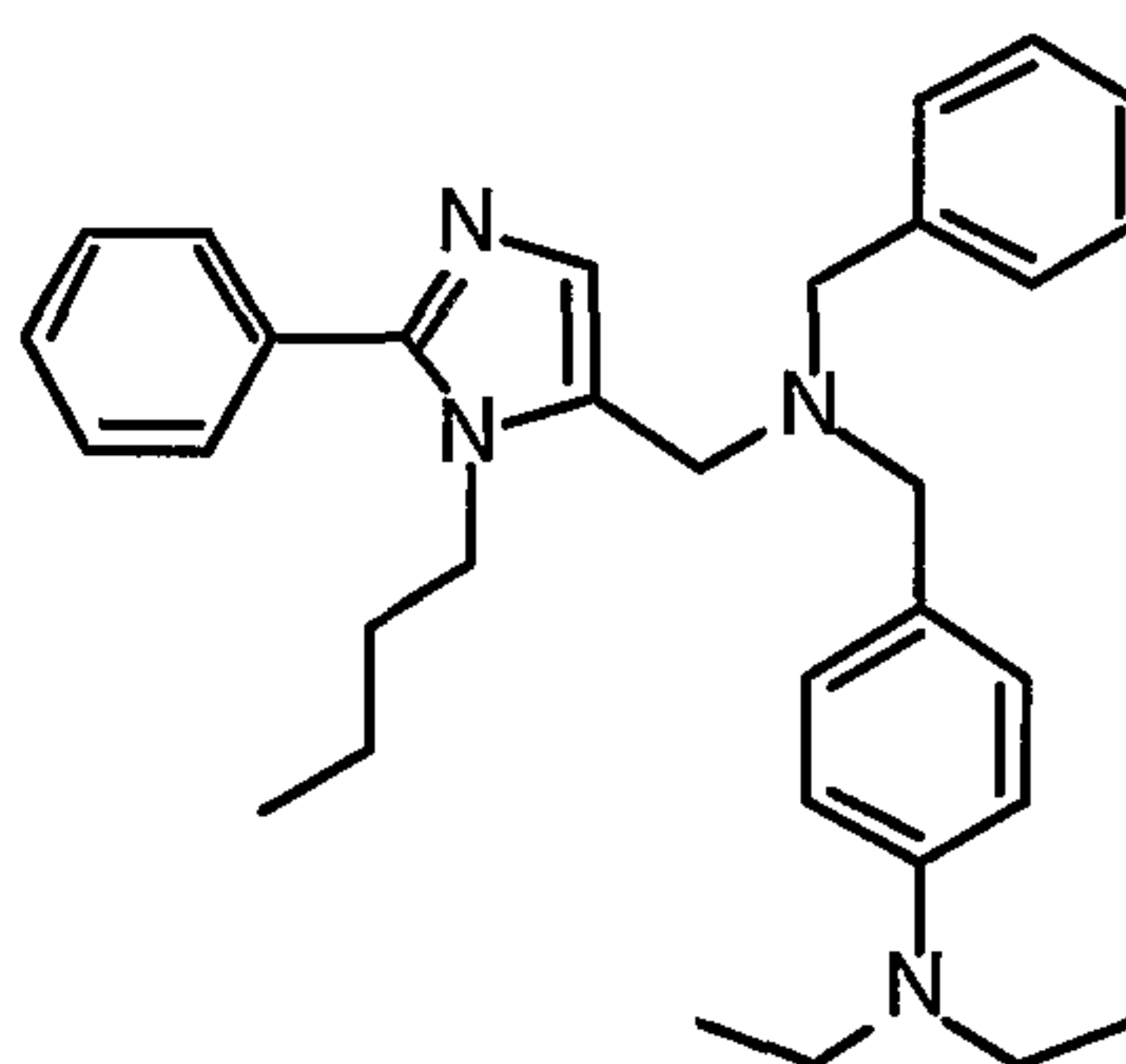
1-(1-Butyl)-2-phenyl-5-(N-[4-diethylaminophenylmethyl]-N-phenylmethyl)aminomethyl-imidazole;
