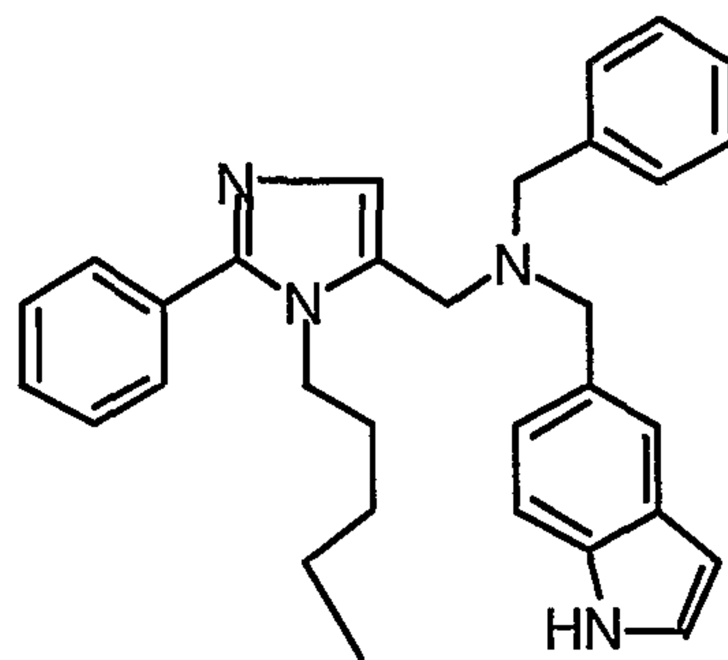
1-(1-Pentyl)-2-phenyl-5-(N-[indol-5-ylmethyl]-N-phenylmethyl) aminomethylimidazole;
