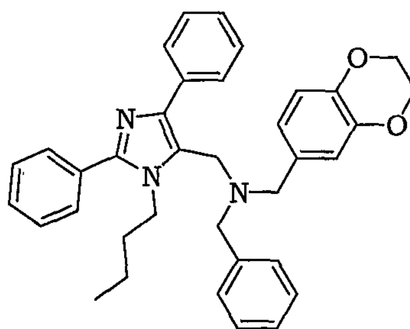
Benzyl-(3-butyl-2,5-diphenyl-3 H -imidazol-4-ylmethyl)-(2,3-dihydro-benzo[1,4]dioxin-6-ylmethyl)-amine
