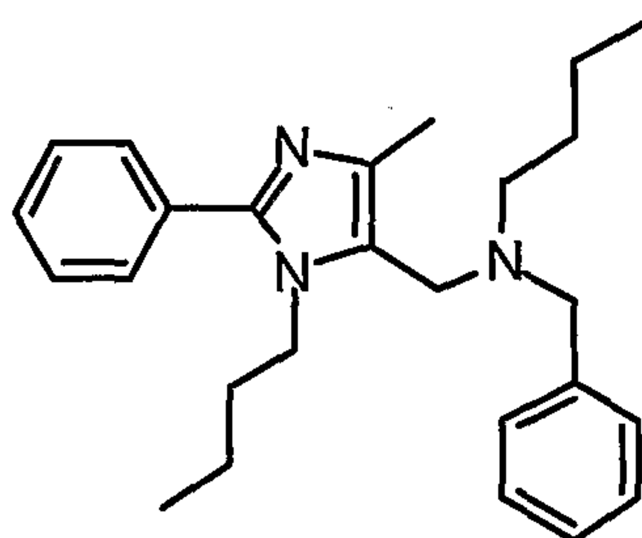
1-(1-Butyl)-2-phenyl-4-methyl-5-(N-phenylmethyl-N-[1-butyl])aminomethylimidazole;
