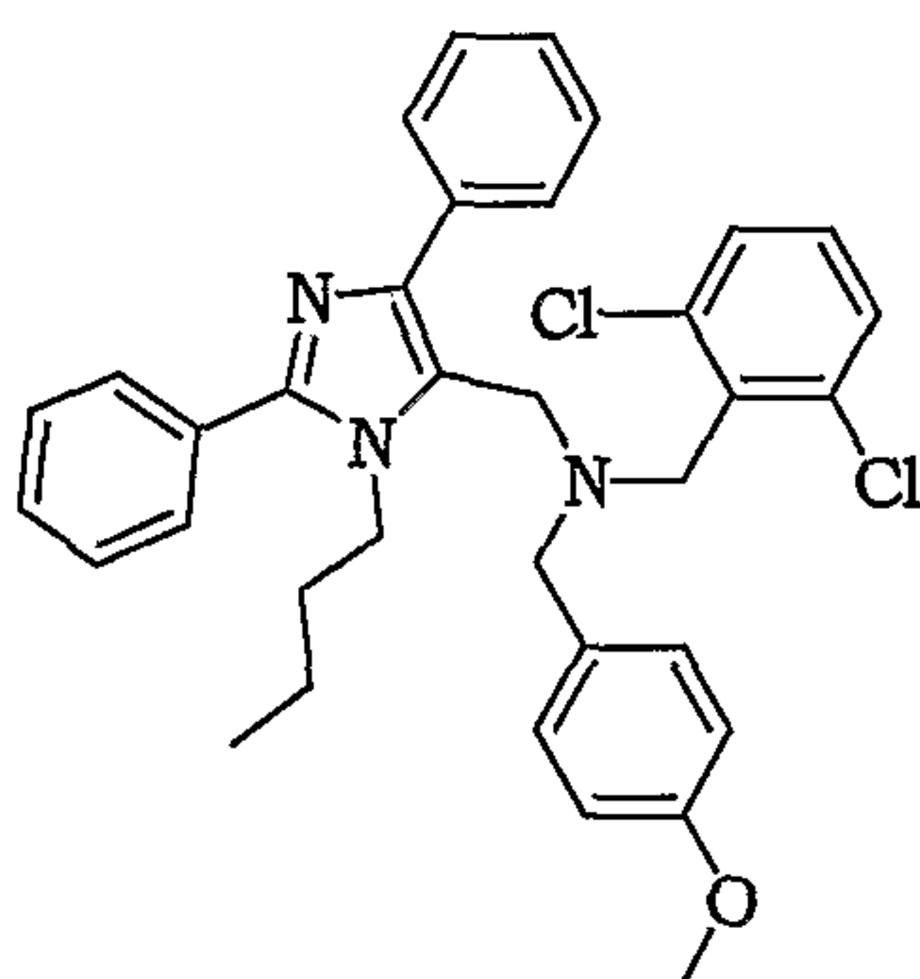
(3-Butyl-2,5-diphenyl-3 H -imidazol-4-ylmethyl)-(2,6-dichloro-benzyl)-(4-methoxy-benzyl)-amine
