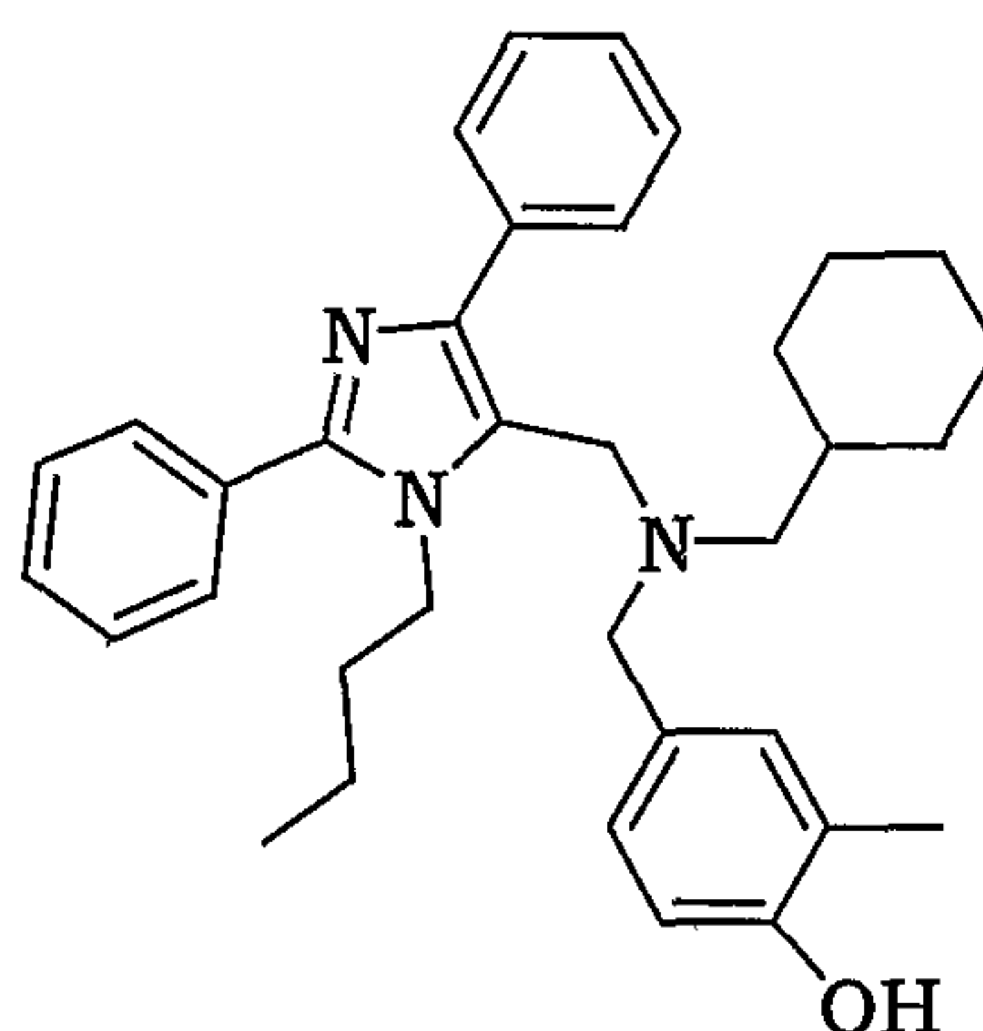
4-[[3-Butyl-2,5-diphenyl-3 H -imidazol-4-ylmethyl]-cyclohexylmethyl-amino]-methyl]-2-methylphenol
