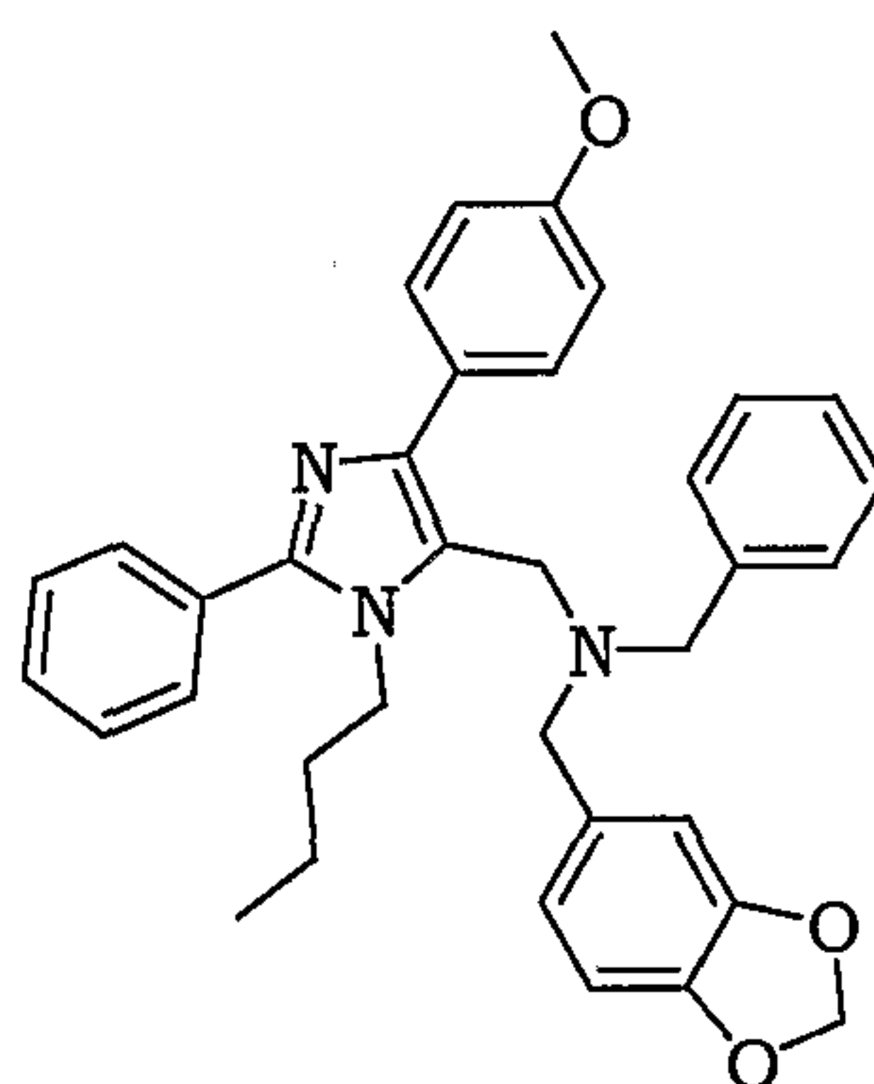
Benzo[1,3]dioxol-5-ylmethyl-benzyl-[3-butyl-5-(4-methoxy-phenyl)-2-phenyl-3 H -imidazol-4-ylmethyl]-amine
