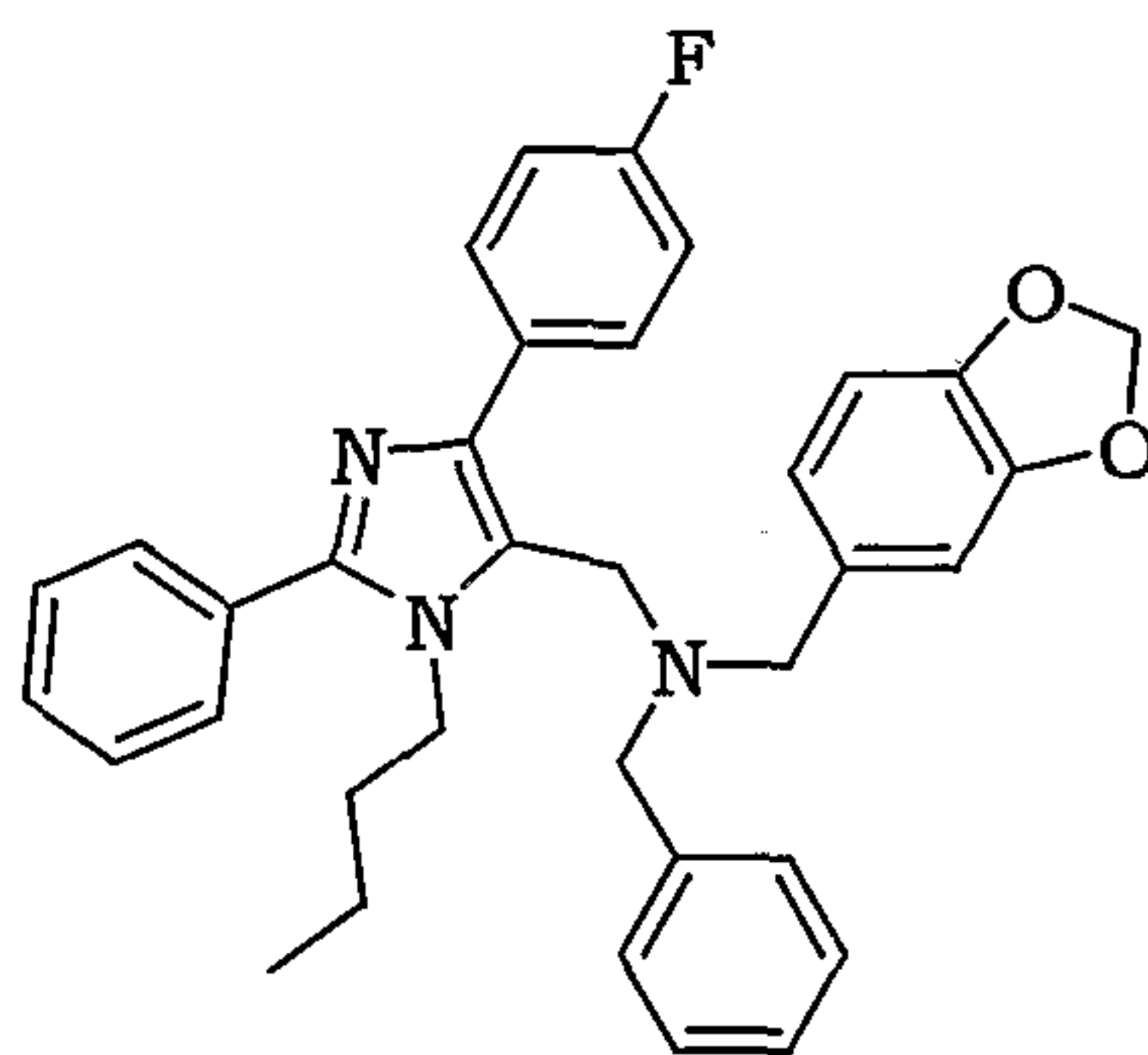
Benzo[1,3]dioxol-5-ylmethyl-benzyl-[3-butyl-5-(4-fluoro-phenyl)-2-phenyl-3 H -imidazol-4-ylmethyl]-amine
