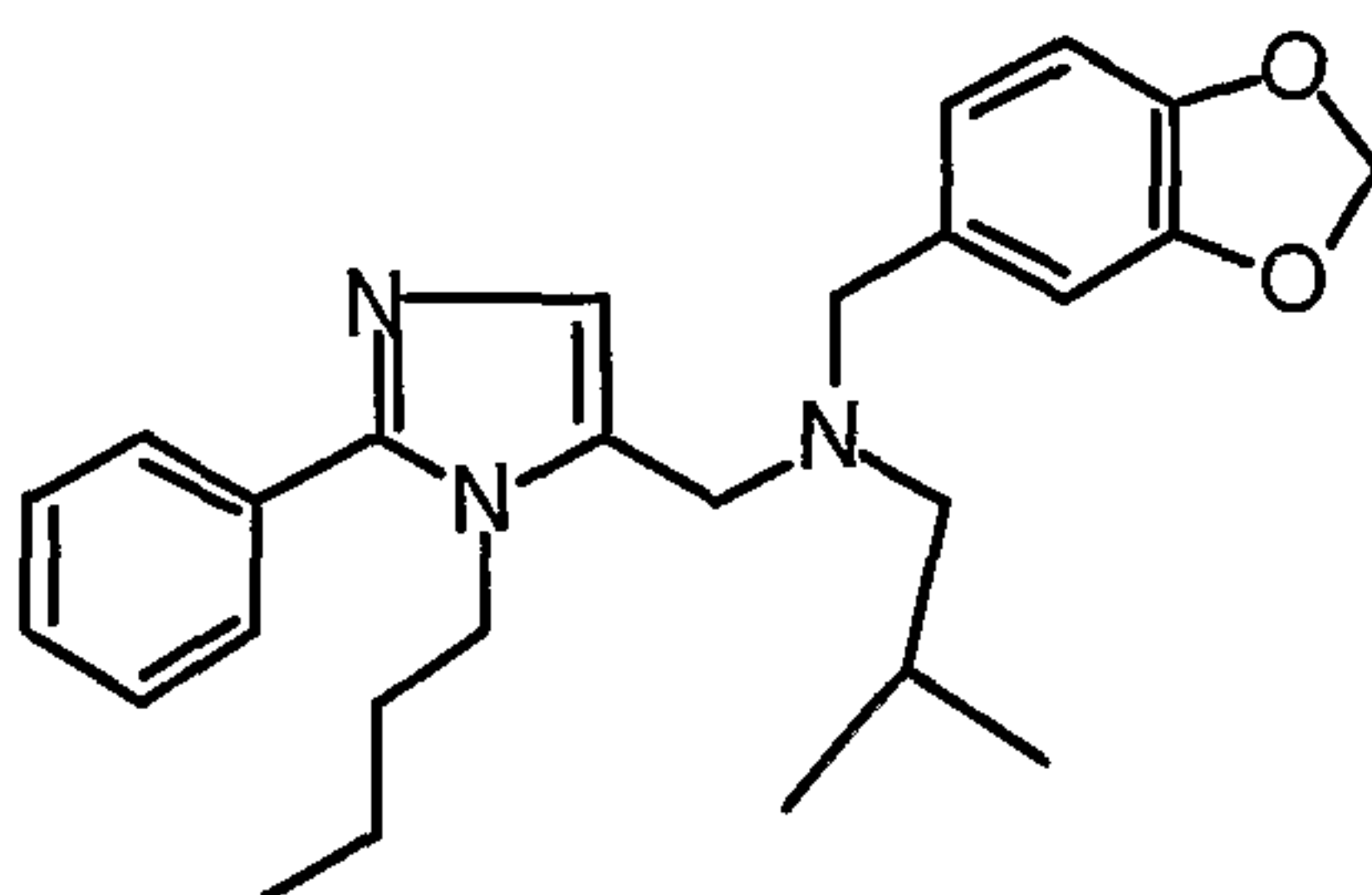
1-(1-Butyl)-2-phenyl-5-(N-[3,4-methylenedioxyphenylmethyl]-N-isobutyl)aminomethyl-imidazole;
