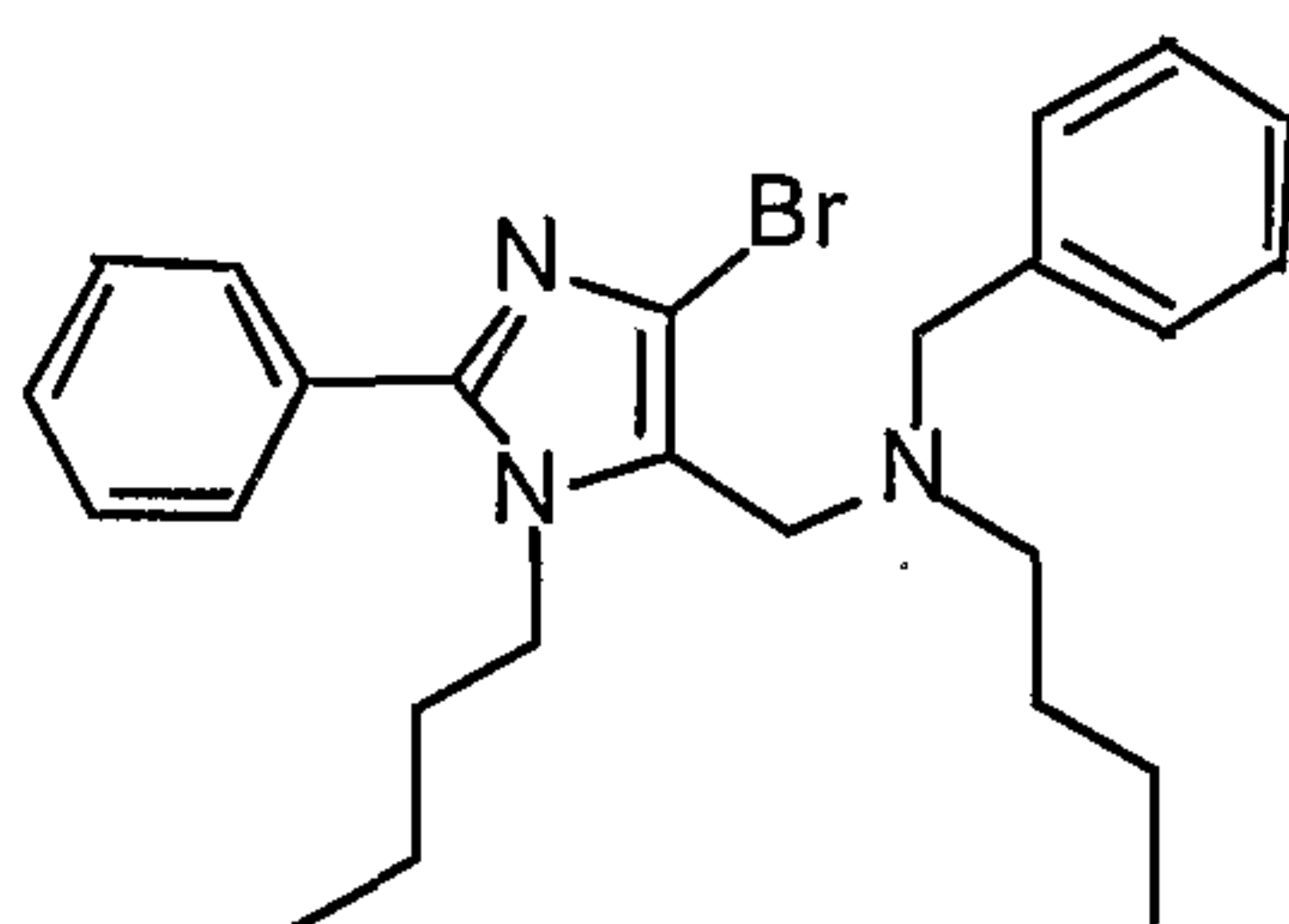
1-(1-Butyl)-2-phenyl-4-bromo-5-(N-phenylmethyl-N-[1-butyl])aminomethylimidazole;
