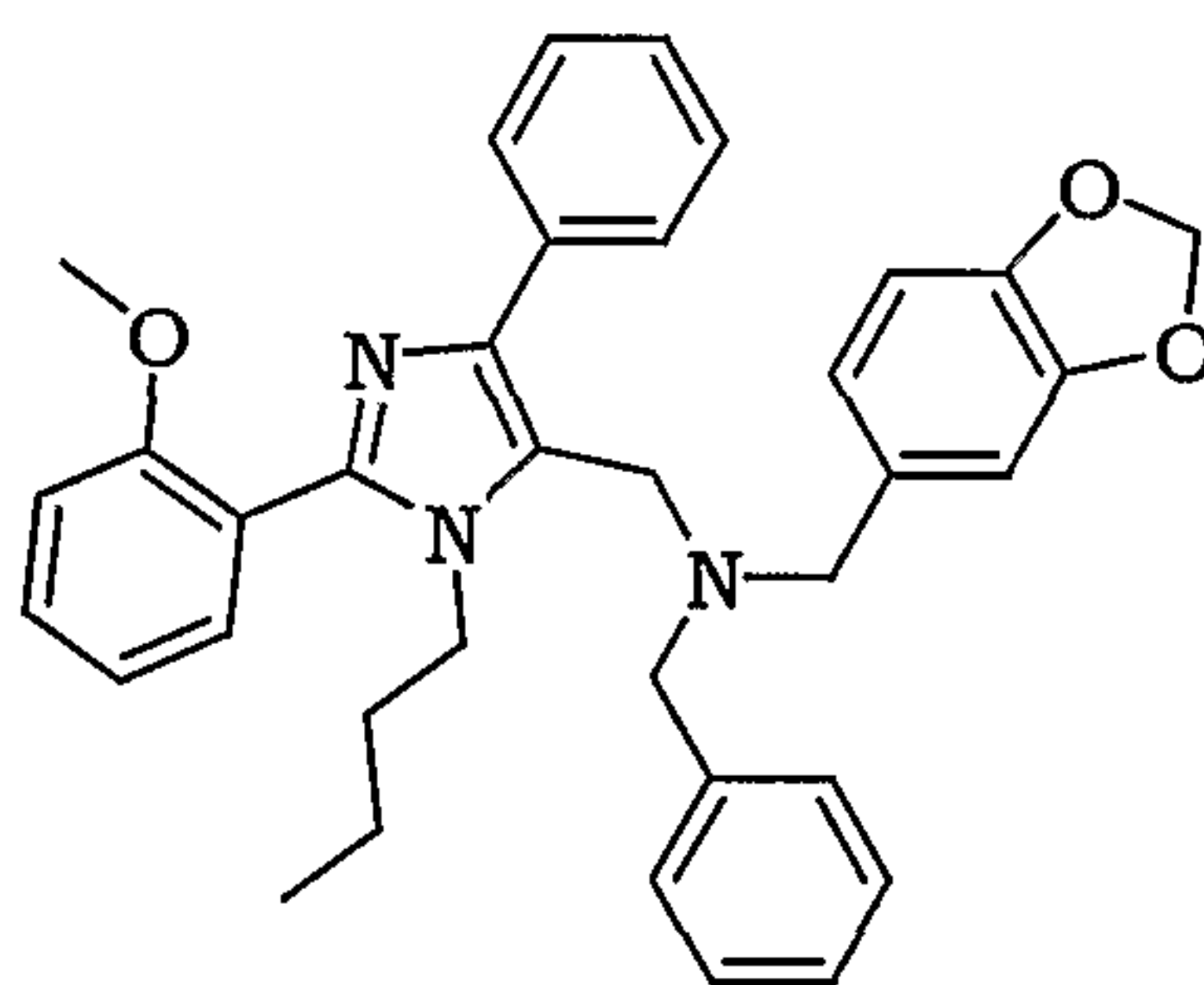
Benzo[1,3]dioxol-5-ylmethyl-benzyl-[3-butyl-2-(2-methoxy-phenyl)-5-phenyl-3 H -imidazol-4-yl methyl]-amine
