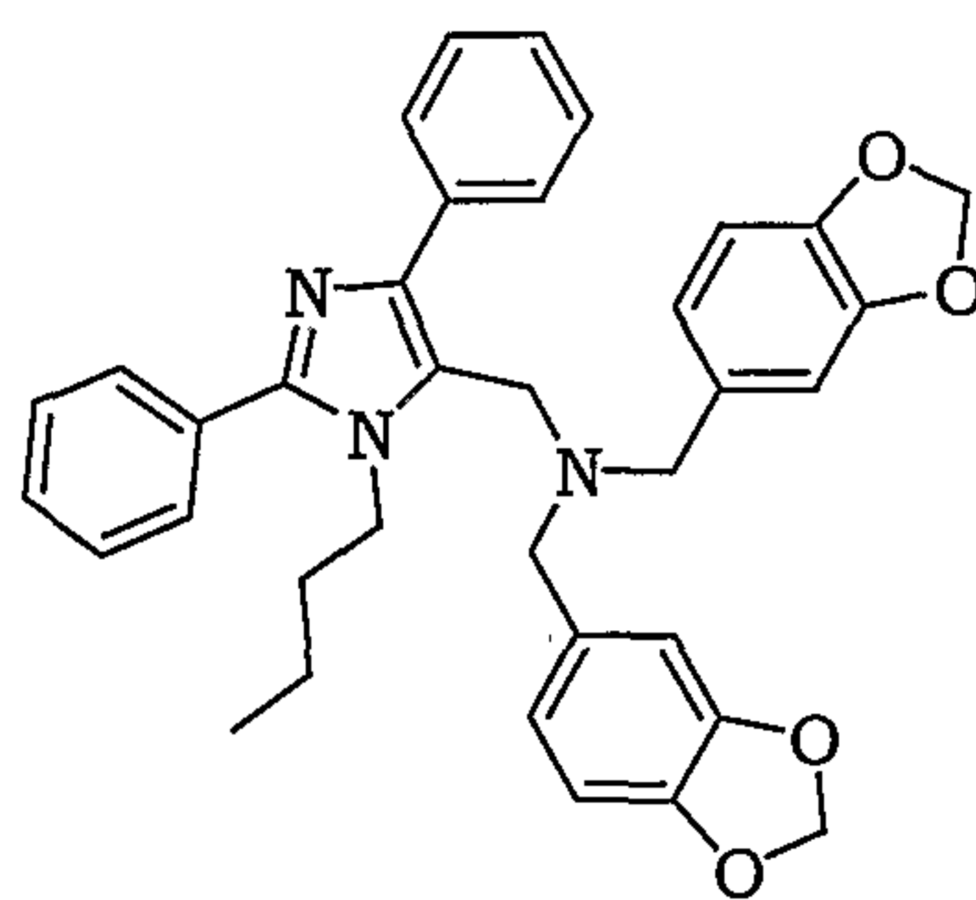
Bis-benzo[1,3]dioxol-5-ylmethyl-(3-butyl-2,5-diphenyl-3 H -imidazol-4-ylmethyl)-amine
