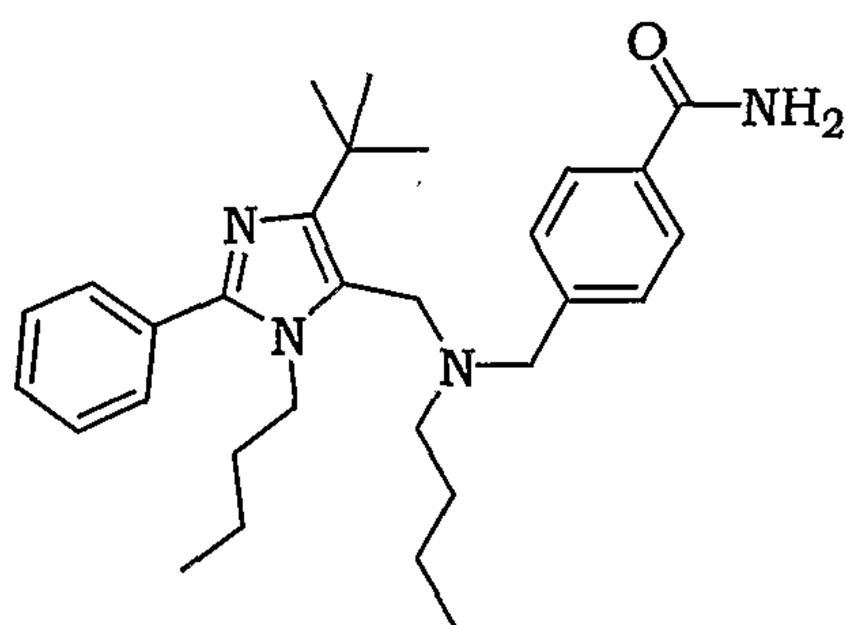
4-[[Butyl-(3-butyl-5- tert -butyl-2-phenyl-3 H -imidazol-4-ylmethyl)-amino]-methyl]-benzamide
