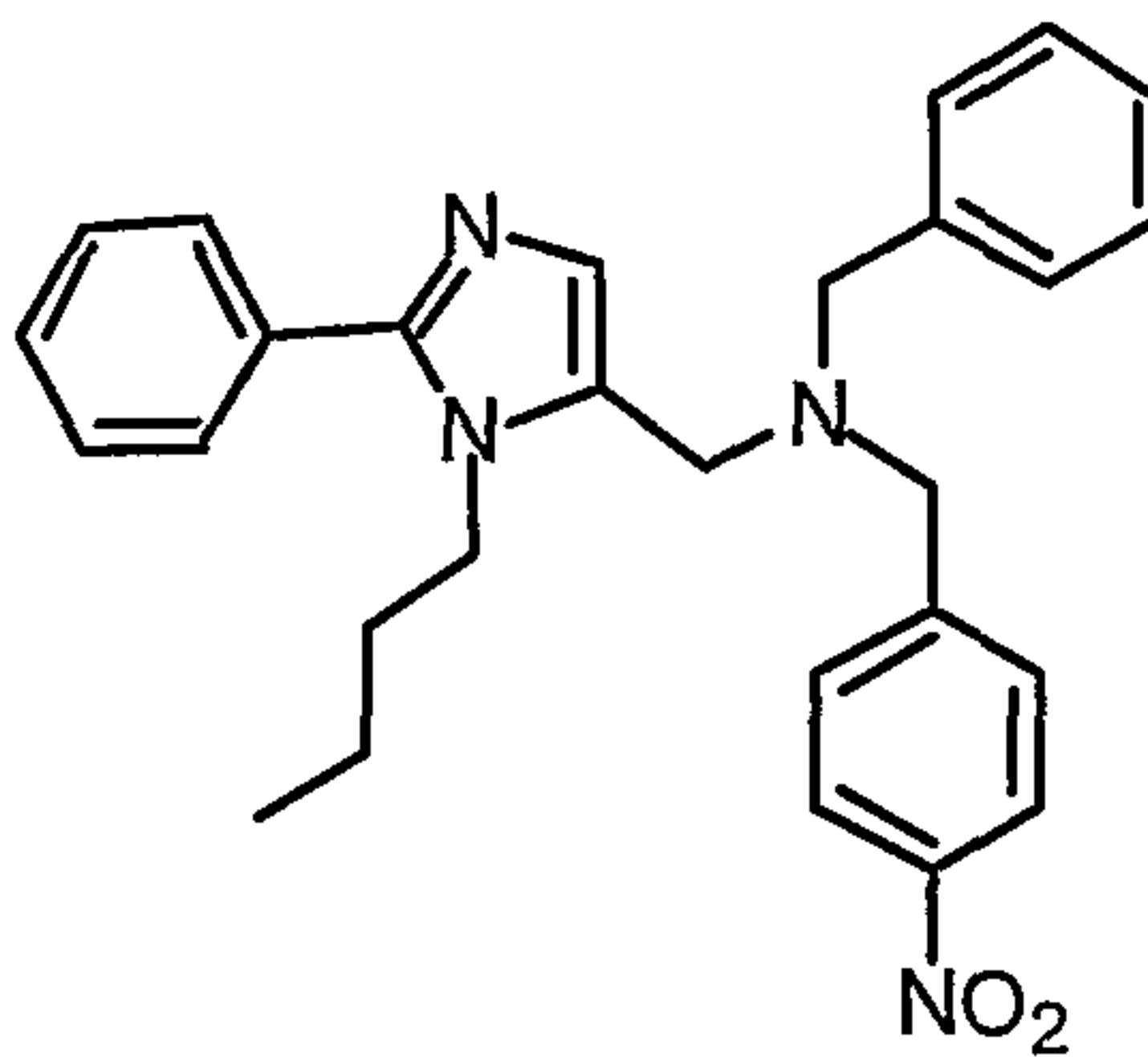
1-(1-Butyl)-2-phenyl-5-(N-[4-nitrophenylmethyl]-N-phenylmethyl)aminomethylimidazole;
