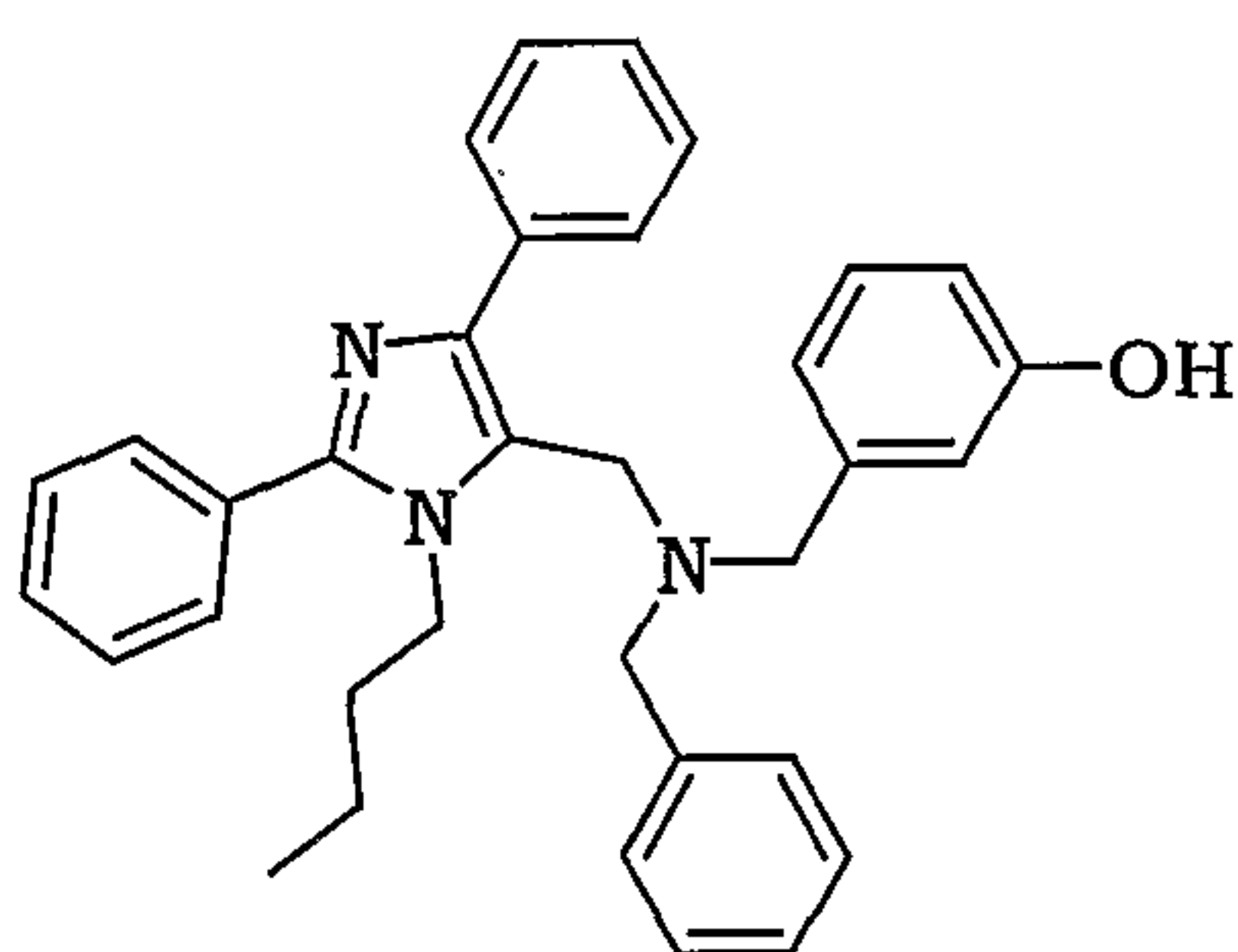
3-[[Benzyl-(3-butyl-2,5-diphenyl-3 H -imidazol-4-ylmethyl)-amino]-methyl]-phenol
