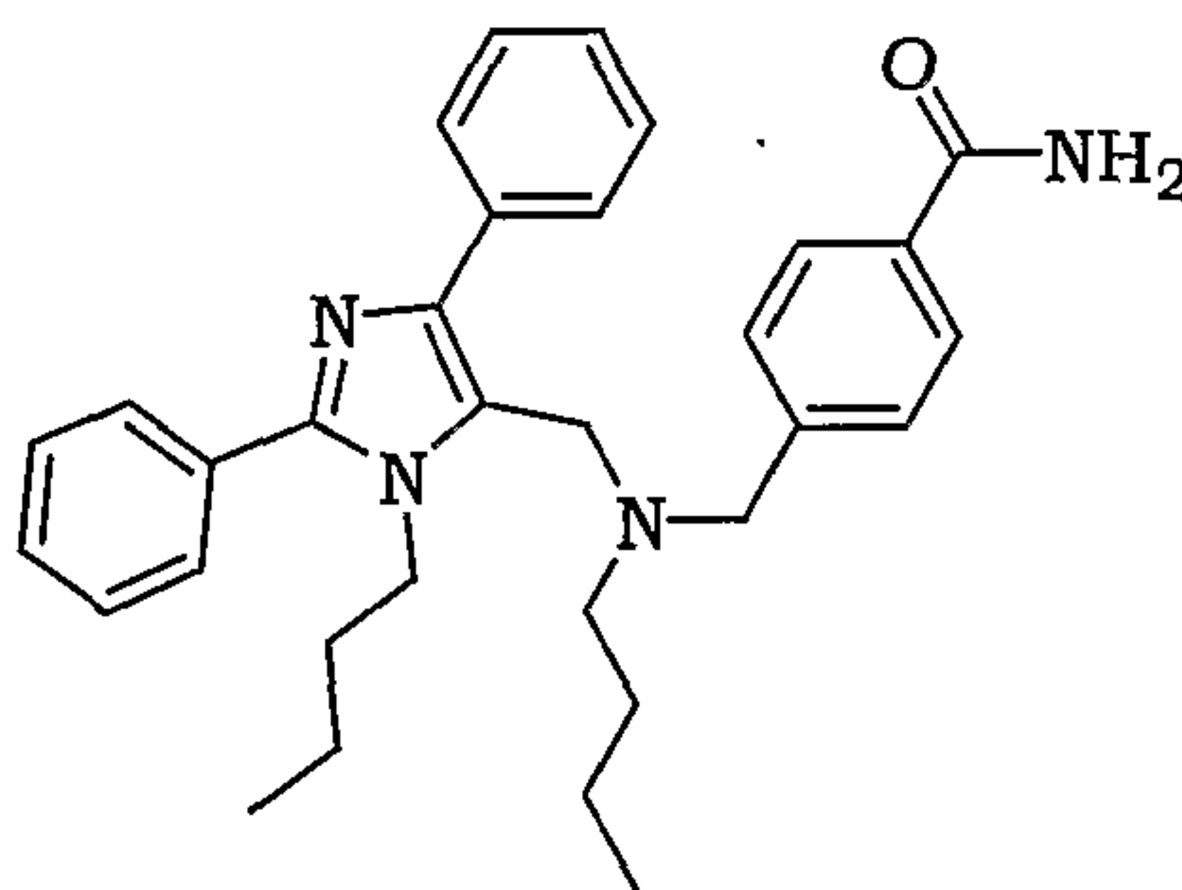
4-[[Butyl-(3-butyl-2,5-diphenyl-3 H -imidazol-4-ylmethyl)-amino]-methyl]-benzamide
