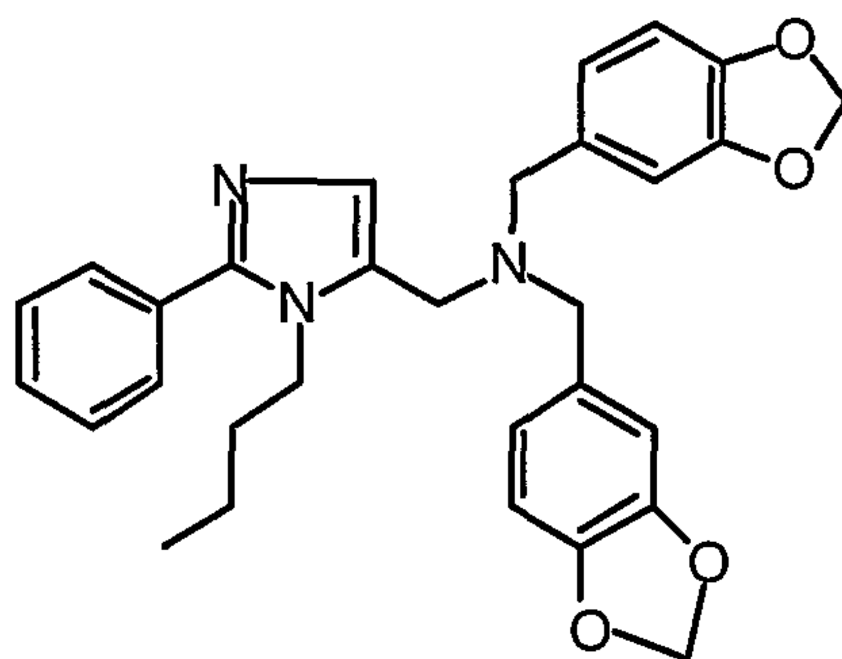
1-(1-Butyl)-2-phenyl-5-(N,N-di[3,4-methylenedioxyphenylmethyl]) aminomethylimidazole;
