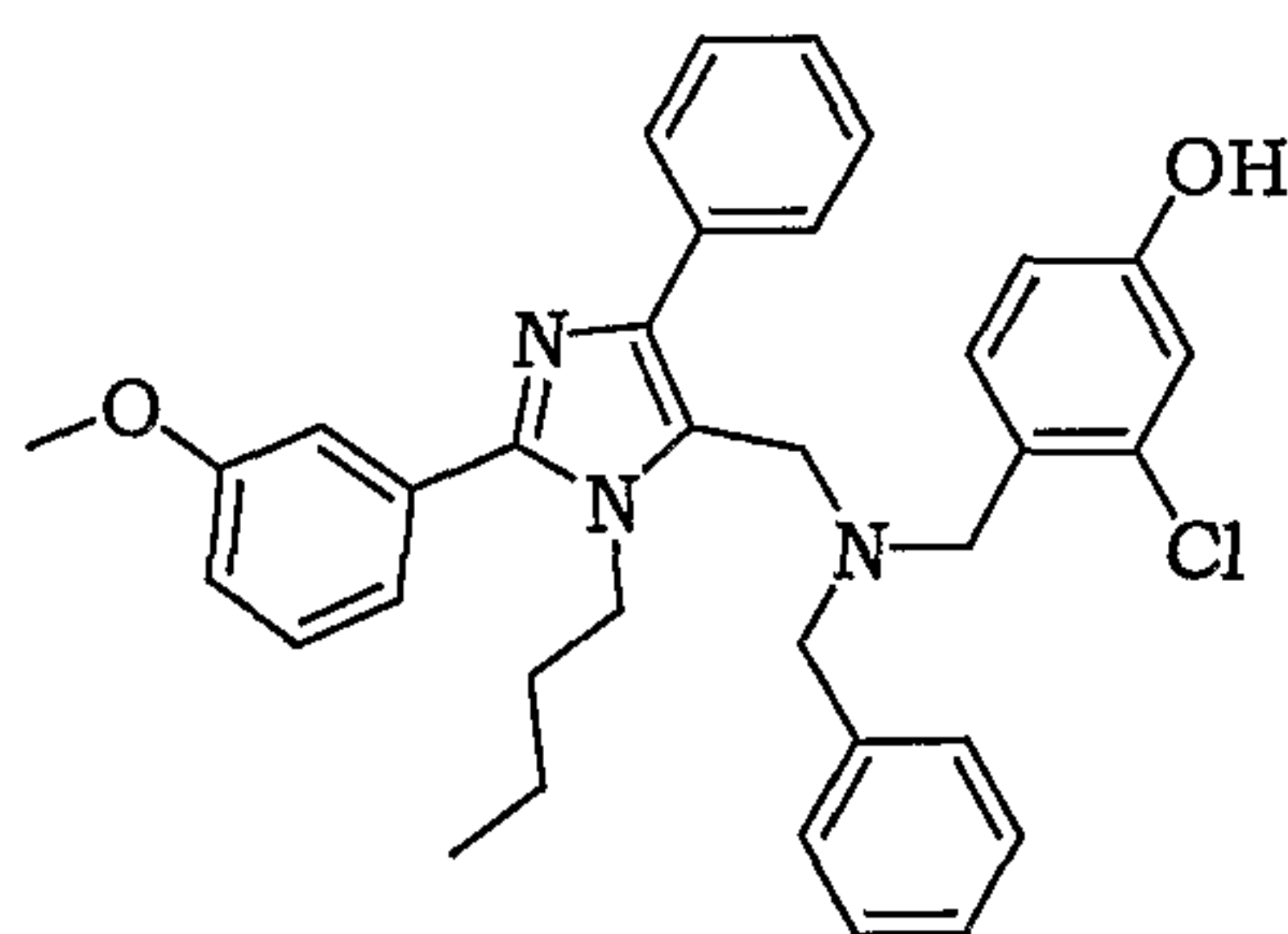
4-((benzyl-3-butyl-2-(3-methoxy-phenyl)-5-phenyl-3 H -imidazol-4-ylmethyl)-amino)-methyl-3-chlorophenol
