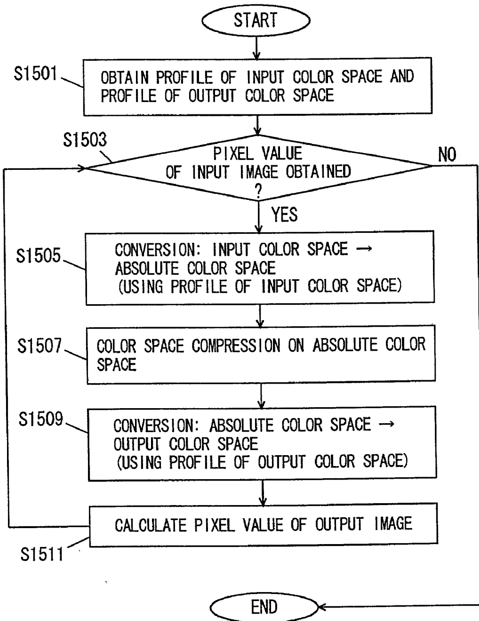
FIG. 15 PRIOR ART
