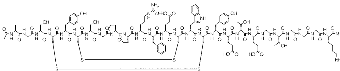
Peptide 1
