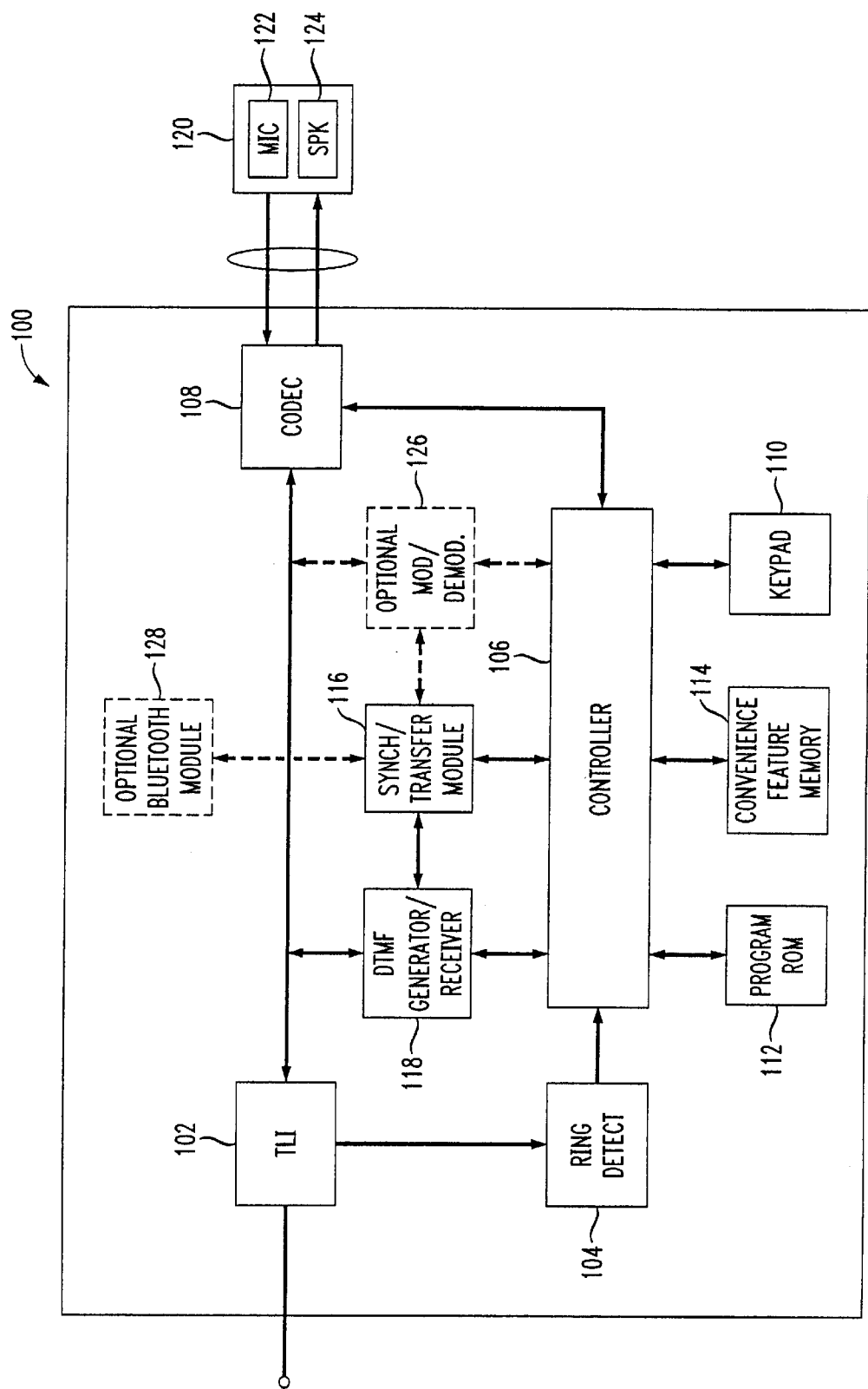
FIG. 2 CORDED TELEPHONE
