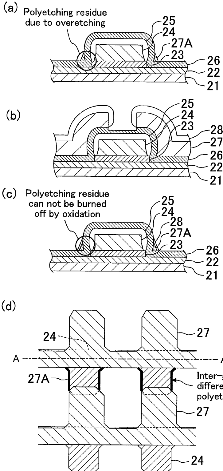
FIG. 18 PRIOR ART
