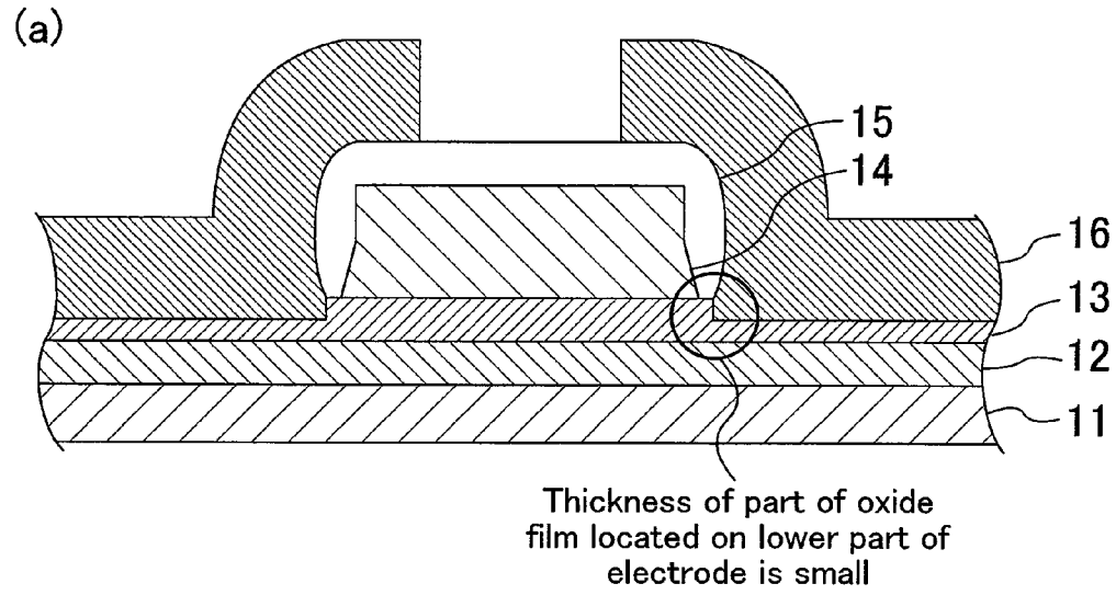
FIG. 16 PRIOR ART
