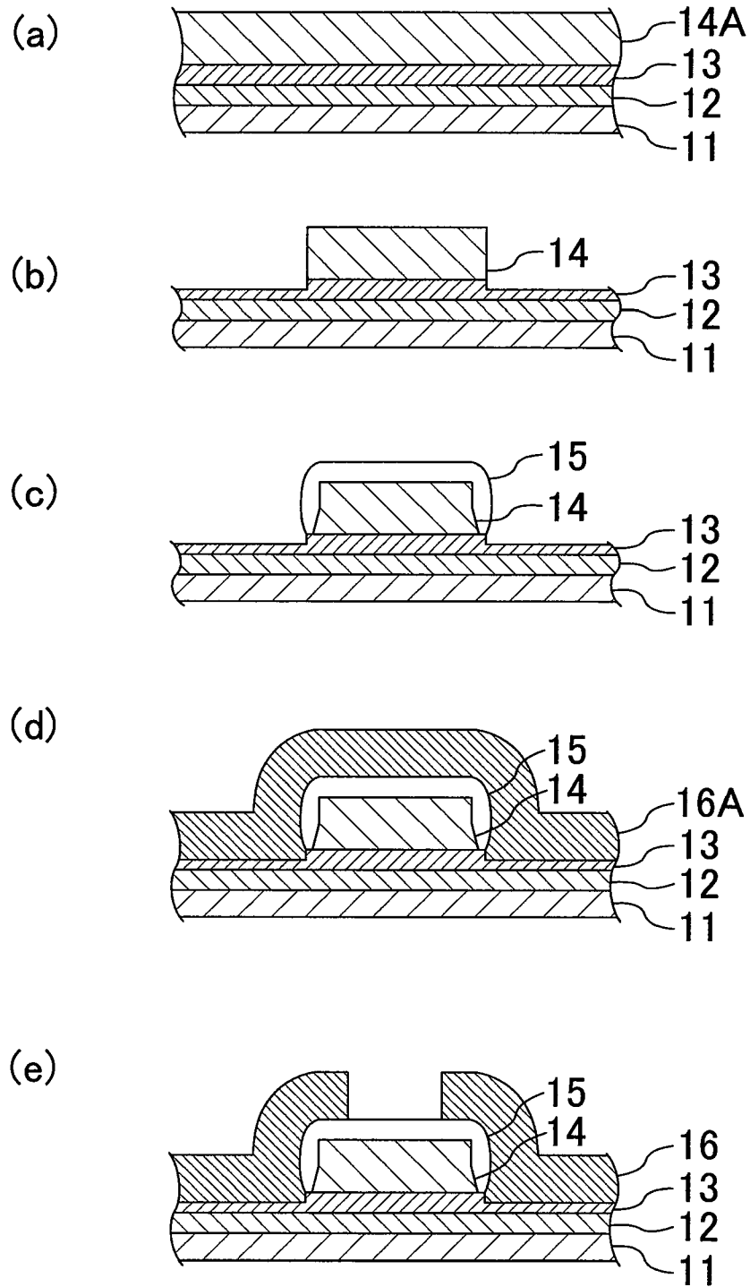
FIG. 15 PRIOR ART
