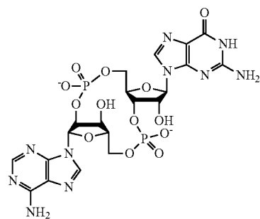
3',2'-cGAMP 5% yield from S2
