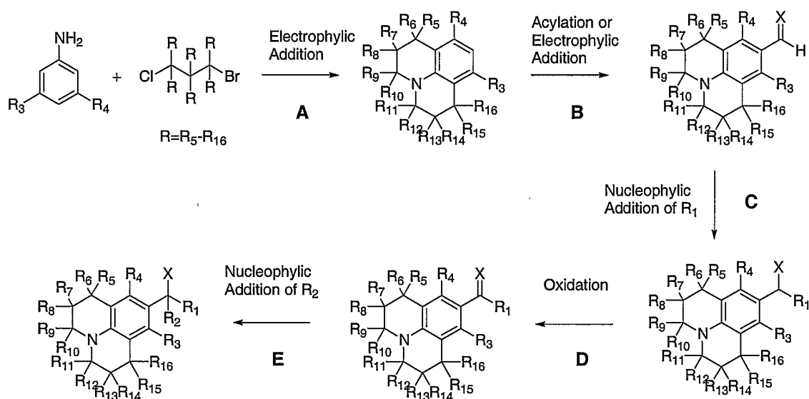
Figure:1 Julolidine Synthesis
