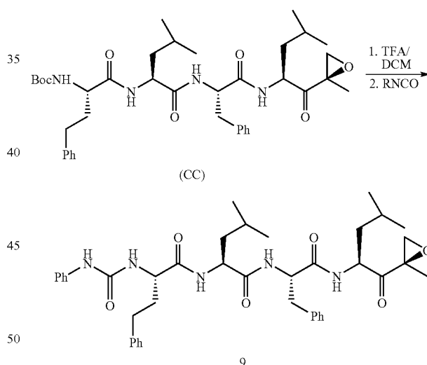
Scheme 9: Synthesis of Example 9
