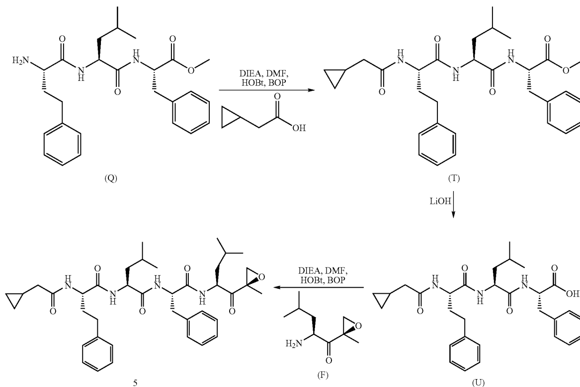
Scheme 5: Synthesis of Example 5
