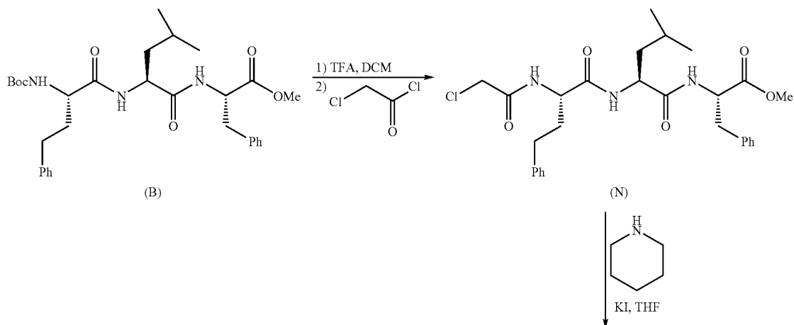
Scheme 4: Synthesis of Example 4
