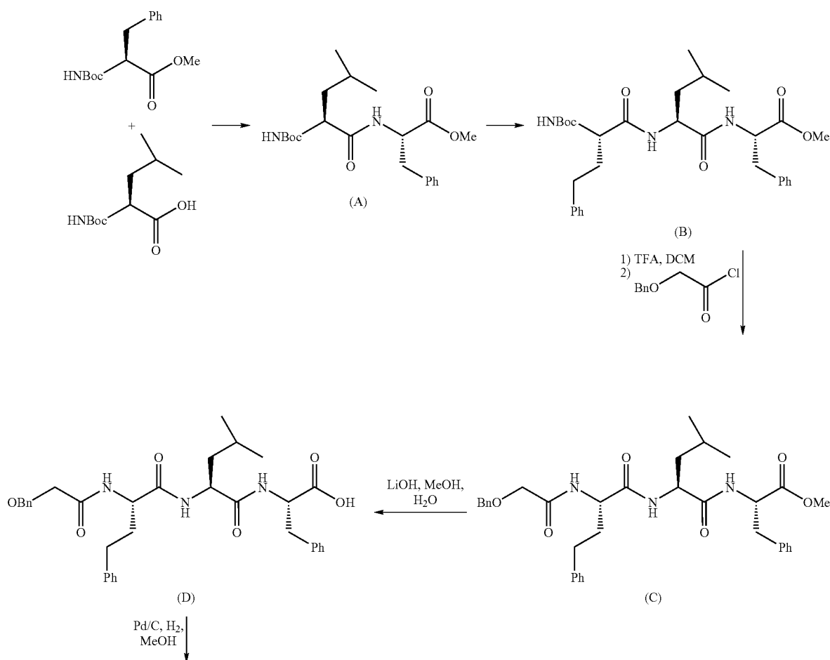
Scheme 1: Synthesis of Example 1
