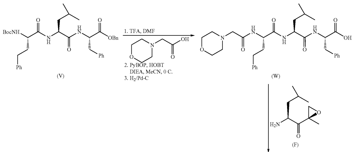
Scheme 6: synthesis of Example 6
