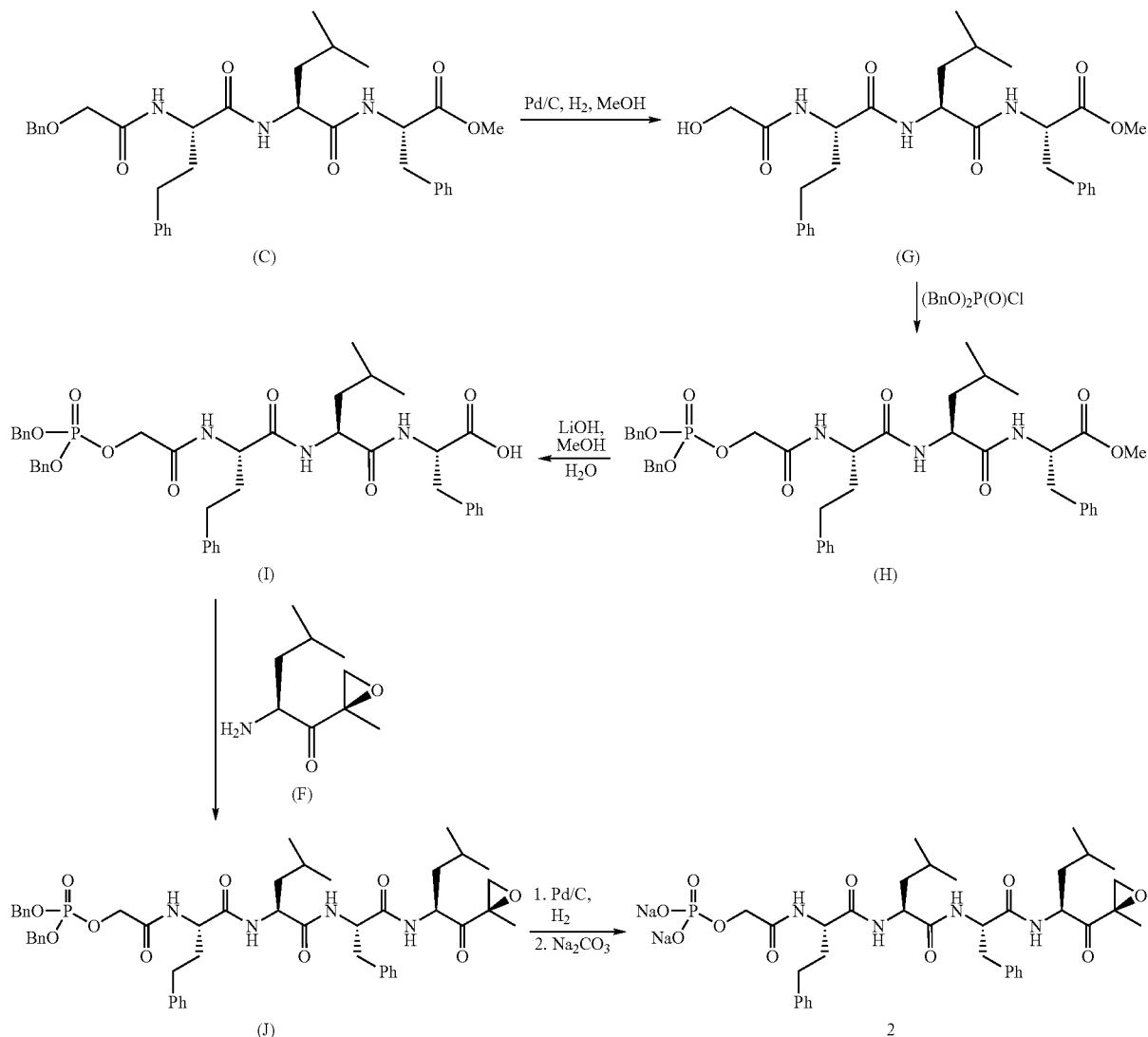
Scheme 2: Synthesis of Example 2
