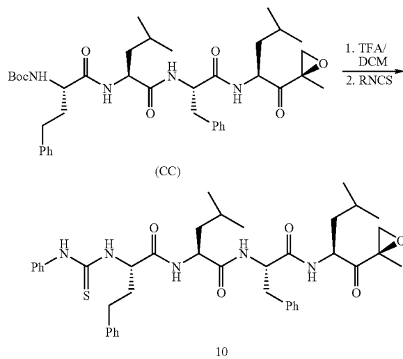
Scheme 10: Synthesis of Example 10
