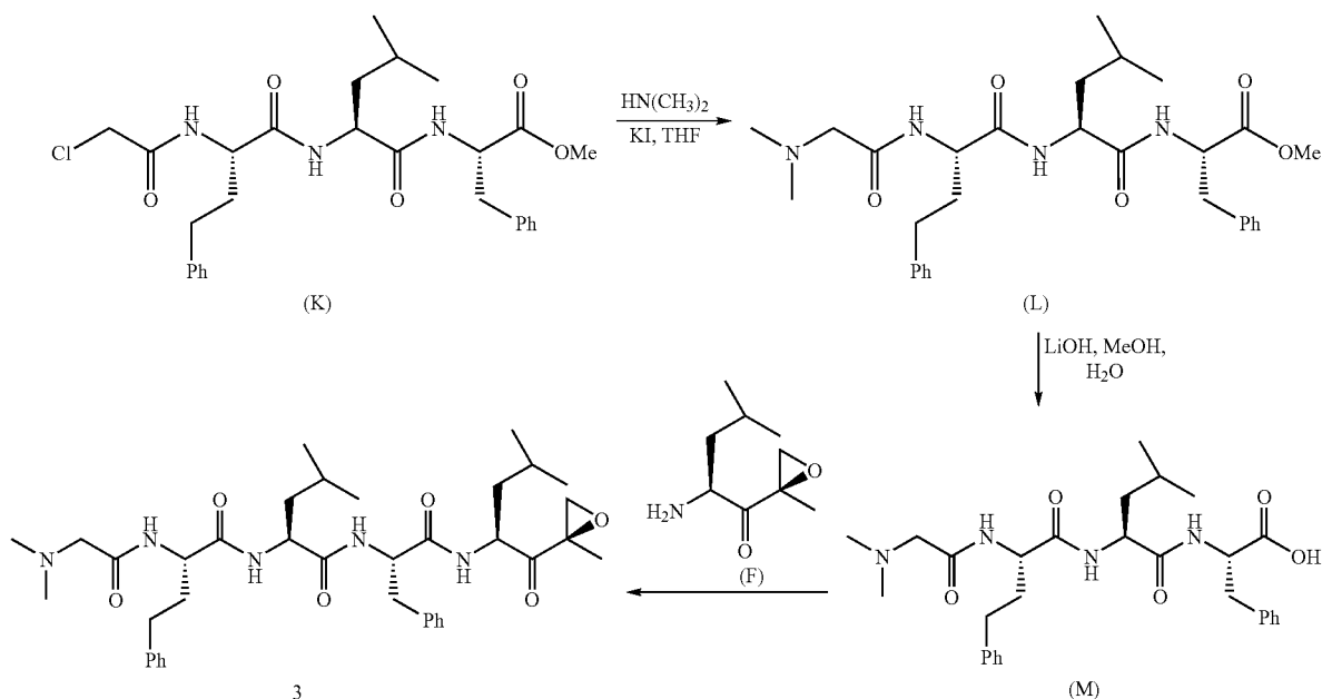
Scheme 3: Synthesis of Example 3
