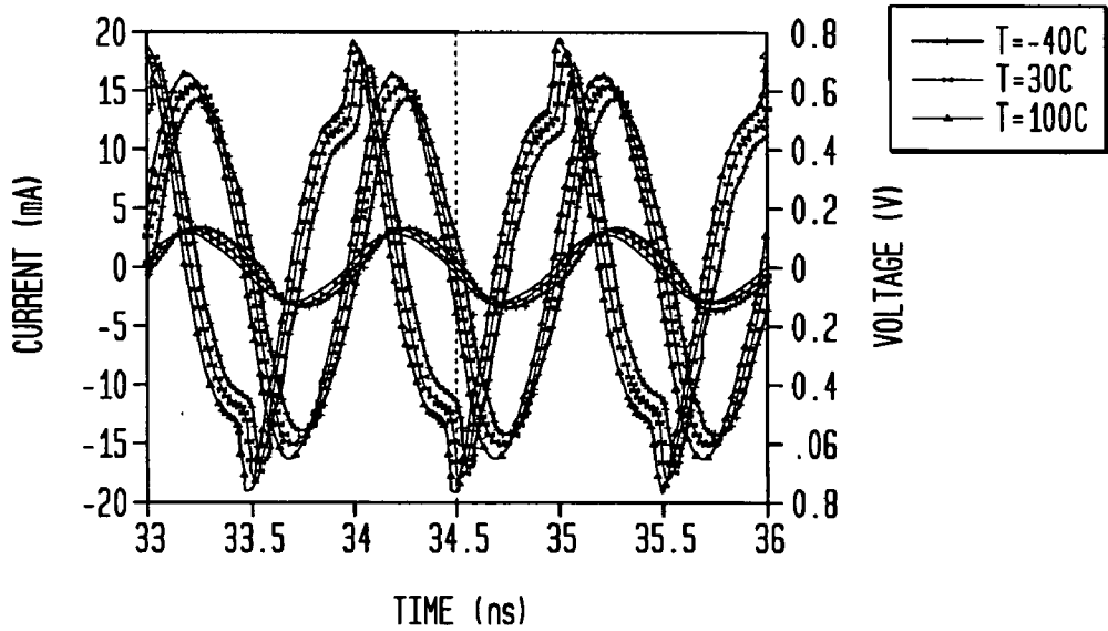
TEMPERATURE/BIAS DEPENDENCE
