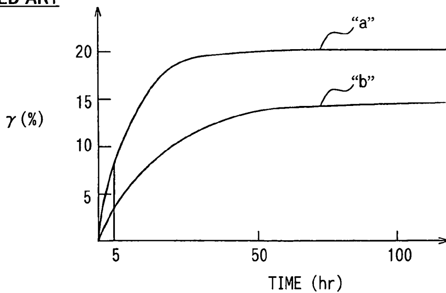
FIG. 6 RELATED ART
