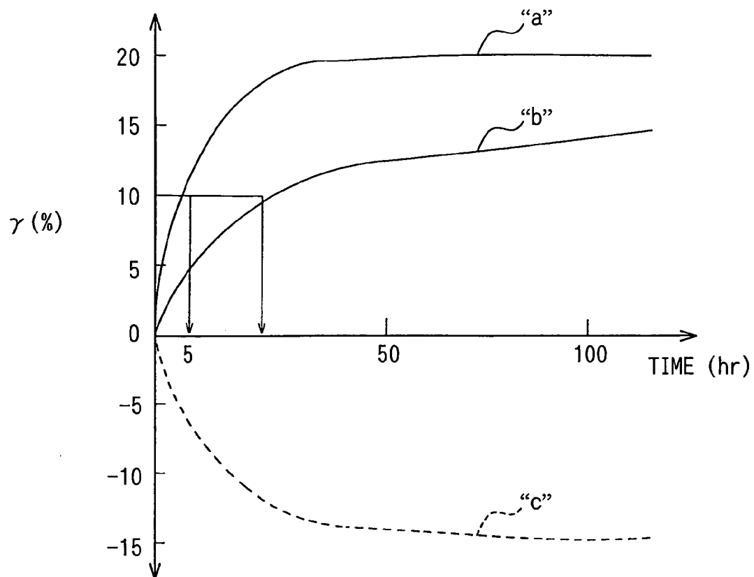
FIG. 6 RELATED ART
