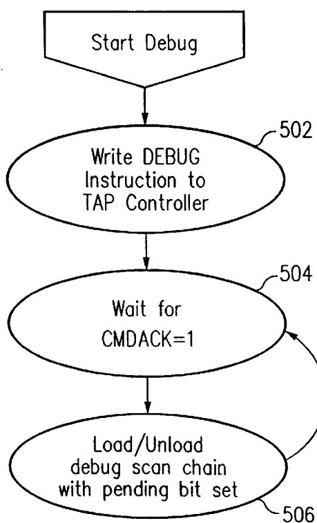
Enhanced JTAG interface access state diagram
