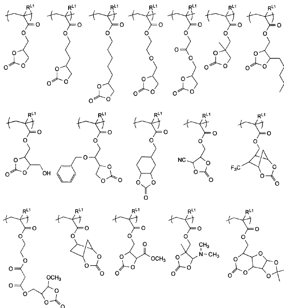
[Chem.8]
