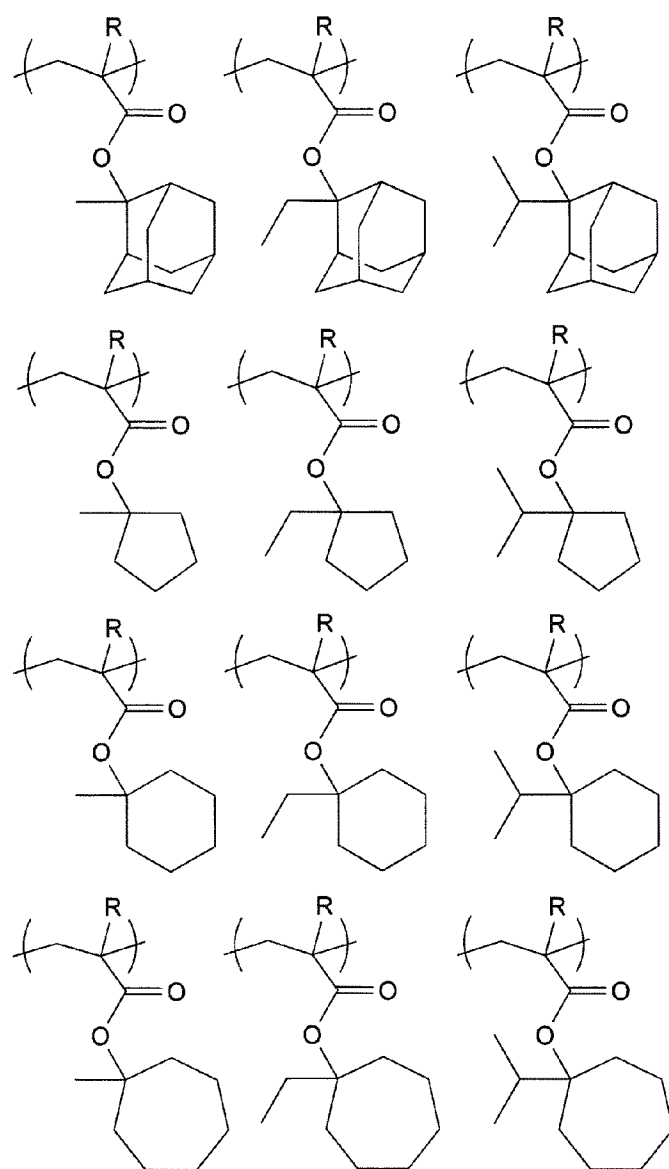
[Chem.4]
