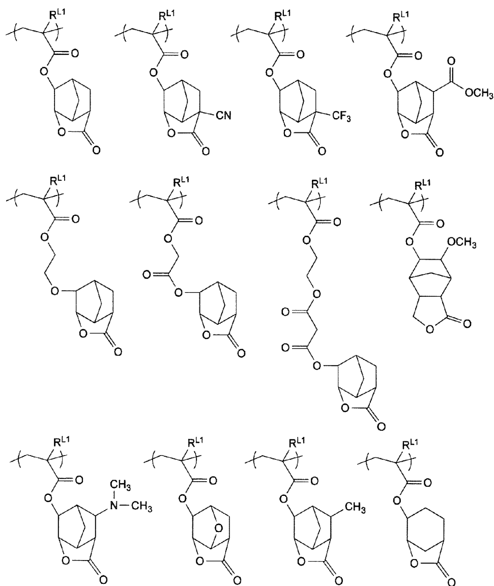
[Chem.6]
