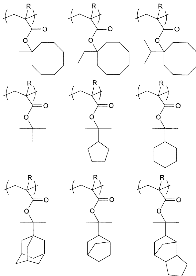
[Chem.5]
