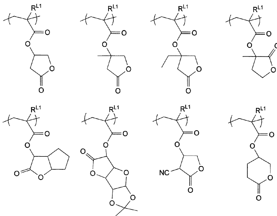
[Chem.7]
