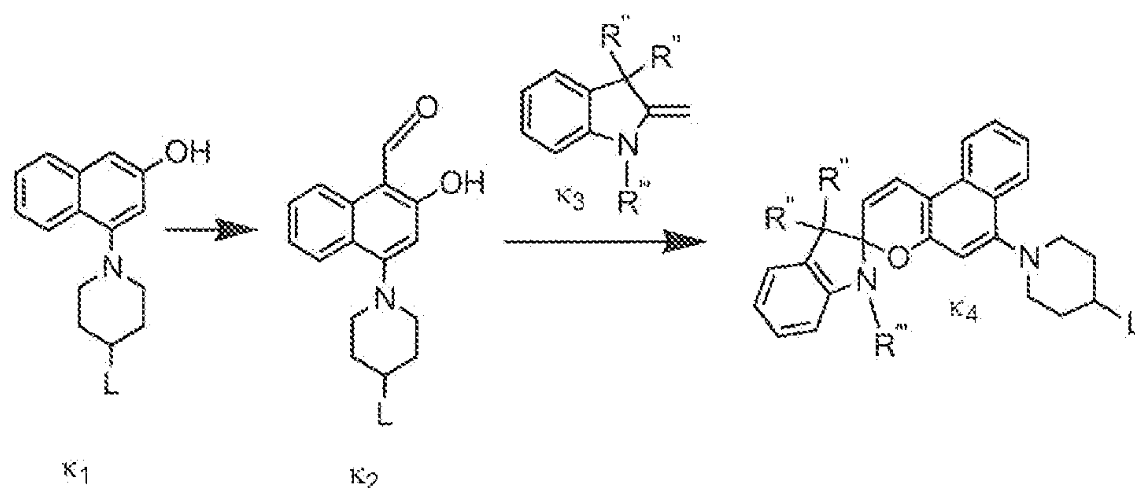
Reaction Sequence K
