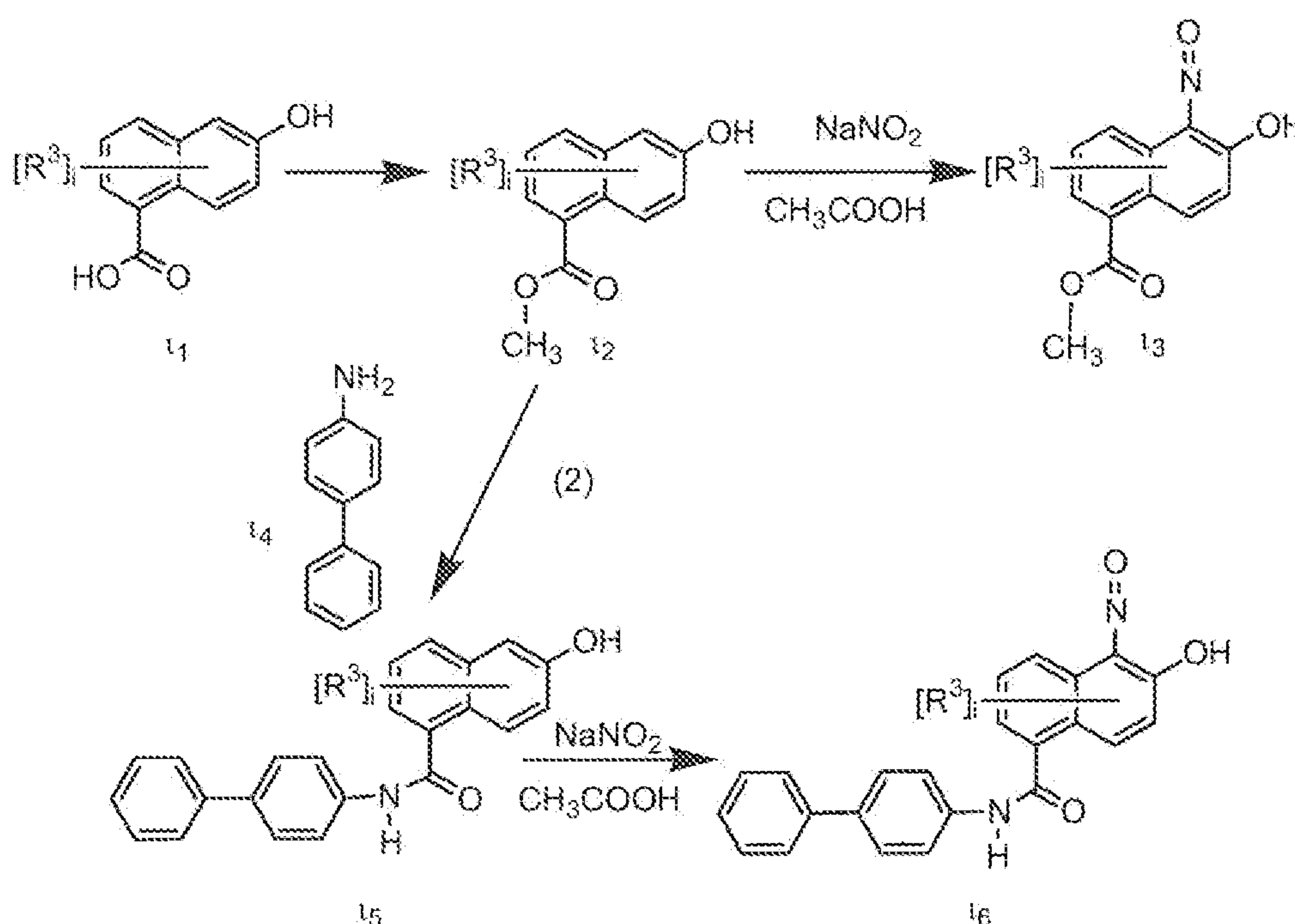
Reaction Sequence I
