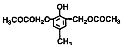
2,6-diacetoxymethyl-p-cresol
