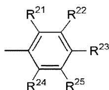
General Formula (2)
