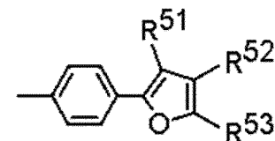
General Formula (5)
