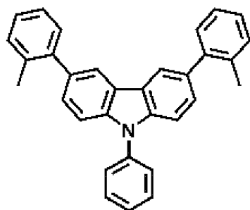
CBZ
