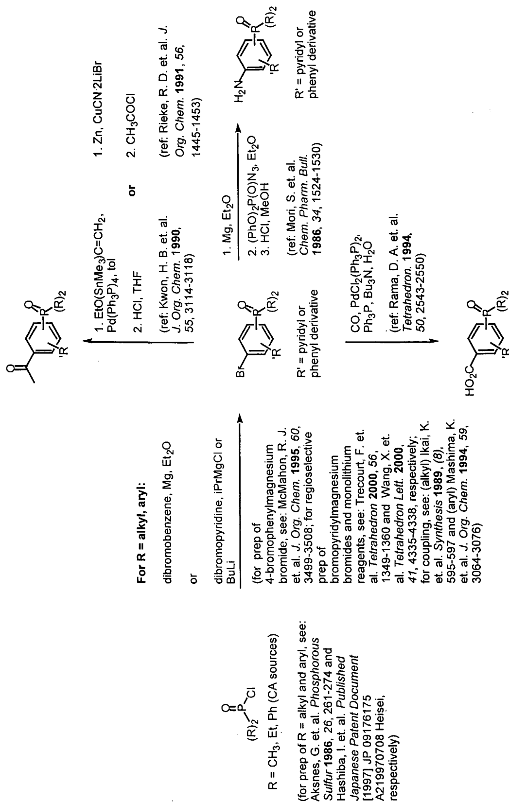
Scheme 2
