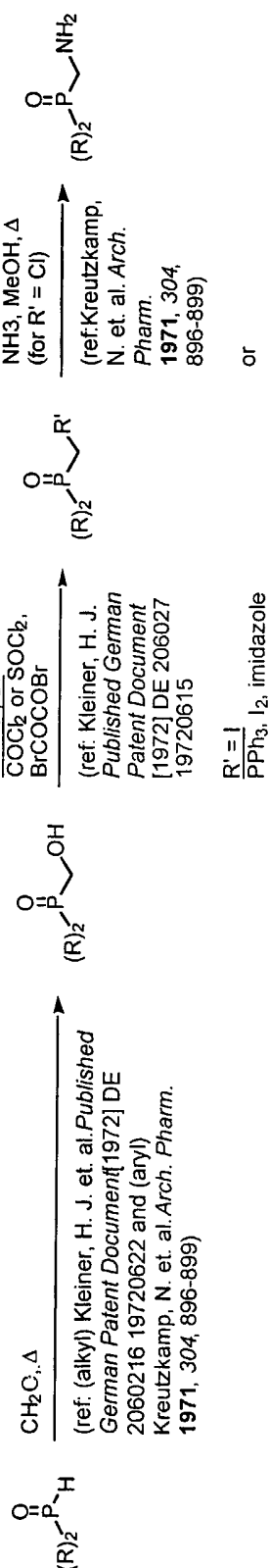
Scheme 1
