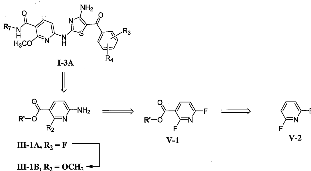
Scheme V
