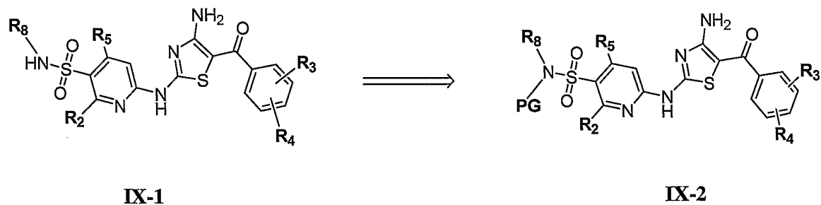
Scheme IX
