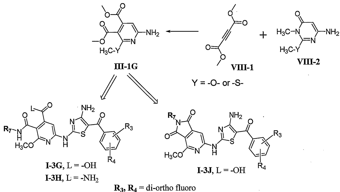
Scheme VIII
