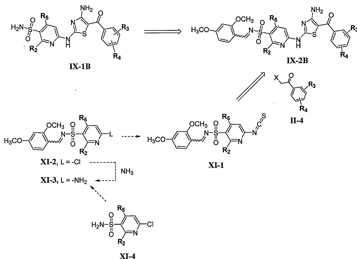
Scheme XI
