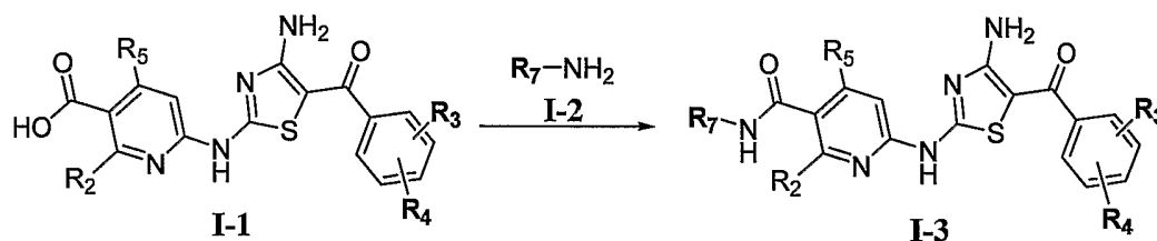
Scheme I
