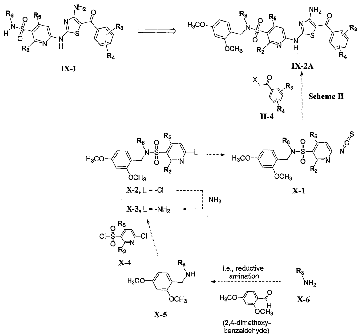
Scheme X
