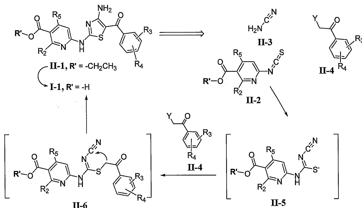
Scheme II
