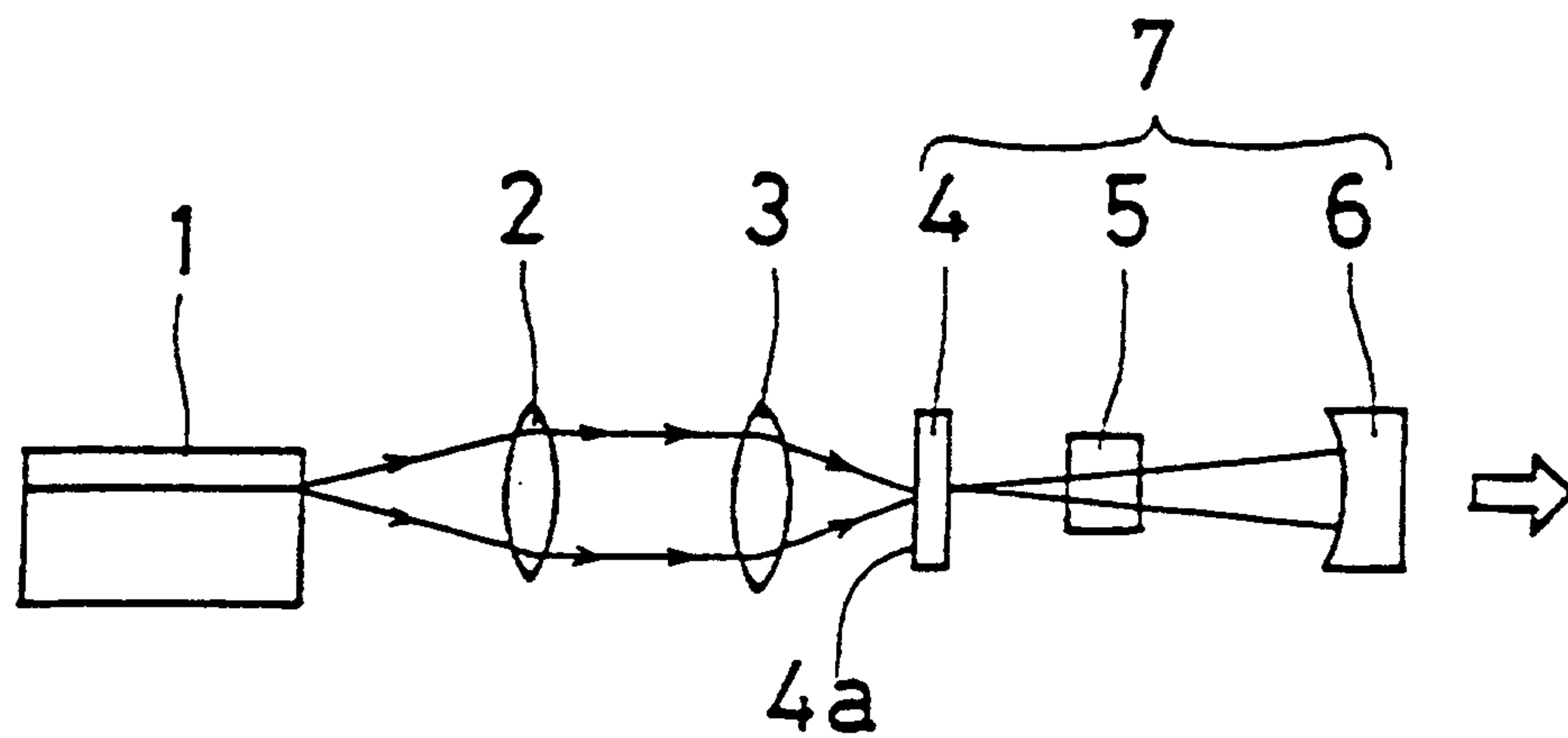
FIG. 25 PRIOR ART
