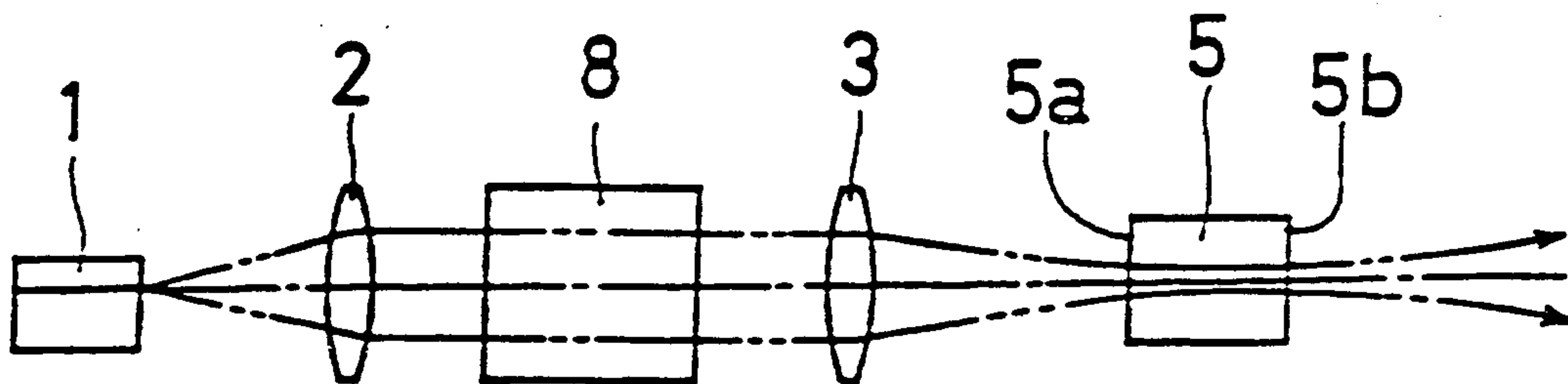
FIG. 27 PRIOR ART
