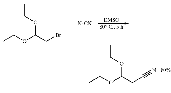
Scheme 3-Synthesis of cyanoacetaldehyde diethyl acetal using cyanide.
