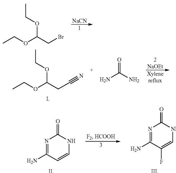
Scheme 2-Inventors proposed synthesis of flucytosine
