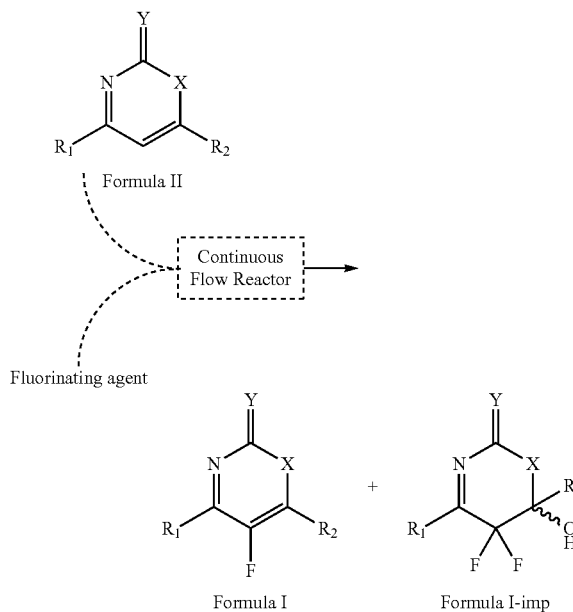
Scheme 1—Reaction to form compound of Formula I and impurity of Formula I-imp
