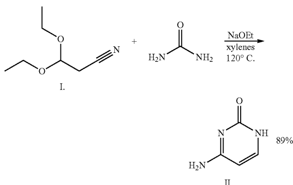
Scheme 4-Synthesis of cytosine from cyanoacetaldehyde and urea
