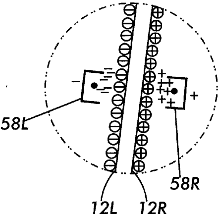
FIG. 5 (PRIOR ART)
