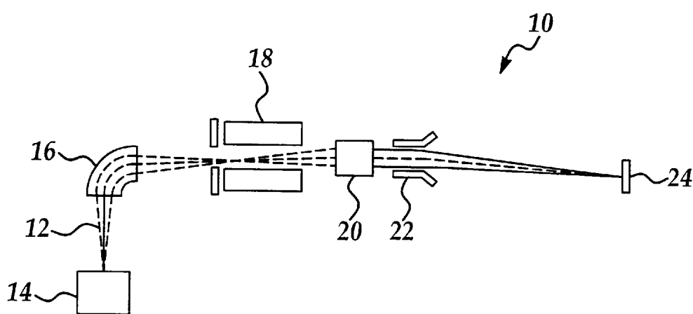
Figure 1 Prior Art
