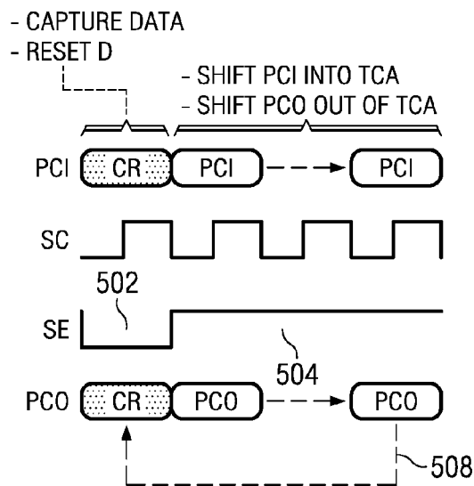
FIG. 5 (PRIOR ART)
