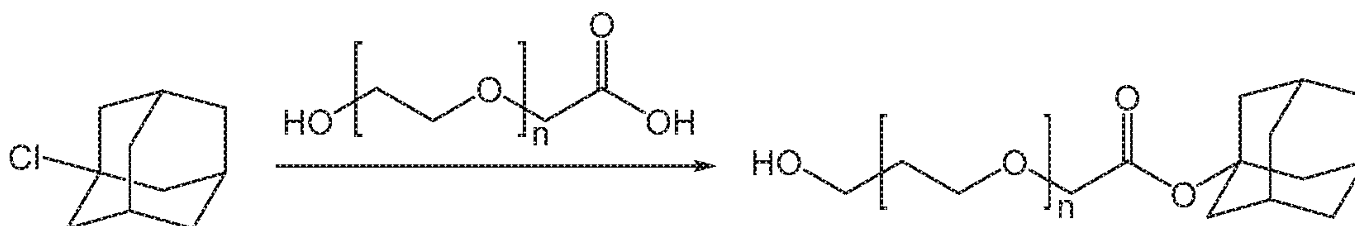
Scheme 10
