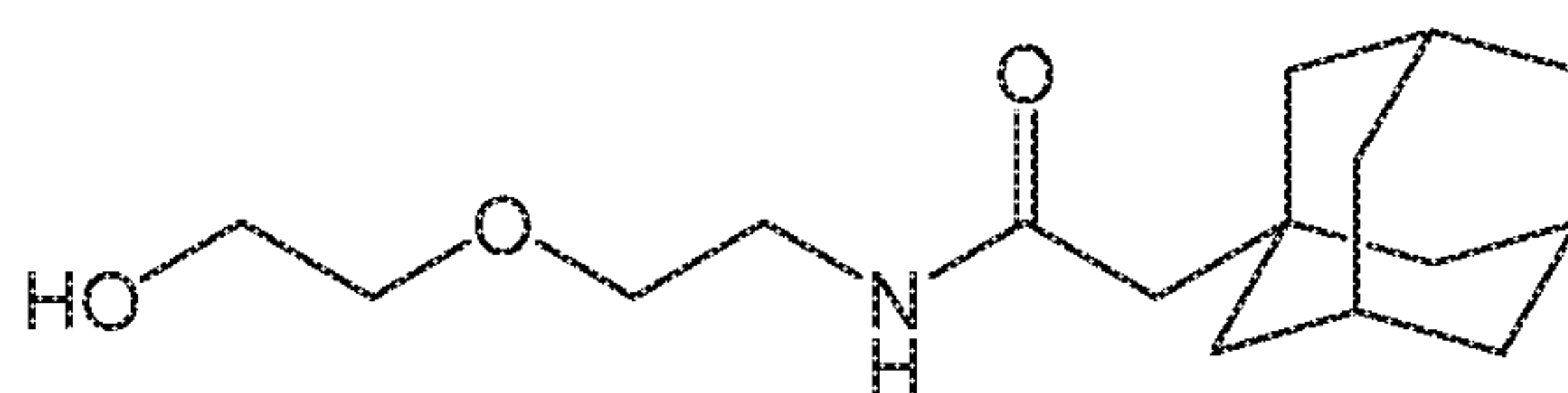
Compound 2
