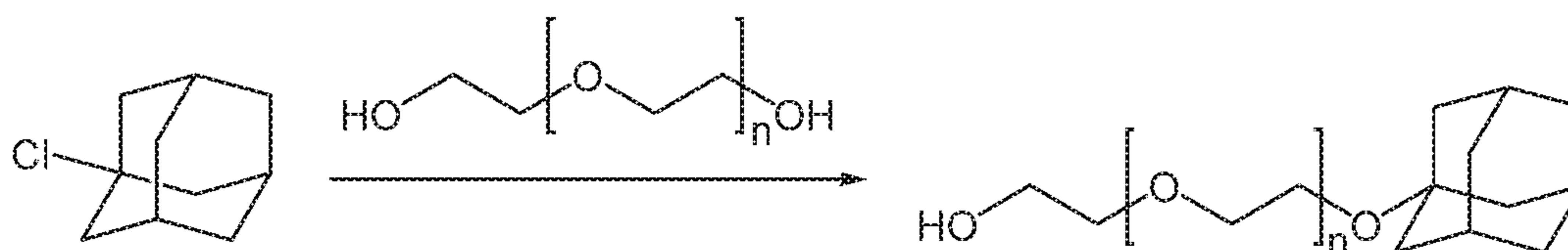
Scheme 5
