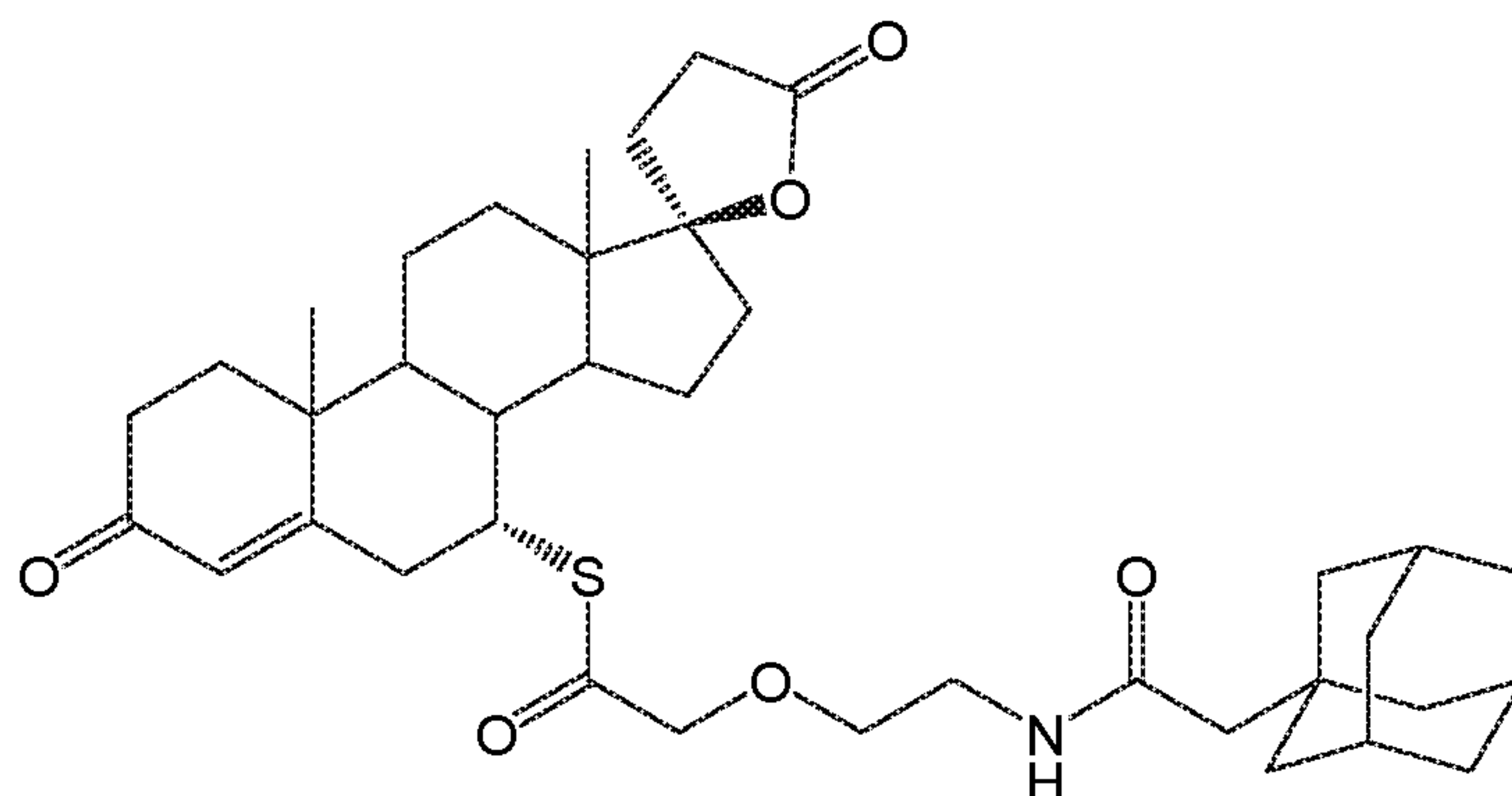
Compound 38
