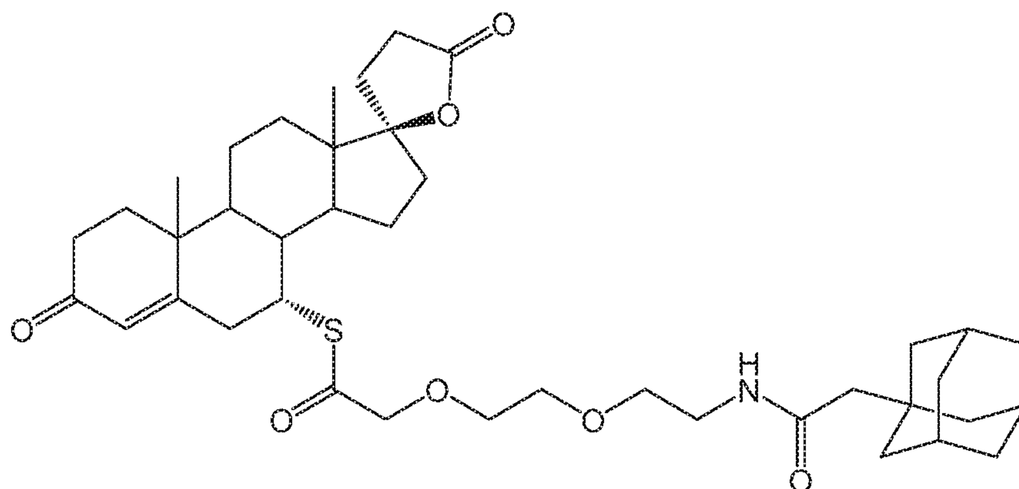
Compound 39
