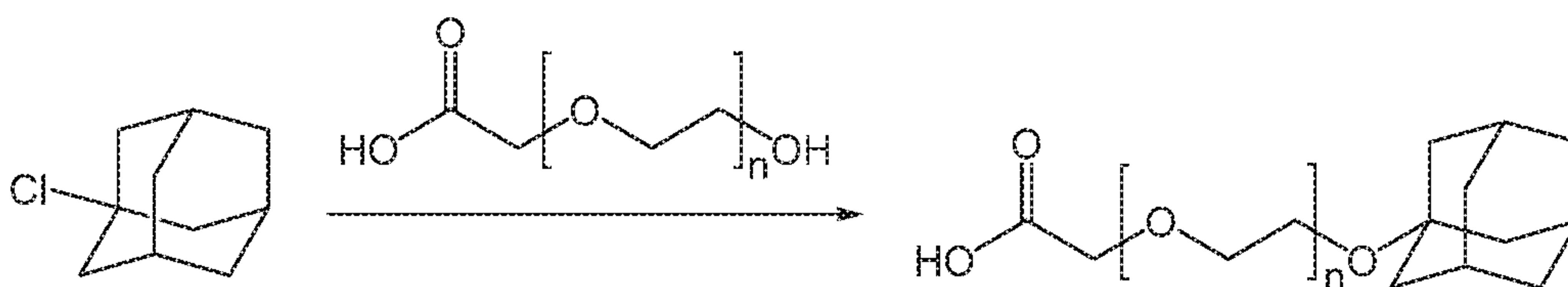
Scheme 6
