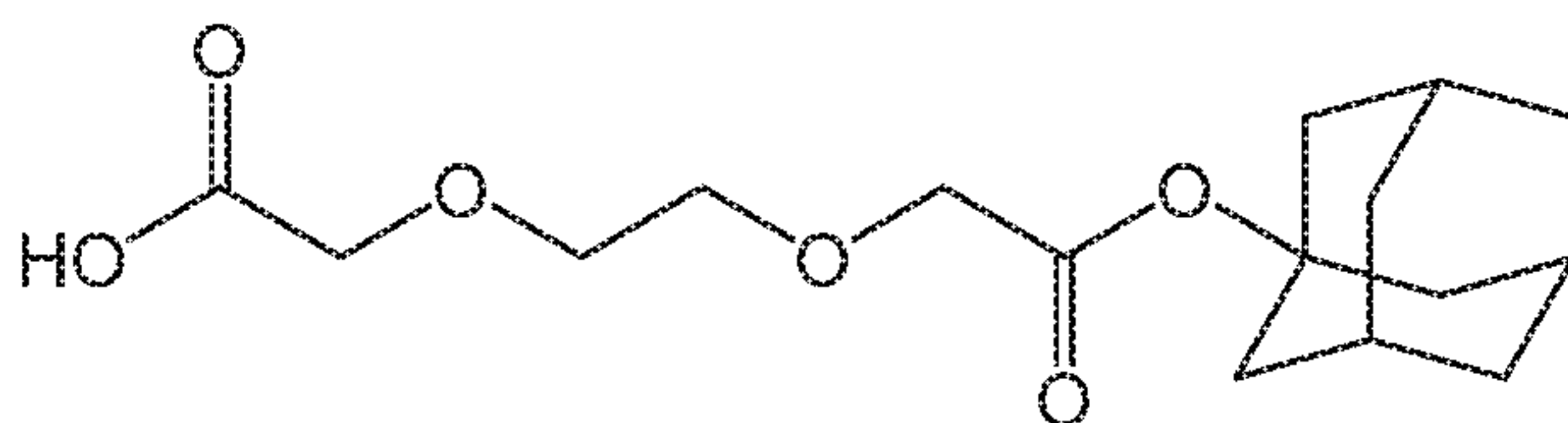
Compound 26
