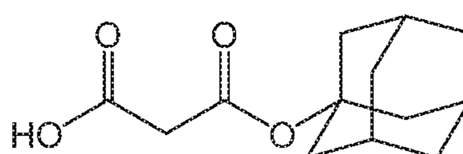
Compound 21
