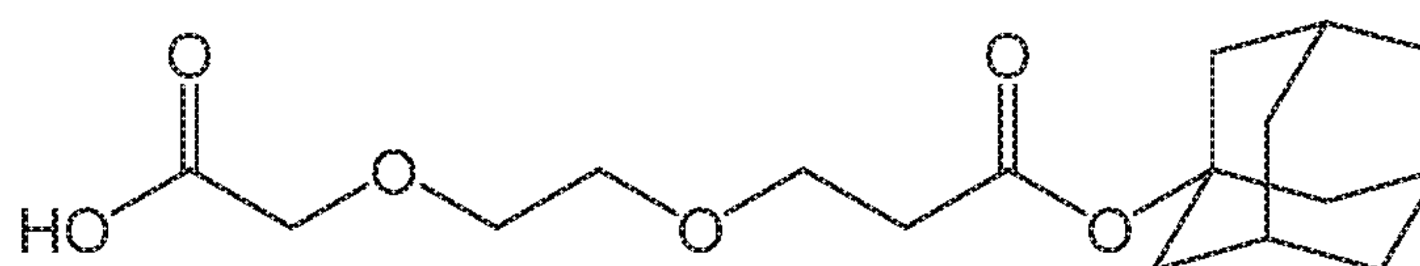
Compound 23
