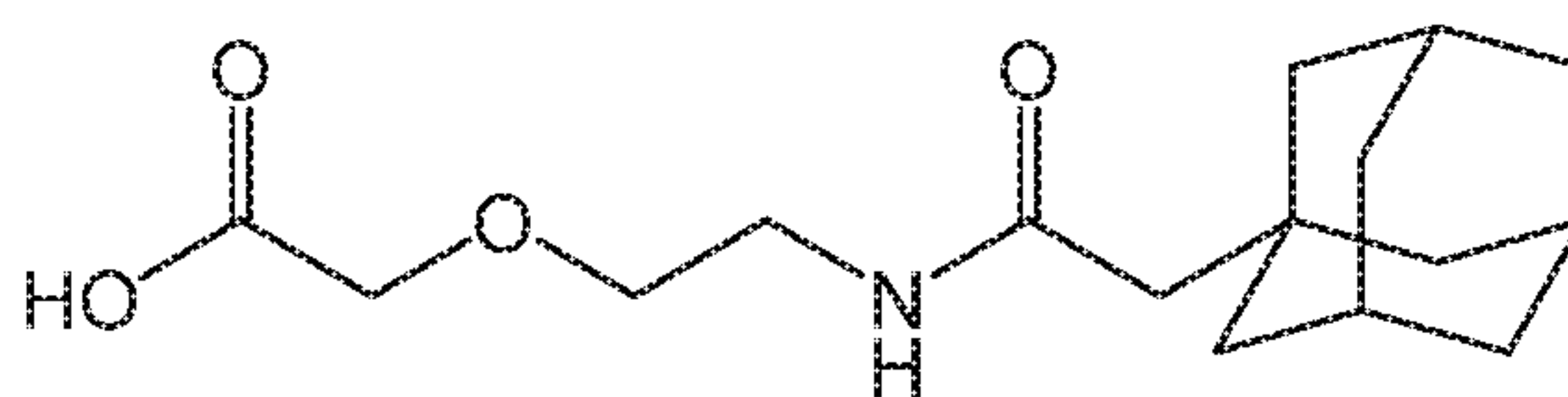
Compound 6
