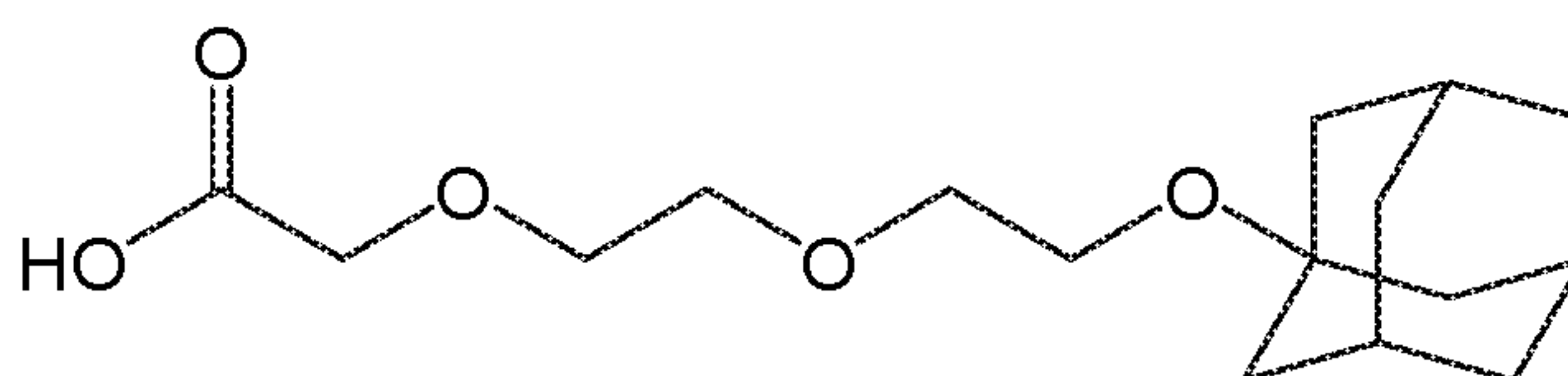
Compound 15
