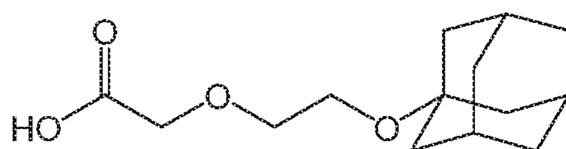
Compound 14
