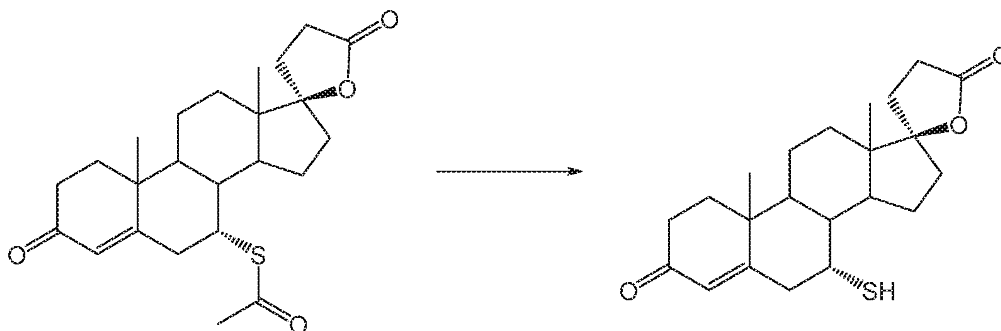
Scheme 12
