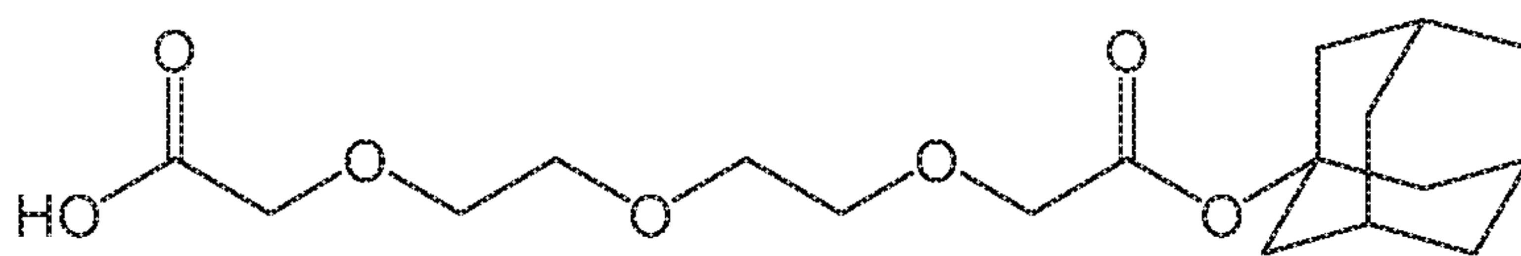
Compound 27
