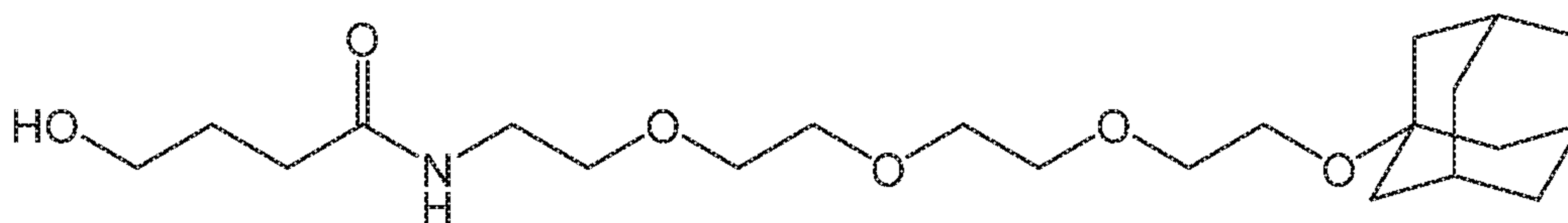
Compound 20
