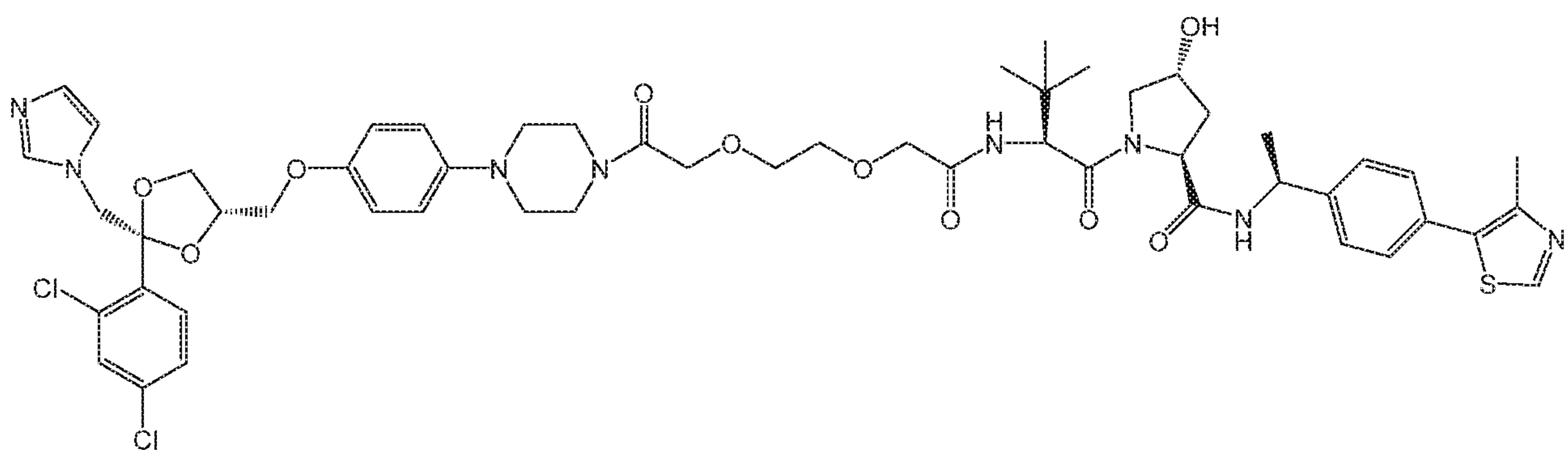
Compound 48
