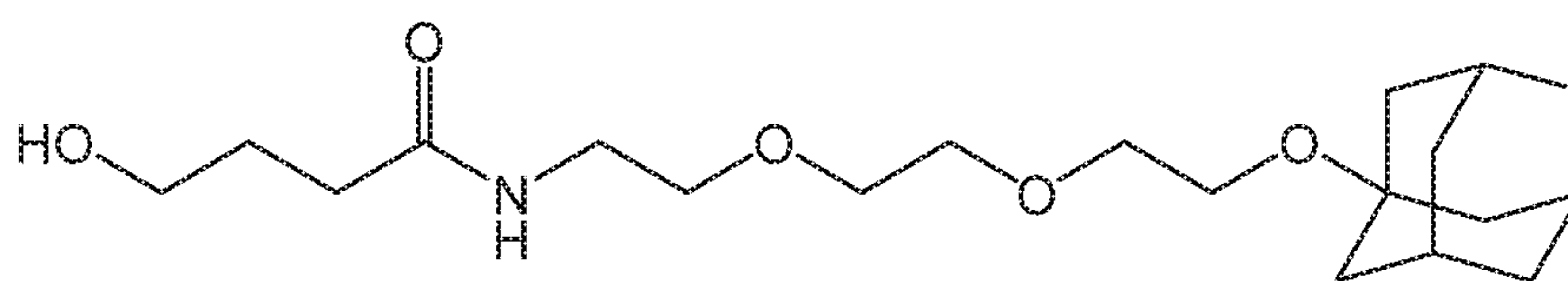
Compound 19
