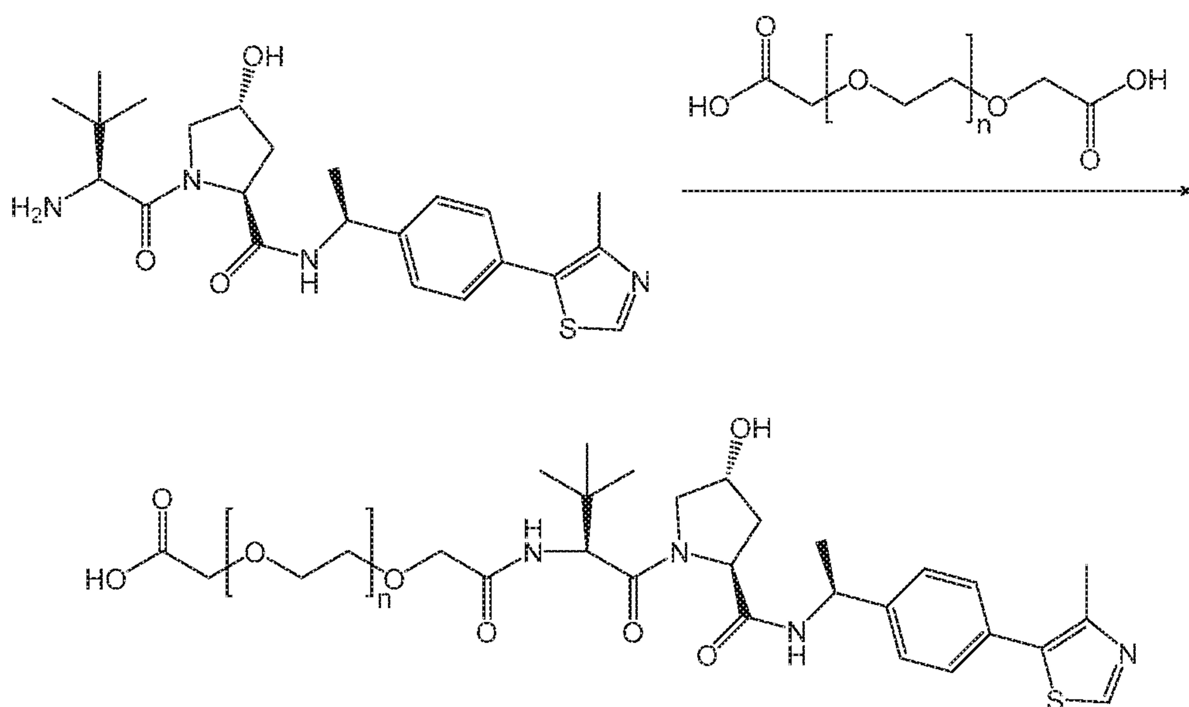
Scheme 11
