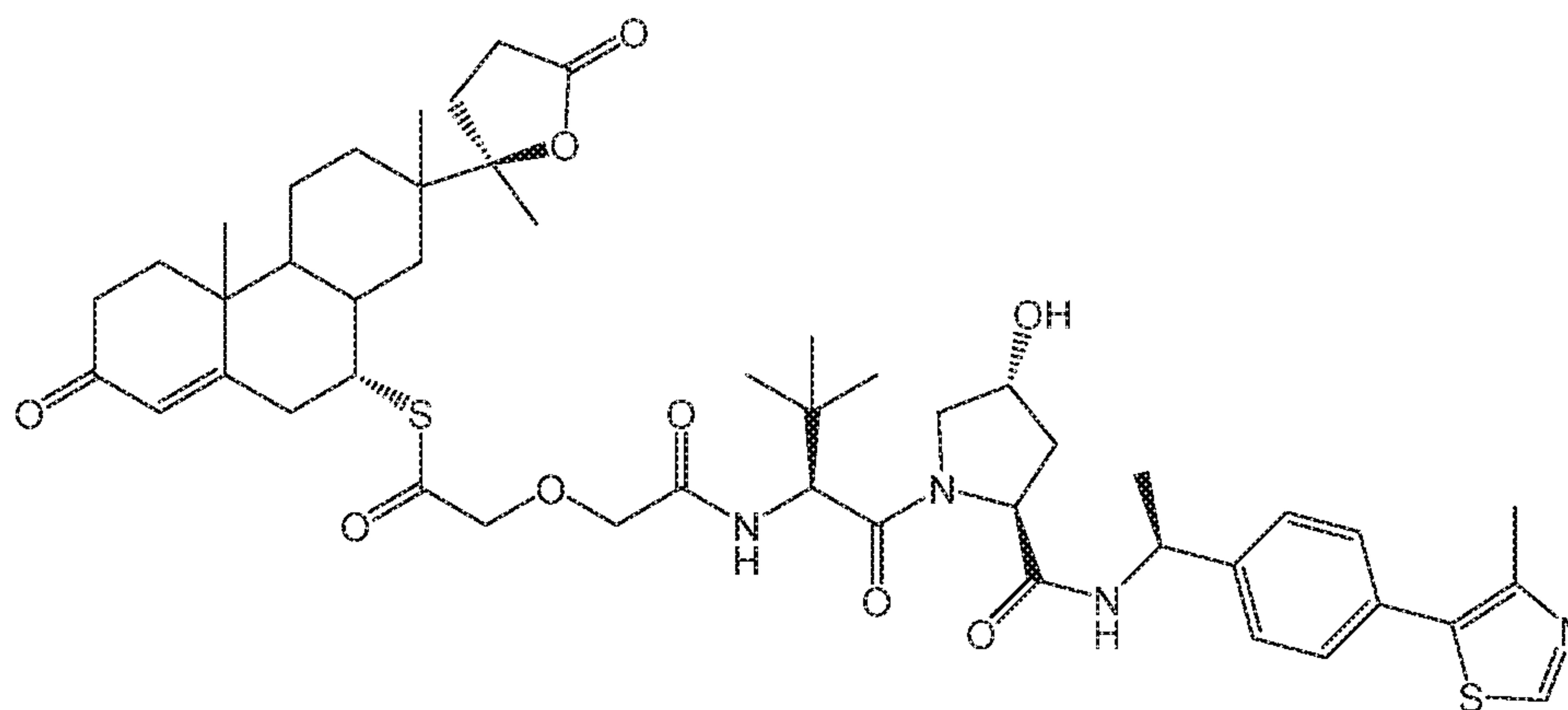
Compound 43
