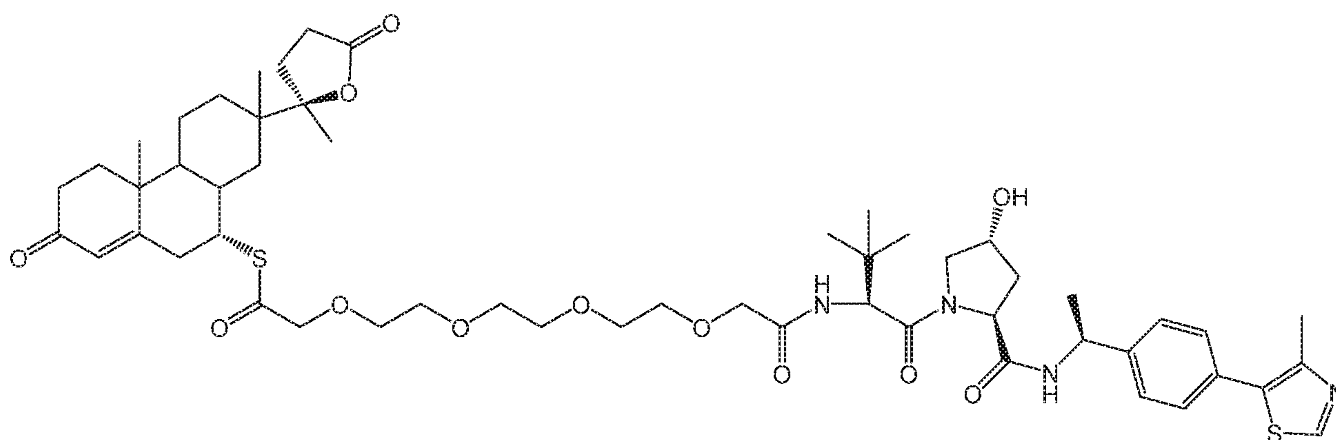
Compound 46
