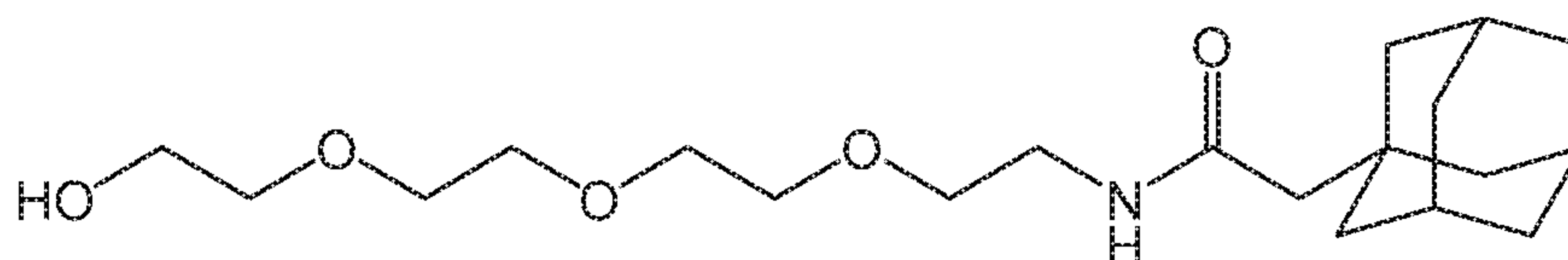
Compound 4
