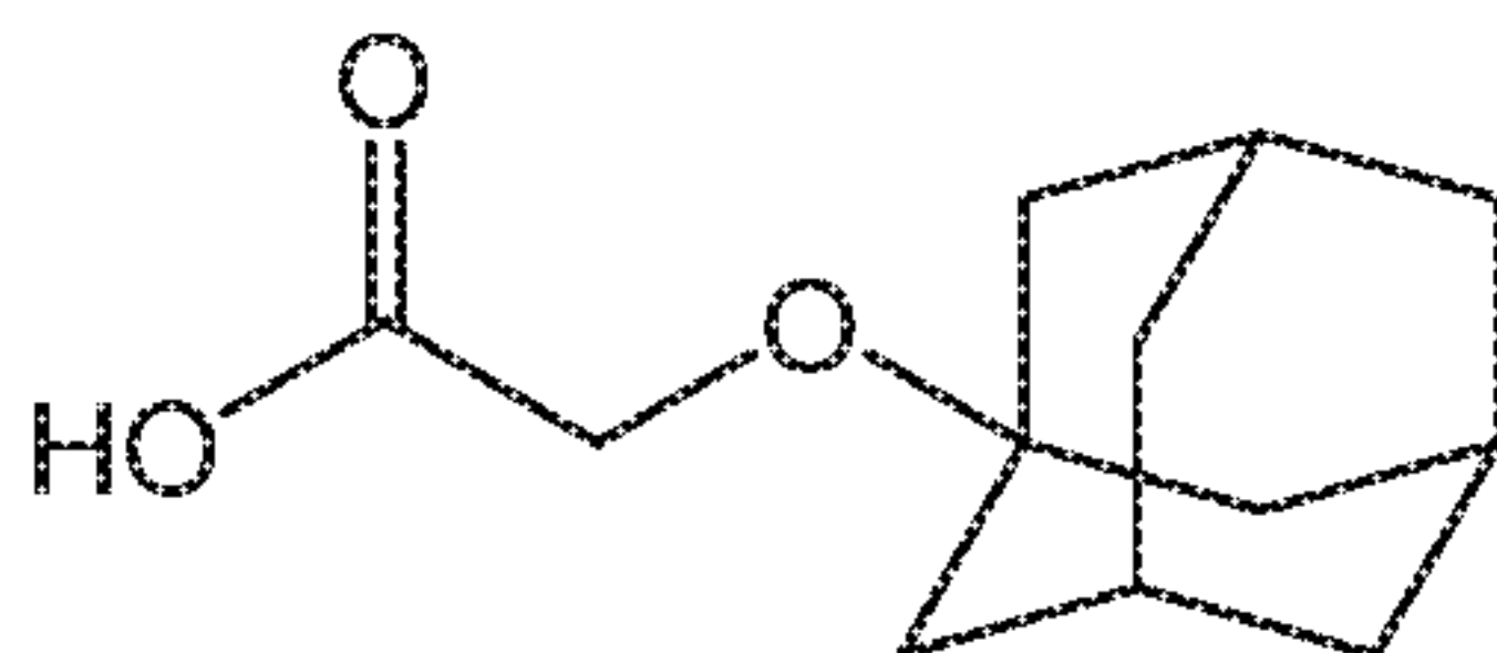
Compound 13
