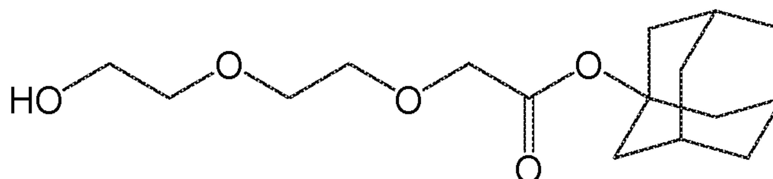
Compound 31
