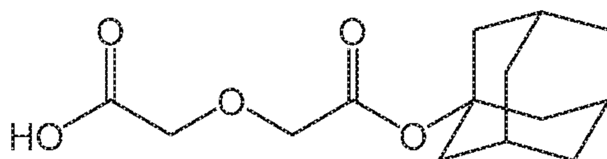
Compound 25
