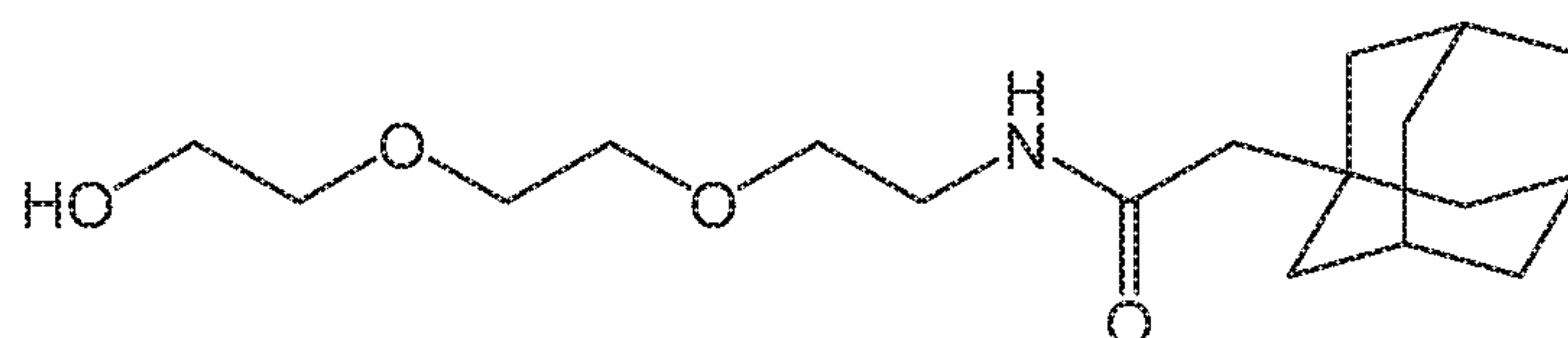
Compound 3
