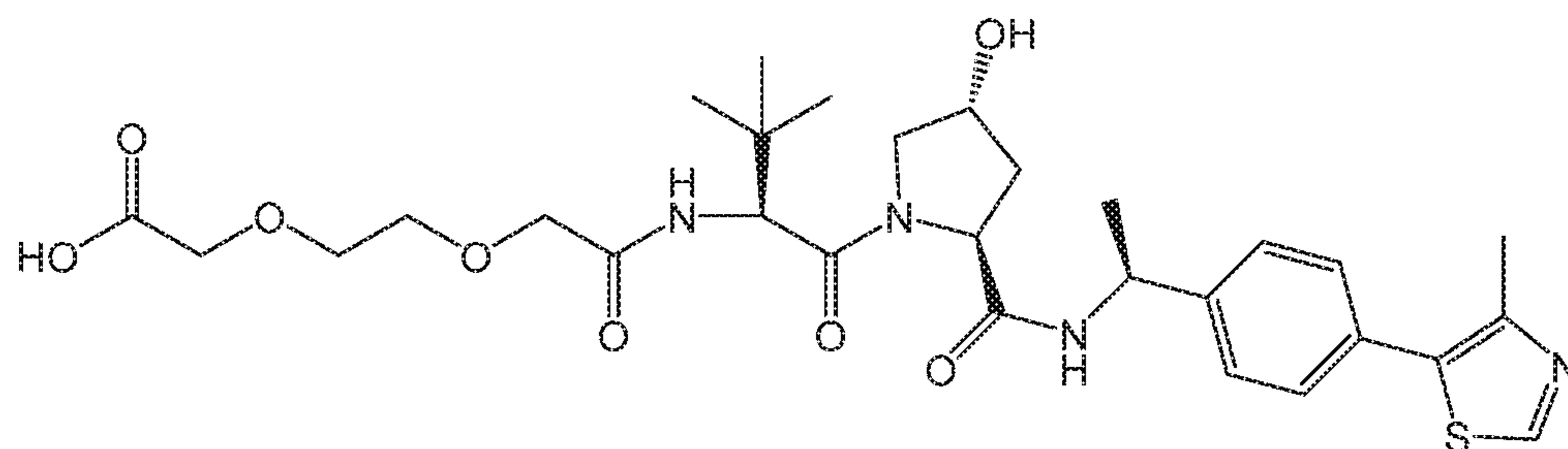
Compound 34
