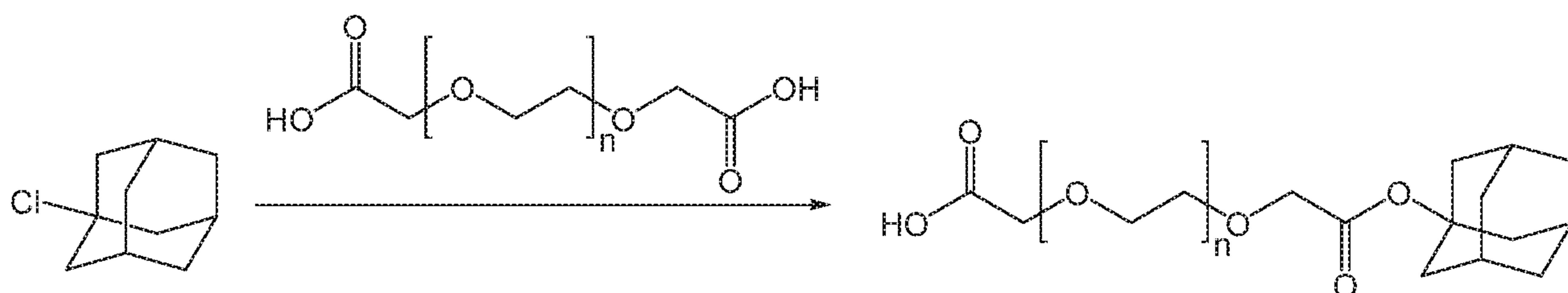
Scheme 9
