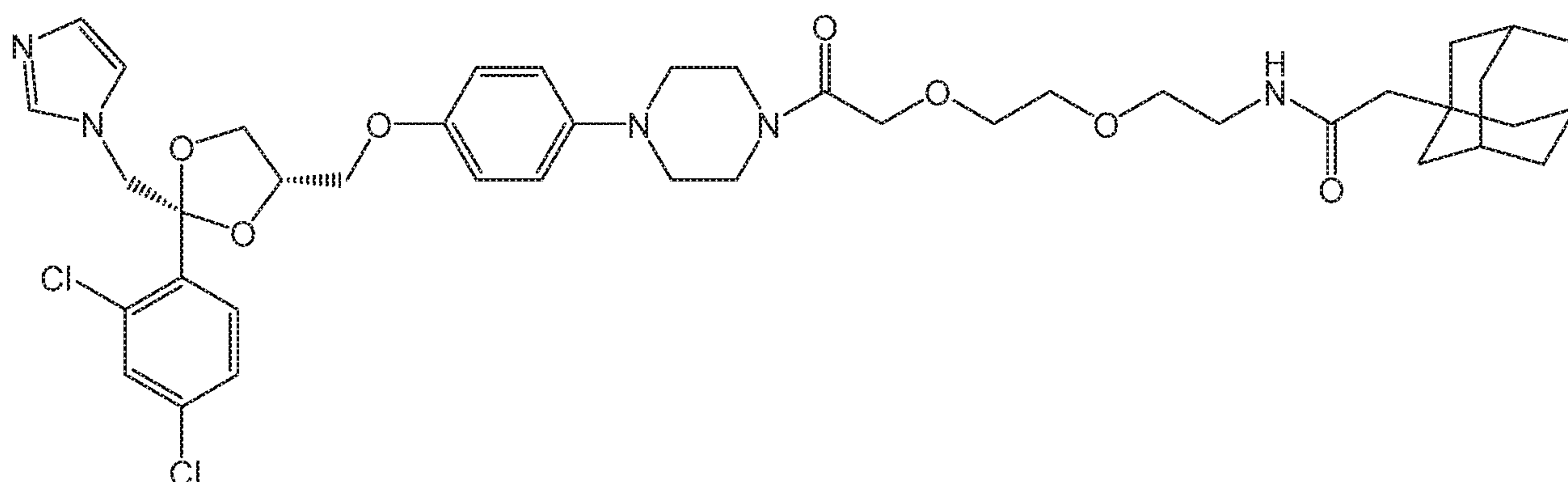
Compound 42
