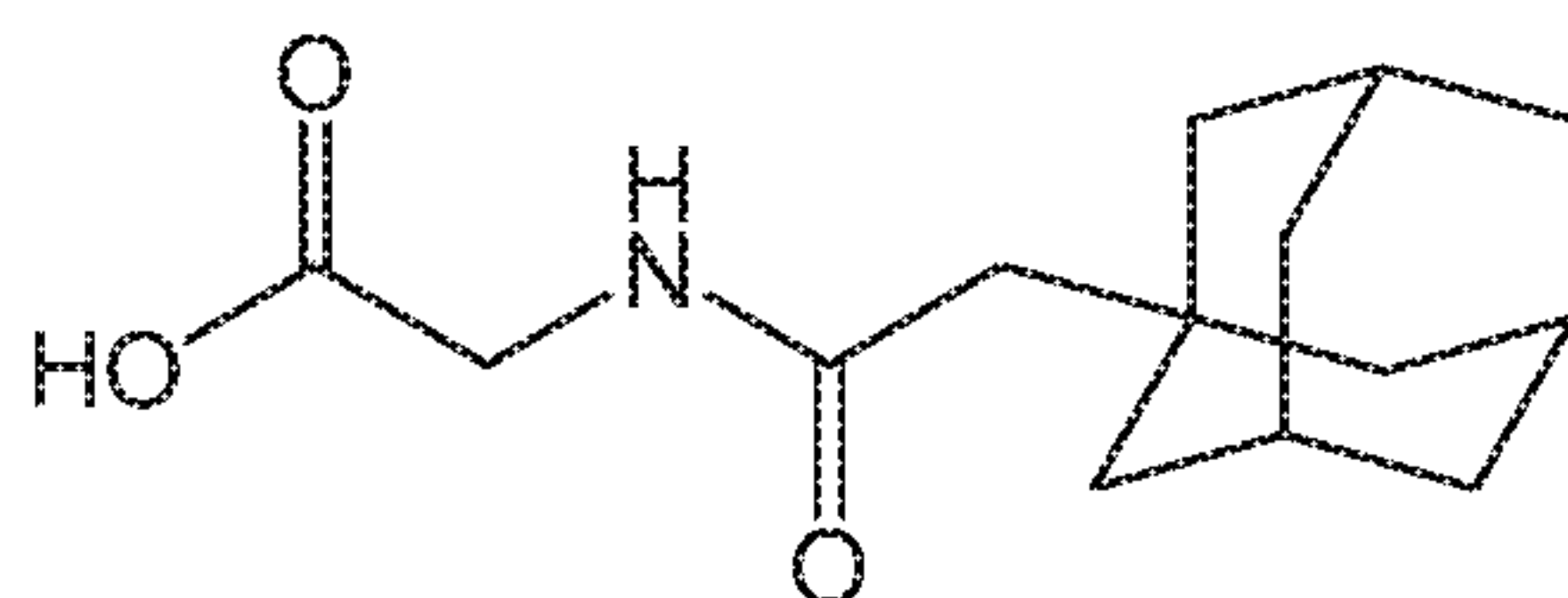
Compound 5
