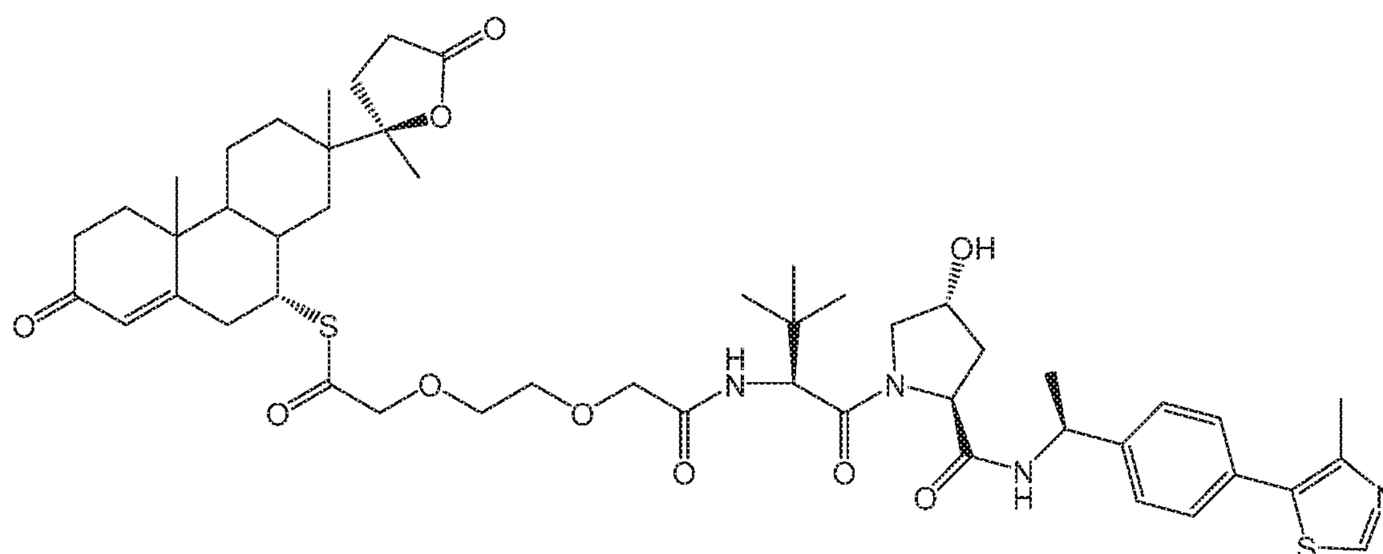
Compound 44
