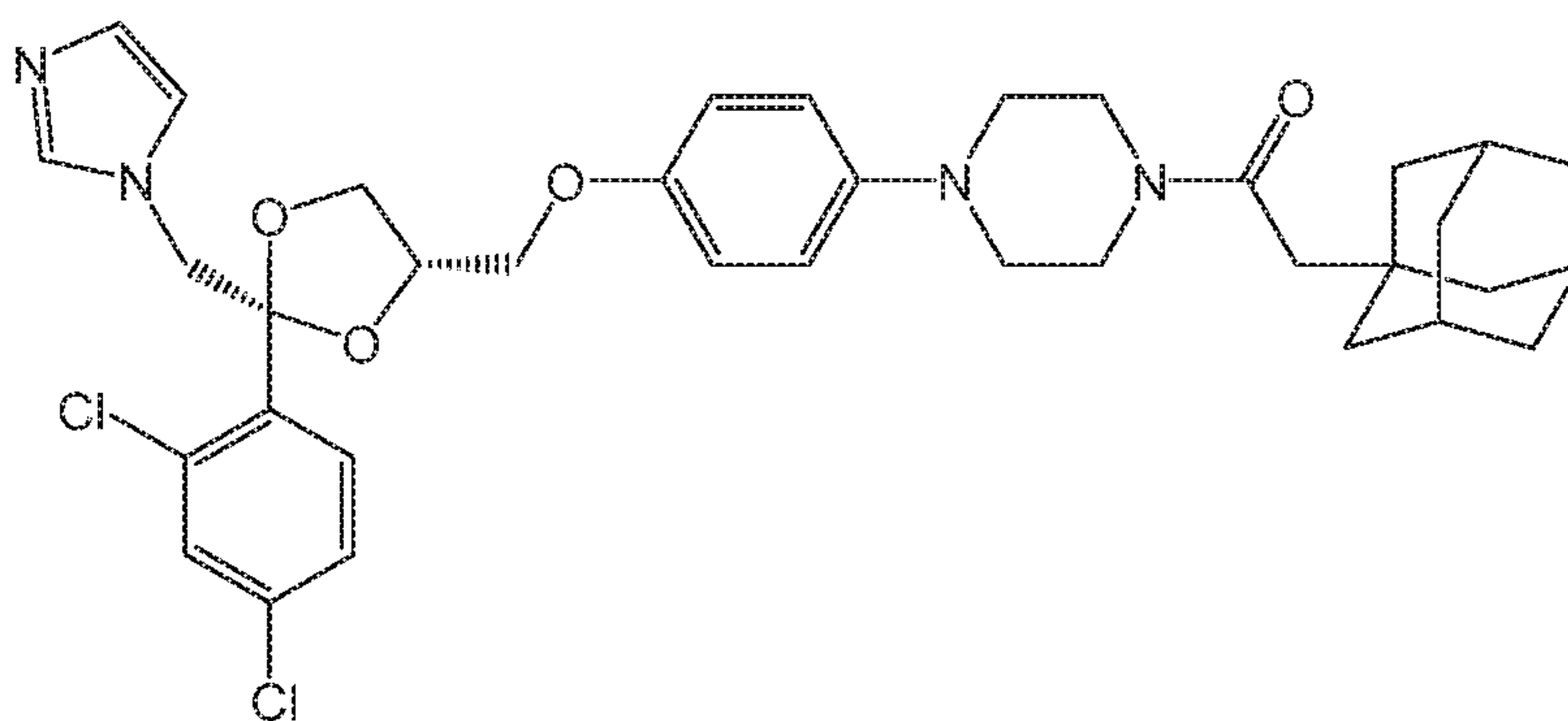
Compound 40
