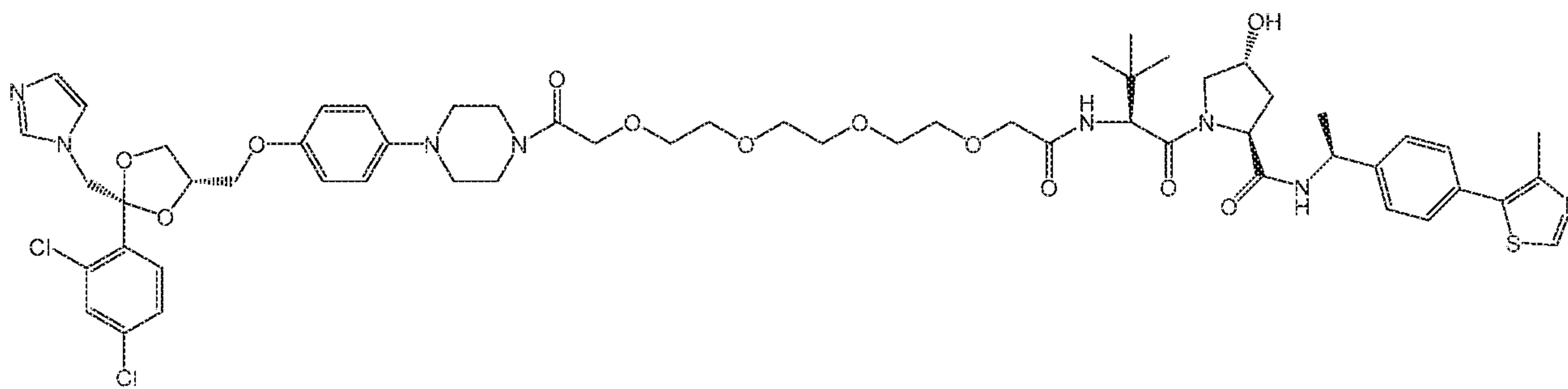
Compound 50
