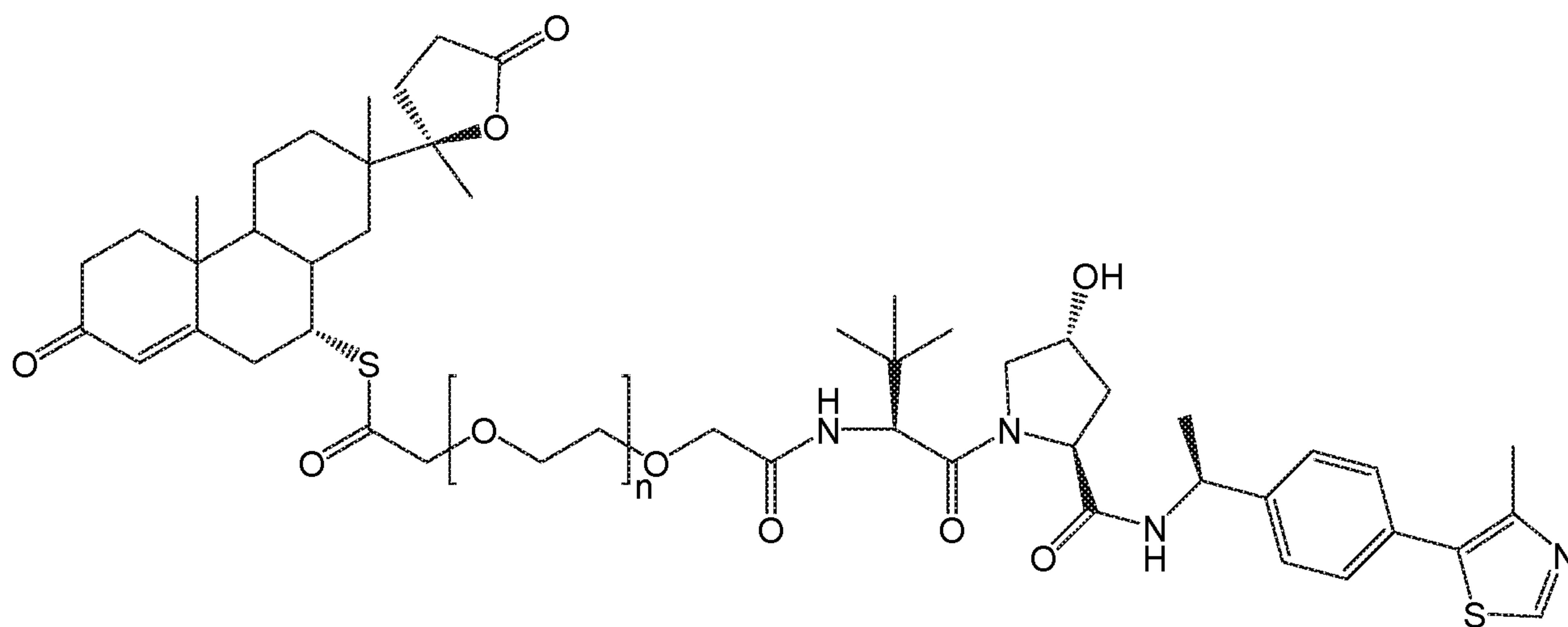
Scheme 18
