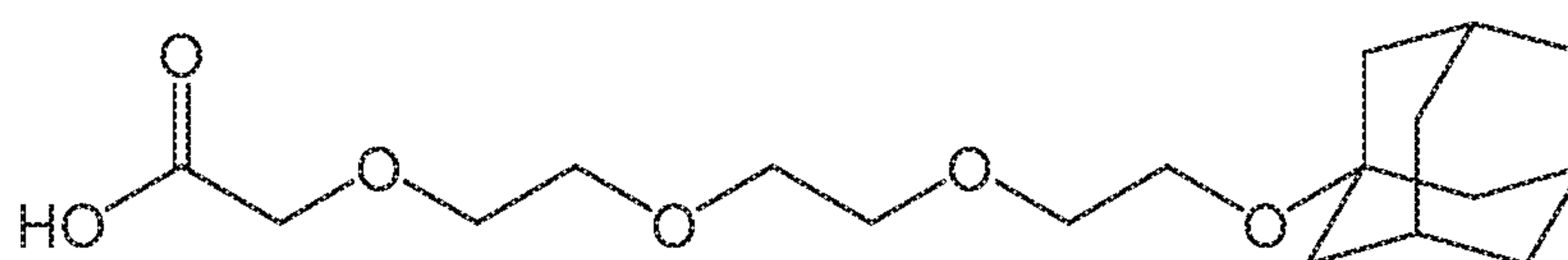
Compound 16
