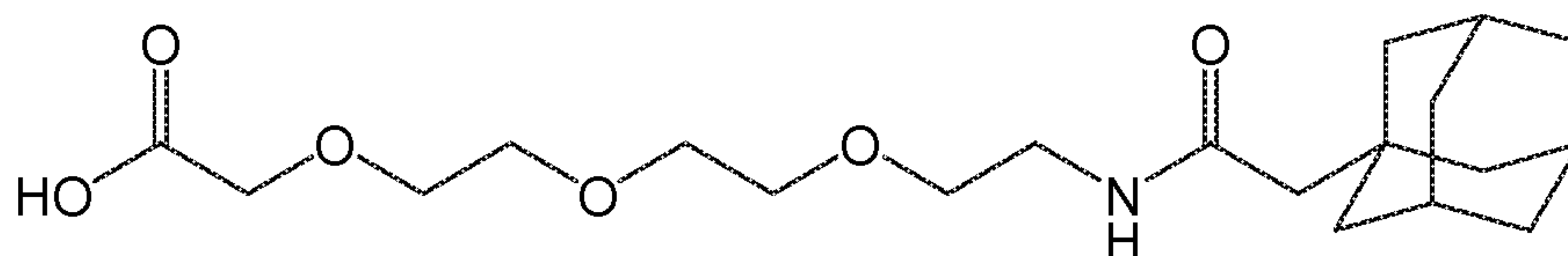
Compound 8
