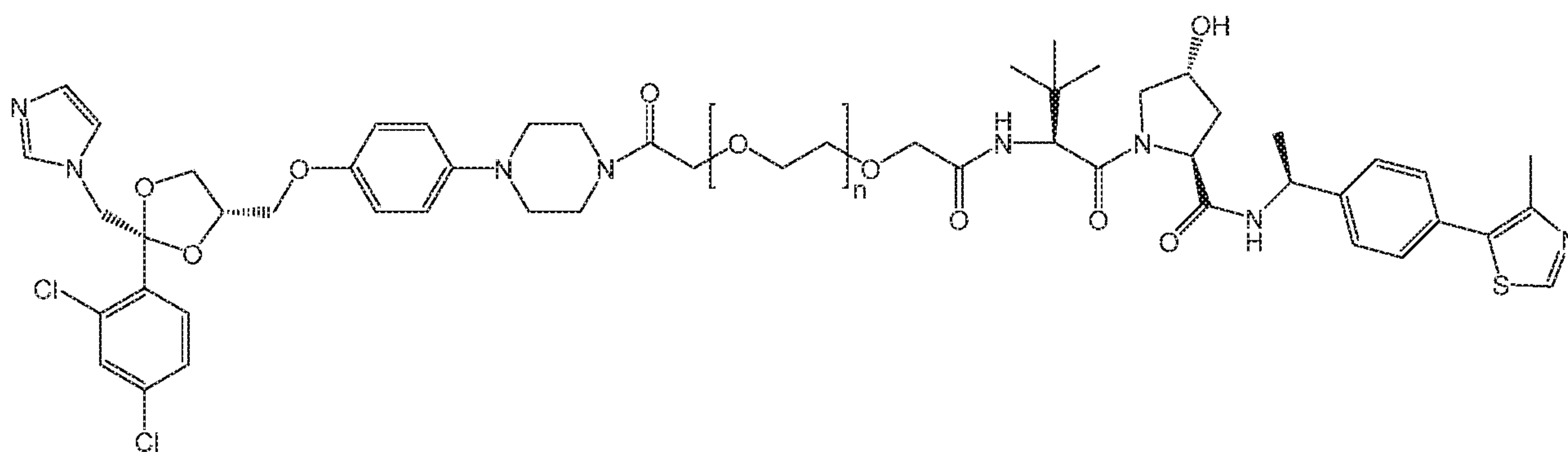
Scheme 19
