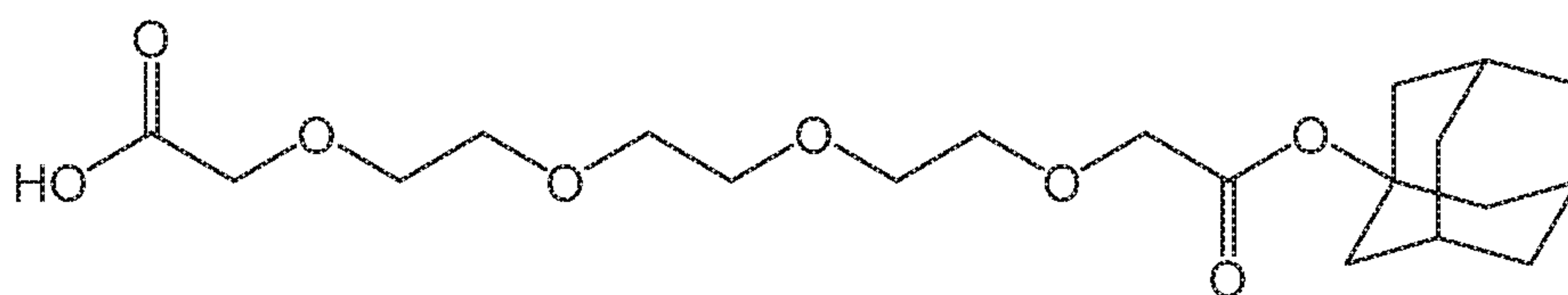
Compound 28
