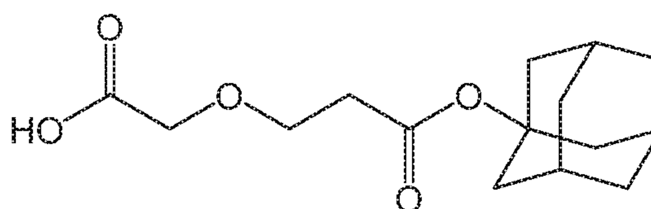
Compound 22
