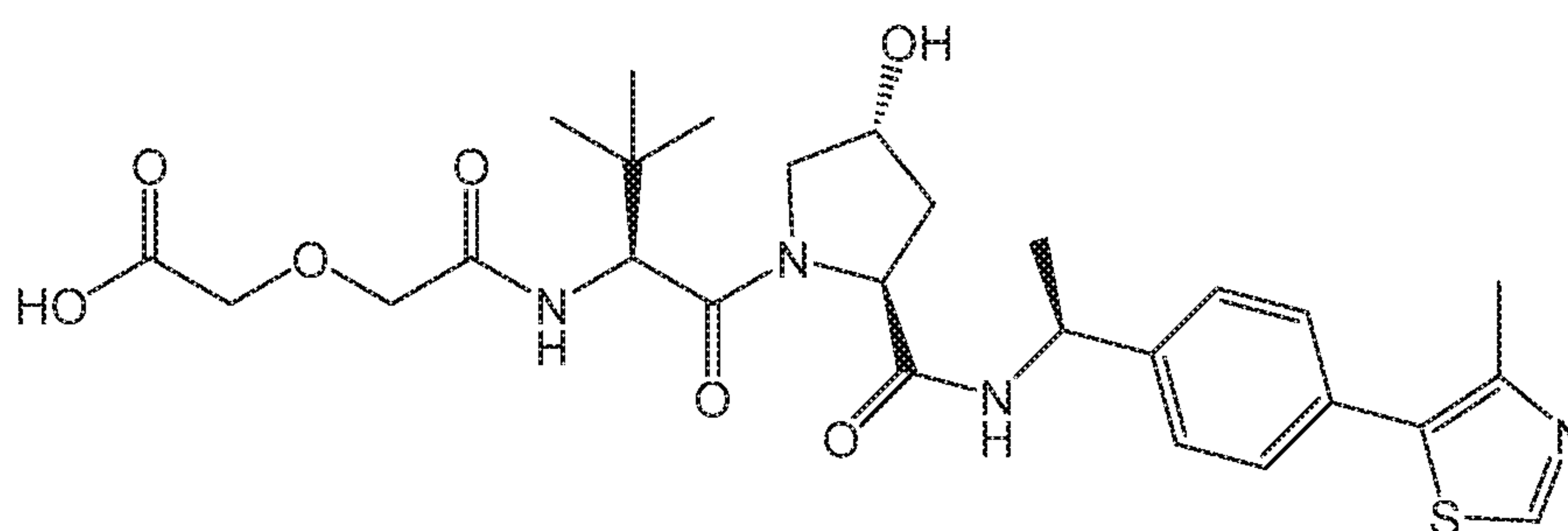
Compound 33
