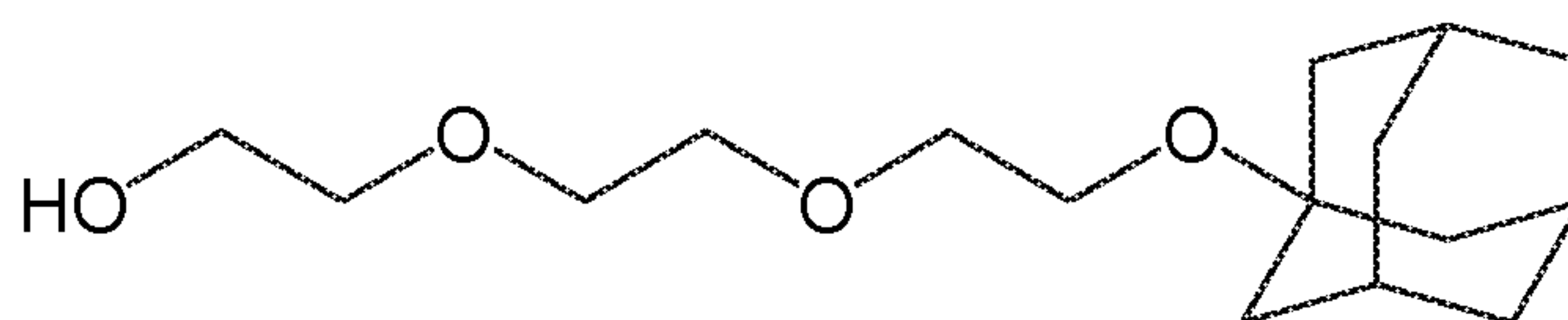
Compound 11
