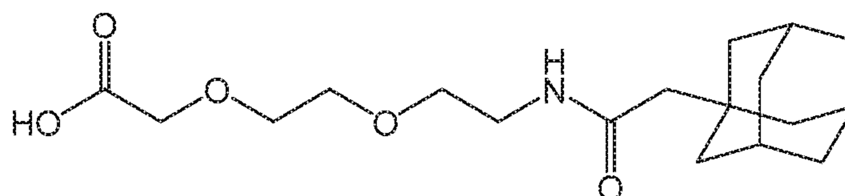
Compound 7
