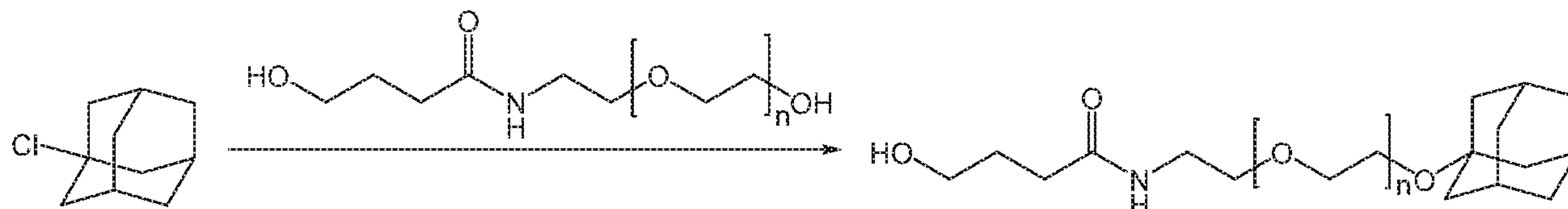
Scheme 7
