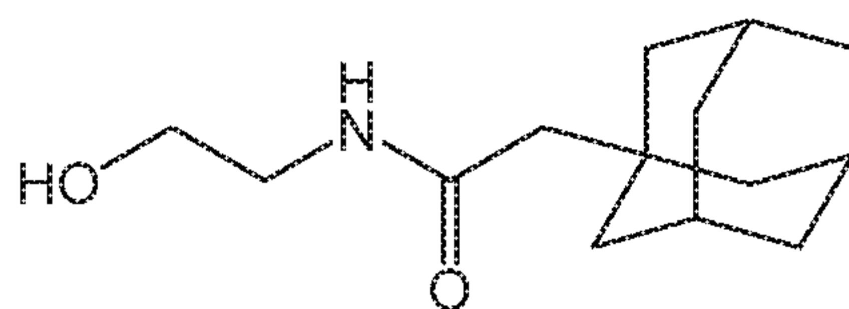
Compound 1
