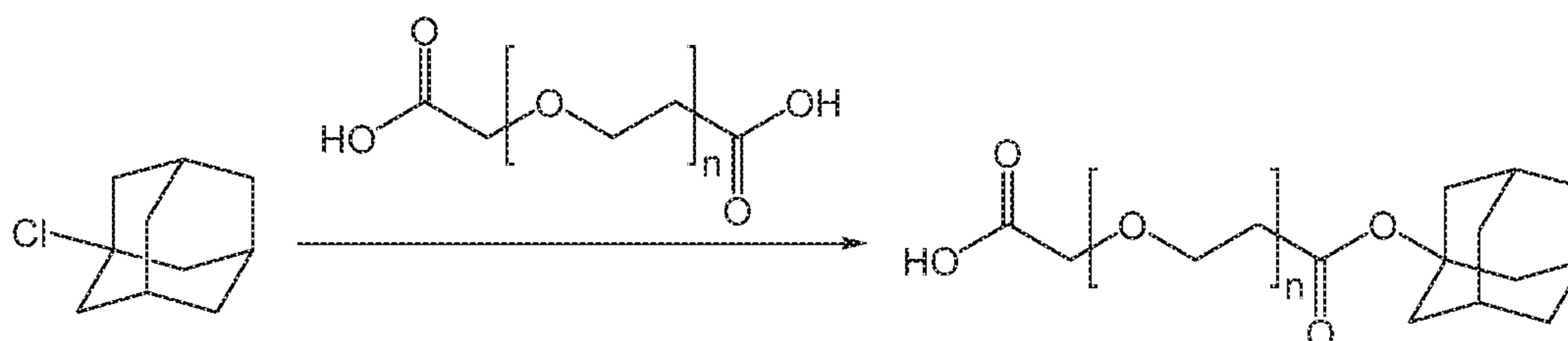
Scheme 8
