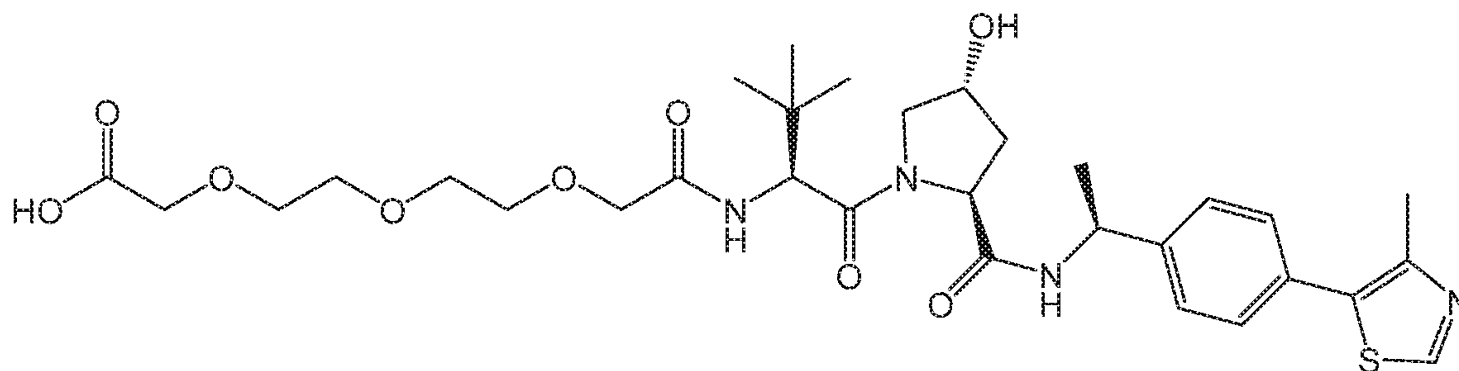
Compound 35
