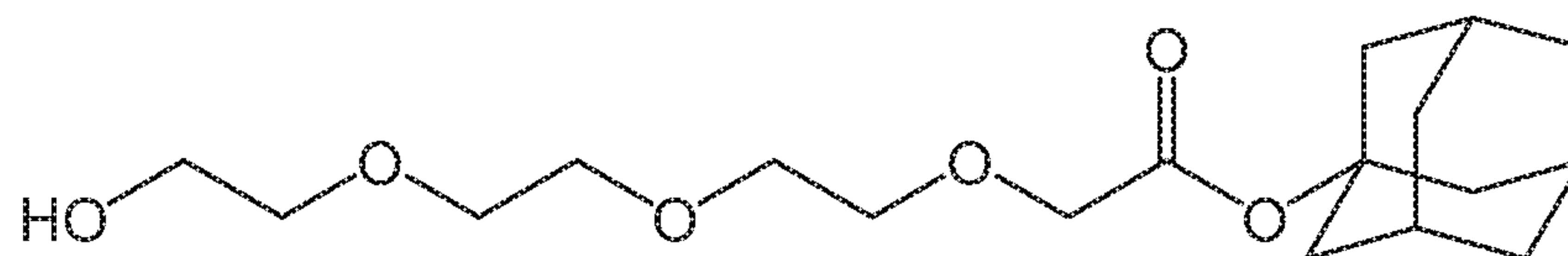
Compound 32
