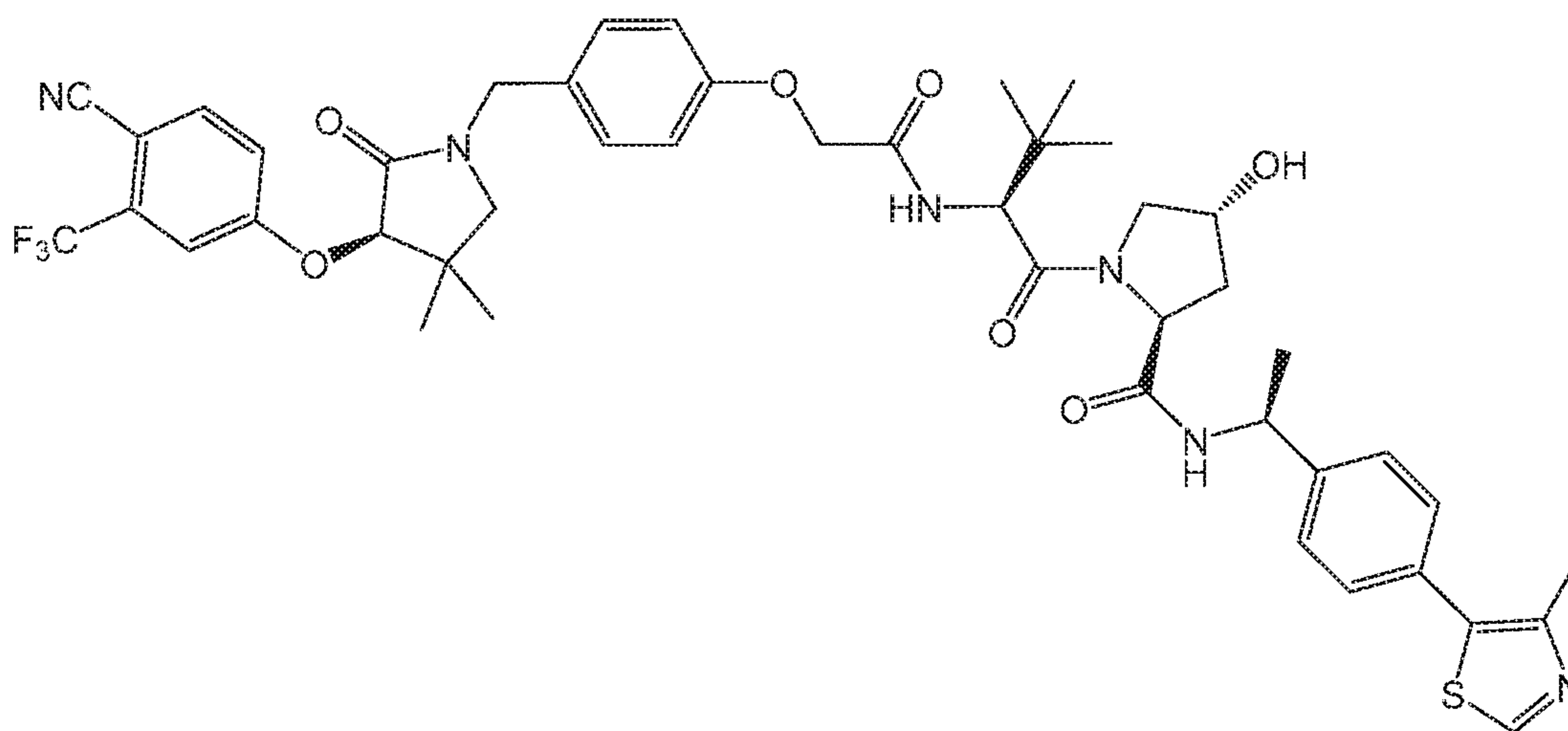
Compound 53
