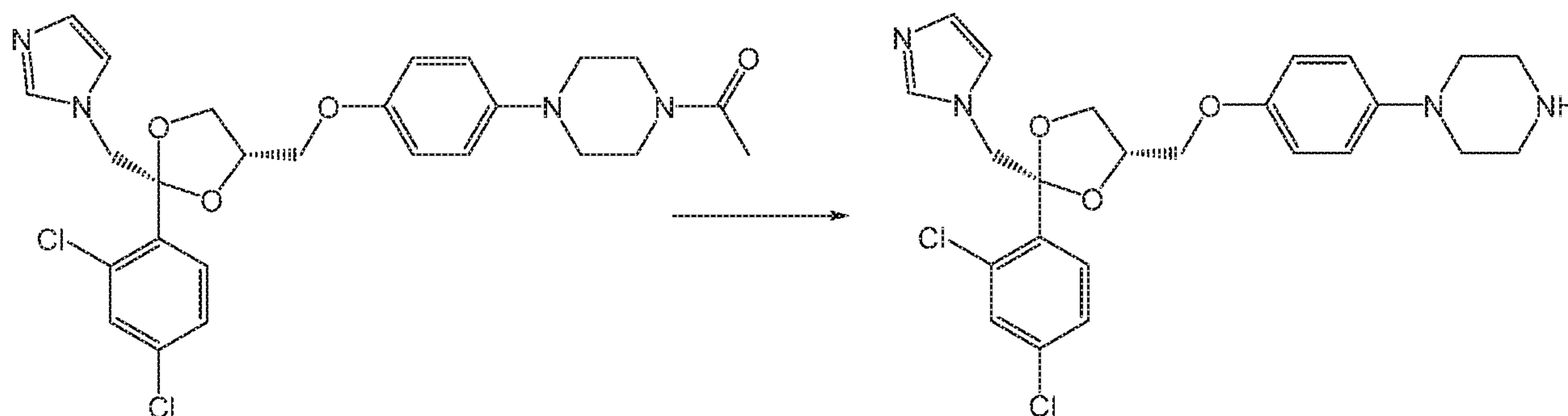
Scheme 13
