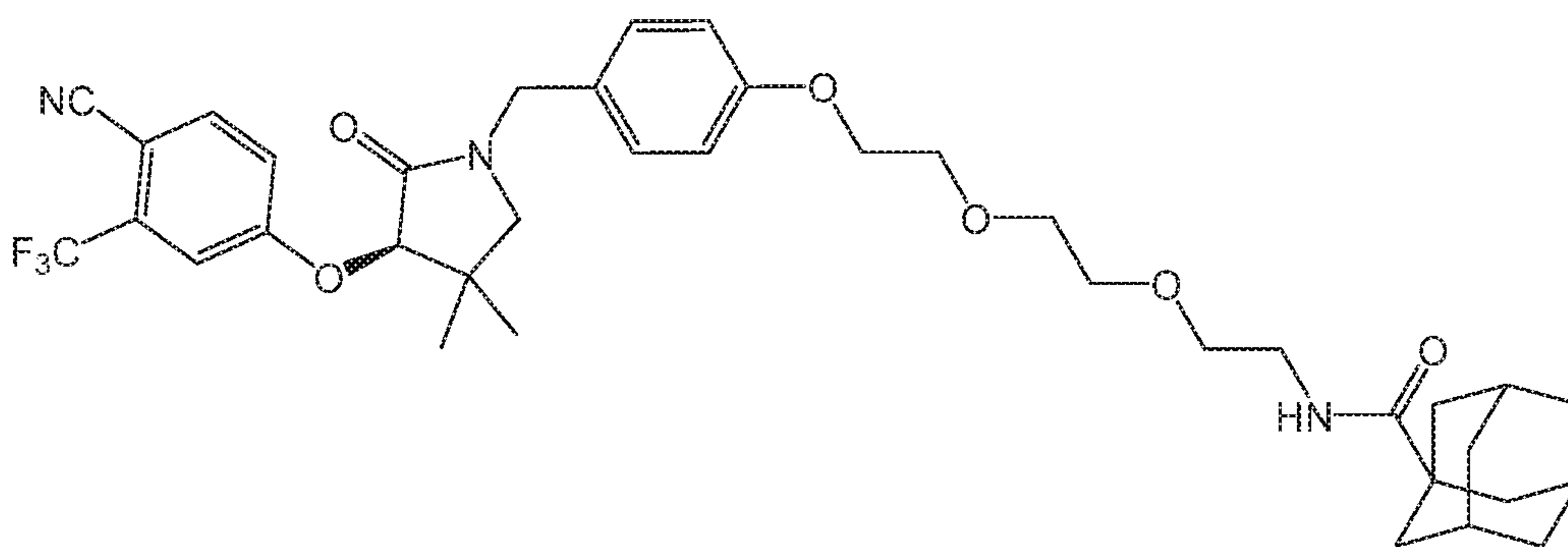
Compound 52
