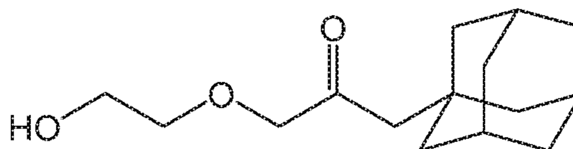
Compound 30
