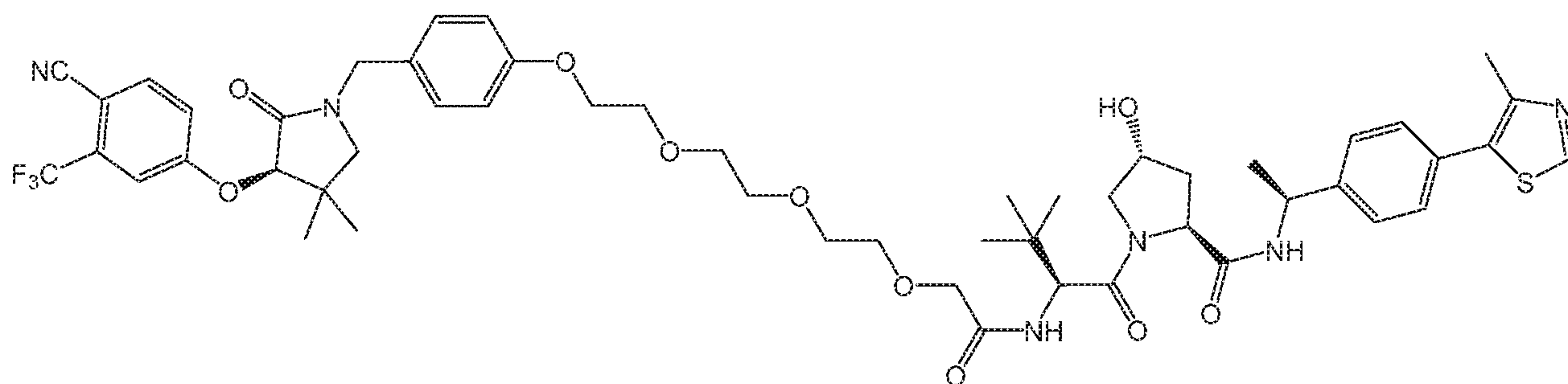
Compound 54
