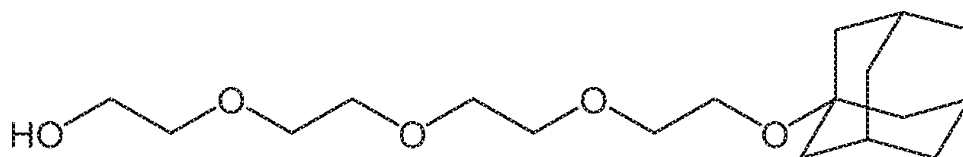
Compound 12
