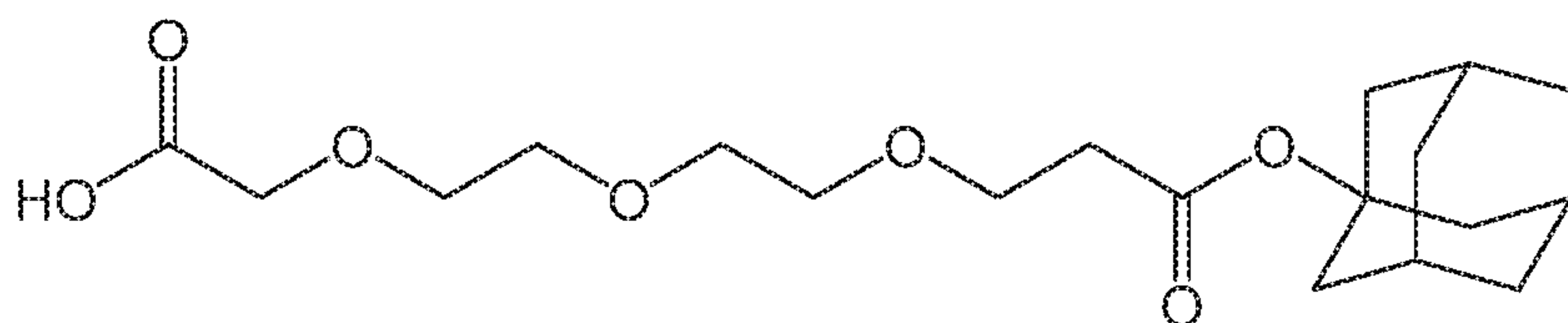
Compound 24
