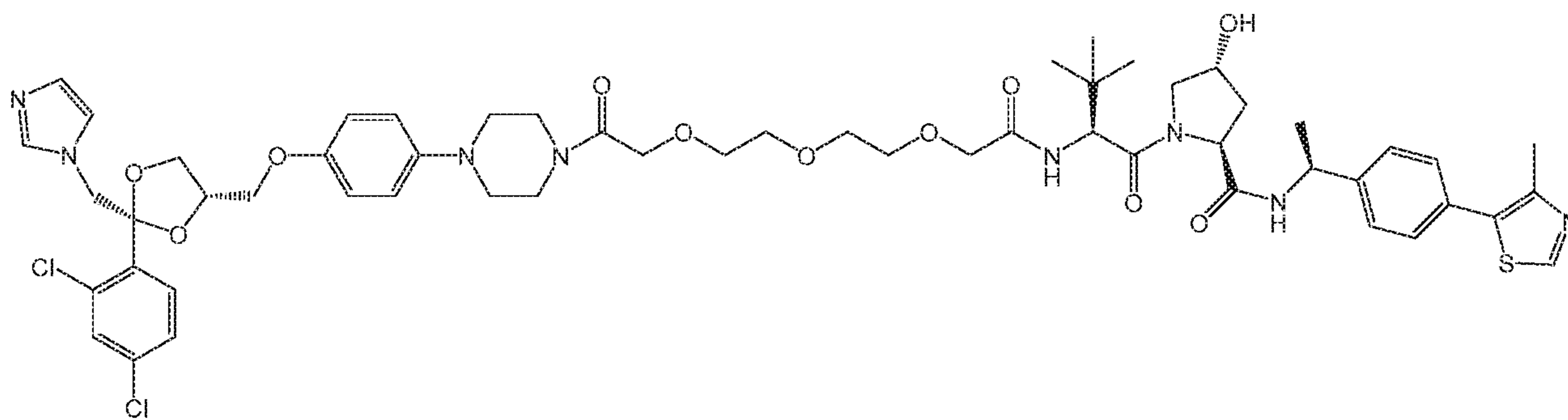
Compound 49
