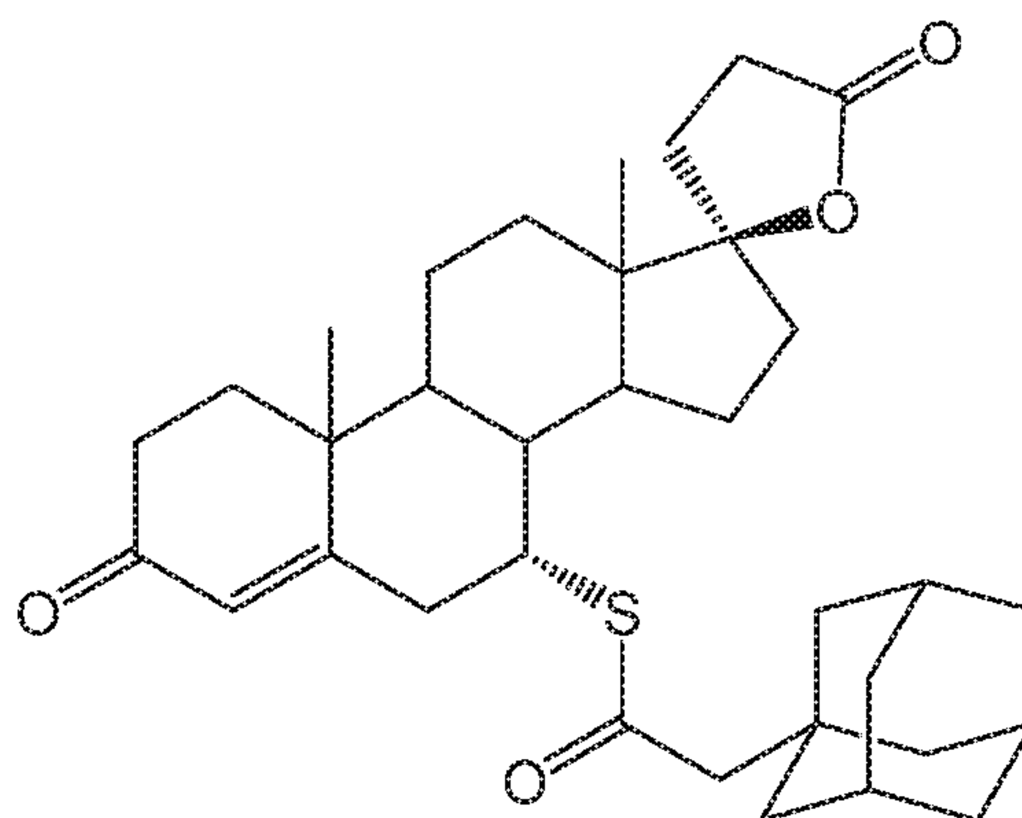
Compound 37
