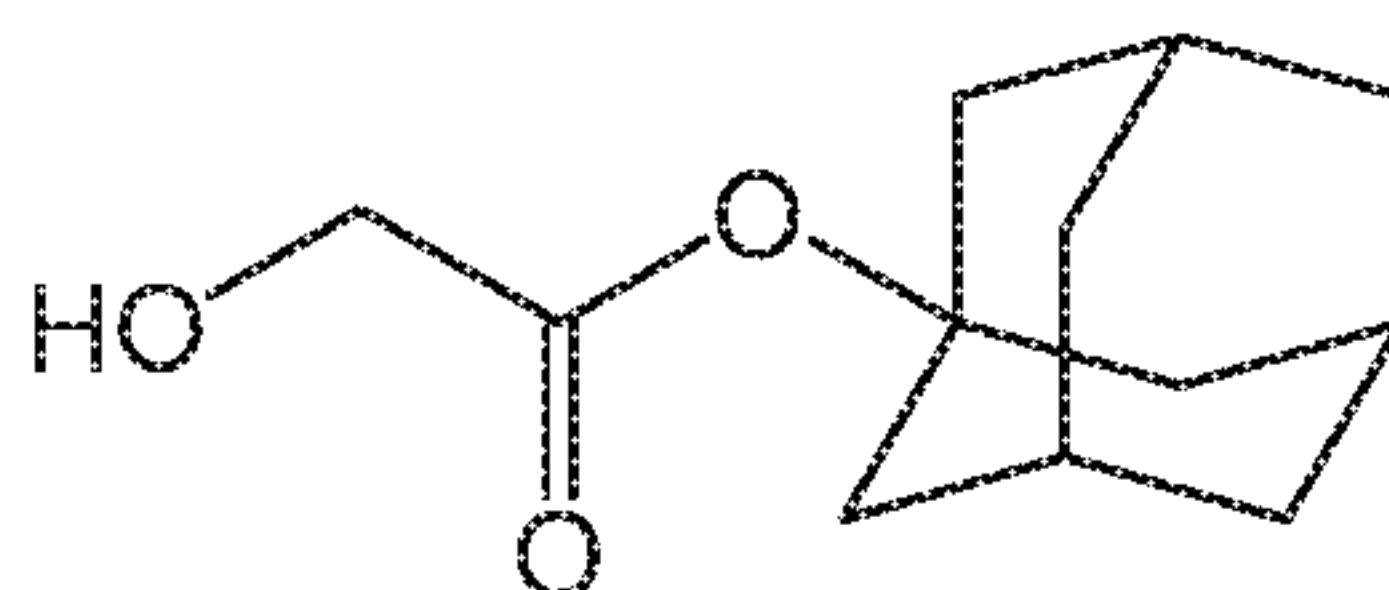
Compound 29
