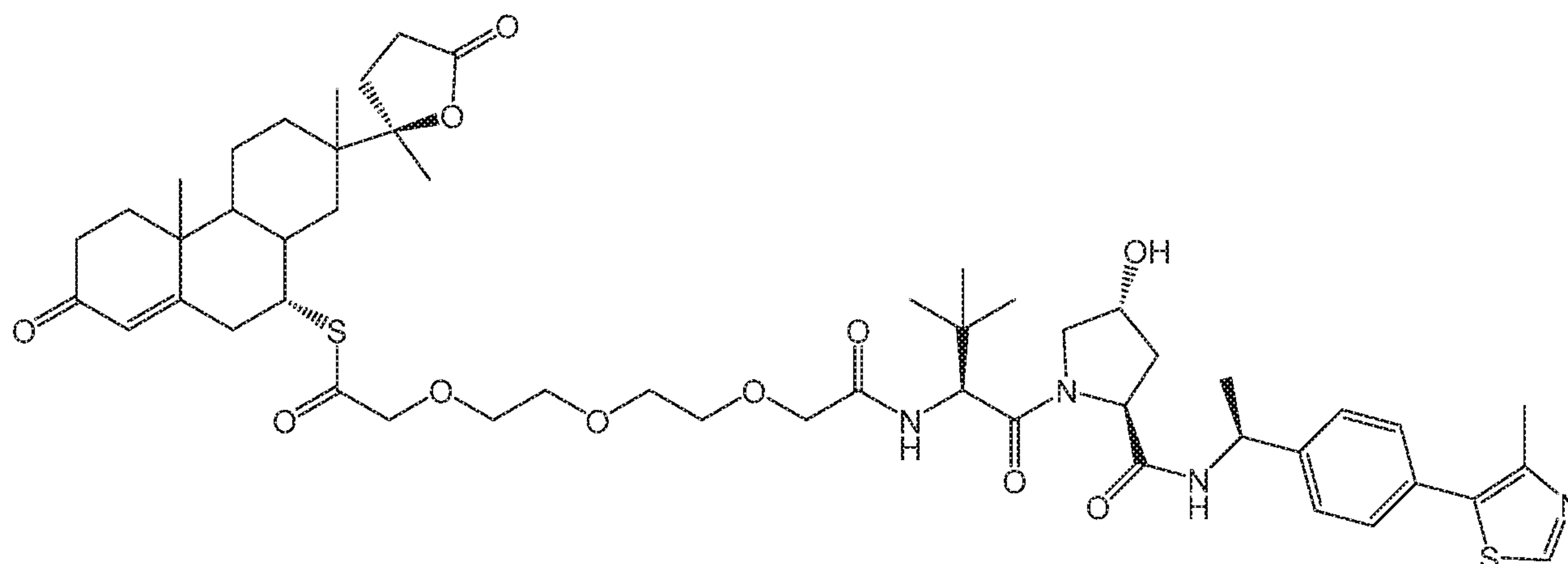
Compound 45
