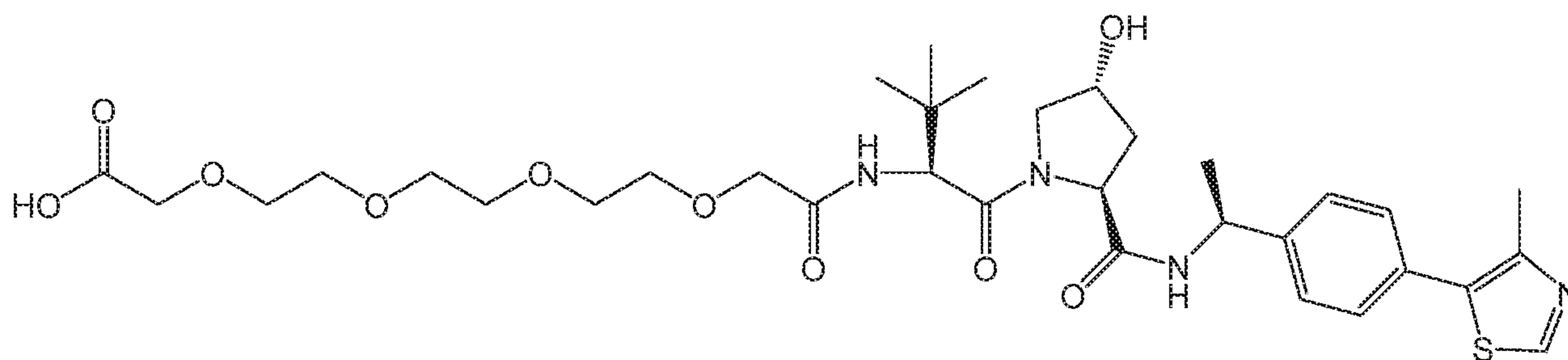
Compound 36
