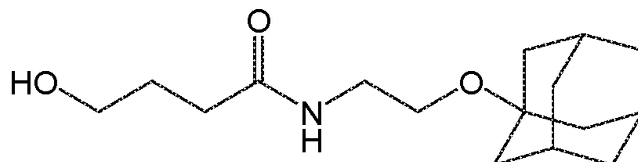
Compound 17
