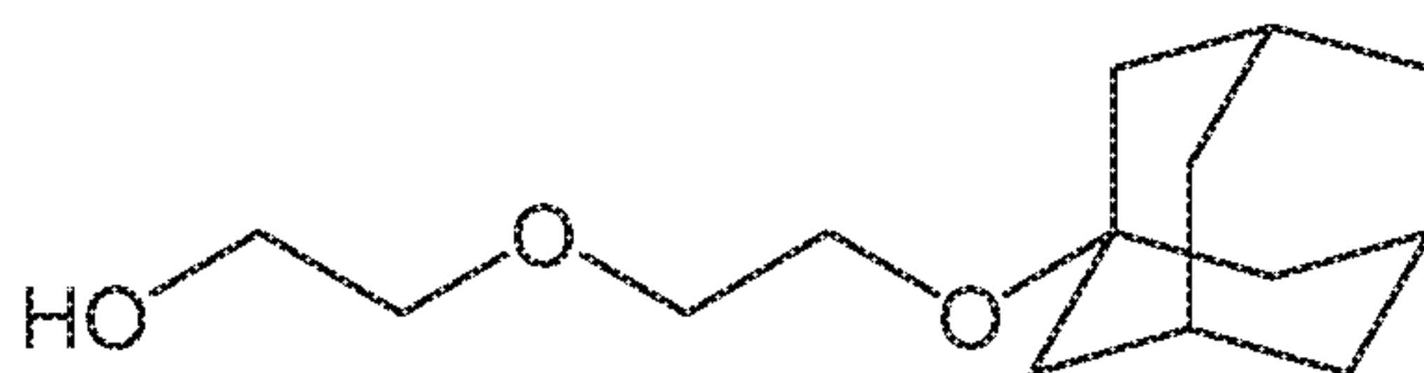
Compound 10
