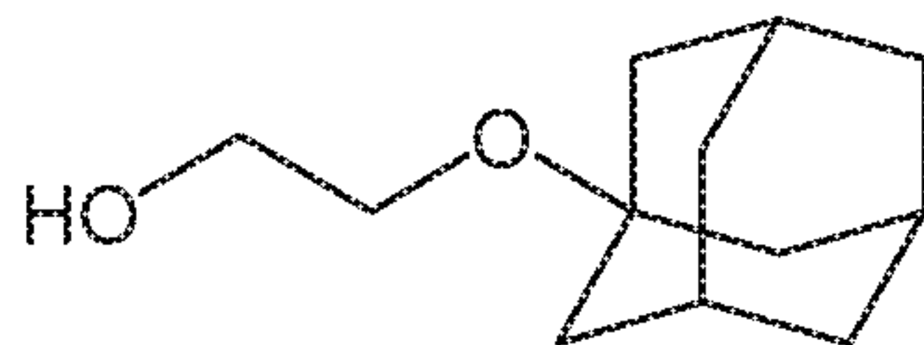
Compound 9
