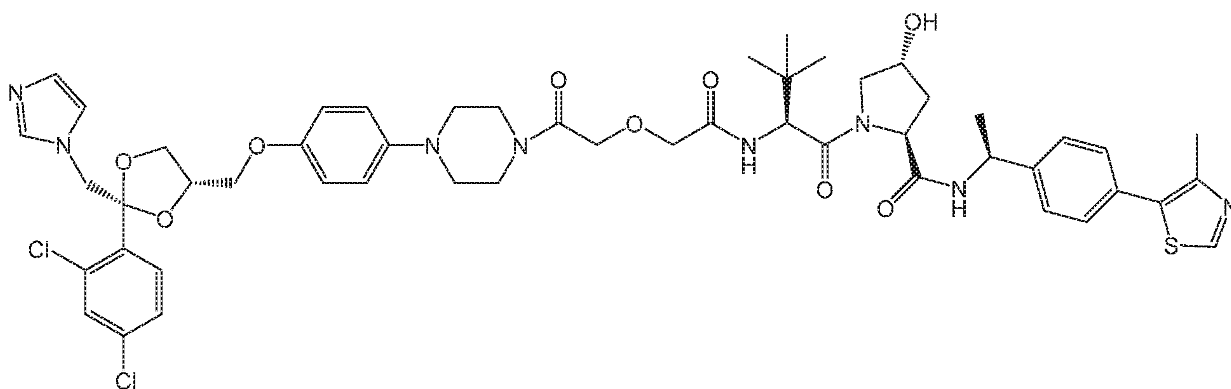
Compound 47
