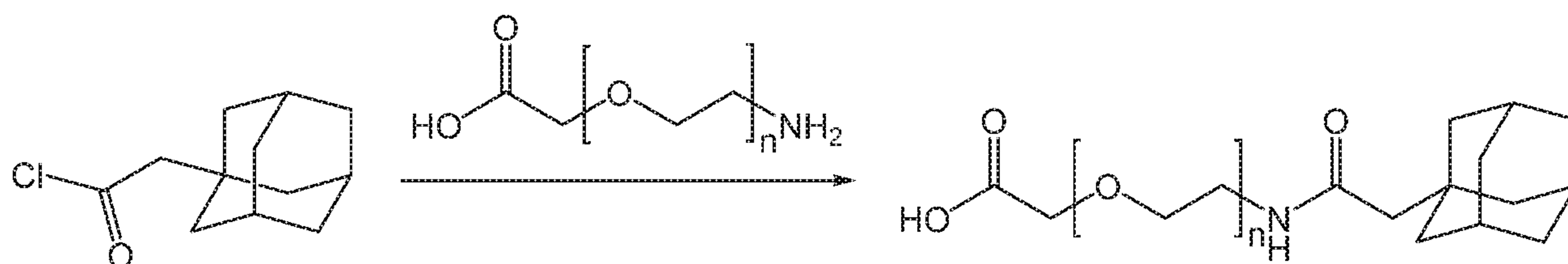
Scheme 4
