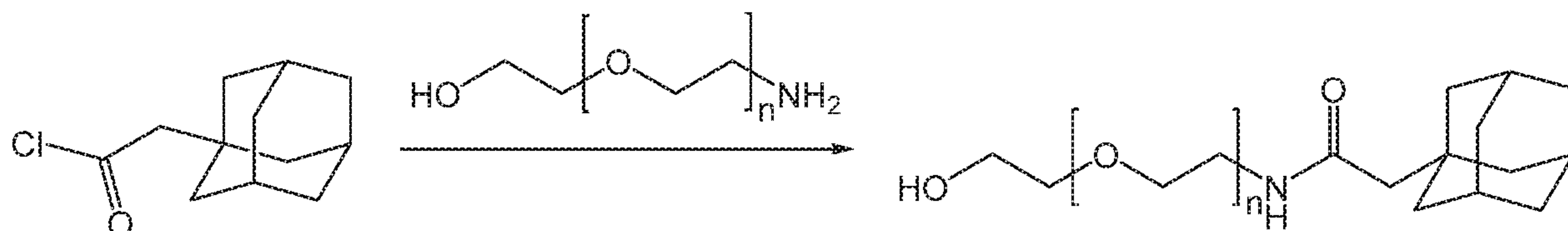
Scheme 3
