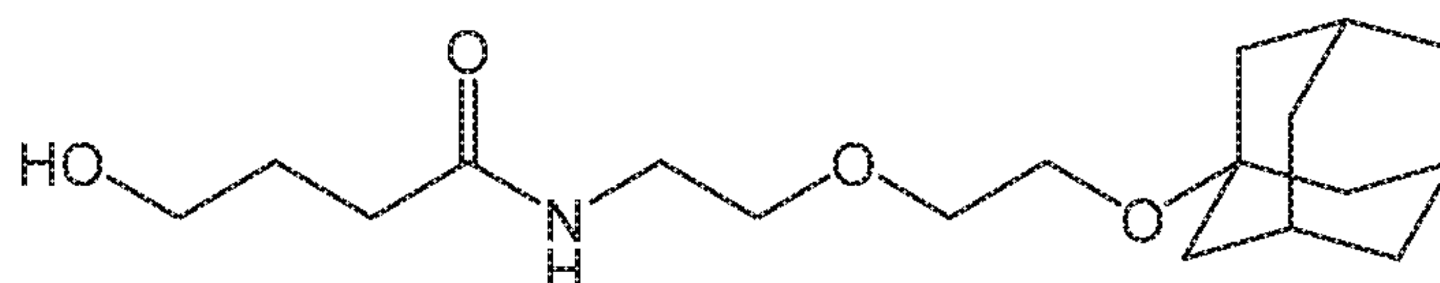
Compound 18
