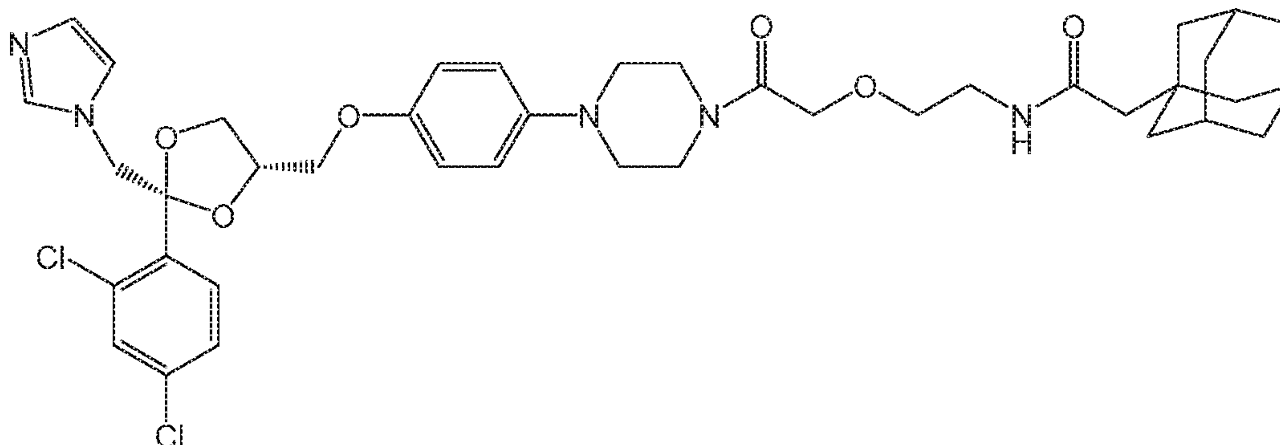
Compound 41
