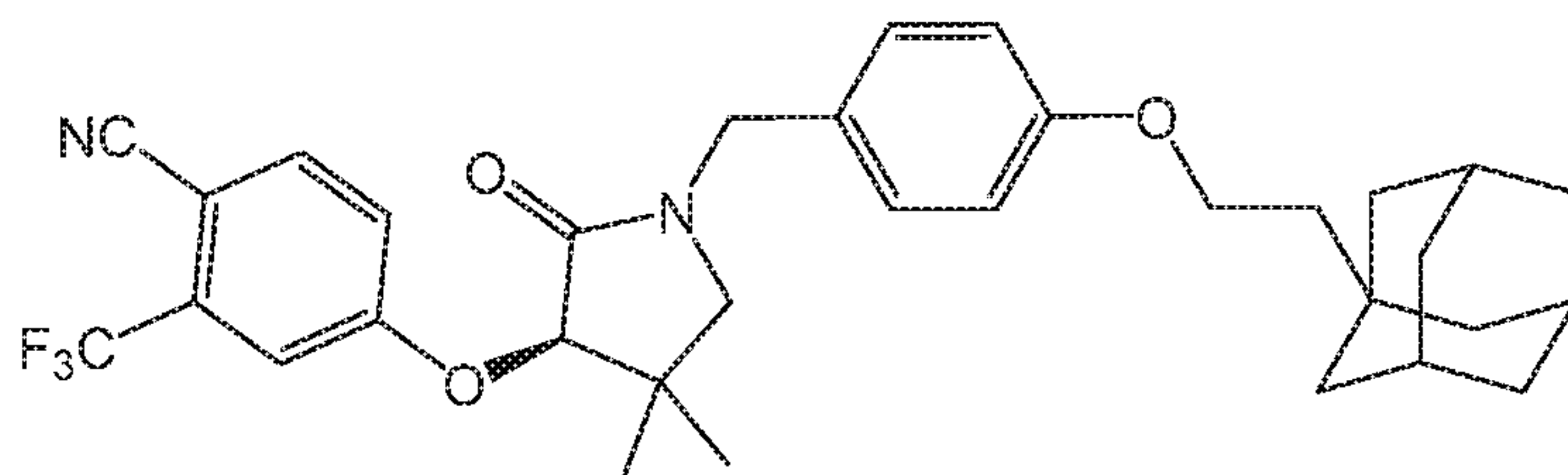
Compound 51
