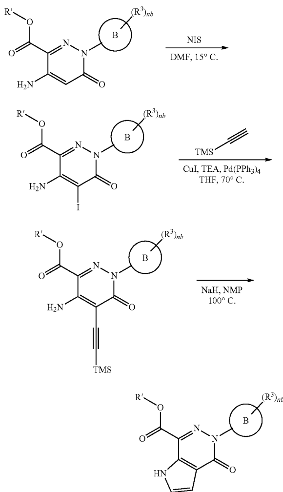
[Reaction Scheme 6C]
