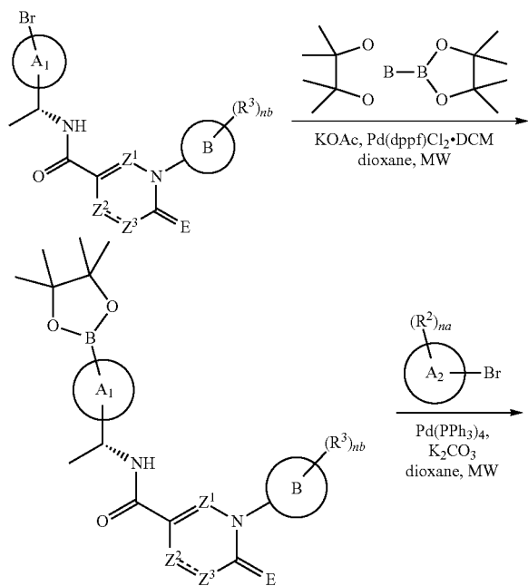
[Reaction Scheme 1C]
