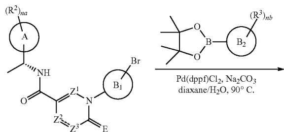
[Reaction Scheme 1F]
