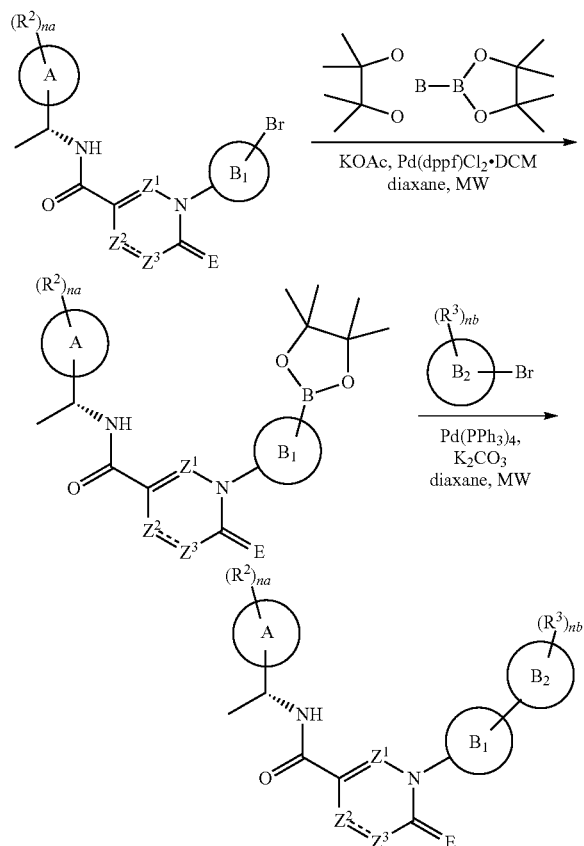
[Reaction Scheme 1E]
