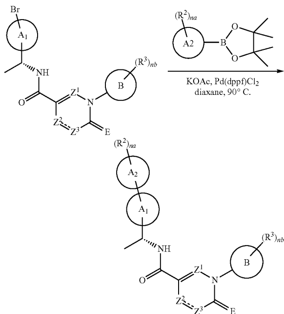
[Reaction Scheme 1D]
