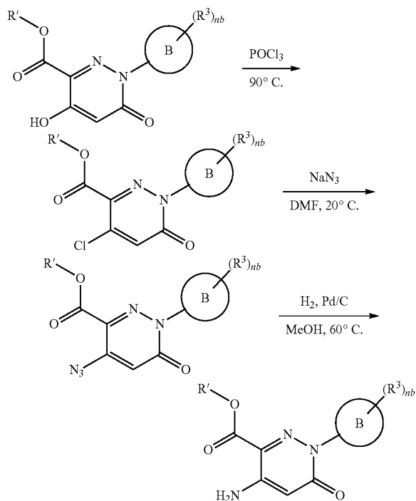
[Reaction Scheme 6B]
