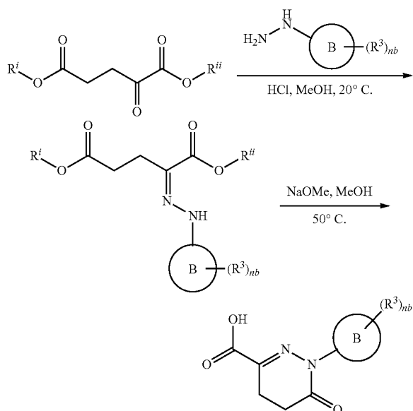
[Reaction Scheme 6A]
